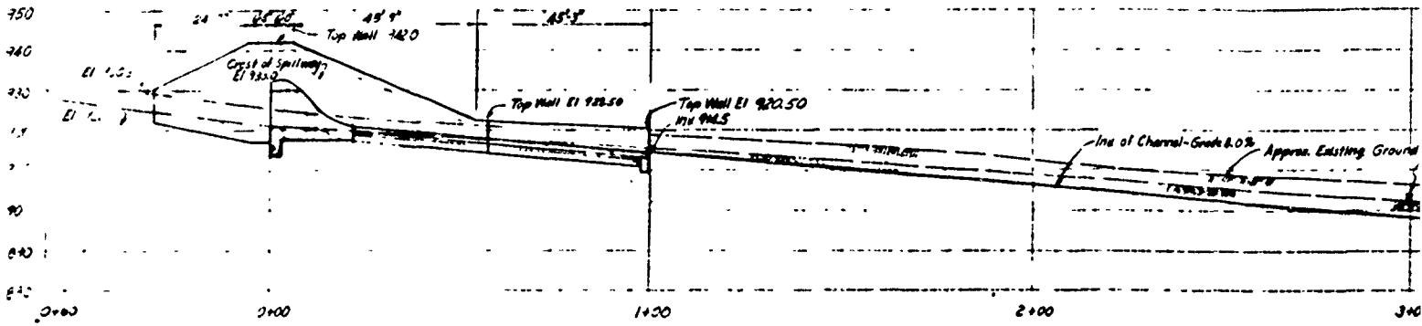
PROFILE ALONG & SPILLWAY
