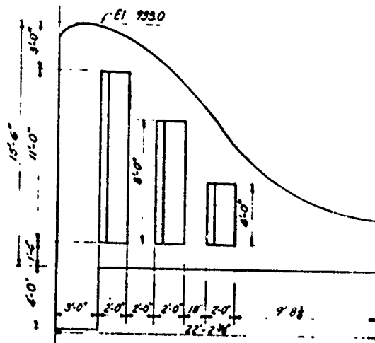
Elevation of Keyway in Spillway Scale: 1"=1'-0"
