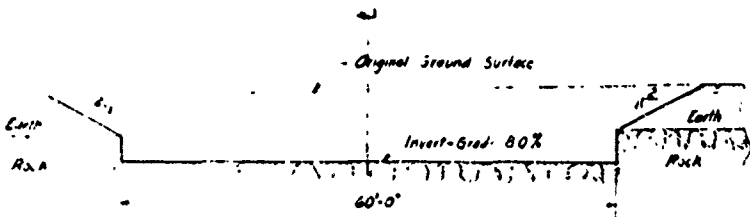
TYPICAL EXCAVATED SPILLWAY CHANNEL SECTION
