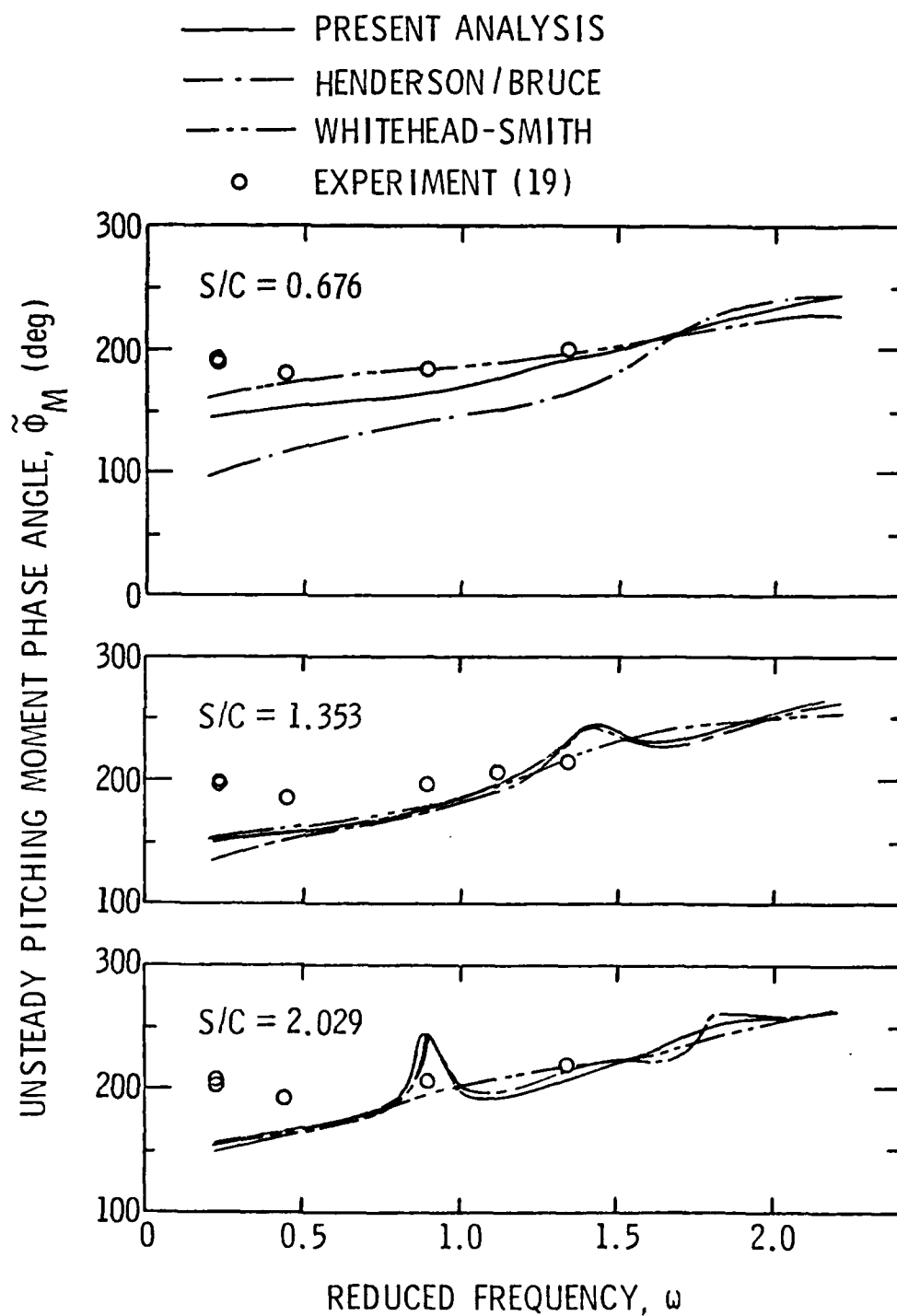
Figure 21. Comparison of Experimental and Theoretical Unsteady Pitching Moment Phase Angles with x_m + y_m^+ = 0 and \alpha = 35^\circ .
