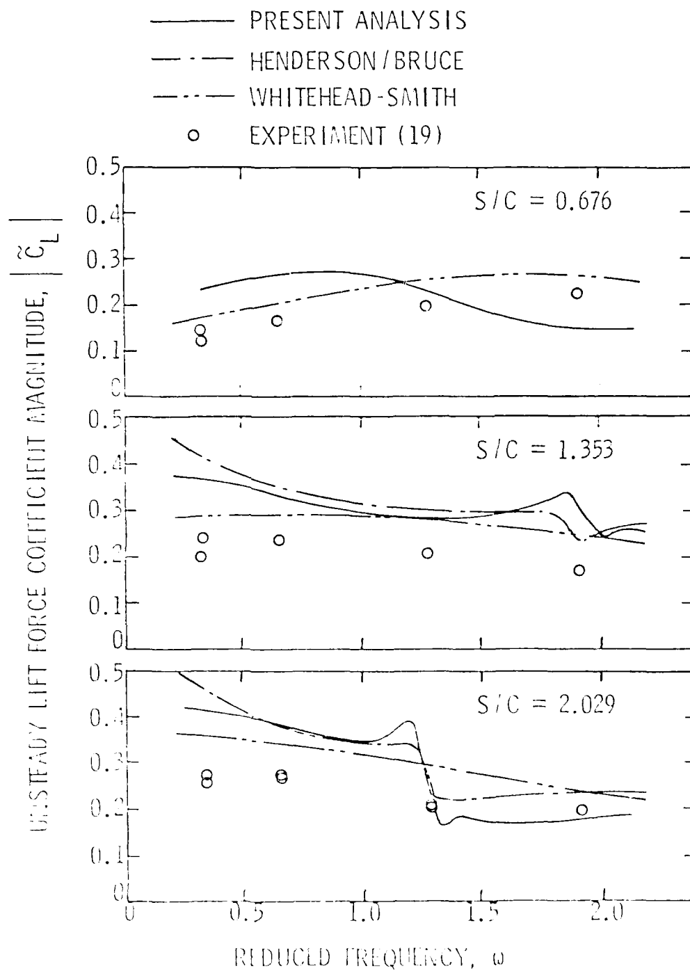
Fig. 10. Comparison of the present model with the experimental data of Henderson and Bruce (19) and the theoretical models of Henderson and Bruce (19) and Whitehead and Smith (19).
