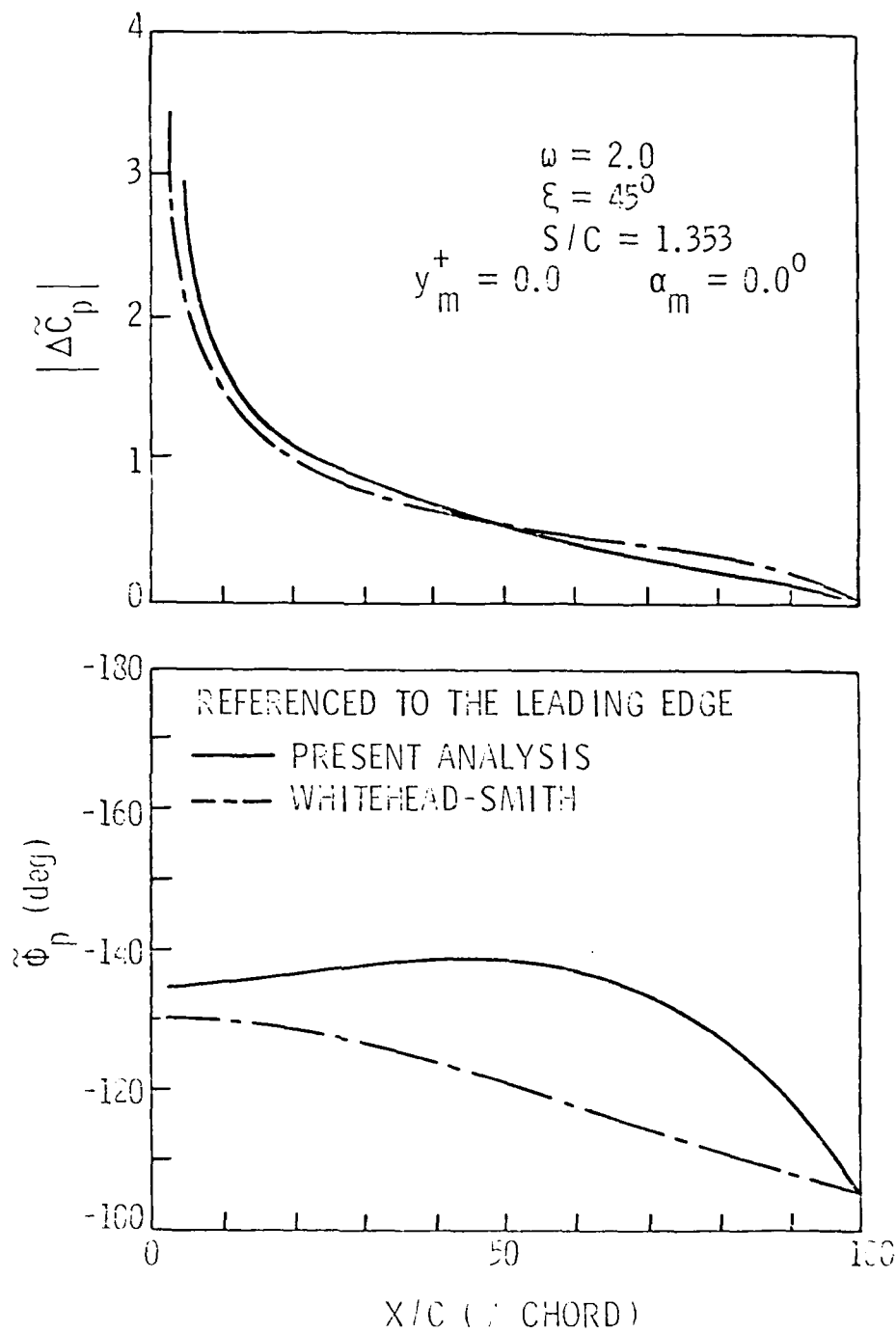
Figure 11. Comparison of Theoretical Unsteady Pressure Distribution with \omega = 2.0 , \xi = 45^\circ , and S/C = 1.353 .
