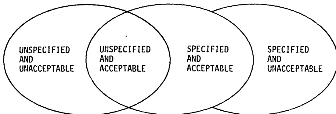
Figure 3.1. Universe of Software Behavior
