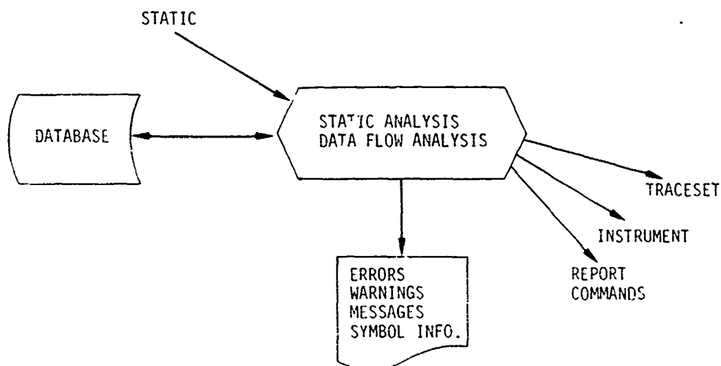
Figure 4.5. Static and Data Flow Analysis
