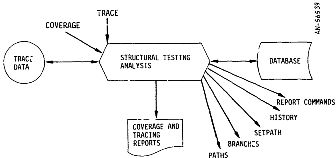
Figure 4.10. Structural Testing Analysis
