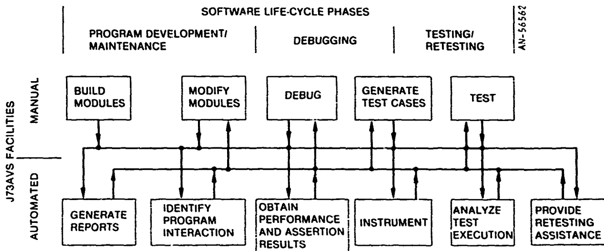
Figure 4.3. Role of J73AVS in the Software Development Cycle
