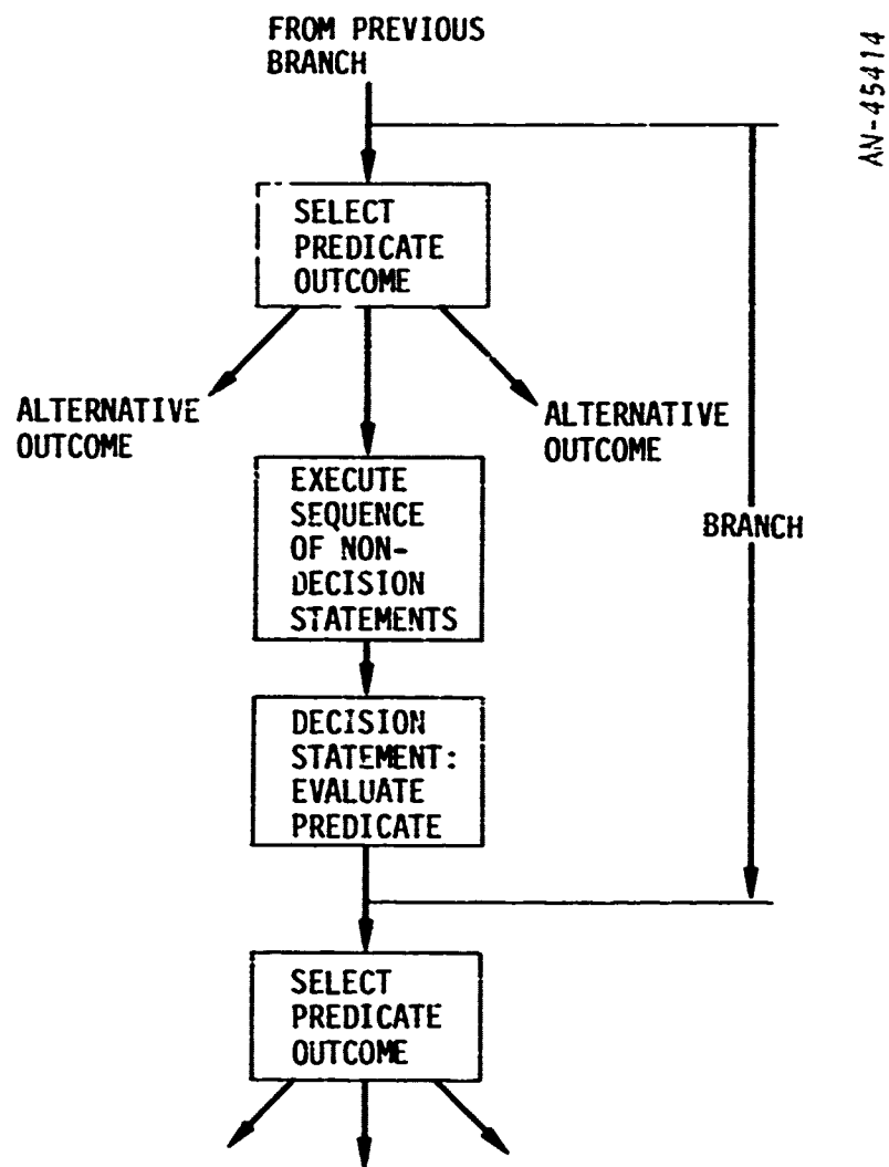
Figure 3.2. Diagram of a Branch
