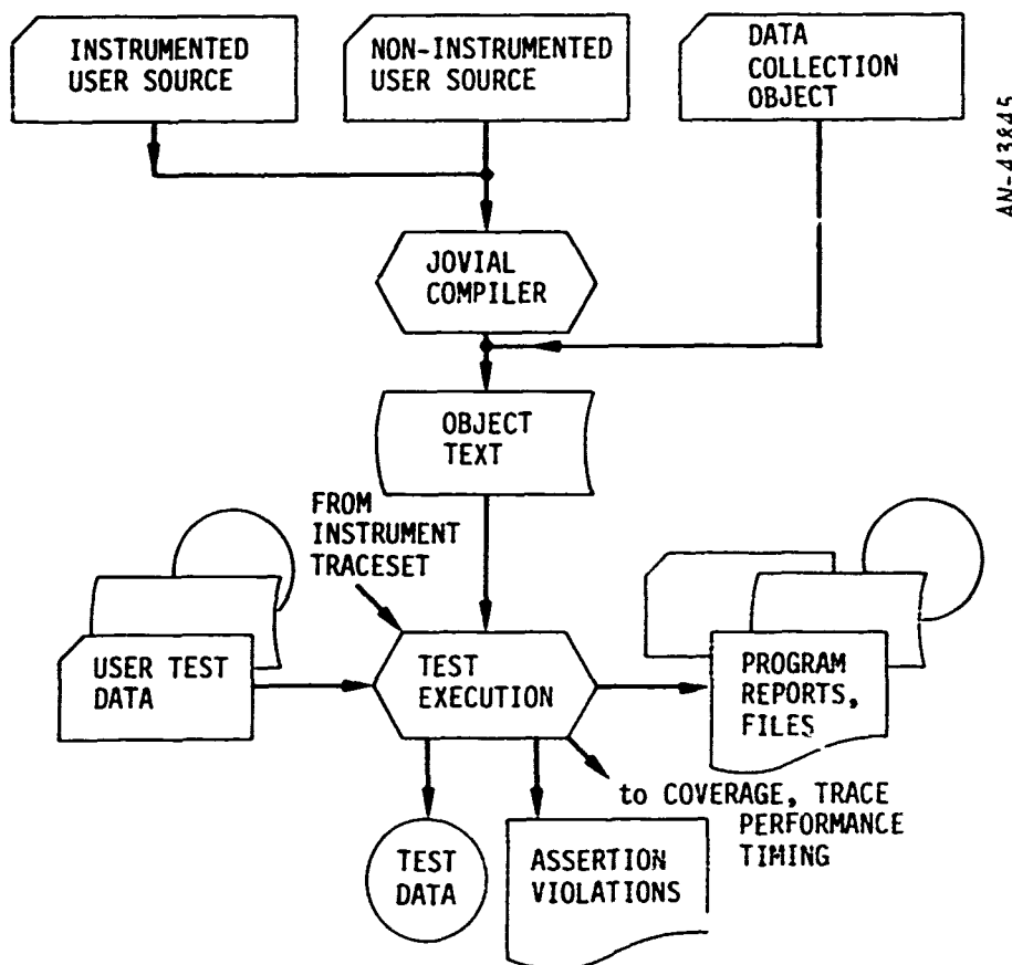
Figure 4.9. Test Execution Processing
