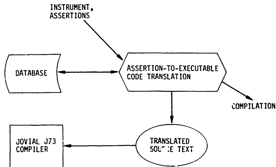
Figure 4.7. Assertion Instrumentation
