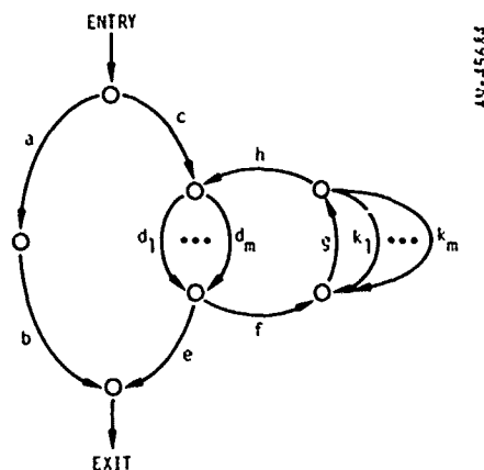
Figure 3.3. Sample Set of Level-i Paths
