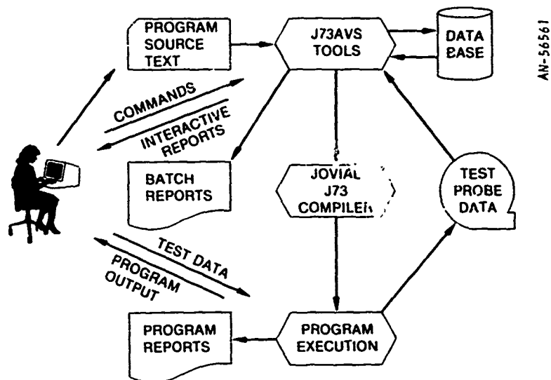
Figure 4.2. J73AVS Interaction with User
