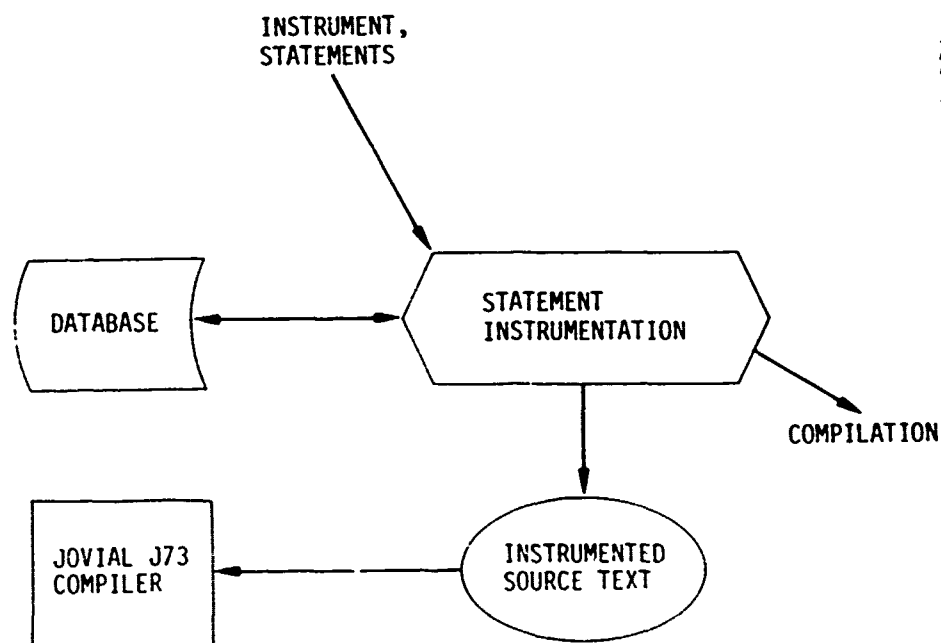
Figure 4.8. Statement Performance Instrumentation
