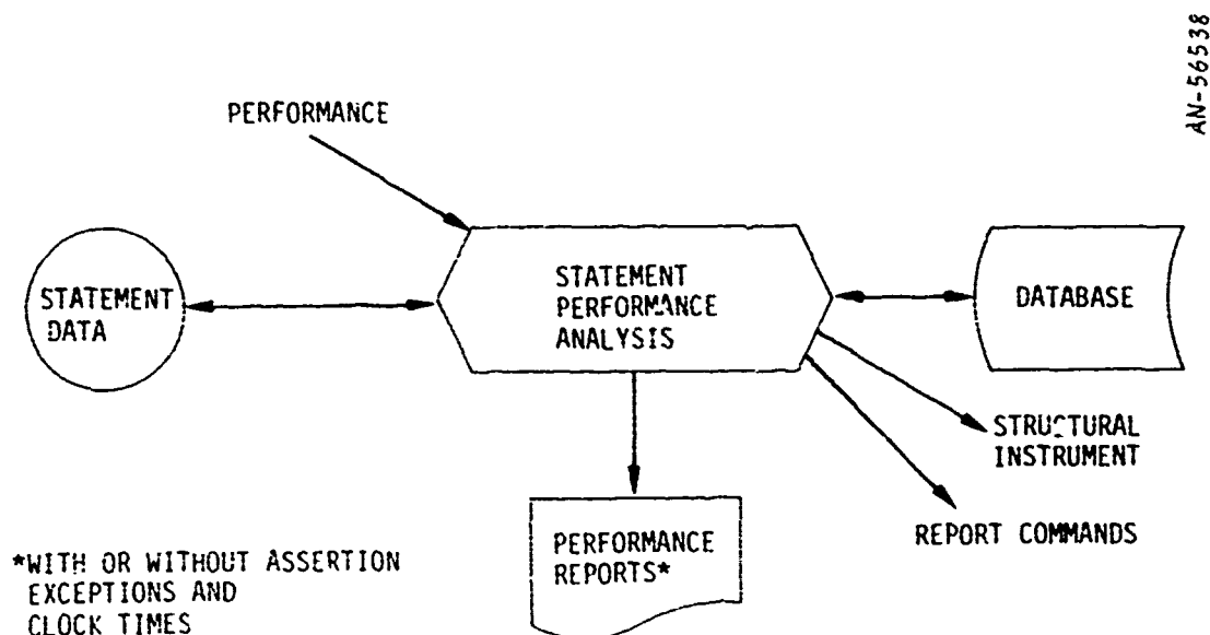
Figure 4.11. Statement Performance Analysis
