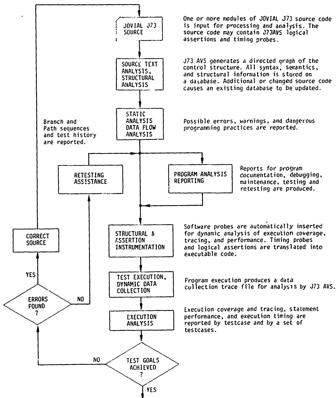
Figure 4.1. Overview of J73AVS
