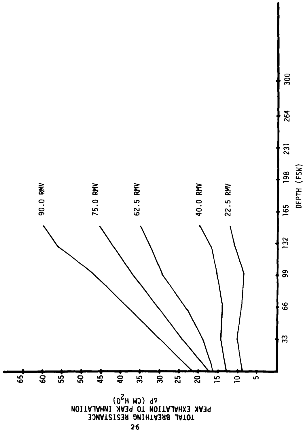
FIGURE 8- BREATHING RESISTANCE MAXIMUM Δ P VS DEPTH
