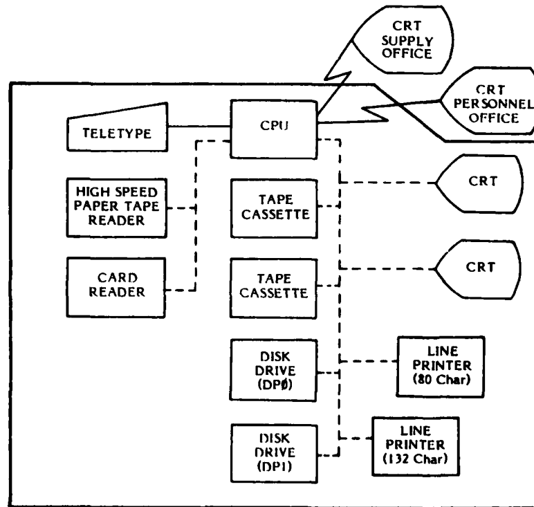
Figure 2. GRIDLEY minicomputer configuration.
