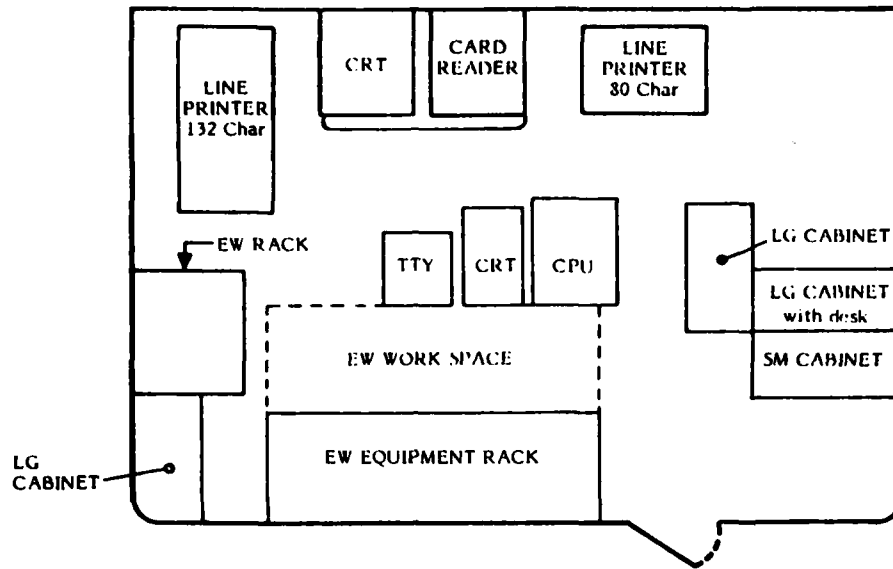
Figure 1. Shipboard Computer Room Compartment 05-90-0-Q.
