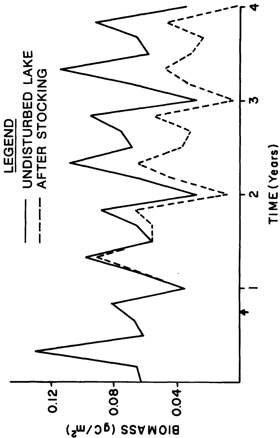
Figure 4. Simulated effect of white amur on phytoplankton biomass. (Arrow denotes time of stocking)
