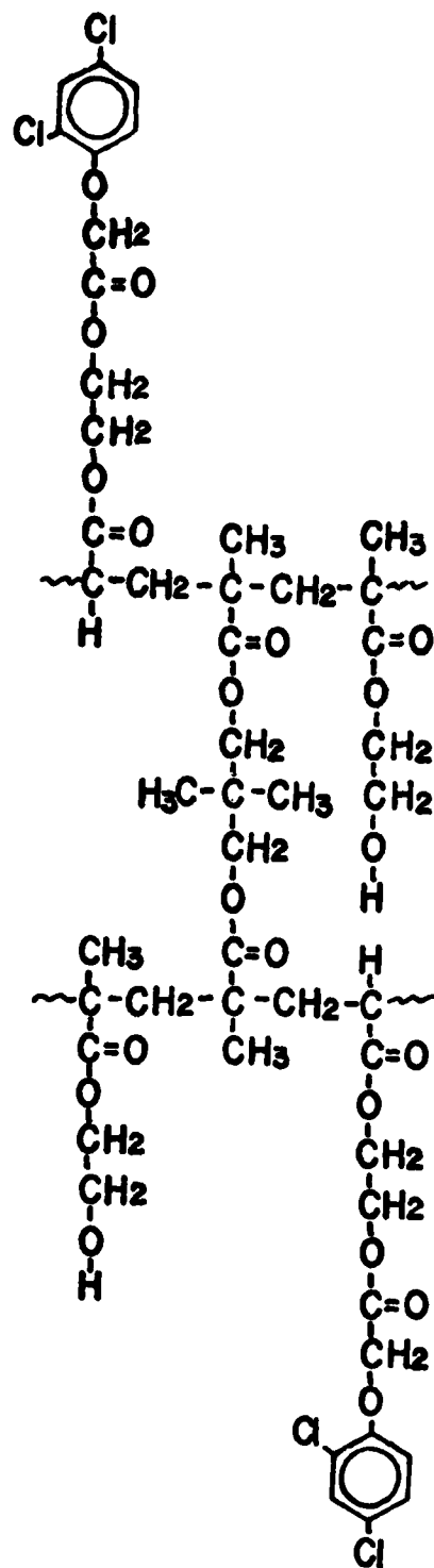
Figure 2. AOE 2,4-D/HEMA/DPDM ( 4 )
