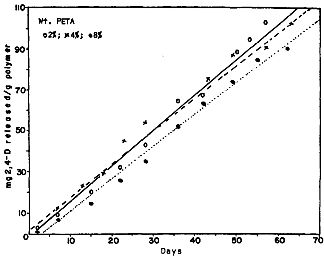
Figure 3. Hydrolysis of polymer 3 prepared in 25 ml MEK
