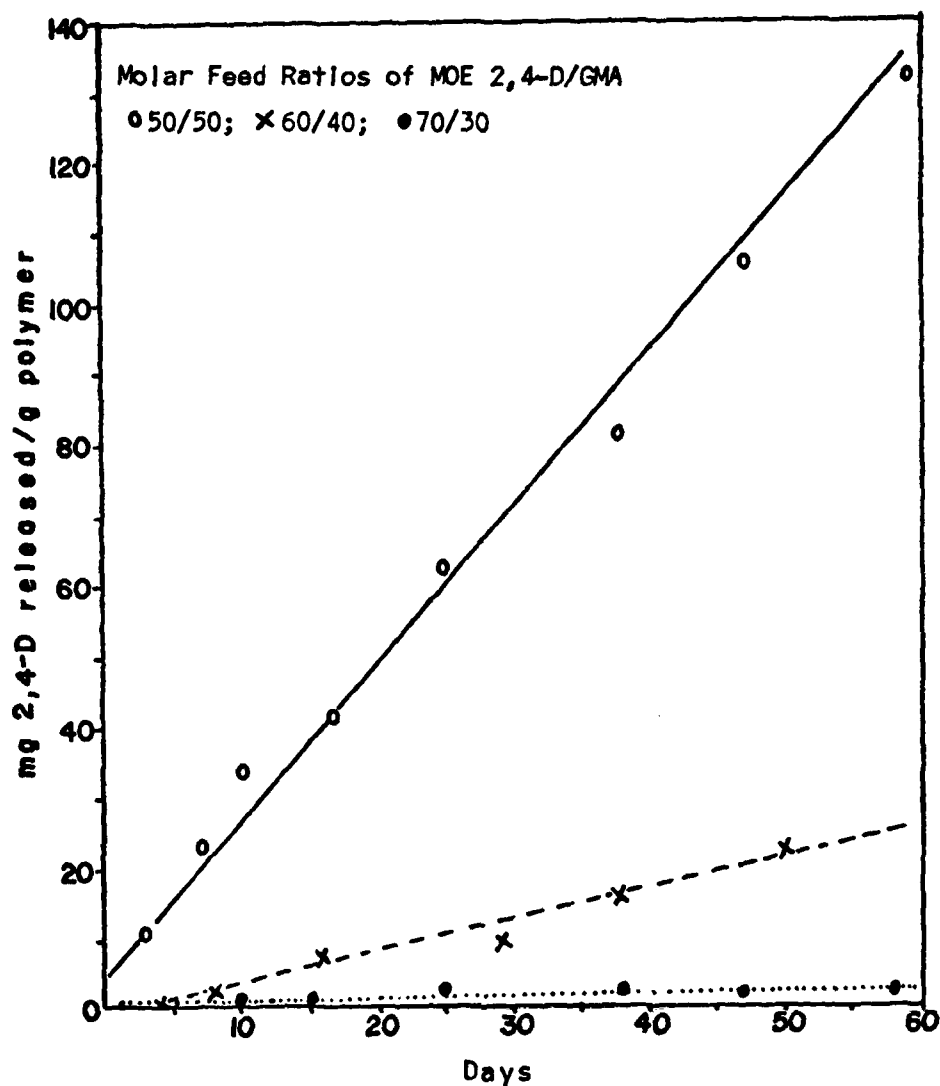
Figure 7. Hydrolysis of MOE 2,4-D/GMA copolymers
