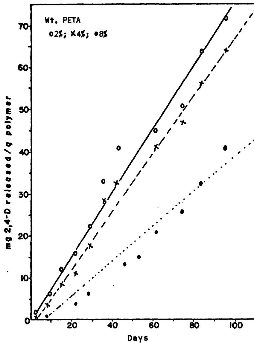
Figure 4. Hydrolysis of polymer 3 prepared in 80 ml MEK
