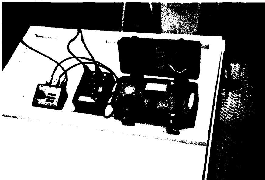
Figure 3. Receiving equipment used at Lake Conway. A coaxial antenna switch is shown on the left, the 180-deg transmission line phase shift unit in the center, and the radiotelemetry receiver on the right
