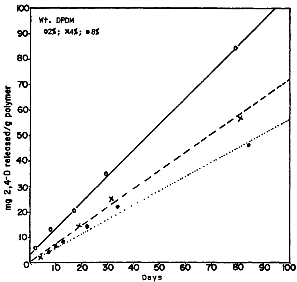
Figure 6. Hydrolysis of polymer 4 prepared in 50 ml MEK
