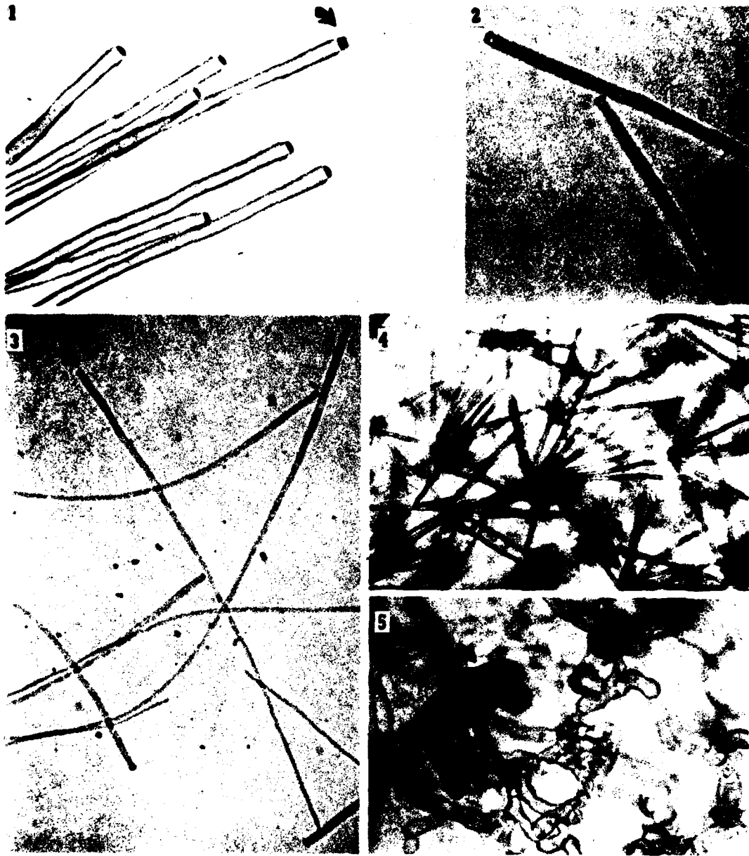
Figure 2. Microscopic (light) details of Cercospora rodmanni morphology and pathological histology. 1. Conidiophores ( 5\ \mu wide) showing conidium attachment (arrow) 400X. 2. Conidium showing truncate base, 400X. 3. Conidia of Cercospora rodmanni ; arrow points to 300- \mu -long conidium. 4. Top view of fascicles of conidiophores on leaf surface, 200X. 5. Subepidermal mycelium; arrow points to base of conidiophores, 400X.
