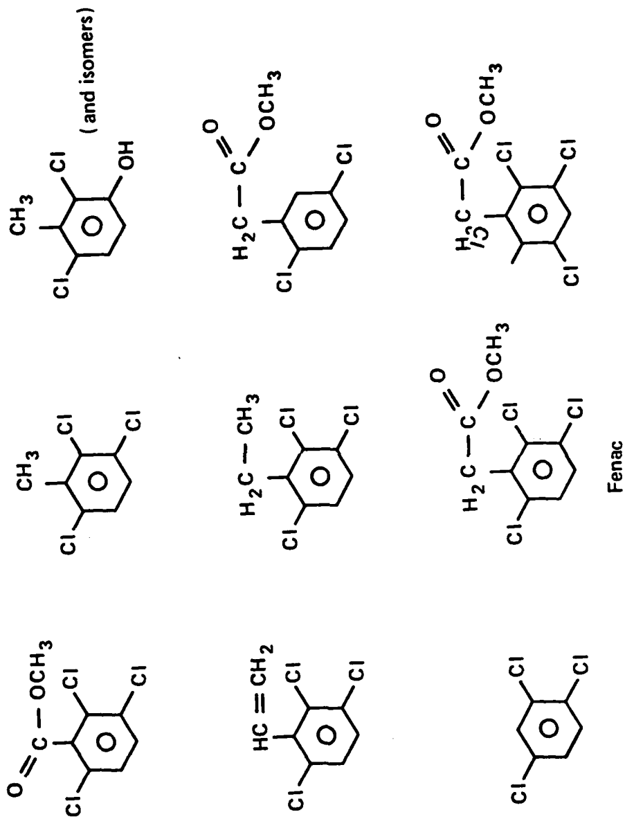
Figure 1. Proposed fenac photodegradation products
