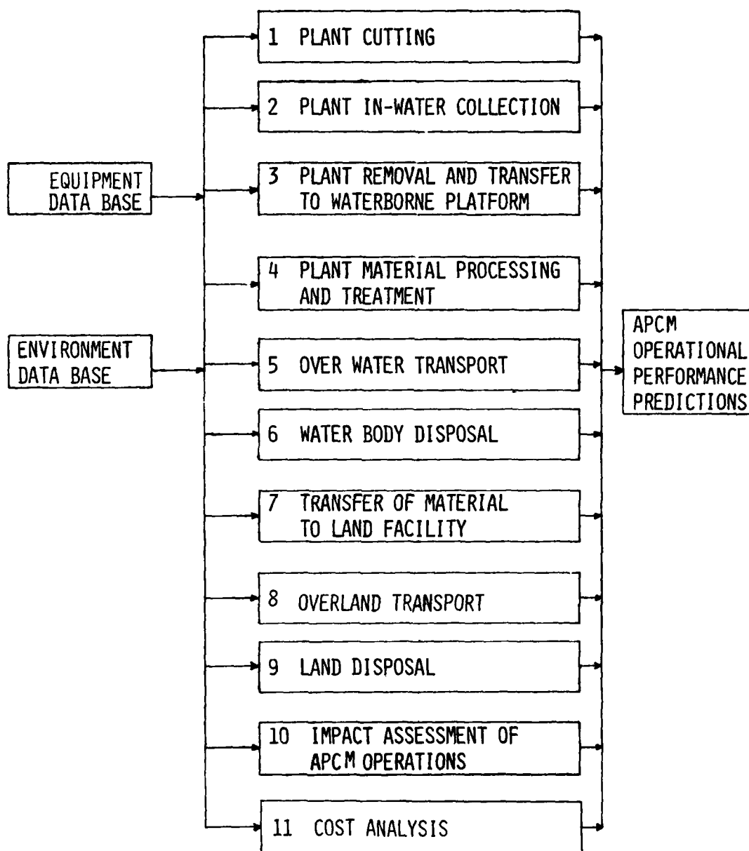
Figure 2. Conceptual APCM model
