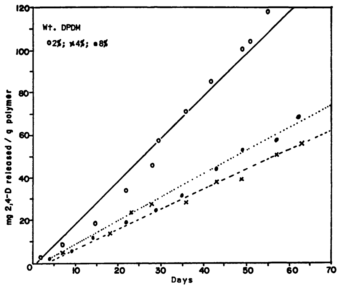
Figure 5. Hydrolysis of polymer 4 prepared in 25 ml MEK
