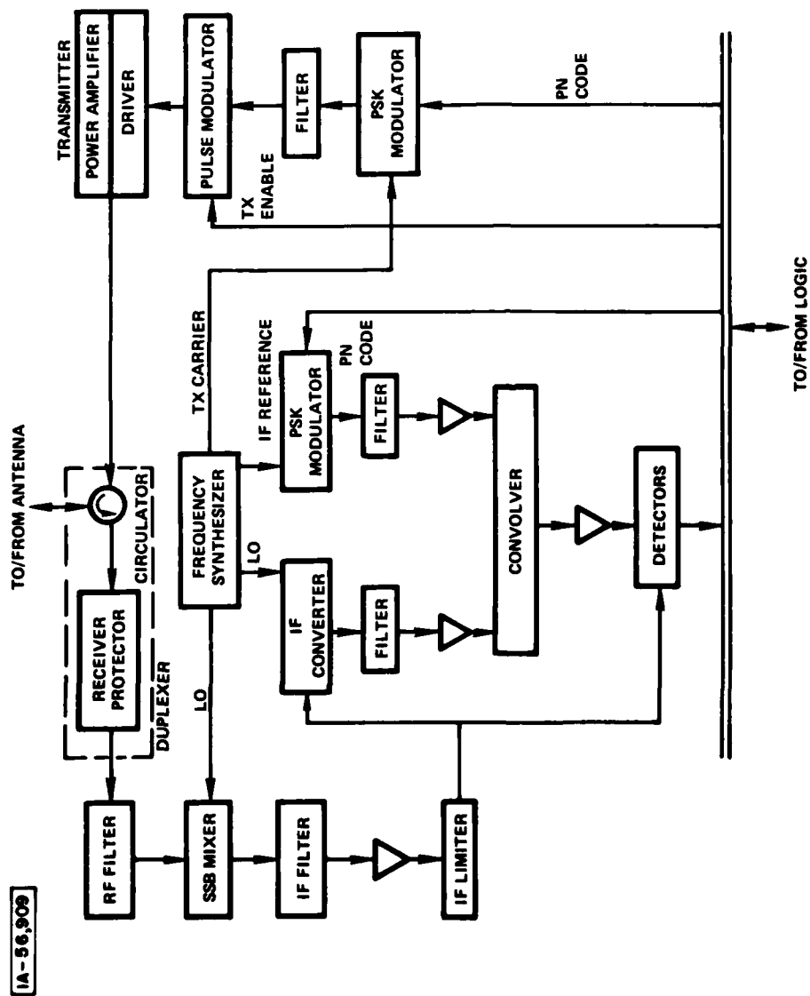
FIGURE 3-12: RF/IF ANALOG SECTION
