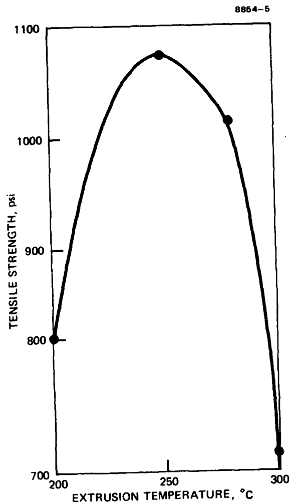
Figure 19. Extruded KCl fiber tensile yield strength versus extrusion temperature.
