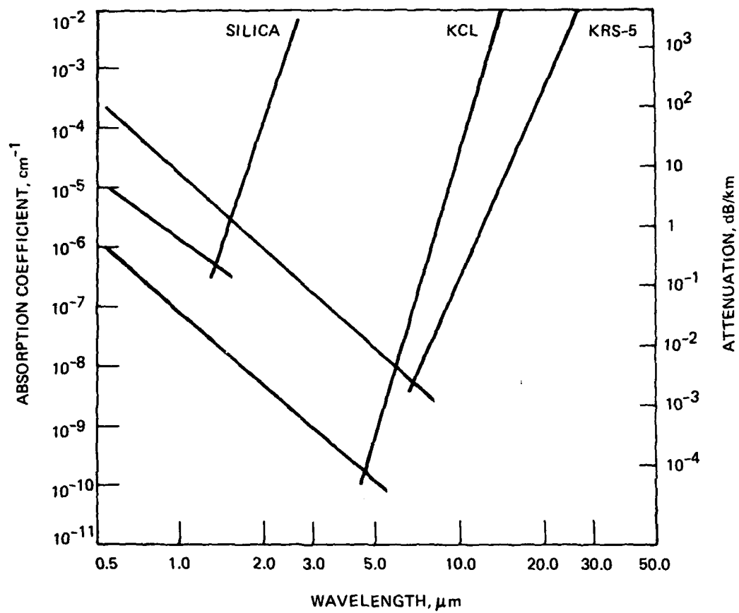
Figure 2. Projected transmission in infrared fibers.
