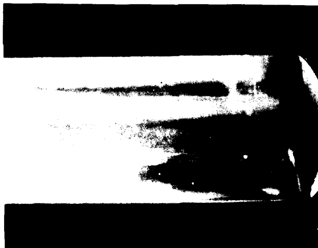
Figure 14(b). 8X, extruded KCl, low rate, 0.25 in. diameter. Right side is first portion out of extruder.
