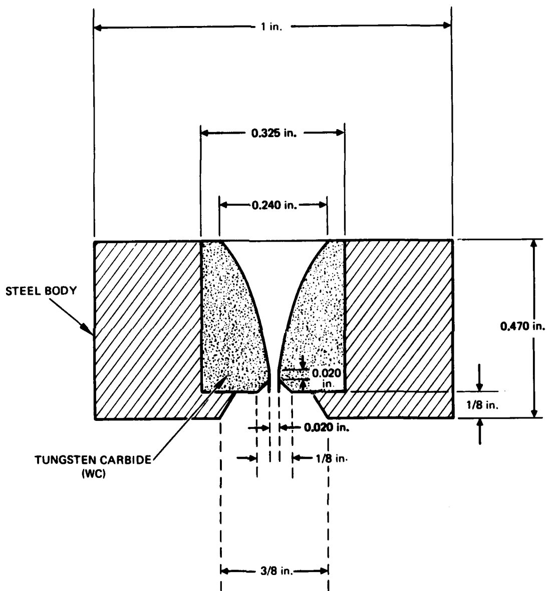
Figure 7. WC die for gentle reduction of KCl.
