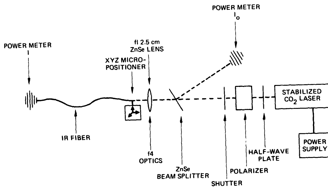
Figure 17. IR fiber loss measurement apparatus.
