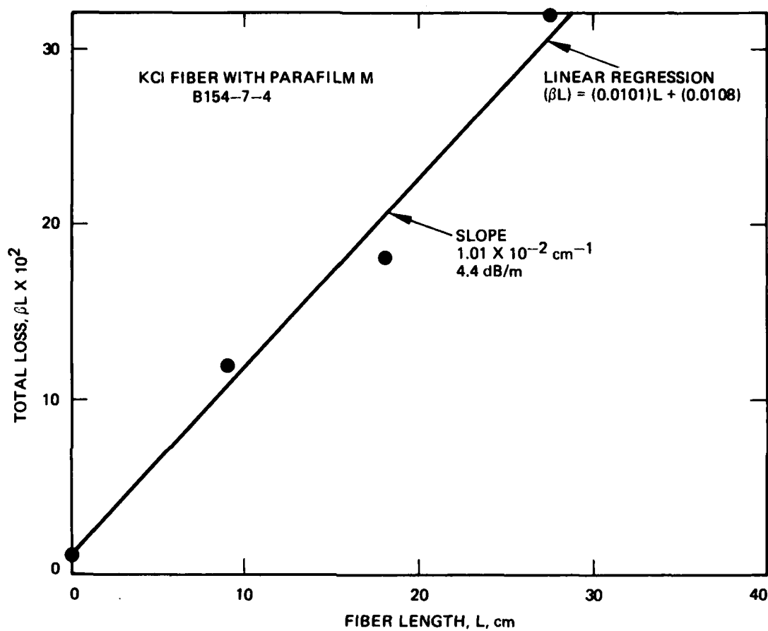
Figure 18. Total loss versus fiber length in 500- \mu\text{m} -diameter KCl fiber.
