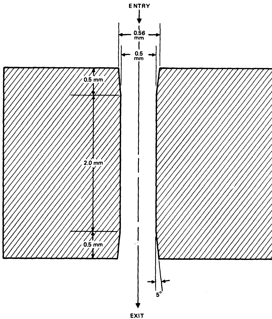
Figure 11. Long-bearing WC die for KCl extrusion.
