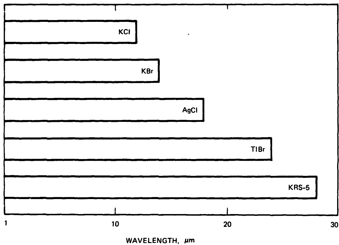
Figure 1. Transmission range of polycrystalline IR fiber materials.
