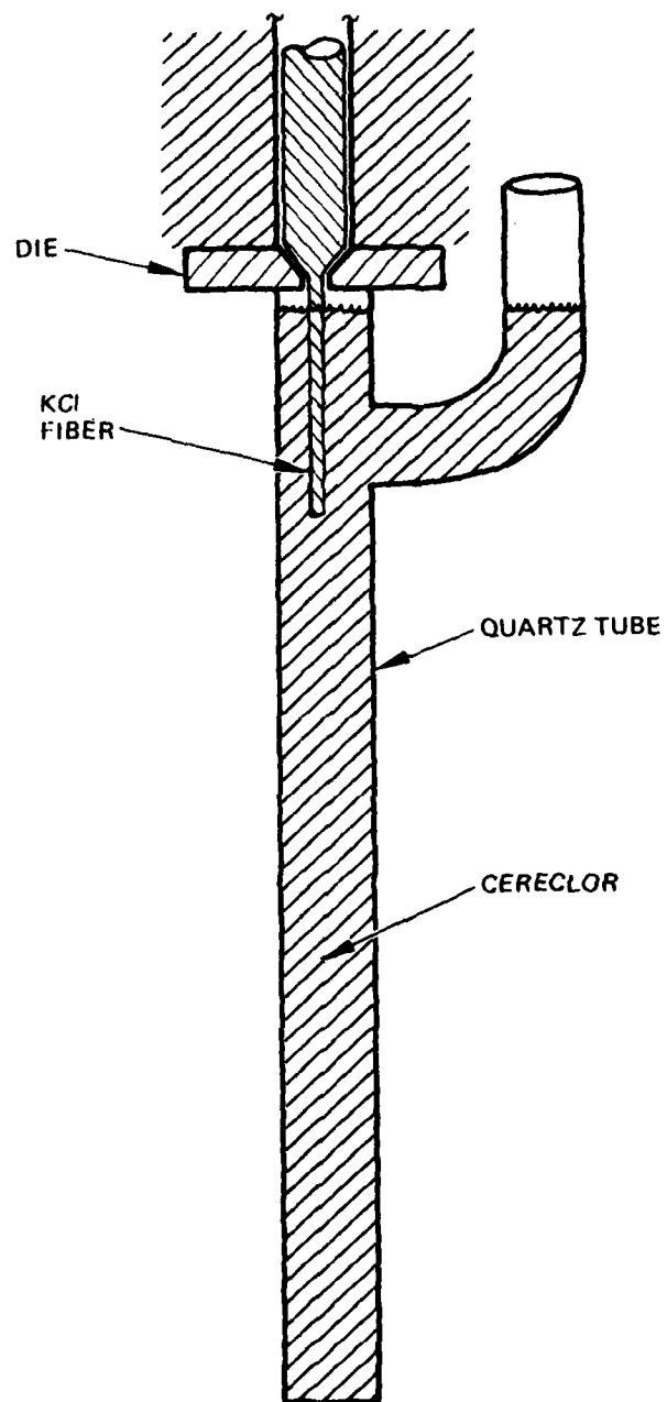
Figure 3. RAP (Cereclor) environment to protect fiber's surface from attack by moisture.
