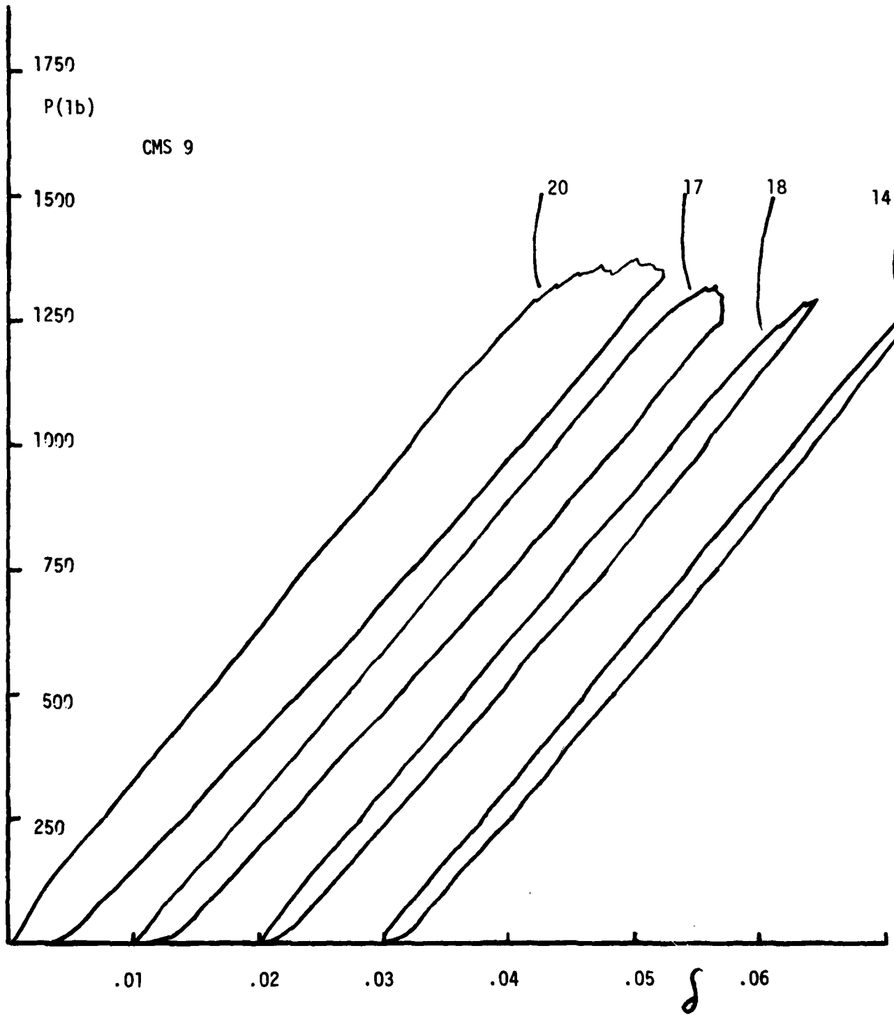
Figure 13a. P- \delta curves for 4 CMS 9 specimens.
