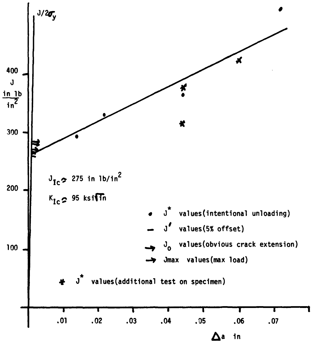
Figure 14. Graphical Determination of J_{Ic} for CMS-9.
