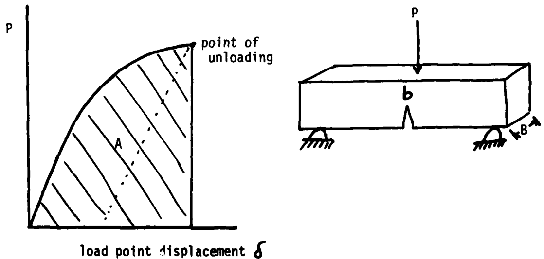
Figure 2. Determination of J from 3 point bend specimen.
