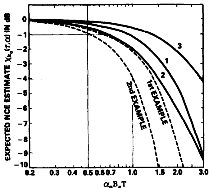
Fig. 6 — Coherence degradation due to imperfect Doppler compensation as a function of \alpha_0 B_p T . (Curves labeled 1, 2, and 3 result from assuming the corresponding probability densities given in Table 3)
