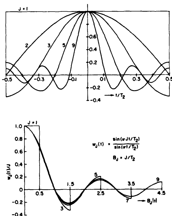
Fig. 3 - Temporal window function w_J(t) for selected values of J
