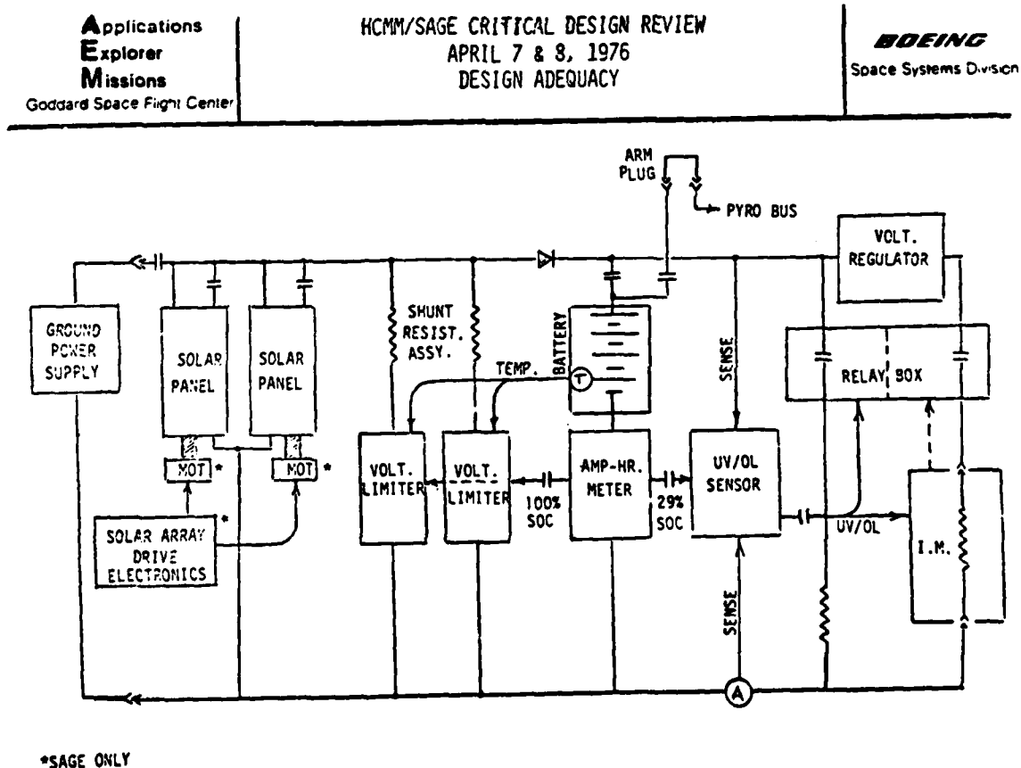
Fig. B-1—Power and distribution subsystem block diagram
