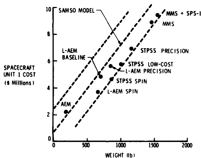
Fig. 6—Spacecraft unit cost versus weight
