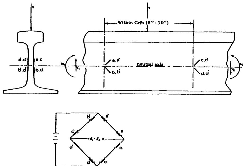
Figure 2. Strain Gage Circuit for Measuring Vertical Wheel/Rail Loads
