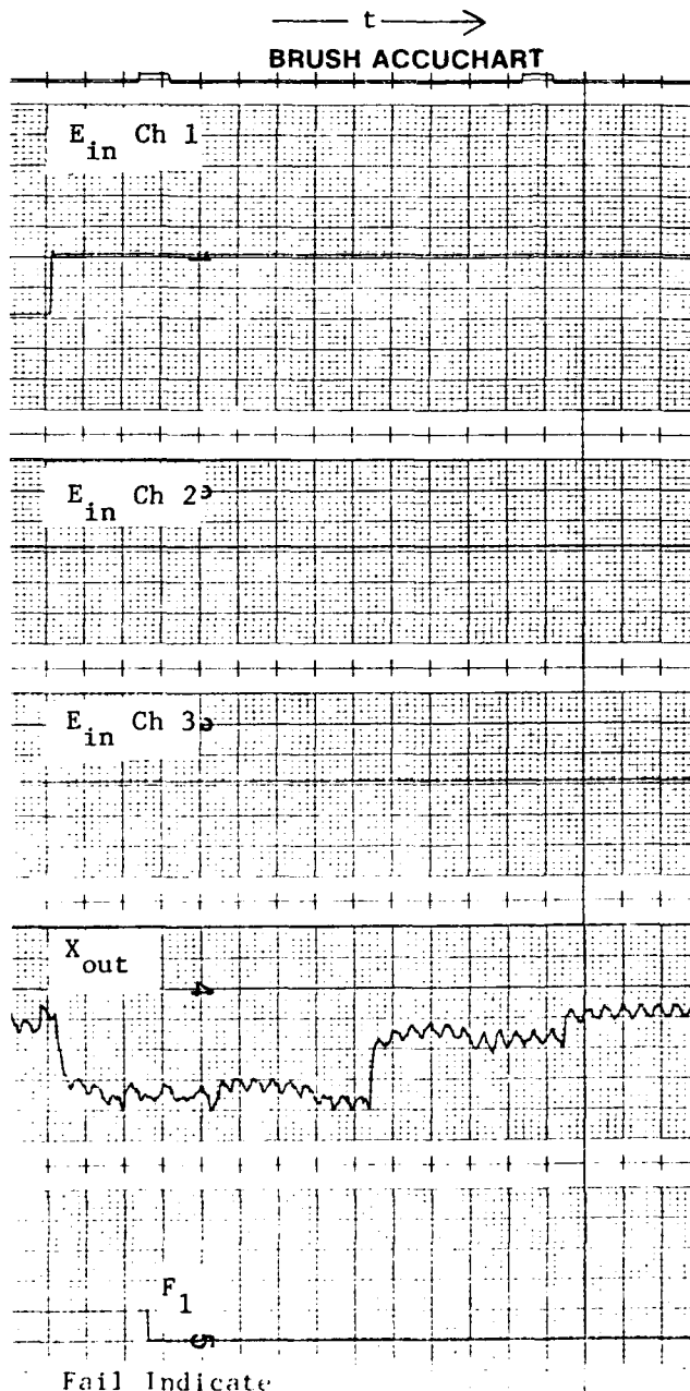
FIGURE 57 Failure Transients - Condition 13 (1st H.O.)
