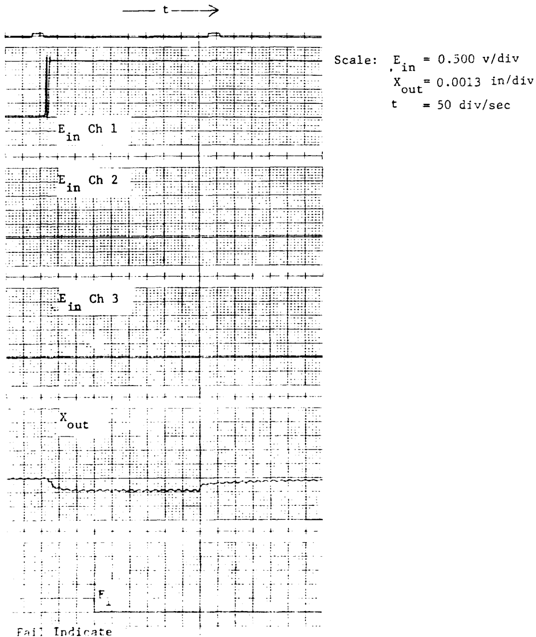
FIGURE 66 Failure Transients - Condition 16 (1st H.O.)
