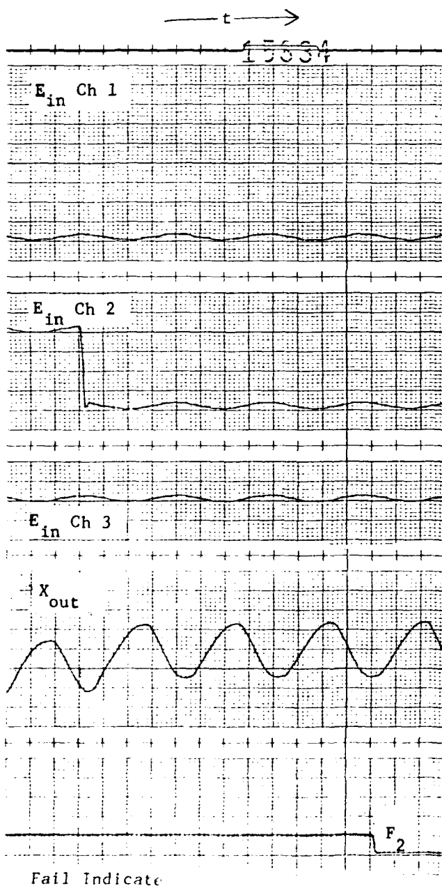
FIGURE 88 Failure Transients - Condition 23 (2nd H.O.)
