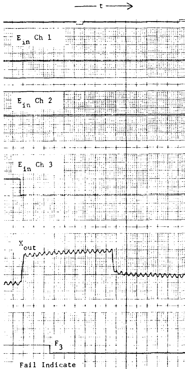
FIGURE 56 Failure Transients - Condition 12 (3rd Failure)
