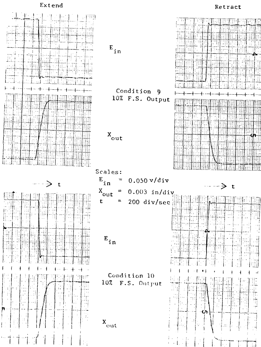
FIGURE 169 Step Response - Conditions 9 & 10
