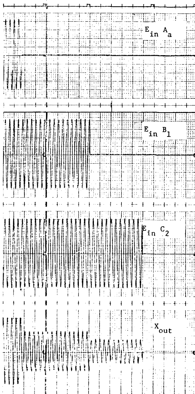
FIGURE 197 Failure Transients - Condition 26
