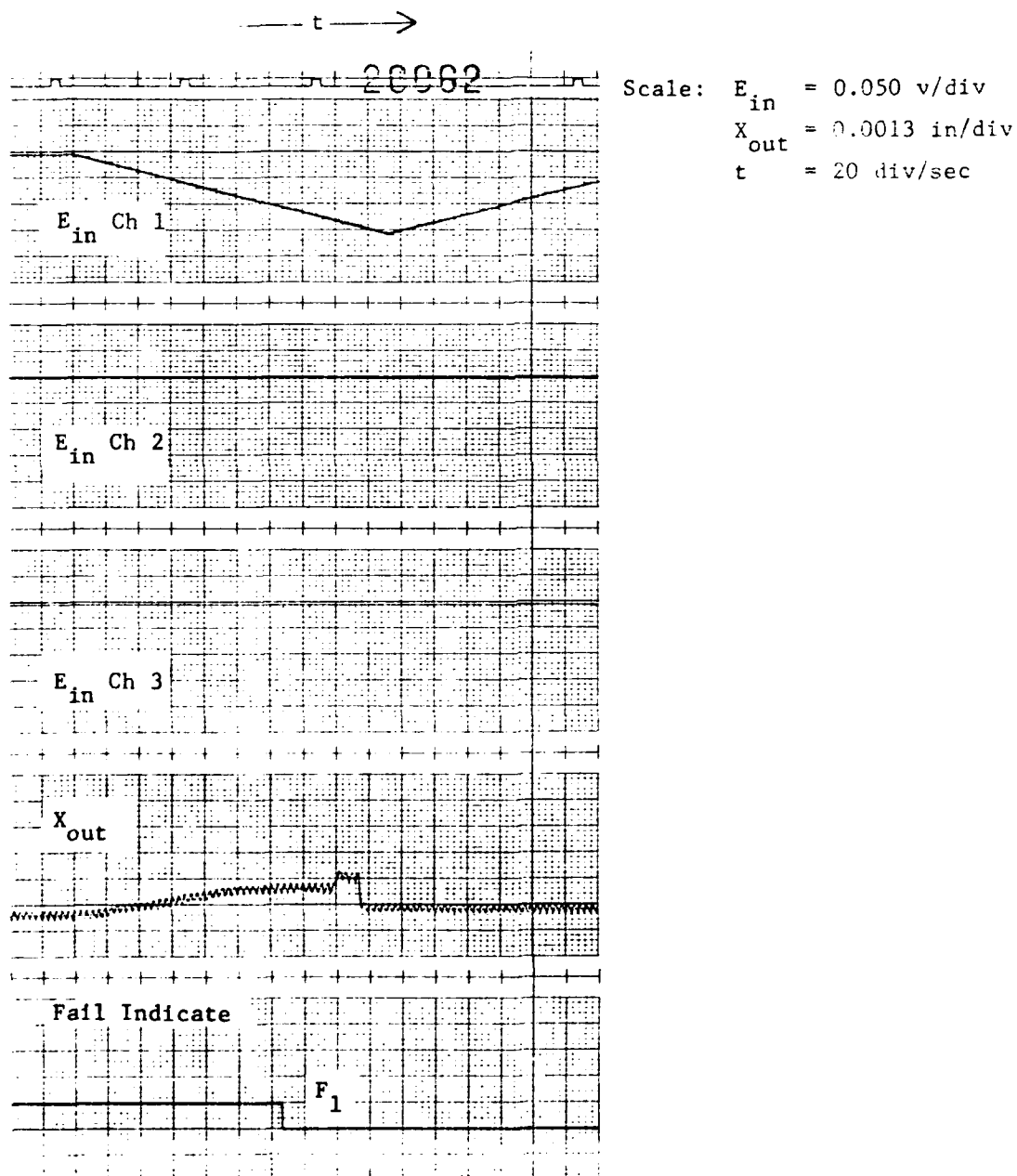
FIGURE 32 Failure Transients - Condition 26 (1 Ch Extend)
