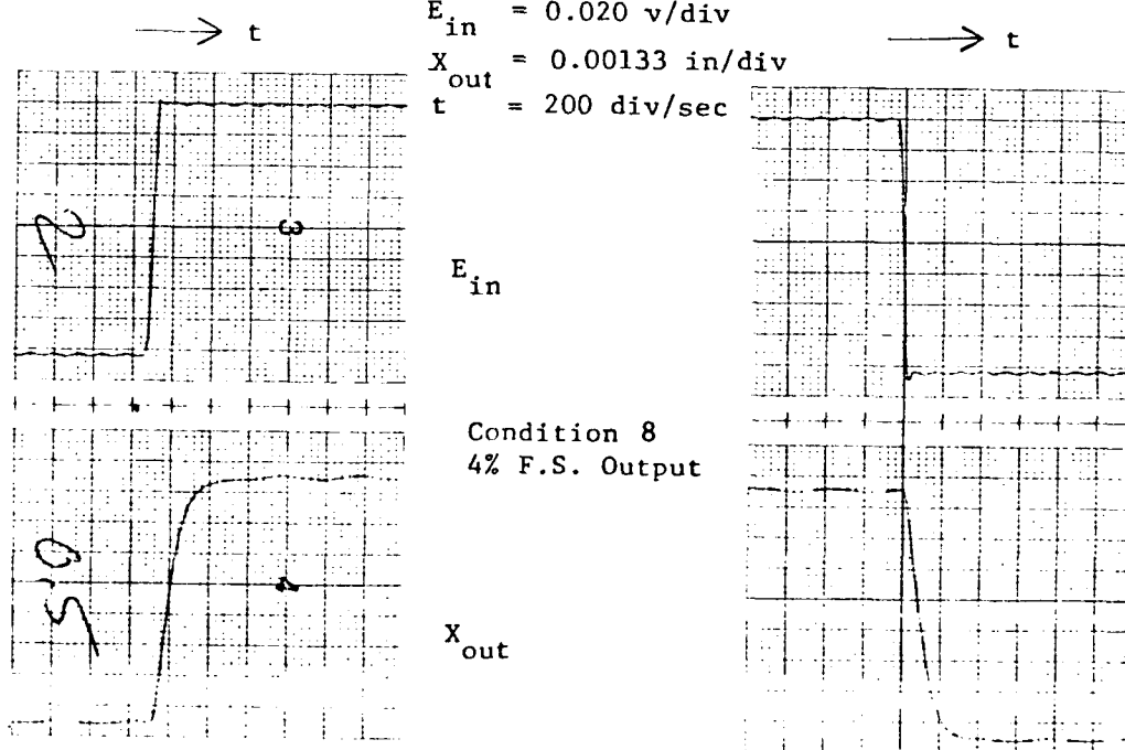
FIGURE 15 Step Response - Conditions 7 & 8
