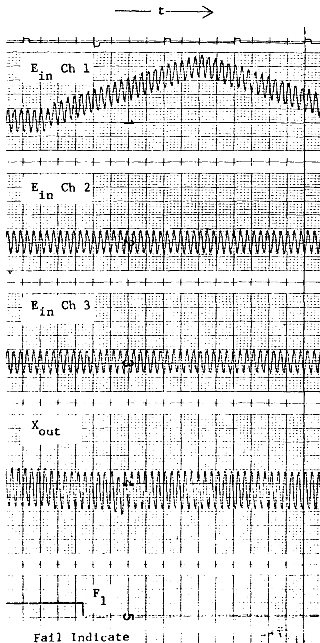
FIGURE 142 Failure Transients - Condition 27 (1 Ch Retract)
