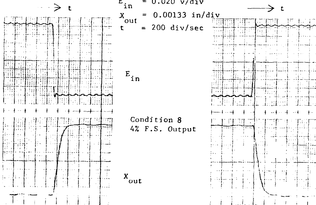
FIGURE 51 Step Response - Conditions 7 & 8
