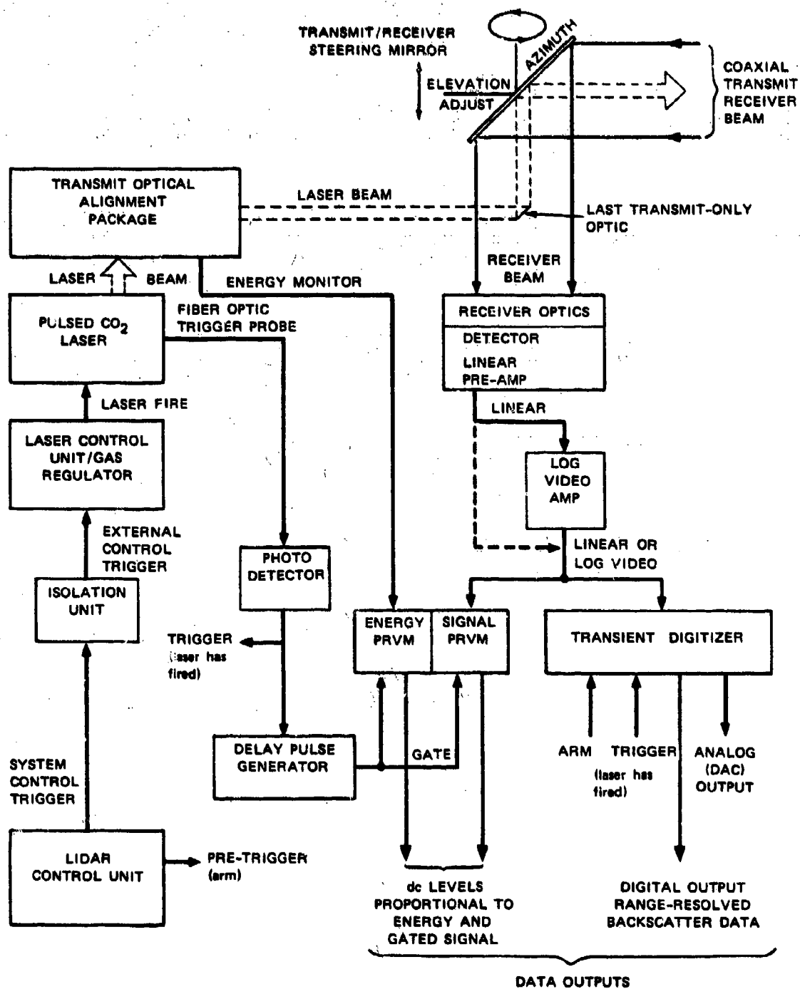
FIGURE 3 ASL LIDAR FUNCTIONAL DIAGRAM
