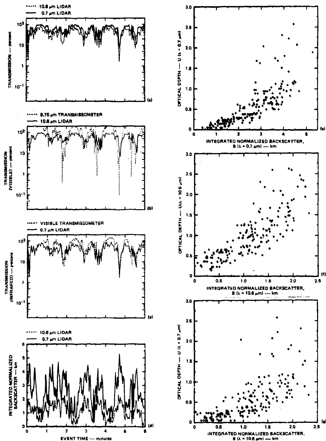
FIGURE 22 TRANSMISSION AND BACKSCATTER DATA PLOTS FOR SMOKE WEEK II, TRIAL 22 (VEHICULAR DUST)
