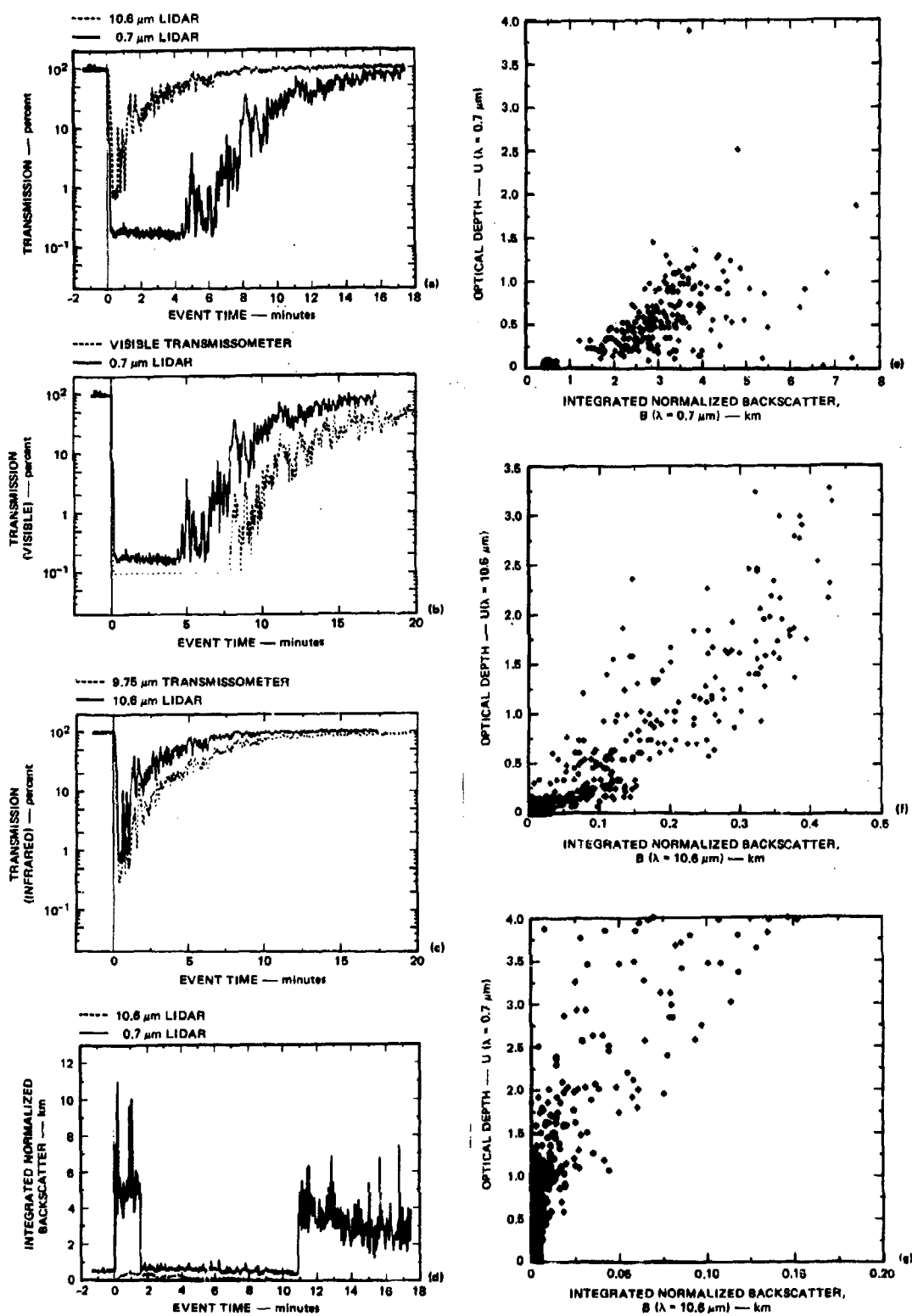
FIGURE 12 ATTENUATION AND BACKSCATTER DATA PLOTS FOR SMOKE WEEK II, TRIAL 2 (PHOSPHORUS)
