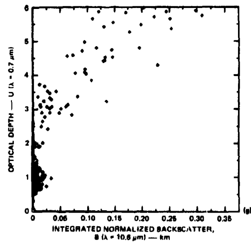
FIGURE 18 TRANSMISSION AND BACKSCATTER DATA PLOTS FOR SMOKE WEEK II, TRIAL 13 (PHOSPHORUS)
