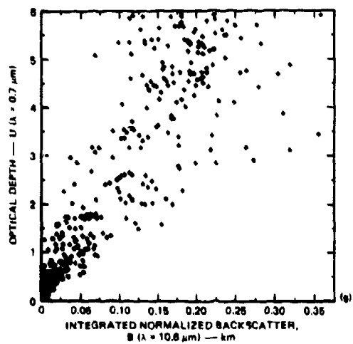
FIGURE 17 TRANSMISSION AND BACKSCATTER DATA PLOTS FOR SMOKE WEEK II, TRIAL 7 (PHOSPHORUS)
