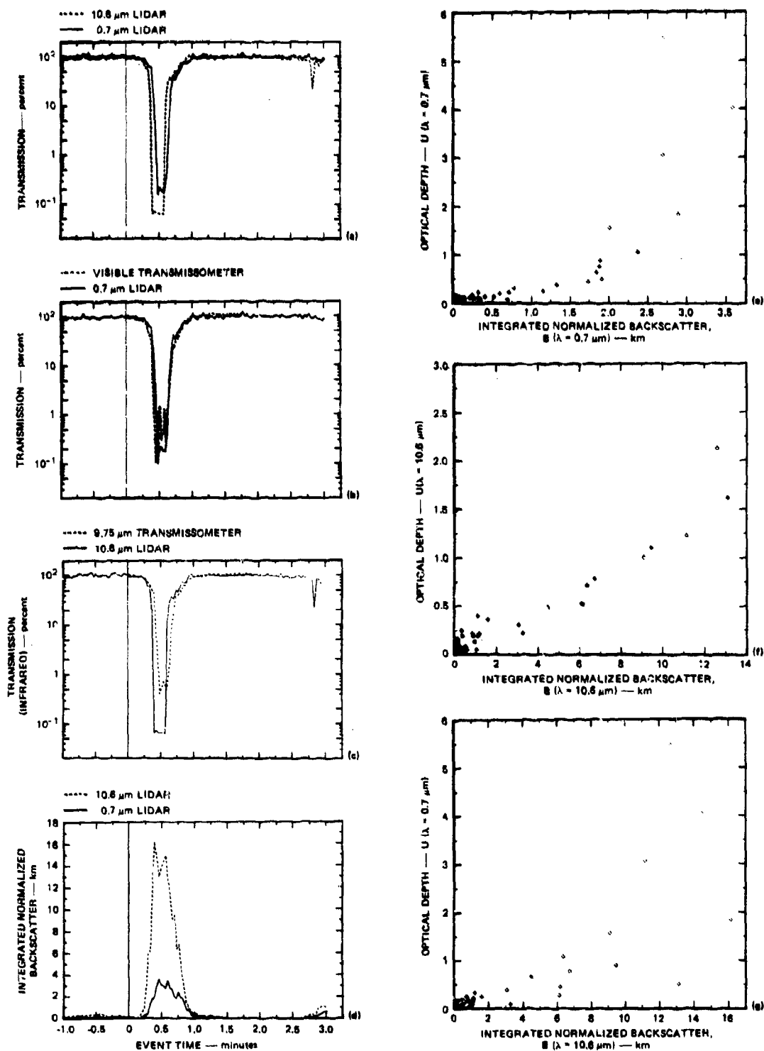
FIGURE 24 ATTENUATION AND BACKSCATTER DATA PLOTS FOR SMOKE WEEK II, TRIAL 23R (HE DUST)
