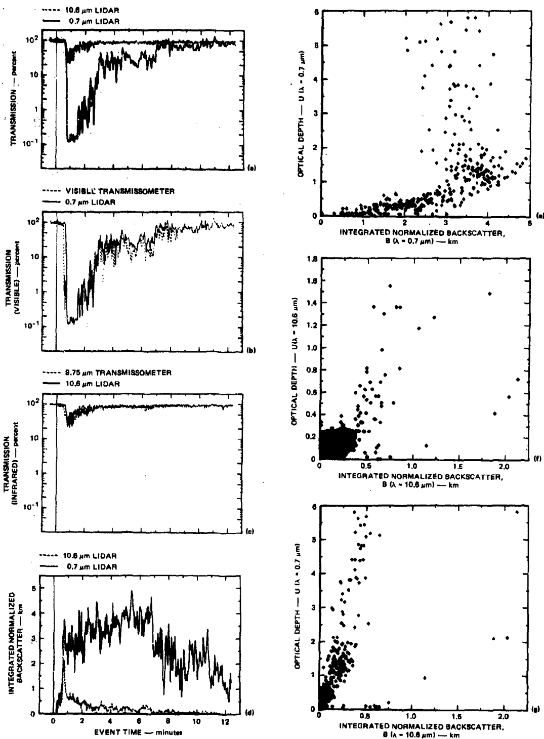
FIGURE 20 TRANSMISSION AND BACKSCATTER DATA PLOTS FOR SMOKE WEEK II, TRIAL 20 (PHOSPHORUS)
