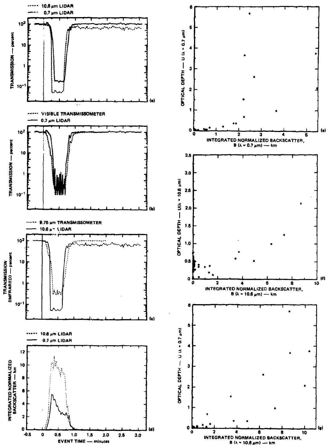
FIGURE 28 ATTENUATION AND BACKSCATTER DATA PLOTS FOR SMOKE WEEK II, TRIAL 26 (HE DUST)
