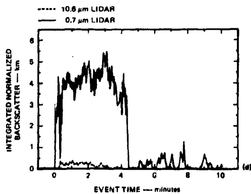
FIGURE 18 TRANSMISSION AND BACKSCATTER DATA PLOTS FOR SMOKE WEEK II, TRIAL 13 (PHOSPHORUS)
