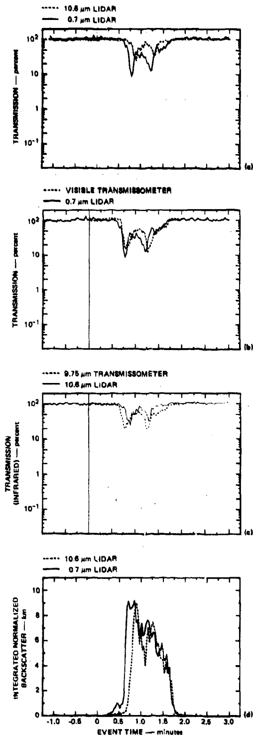
FIGURE 23 ATTENUATION AND BACKSCATTER DATA PLOTS FOR SMOKE WEEK II, TRIAL 23 (HE DUST)
