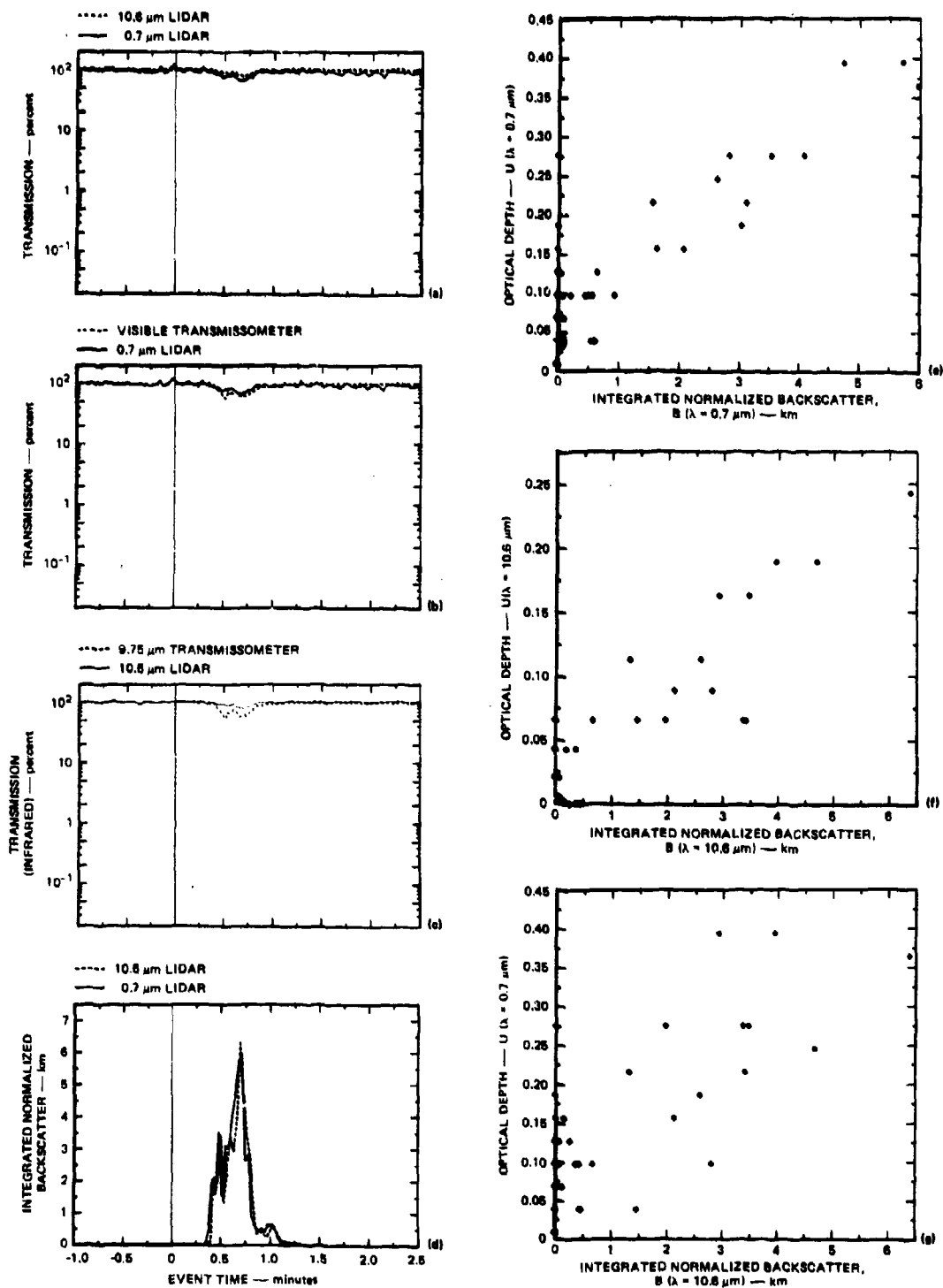
FIGURE 18 TRANSMISSION AND BACKSCATTER DATA PLOTS FOR SMOKE WEEK II, TRIAL 6 (EXPERIMENTAL PARTICLES)
