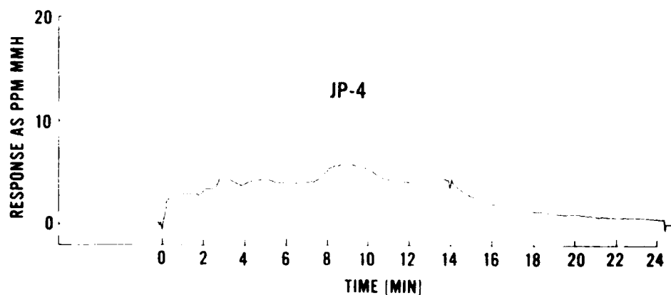
Figure 12. ESI Model 7660 response to JP-4.
