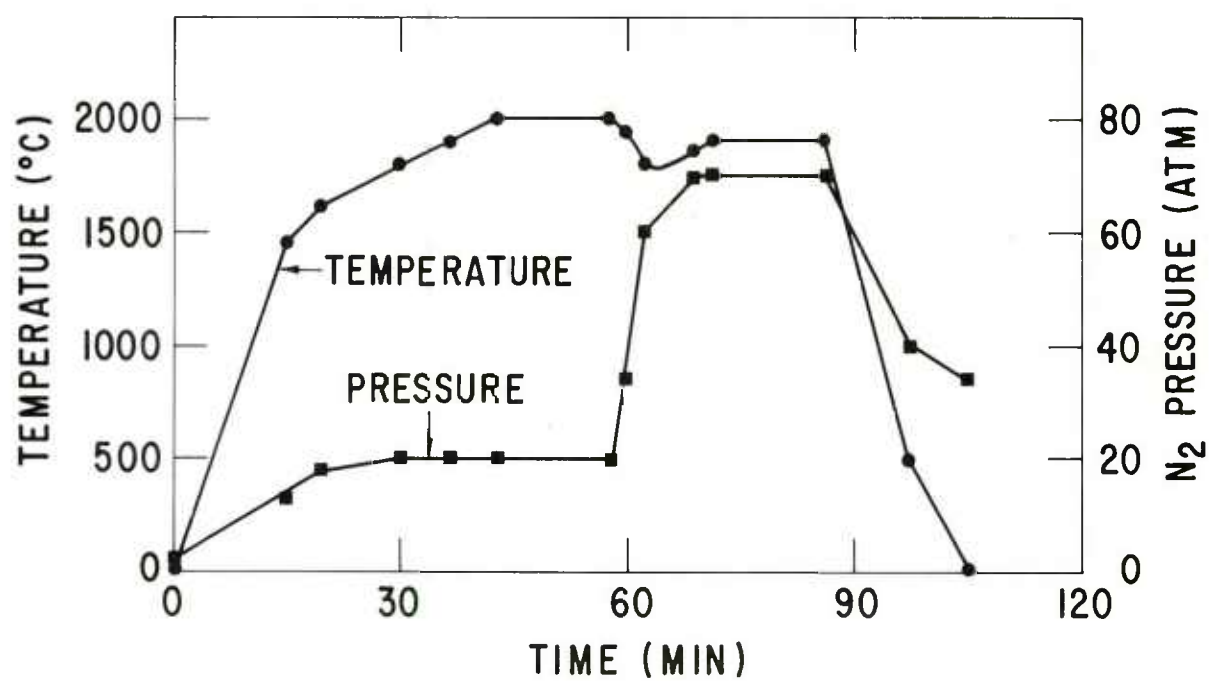
Figure 7. A typical temperature-pressure-time profile used during the sintering of silicon nitride.
