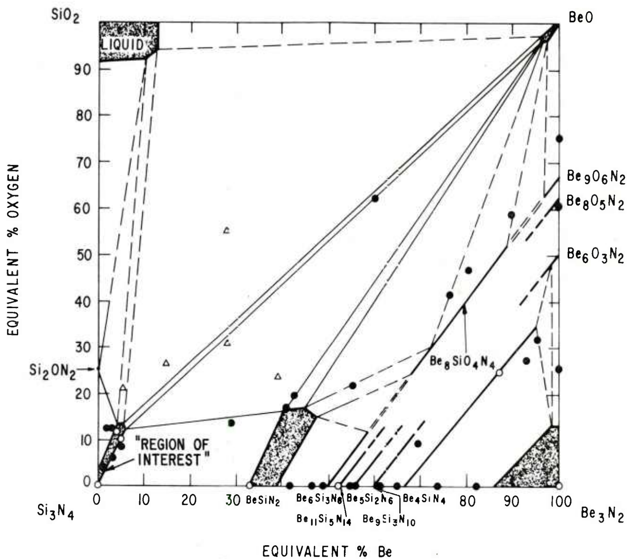
Figure 1. Isothermal section at 1780°C of the system \text{Si}_3\text{N}_4 - \text{SiO}_2 - \text{BeO} - \text{Be}_3\text{N}_2 (17). \circ =1 phase, \circ =2 phases, \Delta =3 phases. The compositional region of interest is designated.
