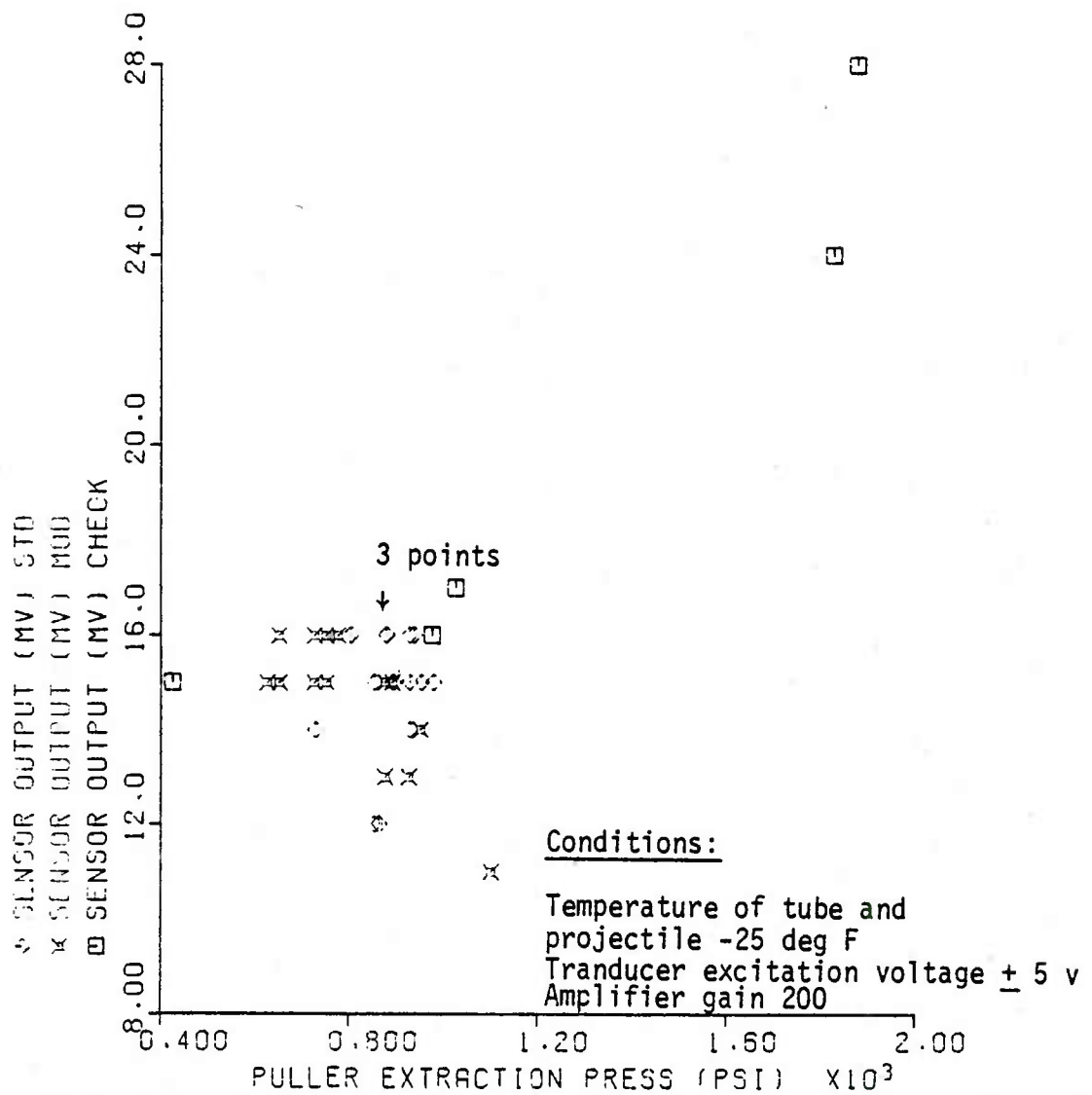
Fig 15. Fallback Sensor Output Versus Extraction Pressure with M106 Projectiles
