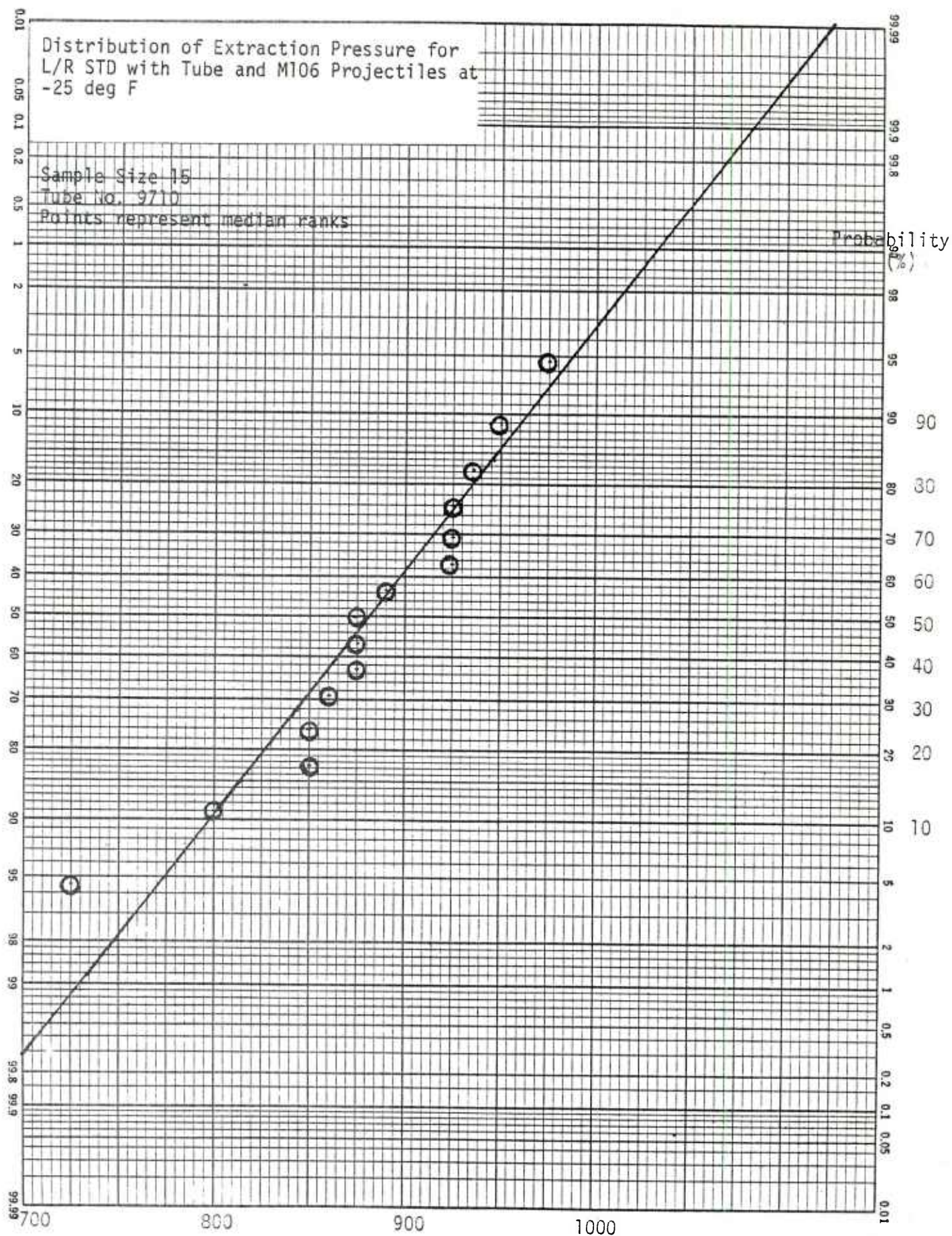
Figure 13. XM753 Extraction Pressure (psig) Distribution of Extraction Pressure in a Cold Environment
