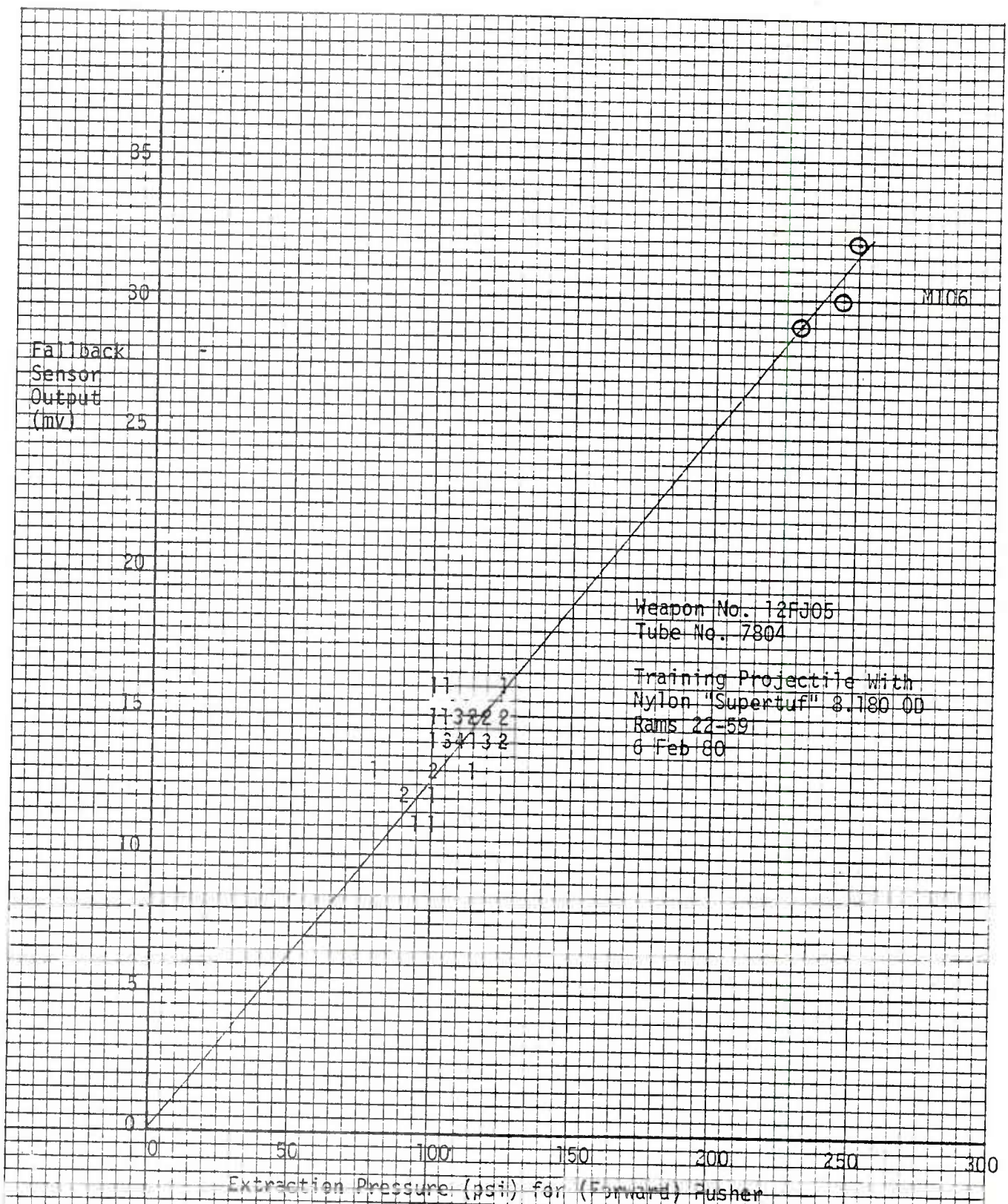
Figure 11. Relationship of Fallback Sensor Output to Extraction Pressure Using Two Projectiles Each Rammed Several Times
