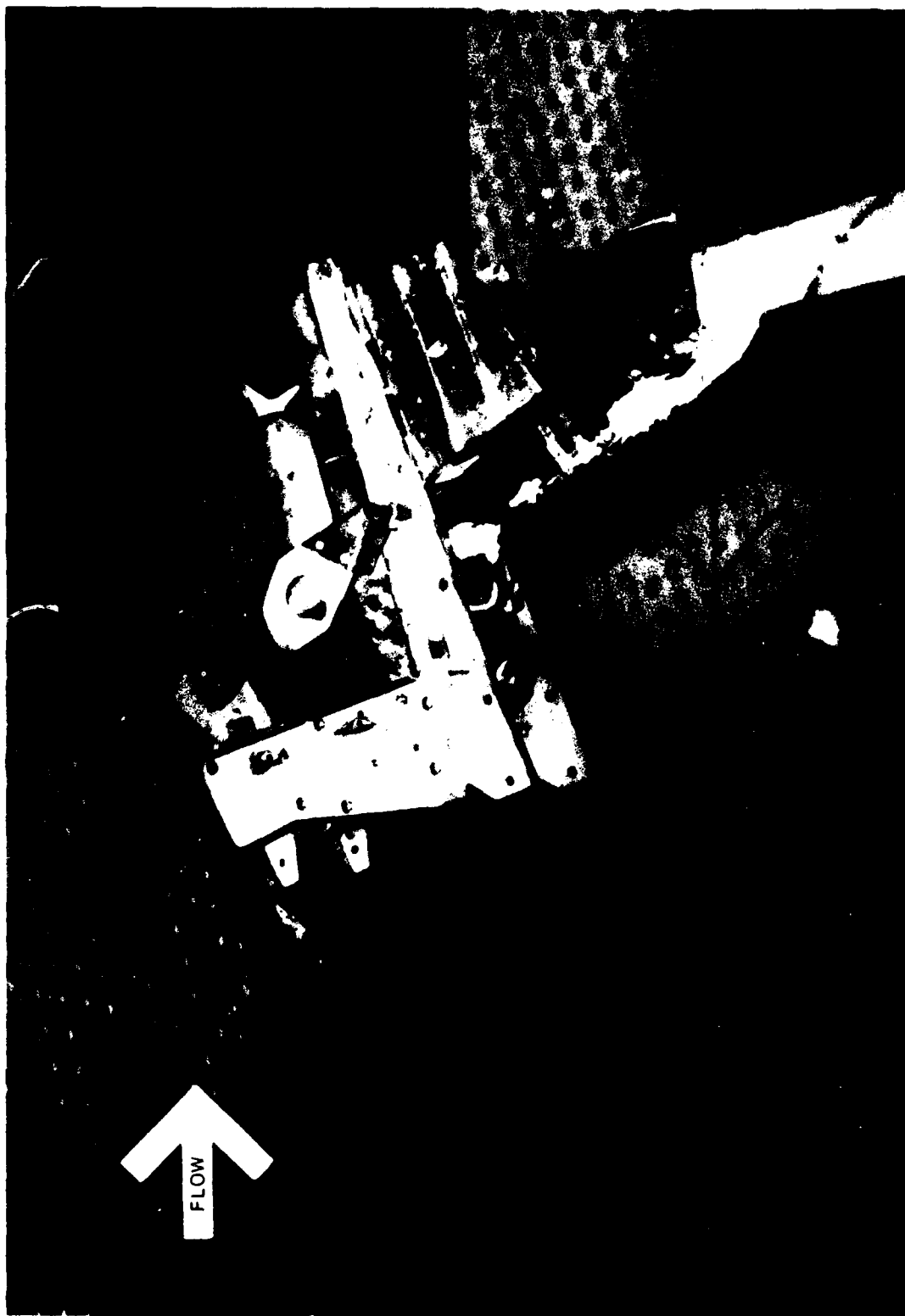
Figure 10. Basic Seat Showing Rocket Nozzle and Plenum Attached to Sting Support - Seat at \alpha=75^\circ (Configuration 9)
