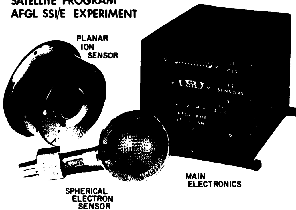
Figure 2-4: DMS SSI/E Flight Components
