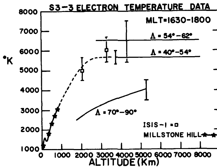
Figure 3-10: The profile of thermal electron temperatures as a function of altitude as determined by S3-3 in the late afternoon sector.
