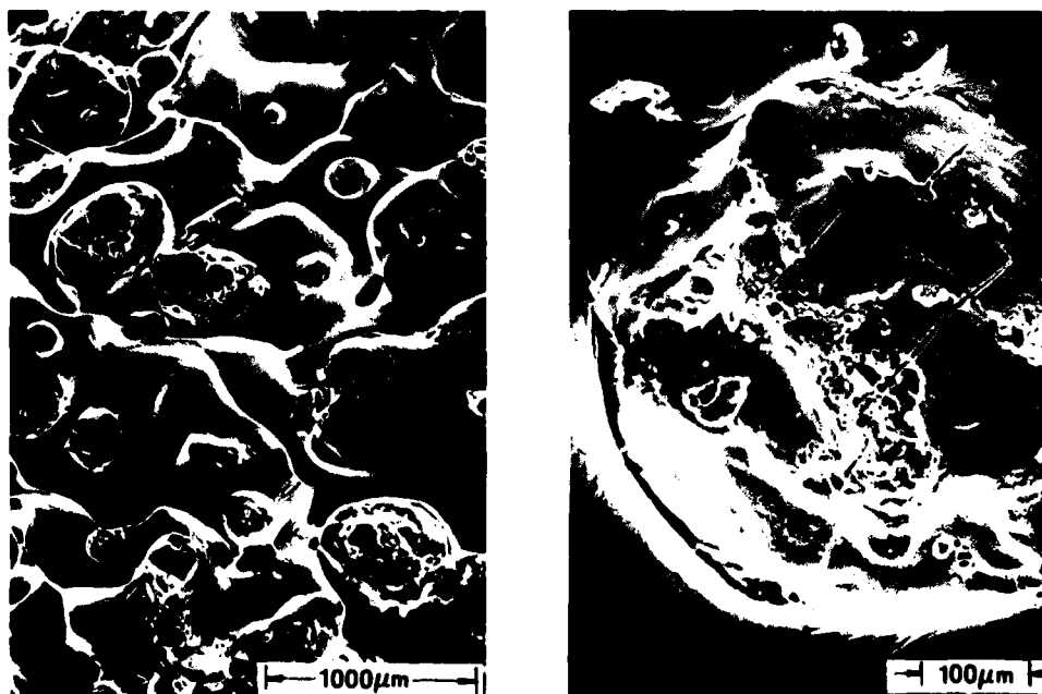
Figure 38. Quenched burning surfaces of AP-HTPB propellant with 600 μm AP, 25% binder. Samples quenched from 6.9 MPa.
