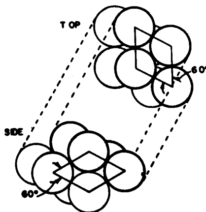
Fig. 1 Configuration of maximum packing density.
