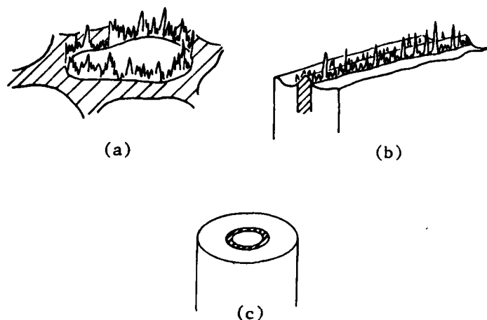
Figure 21. Nature of flame sheets.
