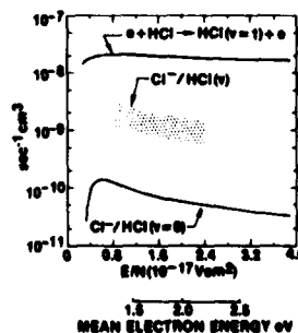
FIG. 1. Rate coefficients for vibrational excitation and dissociative attachment for HCl in the ground vibrational level, computed for a \text{Ne}(0.989) - \text{Xe}(0.01) - \text{HCl}(0.001) laser mixture. The shaded region is indicative of the magnitude of the effective rate coefficient for attachment to vibrationally excited HCl as inferred from the present study.
