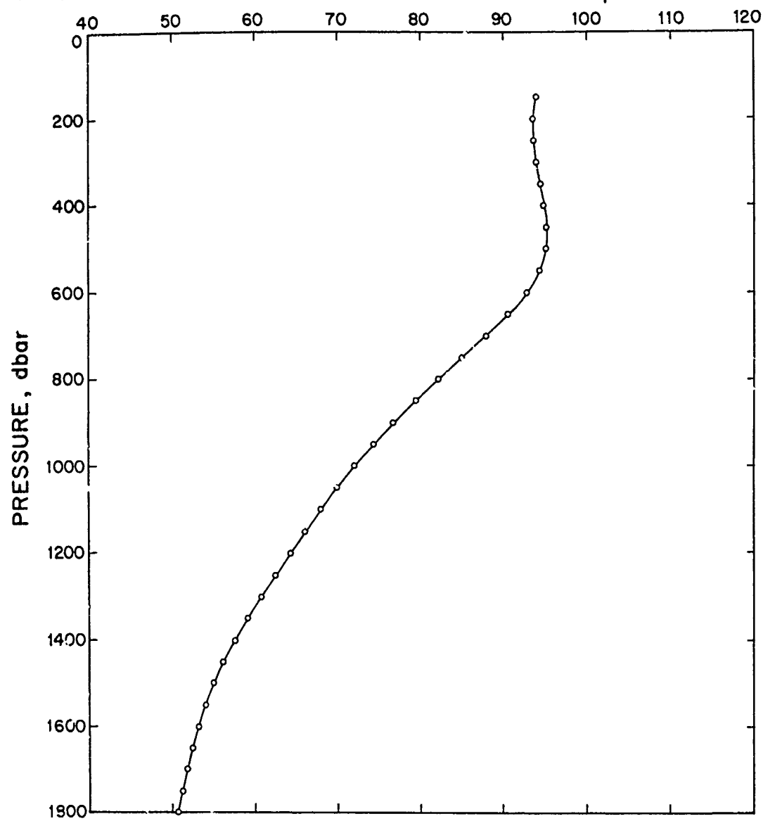
PHYGAS 42 REFERENCE SPECIFIC VOLUME ANOMALY, \delta_f ( 10^5 \text{ cm}^3 \cdot \text{gm}^{-1} )
