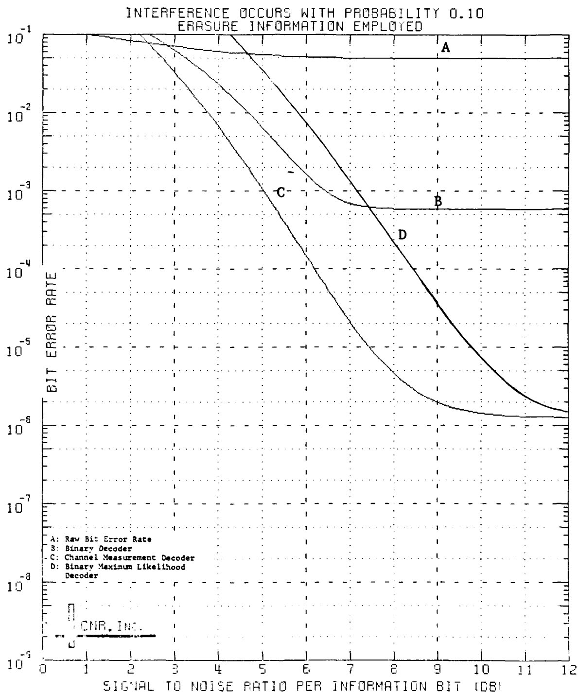
Figure 5.25 Decoded Performance of a Block Code Dimensions (24,12;8)
