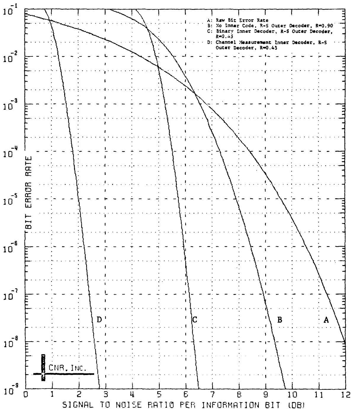
Figure 9.56 Decoded Performance of a Two-Stage Coding Approach Outer Decoder: Reed-Solomon Code (40,36;5) Bit Interleaver Employed Inner Decoder: Block Code (128,64;22) \delta=0.00 and No Erasure Information Employed
