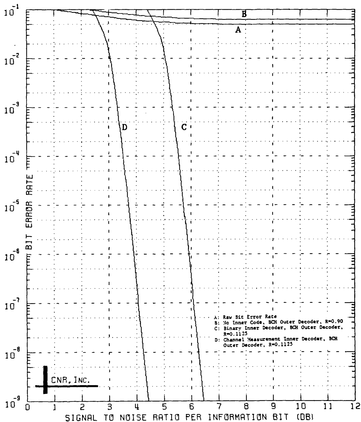
Figure 8.25 Decoded Performance of a Two-Stage Coding Approach Outer Decoder: BCH Code (240,216;7) Inner Decoder: Convolutional Code; Rate=1/8; K=7 \delta=0.10 and Erasure Information is Employed
