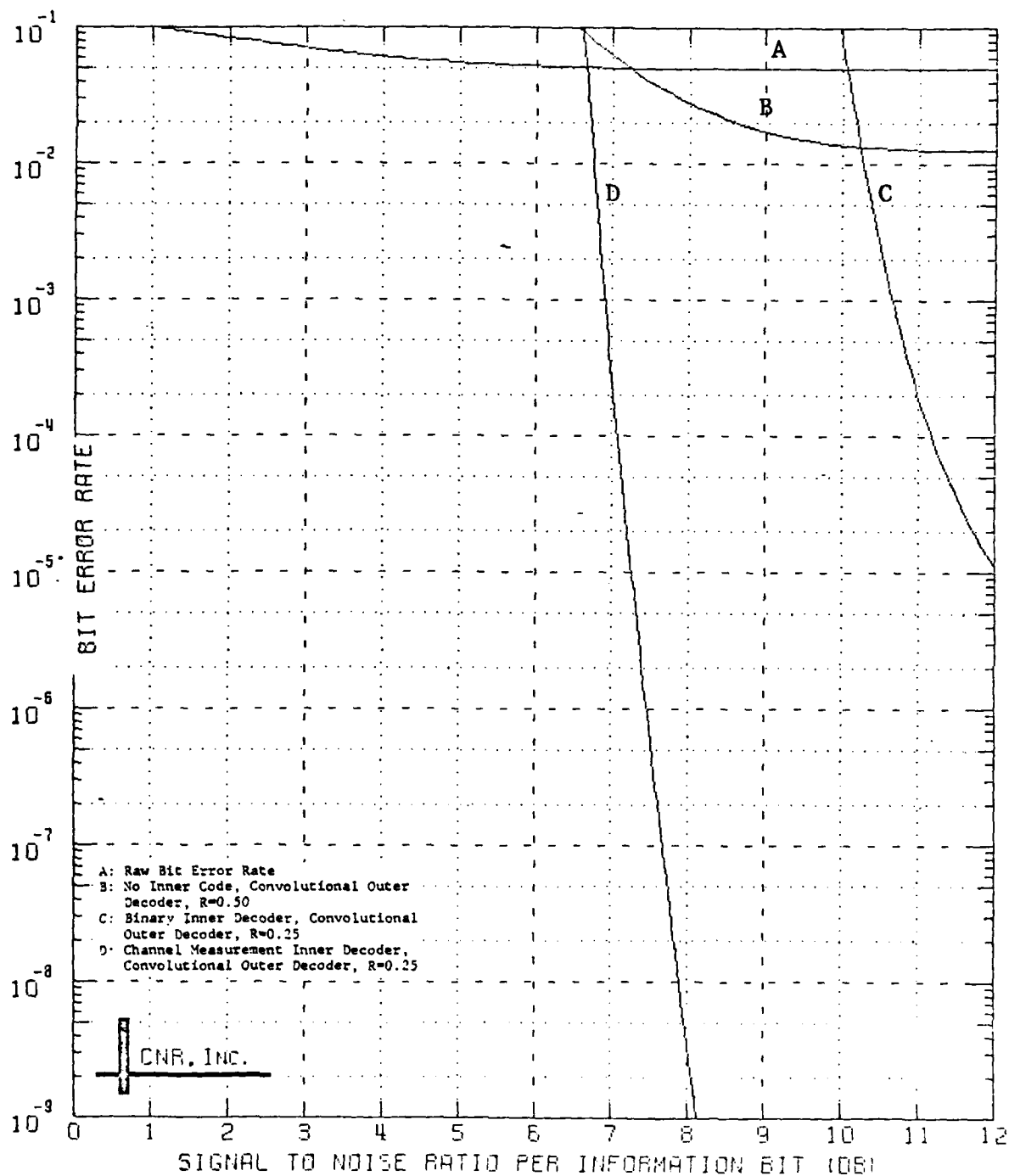
Figure 8.30 Decoded Performance of a Two-Stage Coding Approach Outer Decoder: Convolutional Code, Rate=1/2; K=7 Inner Decoder: Convolutional Code, Rate=1/2; K=7 \delta=0.10 and No Erasure Information Employed
