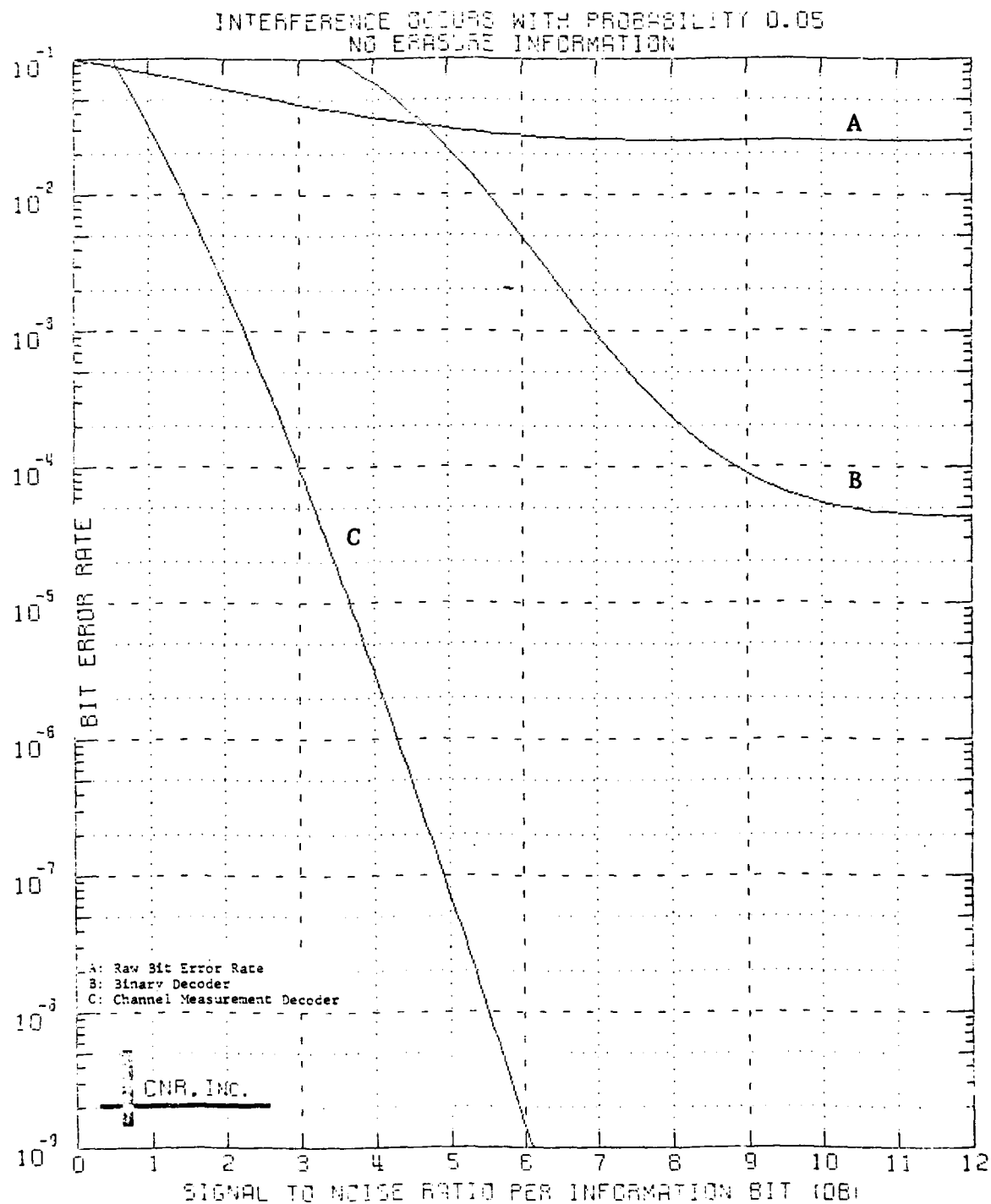
Figure 5.11 Decoded Performance of a Block Code Dimensions (128,64;22)
