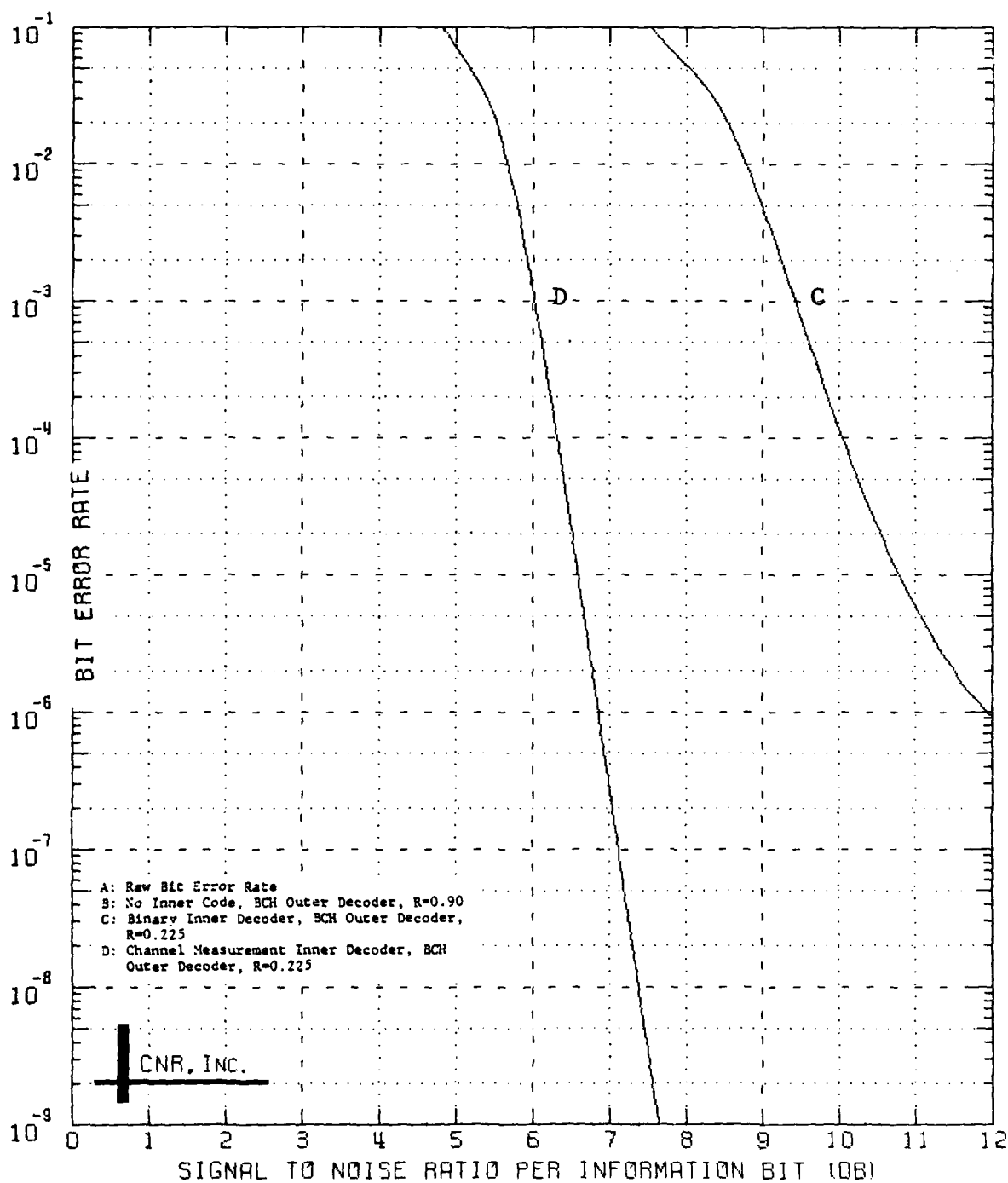
Figure 8.14 Decoded Performance of a Two-Stage Coding Approach Outer Decoder: BCH Code (240,216;7) Inner Decoder: Convolutional Code; Rate=1/4; K=7 \delta=0.20 and No Erasure Information Employed
