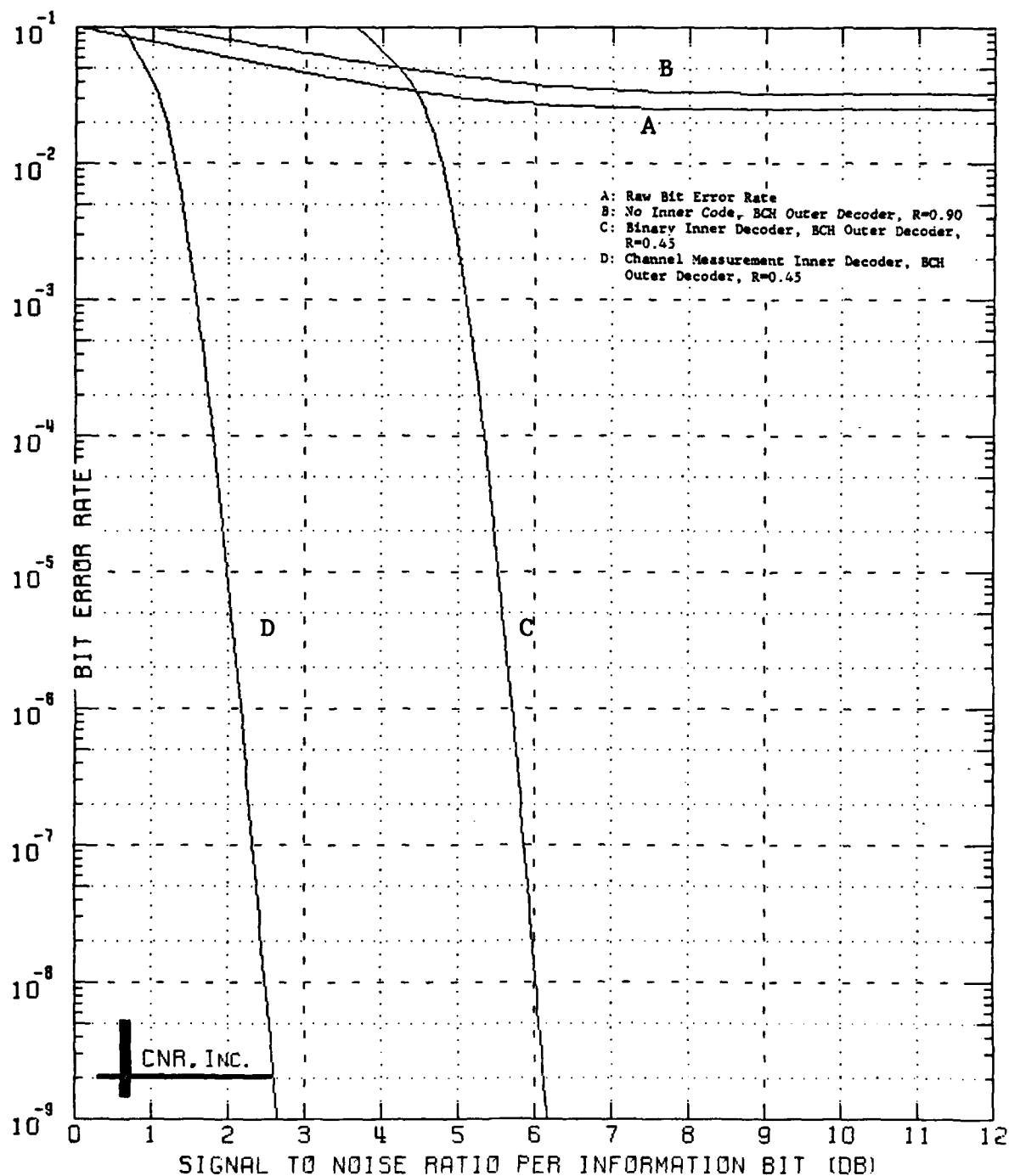
Figure 7.6 Decoded Performance of a Two-Stage Coding Approach Outer Decoder: BCH Code (240,216;7) Inner Decoder: Block Code (128,64;22) \delta=0.05 and Erasure Information is Employed
