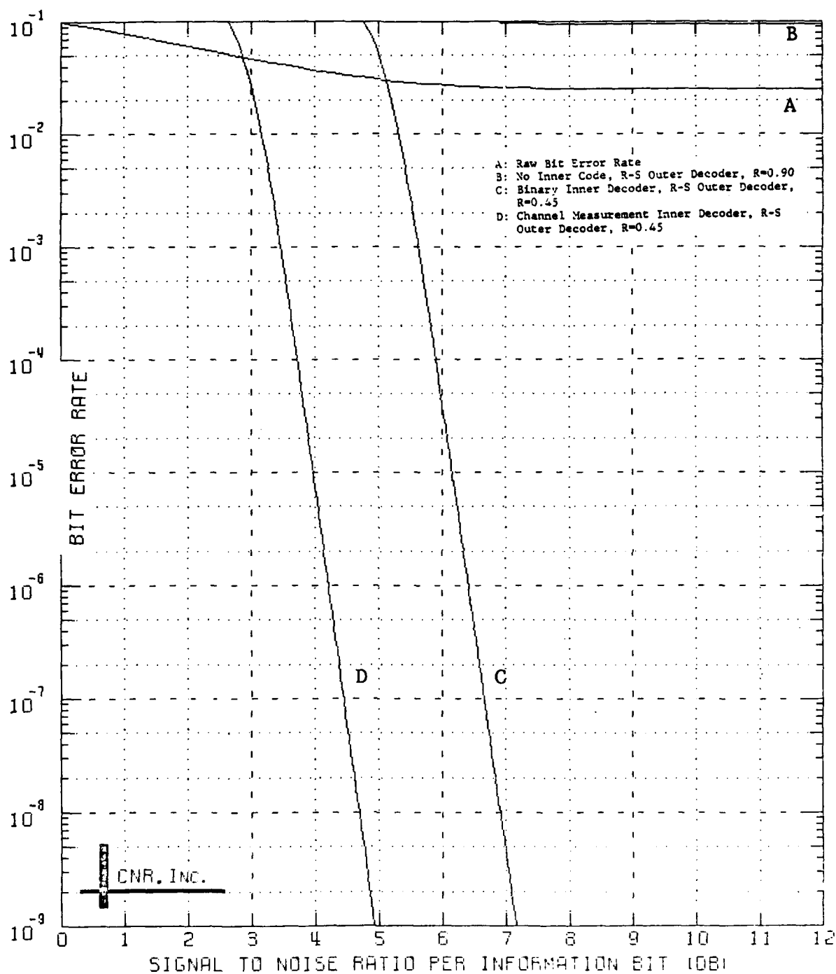
Figure 9.25 Decoded Performance of a Two-Stage Coding Approach Outer Decoder: Reed-Solomon Code (40,36;5) Bit Interleaver Employed Inner Decoder: Convolutional Code, Rate=1/2; K=7 \delta=0.05 and Erasure Information is Employed
