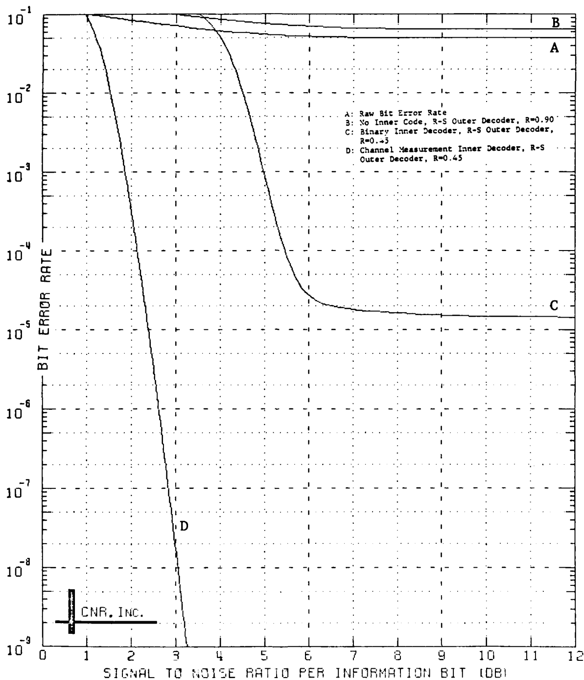
Figure 9.71 Decoded Performance of a Two-Stage Coding Approach Outer Decoder: Reed-Solomon Code (40,36;5) Symbol Interleaver Employed Inner Decoder: Block Code (128,64;22) \delta=0.10 and Erasure Information Employed
