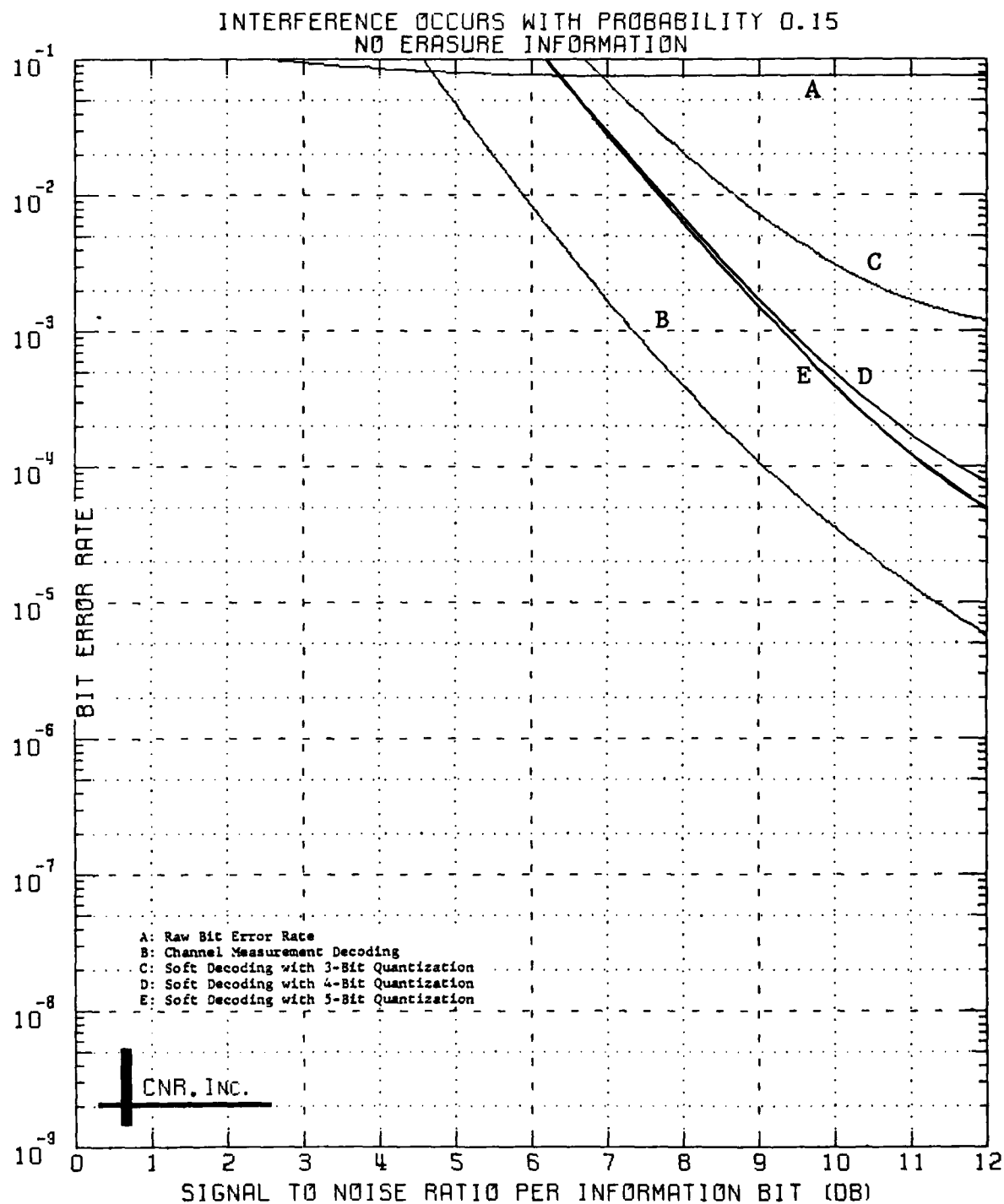
Figure 5 Decoded Performance of a Convolutional Code Rate 1/2; Constraint Length = 7; Gaussian Channel; CPSK Modulation
