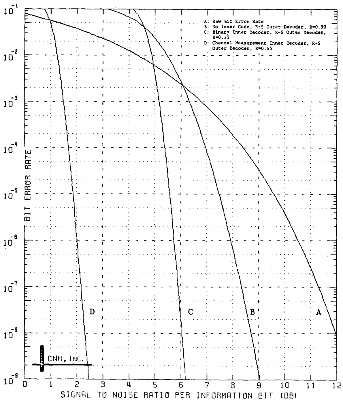
Figure 9.38 Decoded Performance of a Two-Stage Coding Approach Outer Decoder: Reed-Solomon Code (60,54;7) Bit Interleaver Employed Inner Decoder: Block Code (128,64;22) \delta=0.00 and No Erasure Information Employed
