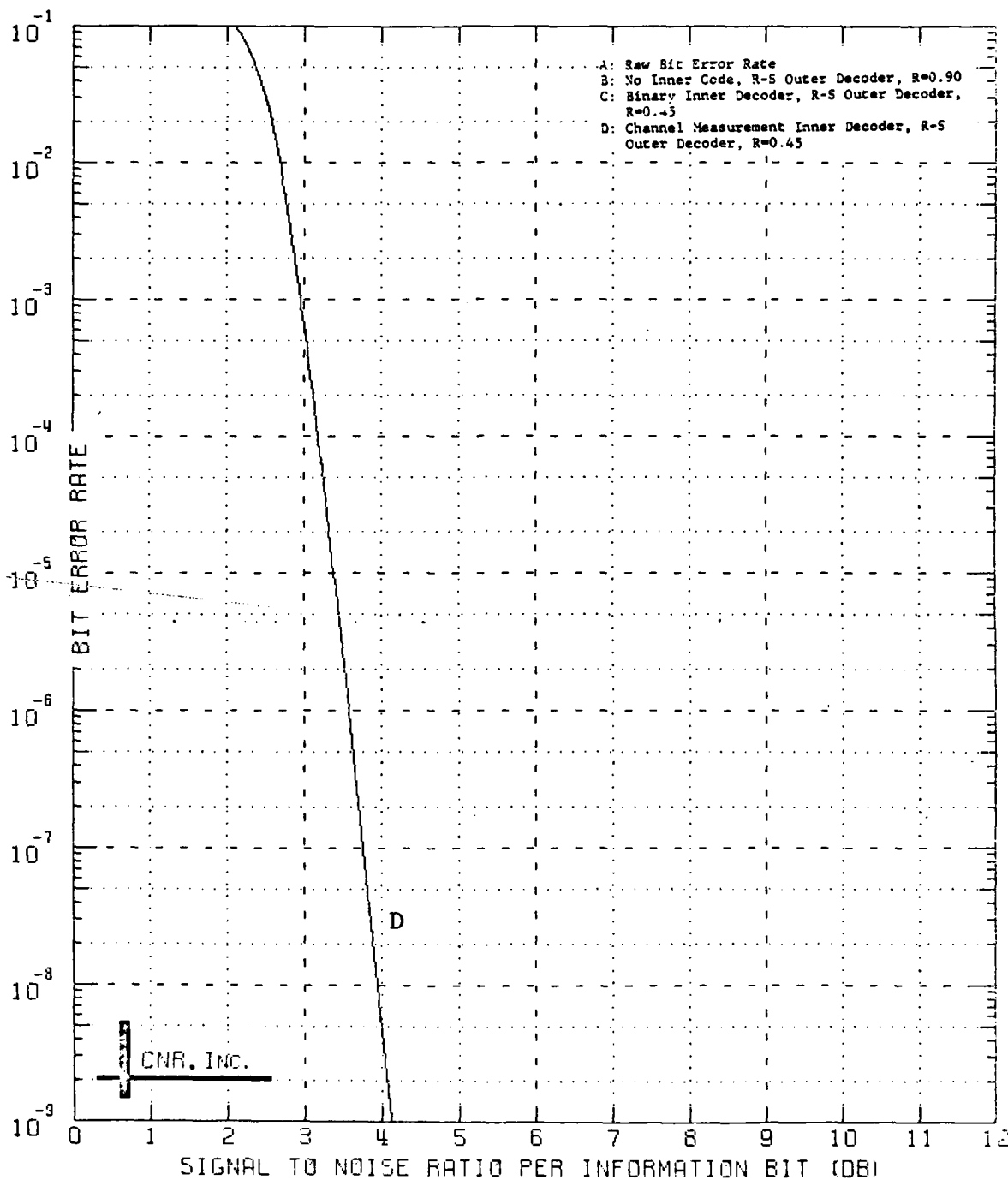
Figure 9.46 Decoded Performance of a Two-Stage Coding Approach Outer Decoder: Reed-Solomon Code (60,54;7) Bit Interleaver Employed Inner Decoder: Block Code (128,64;22) \delta=0.20 and Erasure Information is Employed
