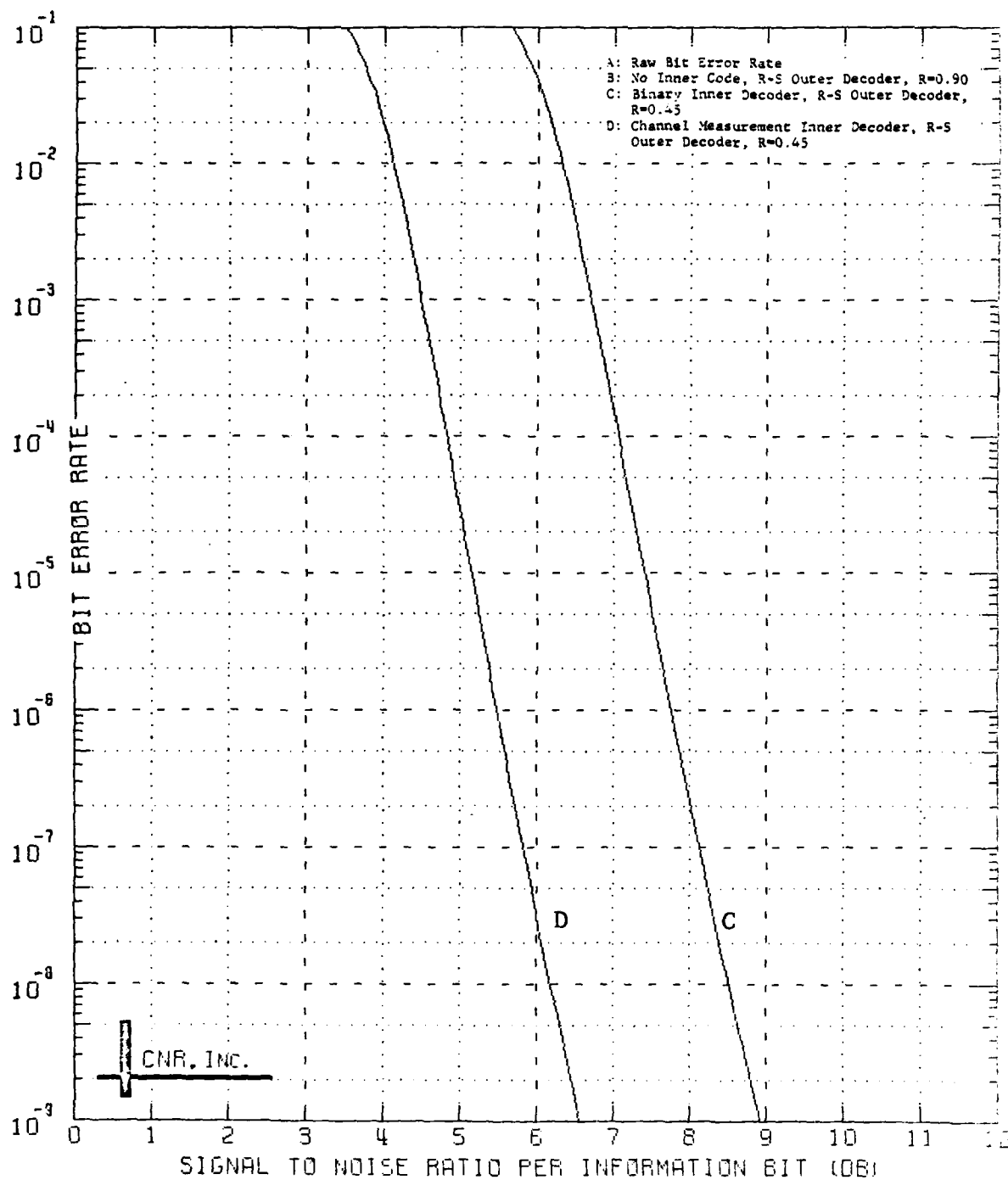
Figure 9.37 Decoded Performance of a Two-Stage Coding Approach Outer Decoder: Reed-Solomon Code (40,36;5) Symbol Interleaver Employed Inner Decoder: Convolutional Code, Rate=1/2; K=7 \delta=0.20 and Erasure Information is Employed
