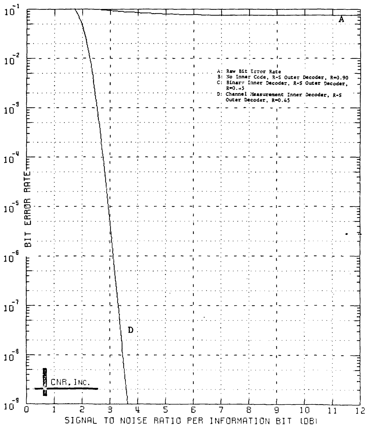
Figure 9.45 Decoded Performance of a Two-Stage Coding Approach Outer Decoder: Reed-Solomon Code (60,54;7) Bit Interleaver Employed Inner Decoder: Block Code (128,64;22) \delta=0.15 and Erasure Information is Employed
