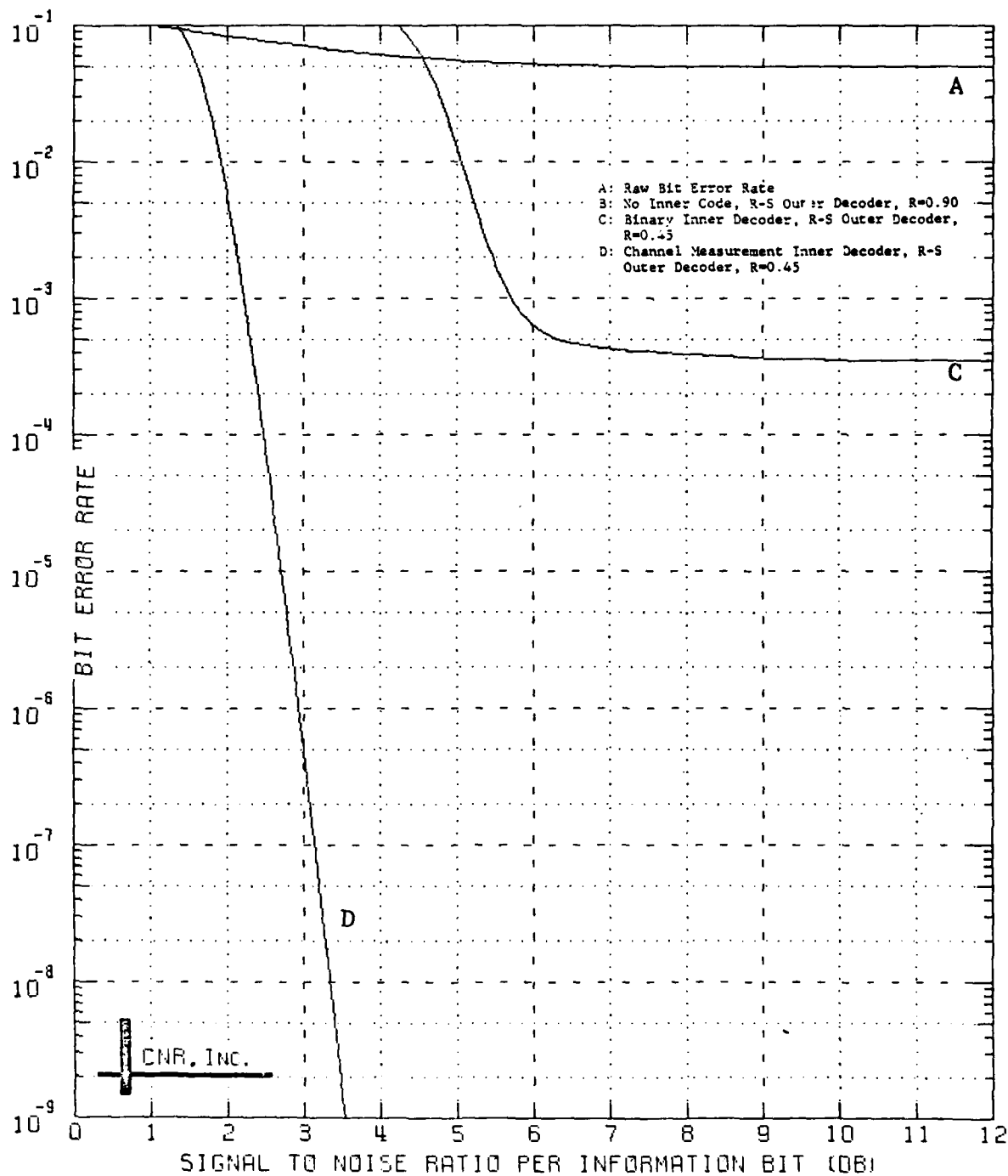
Figure 9.62 Decoded Performance of a Two-Stage Coding Approach Outer Decoder: Reed-Solomon Code (40,36;5) Bit Interleaver Employed Inner Decoder: Block Code (128,64;22) \delta=0.10 and Erasure Information Employed
