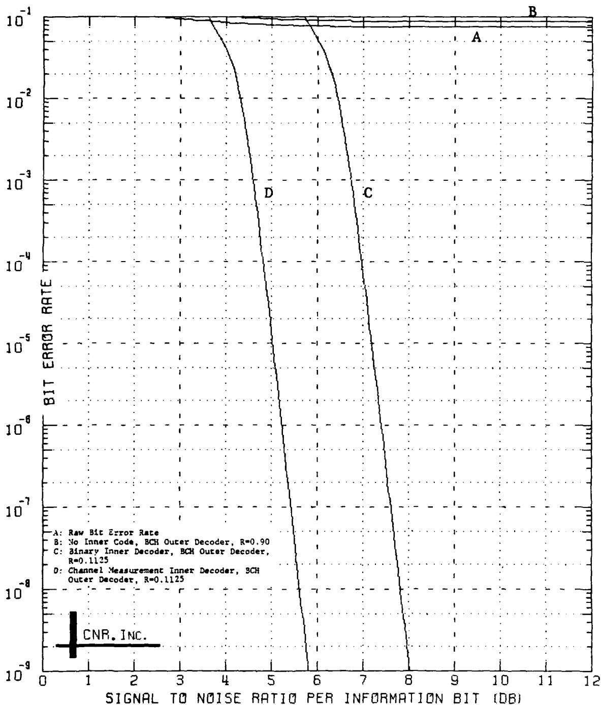
Figure 8.22 Decoded Performance of a Two-Stage Coding Approach Outer Decoder: BCH Code (240,216;7) Inner Decoder: Convolutional Code; Rate=1/8; K=7 \delta=0.15 and No Erasure Information Employed
