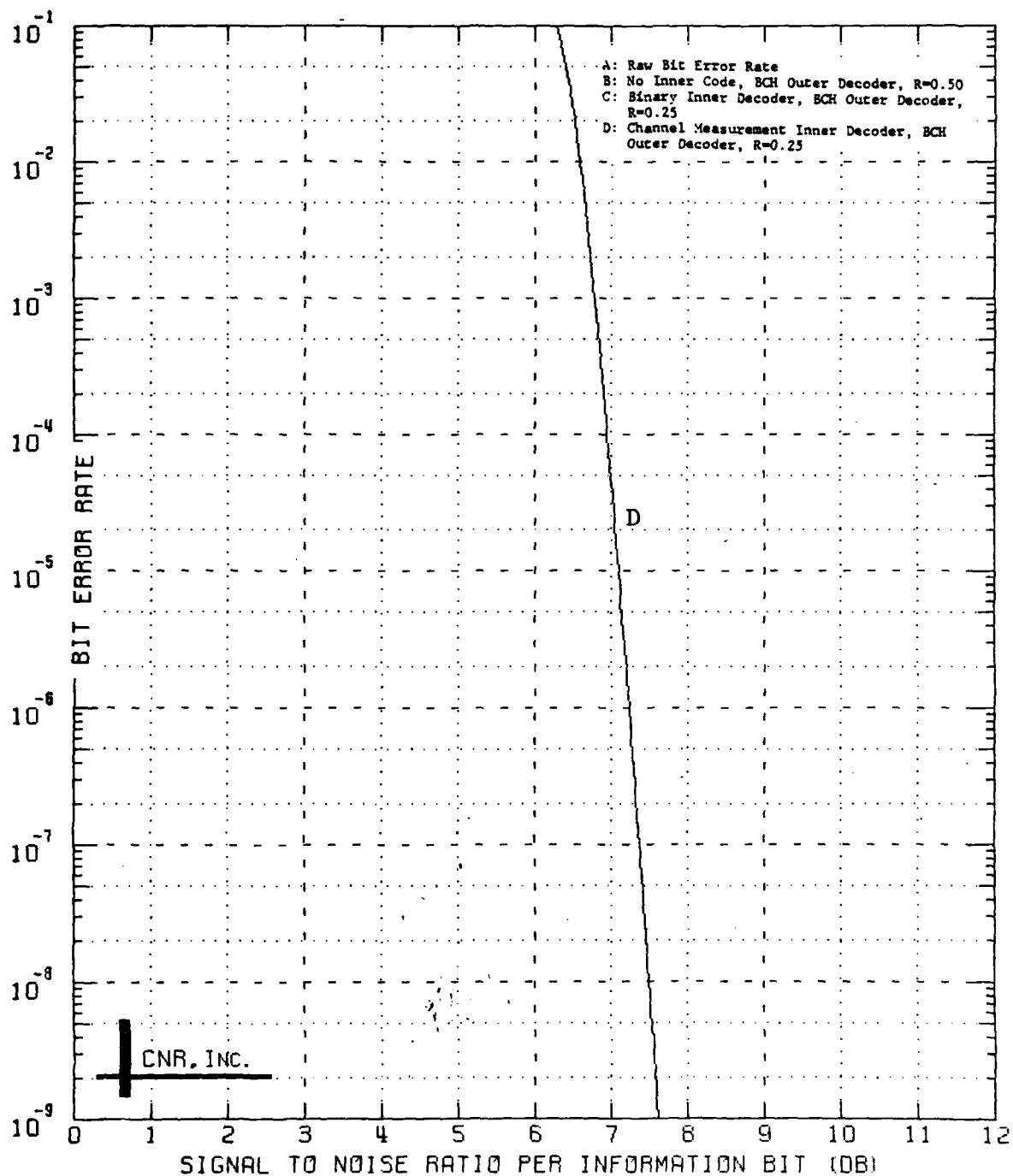
Figure 7.14 Decoded Performance of a Two-Stage Coding Approach Outer Decoder: BCH Code (128,64;22) Inner Decoder: Block Code (128,64;22) \delta=0.20 and No Erasure Information Employed
