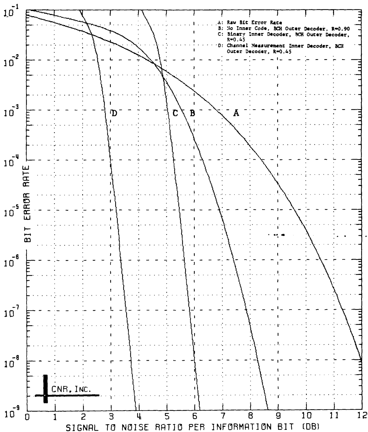
Figure 8.1 Decoded Performance of a Two-Stage Coding Approach Outer Decoder: BCH Code (240,216;7) Inner Decoder: Convolutional Code; Rate=1/2; K=7 \delta=0.00 and No Erasure Information Employed
