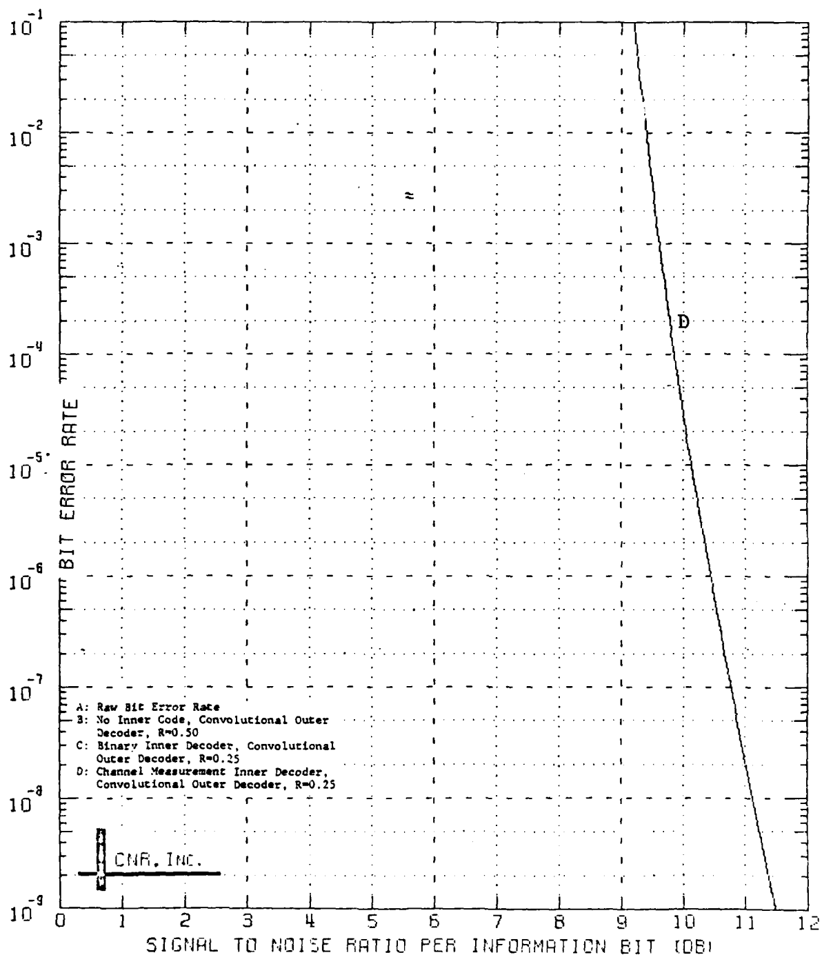
Figure 8.32 Decoded Performance of a Two-Stage Coding Approach Outer Decoder: Convolutional Code, Rate=1/2; K=7 Inner Decoder: Convolutional Code, Rate=1/2; K=7 \delta=0.20 and No Erasure Information Employed
