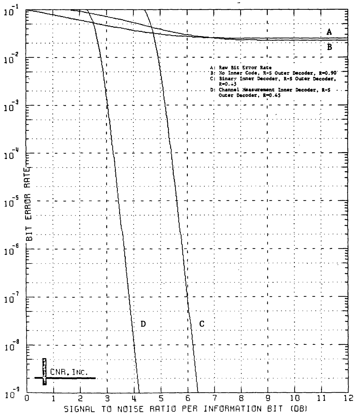
Figure 9.16 Decoded Performance of a Two-Stage Coding Approach Outer Decoder: Reed-Solomon Code (60,54;7) Symbol Interleaver Employed Inner Decoder: Convolutional Code, Rate=1/2; K=7 \delta=0.05 and Erasure Information is Employed
