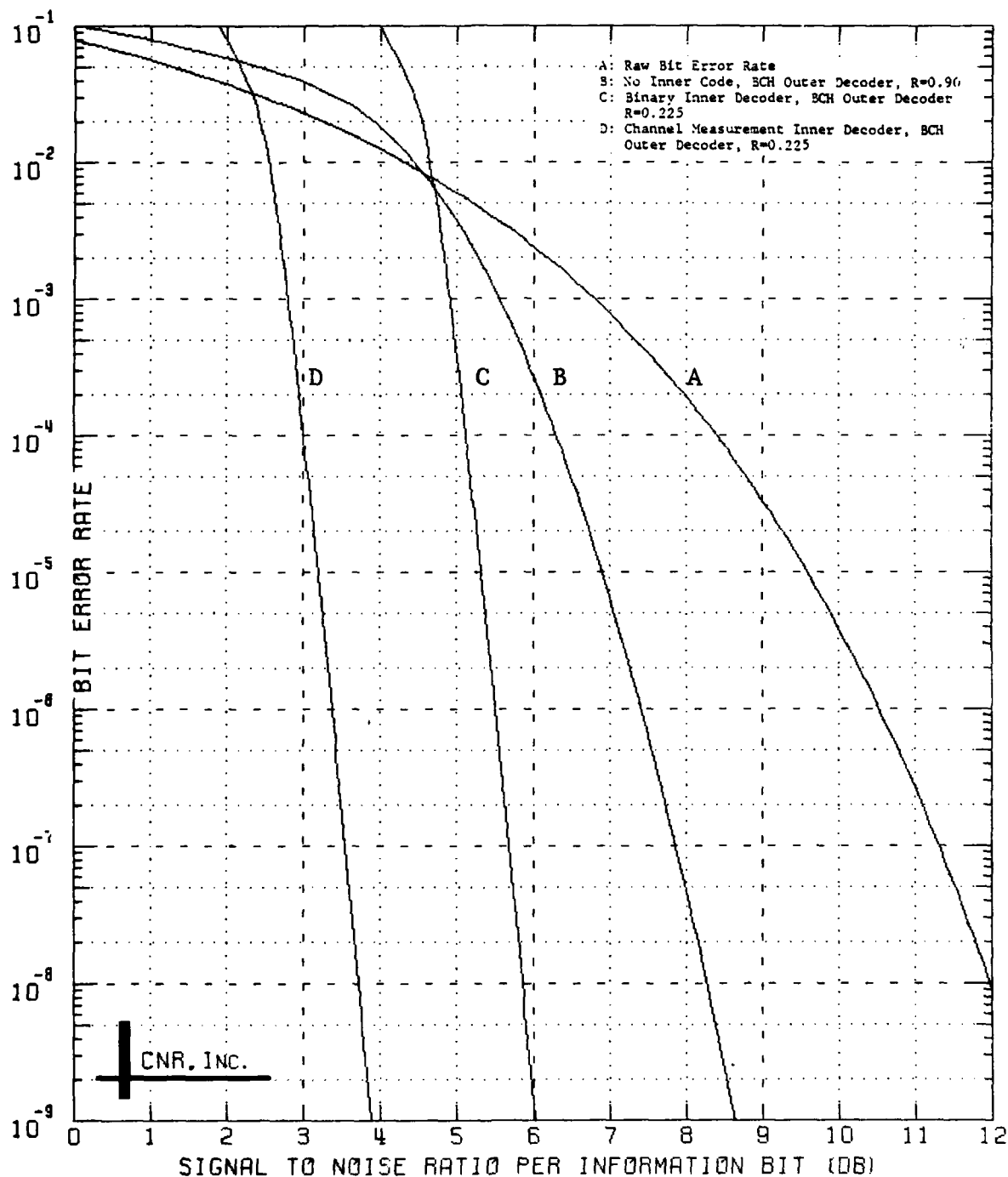
Figure 8.10 Decoded Performance of a Two-Stage Coding Approach Outer Decoder: BCH Code (240,216;7) Inner Decoder: Convolutional Code; Rate=1/4; K=7 \delta=0.00 and No Erasure Information is Employed
