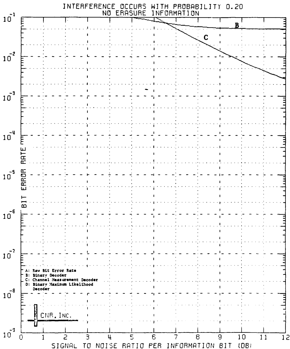
Figure 5.23 Decoded Performance of a Block Code Dimensions (24,12;8)
