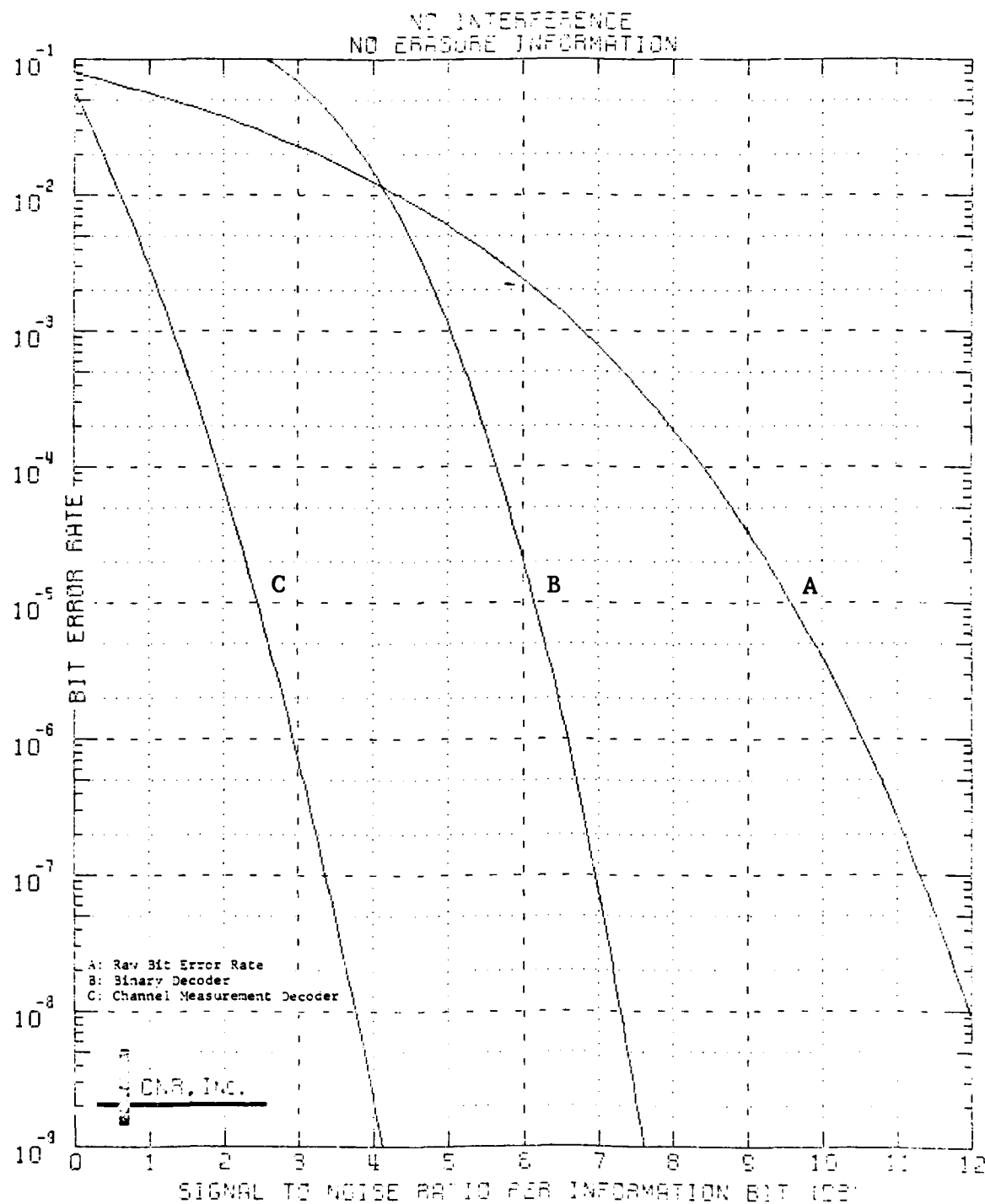
Figure 5.10 Decoded Performance of a Block Code Dimensions (128,64;22)
