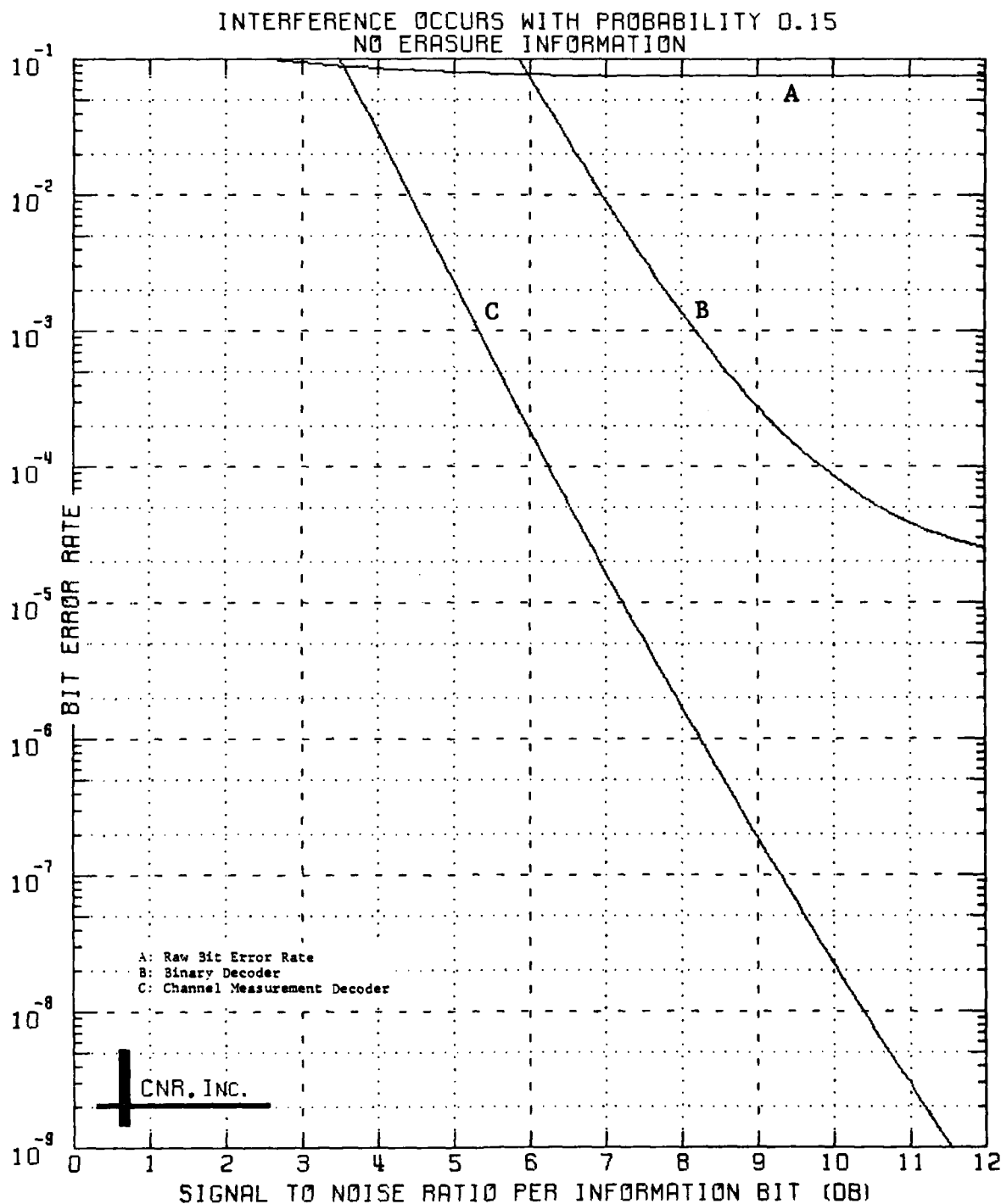
Figure 6.13 Decoded Performance of a Convolutional Code Rate 1/4; Constraint Length = 7
