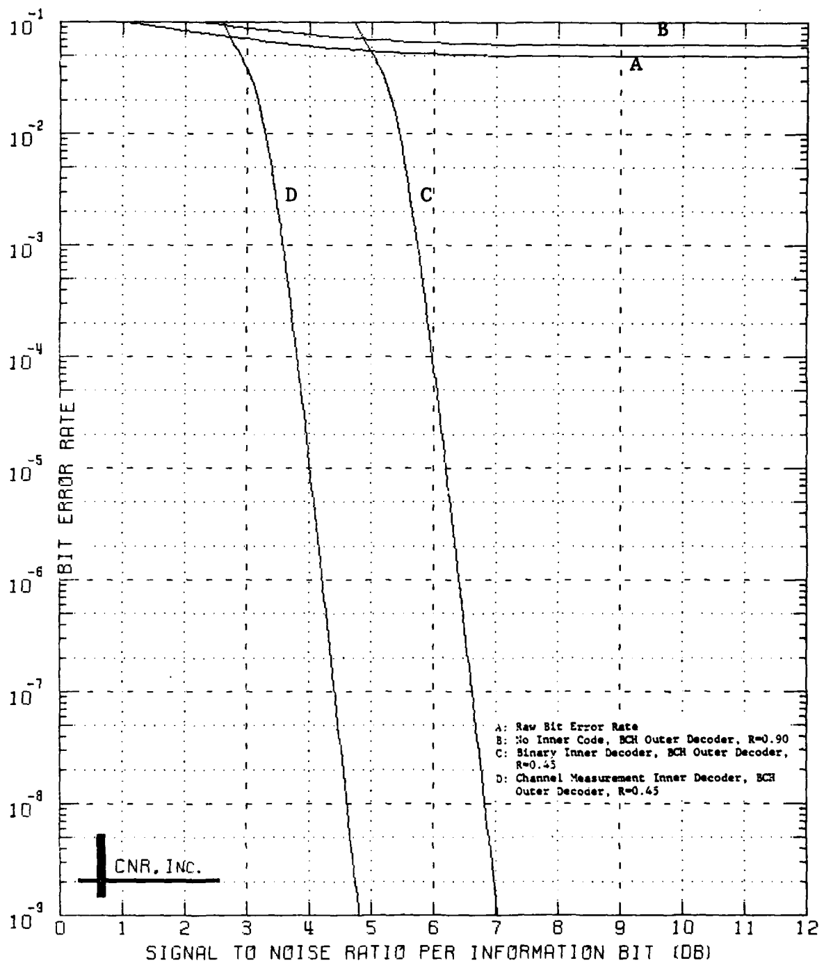
Figure 8.7 Decoded Performance of a Two-Stage Coding Approach Outer Decoder: BCH Code (240,216;7) Inner Decoder: Convolutional Code; Rate=1/2; K=7 \delta=0.10 and Erasure Information is Employed
