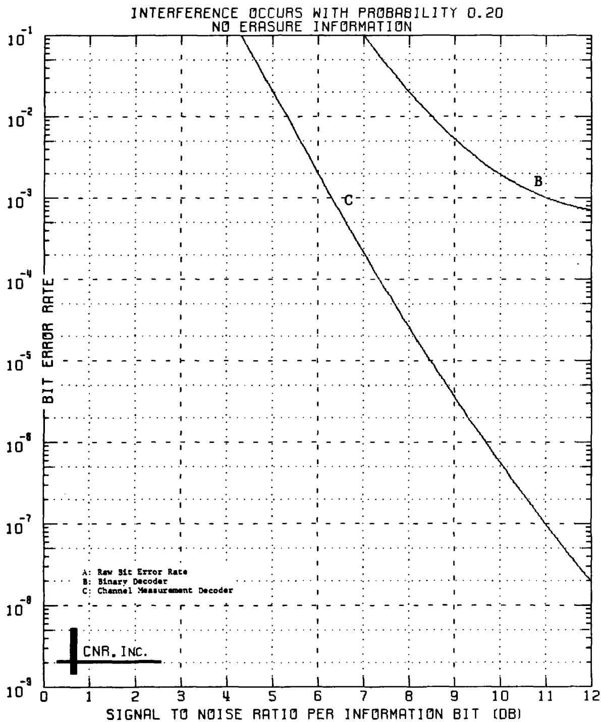
Figure 6.14 Decoded Performance of a Convolutional Code Rate 1/4; Constraint Length = 7
