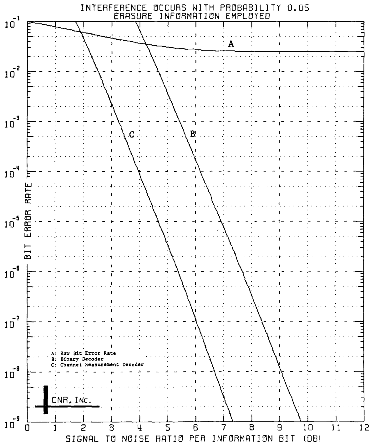
Figure 6.6 Decoded Performance of a Convolutional Code Rate 1/2; Constraint Length = 7
