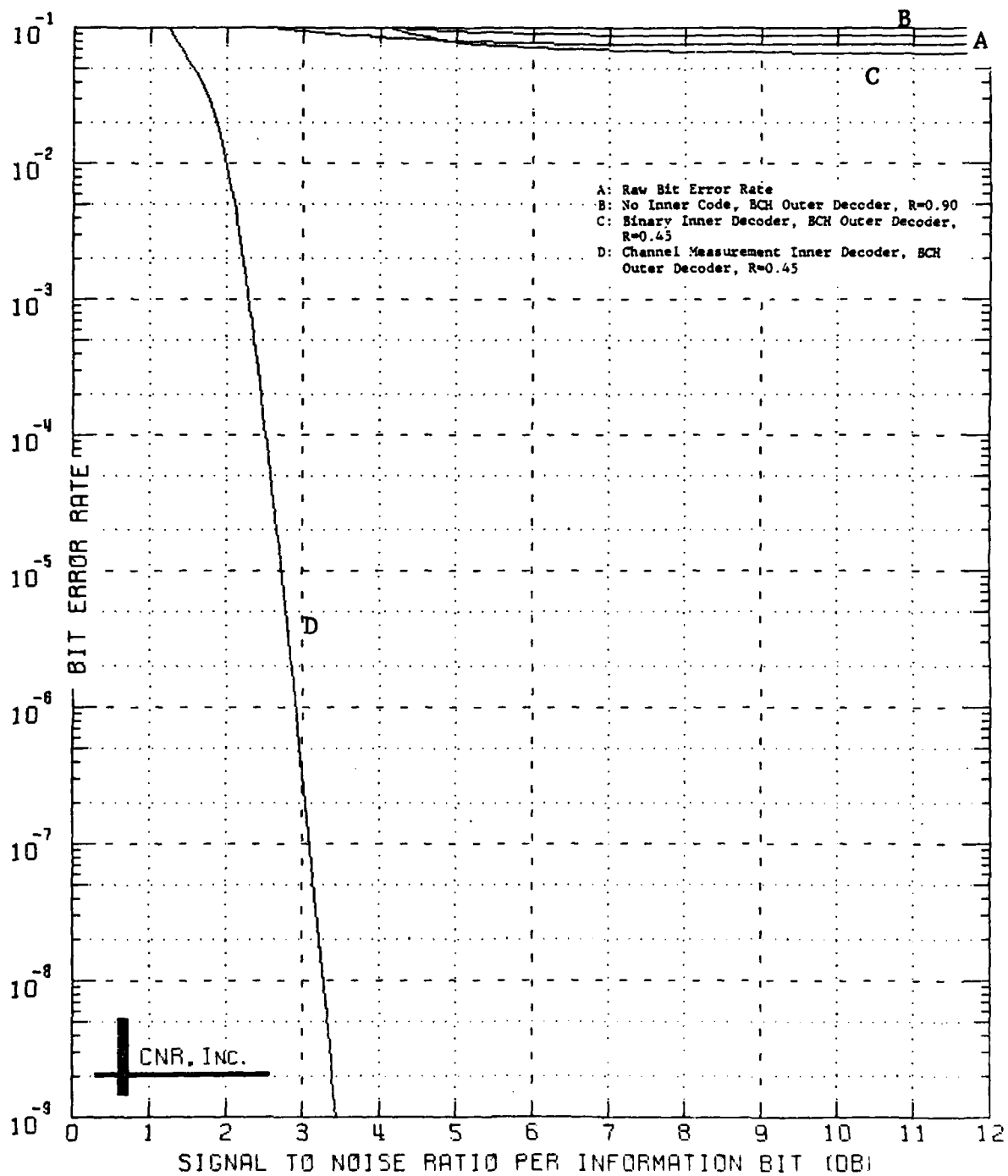
Figure 7.8 Decoded Performance of a Two-Stage Coding Approach Outer Decoder: BCH Code (240,216;7) Inner Decoder: Block Code (128,64;22) \delta=0.15 and Erasure Information is Employed
