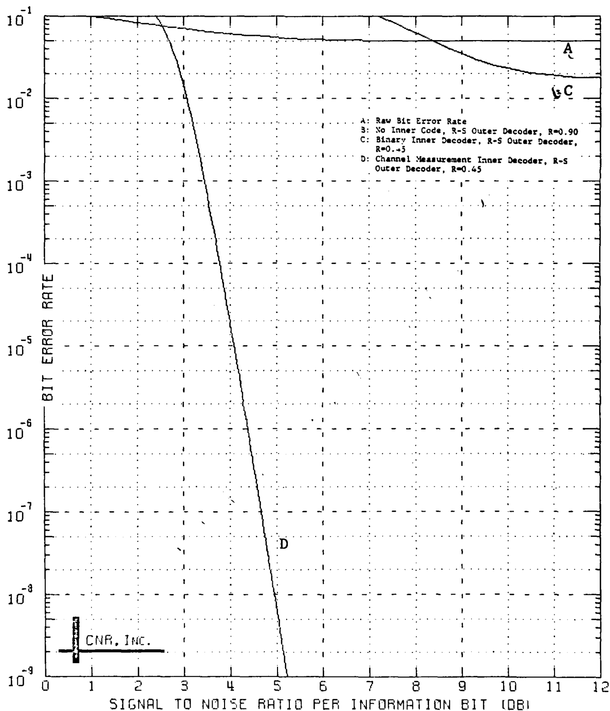
Figure 9.58 Decoded Performance of a Two-Stage Coding Approach Outer Decoder: Reed-Solomon Code (40,36;5) Bit Interleaver Employed Inner Decoder: Block Code (128,64;22) \delta=0.10 and No Erasure Information Employed
