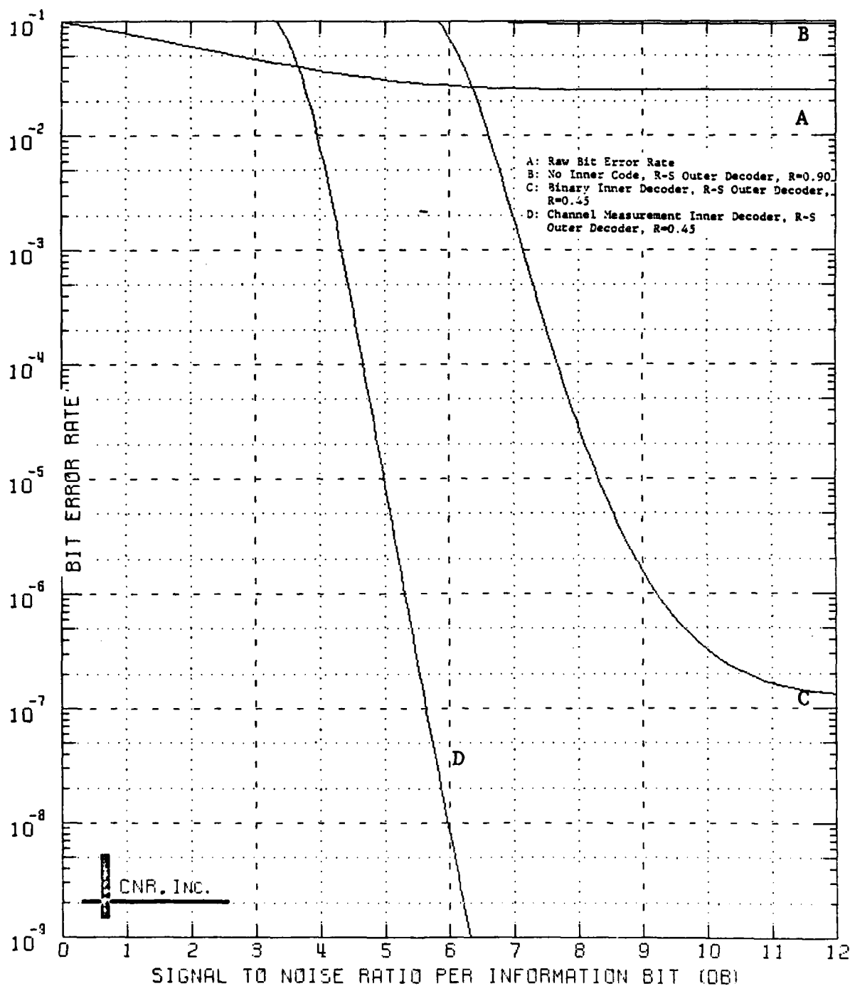
Figure 9.21 Decoded Performance of a Two-Stage Coding Approach Outer Decoder: Reed-Solomon Code (40,36;5) Bit Interleaver Employed Inner Decoder: Convolutional Code, Rate=1/2; K=7 \delta=0.05 and No Erasure Information Employed
