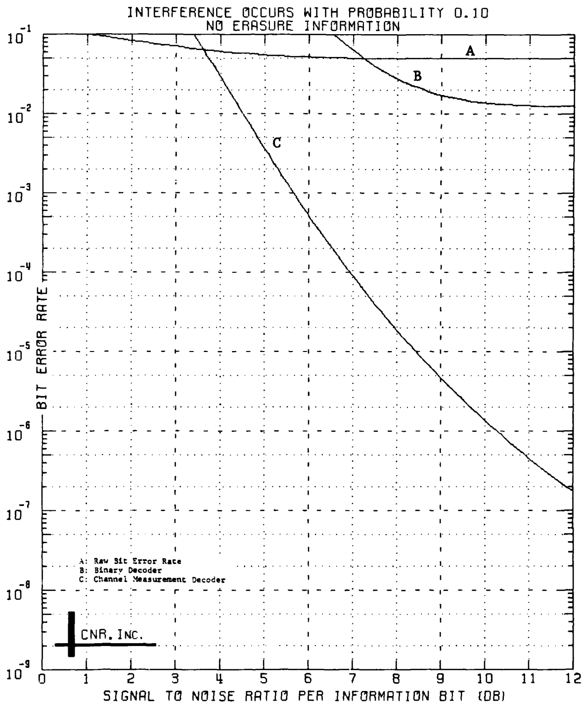
Figure 6.3 Decoded Performance of a Convolutional Code Rate 1/2; Constraint Length = 7
