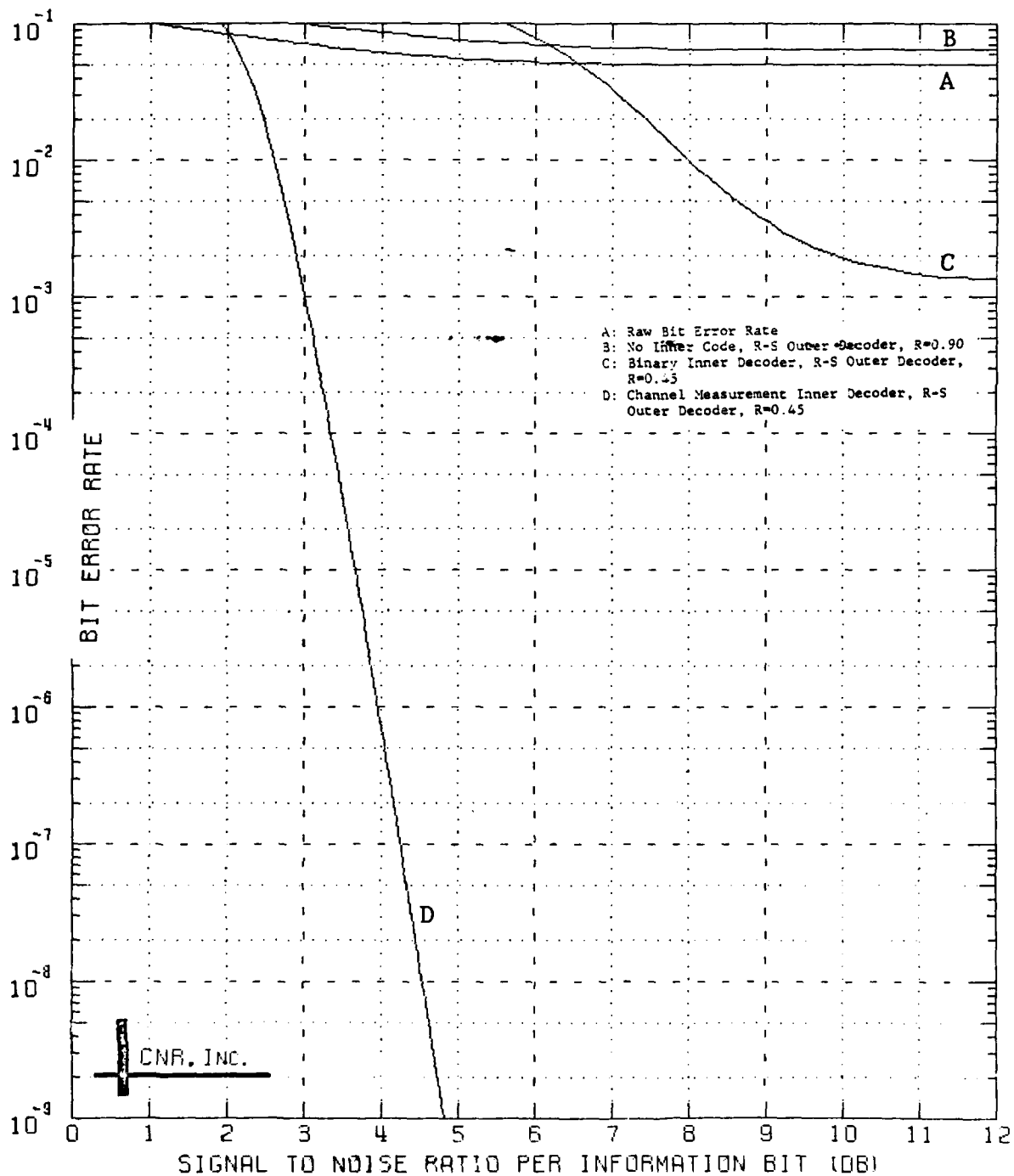
Figure 9.67 Decoded Performance of a Two-Stage Coding Approach Outer Decoder: Reed-Solomon Code (40,36;5) Symbol Interleaver Employed Inner Decoder: Block Code (128,64;22) \delta=0.10 and No Erasure Information Employed
