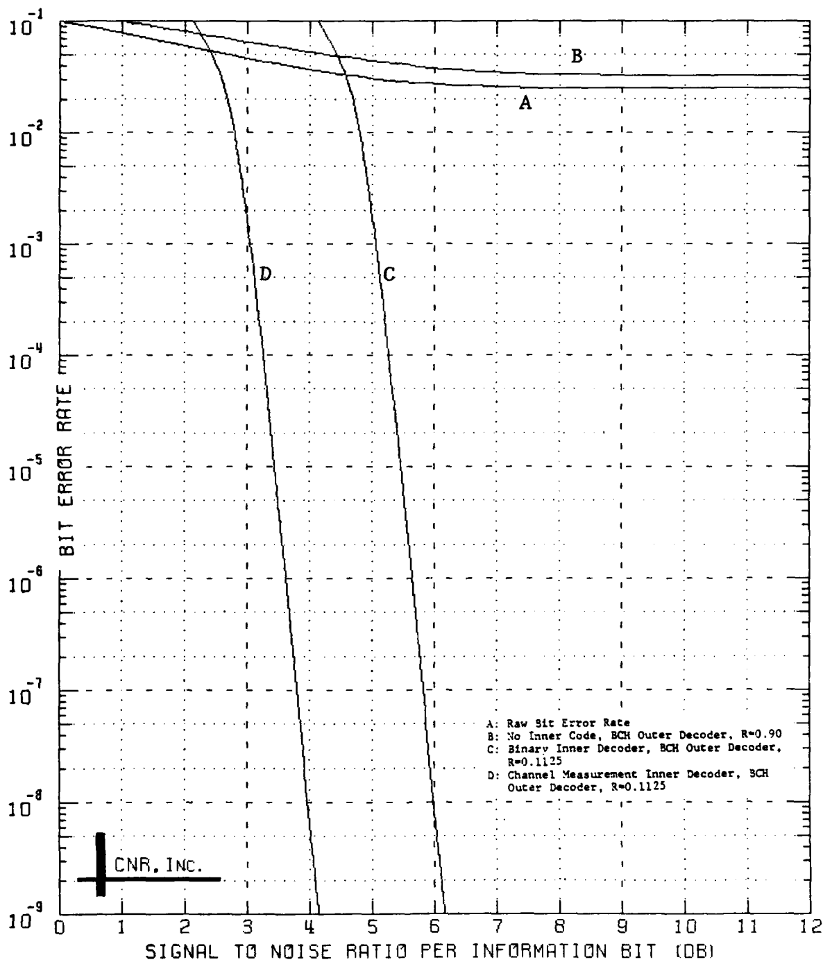
Figure 8.24 Decoded Performance of a Two-Stage Coding Approach Outer Decoder: BCH Code (240,216;7) Inner Decoder: Convolutional Code; Rate=1/8; K=7 \delta=0.05 and Erasure Information is Employed
