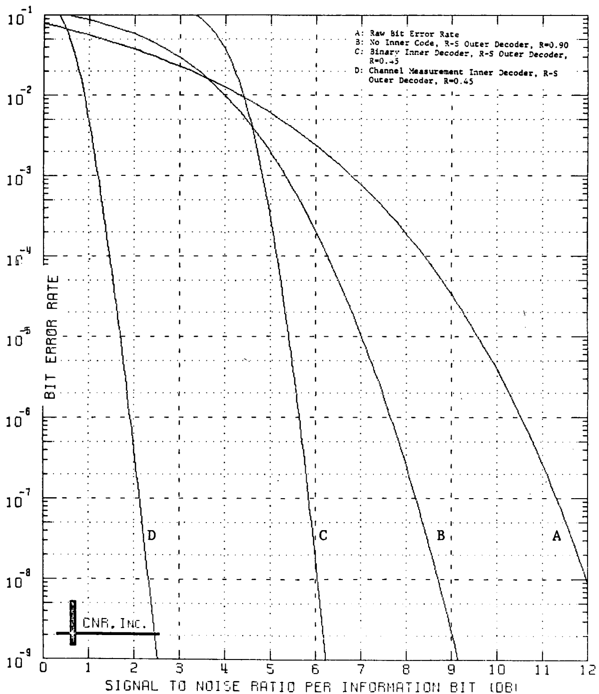
Figure 9.65 Decoded Performance of a Two-Stage Coding Approach Outer Decoder: Reed-Solomon Code (40,36;5) Symbol Interleaver Employed Inner Decoder: Block Code (128,64;22) \delta = 0.00 and No Erasure Information Employed
