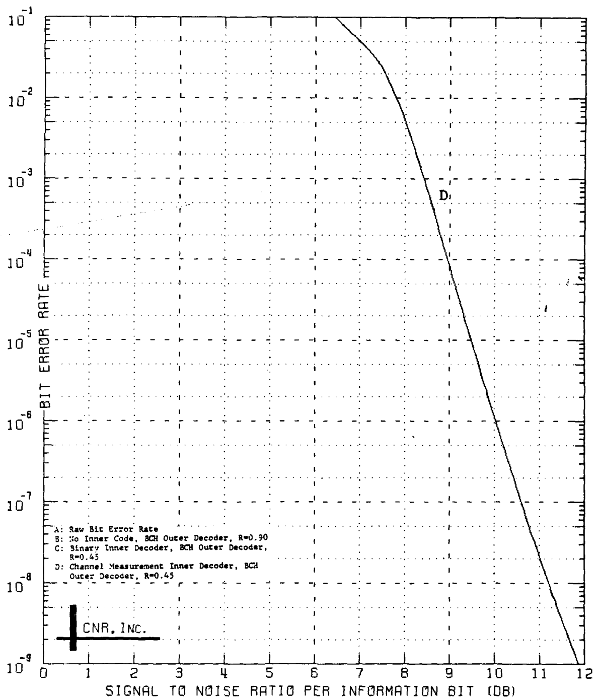
Figure 8.5 Decoded Performance of a Two-Stage Coding Approach Outer Decoder: BCH Code (240,216;7) Inner Decoder: Convolutional Code; Rate=1/2; K=7 \delta=0.20 and No Erasure Information Employed
