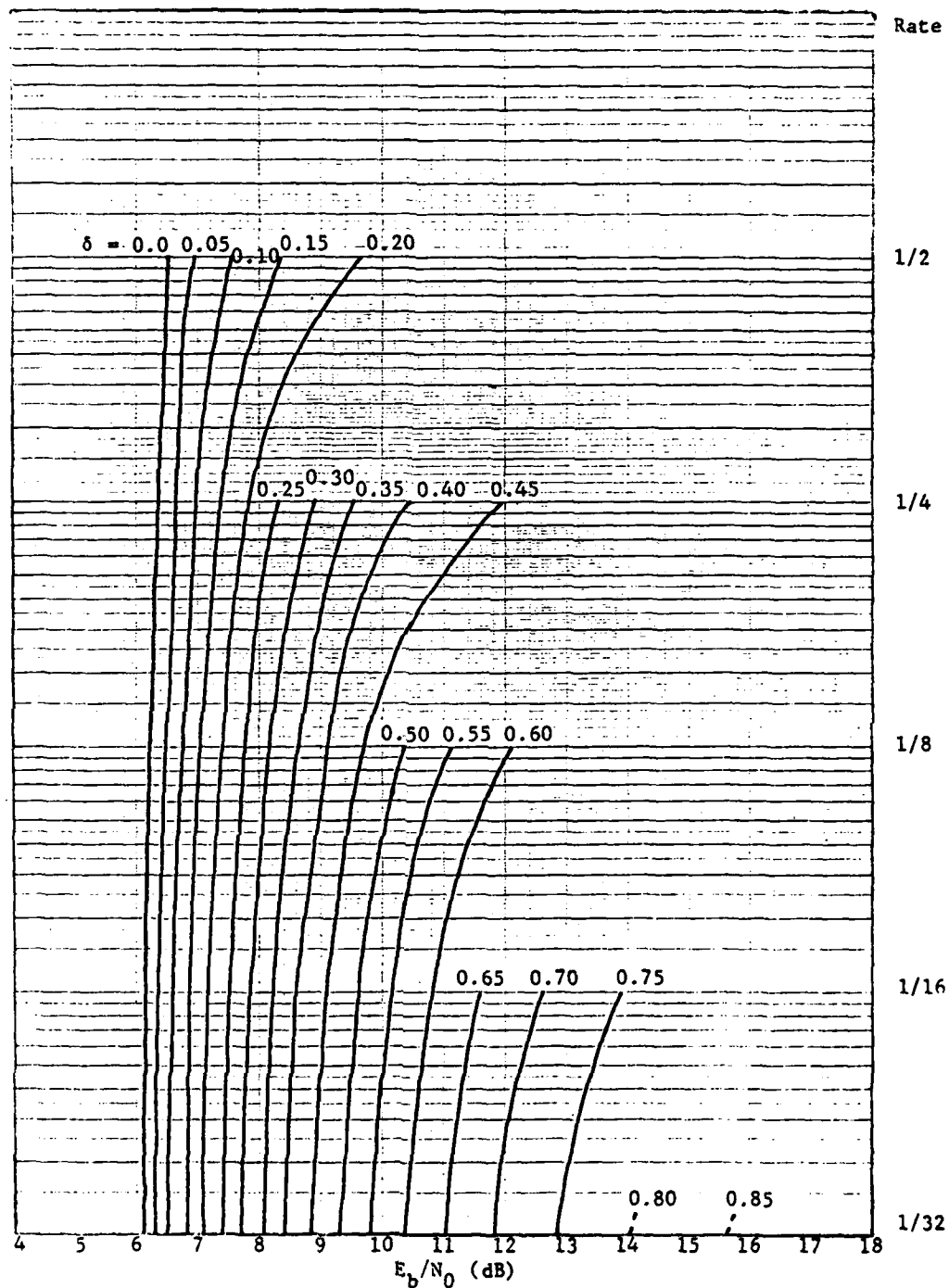
Figure 6.35 Convolutional Coding Performance with Interference Probability as a Parameter Binary Decoding-Erasure Information Available
