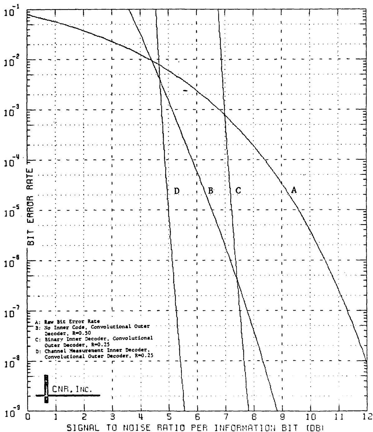
Figure 8.28 Decoded Performance of a Two-Stage Coding Approach Outer Decoder: Convolutional Code, Rate=1/2; K=7 Inner Decoder: Convolutional Code, Rate=1/2; K=7 \delta=0.00 and No Erasure Information Employed
