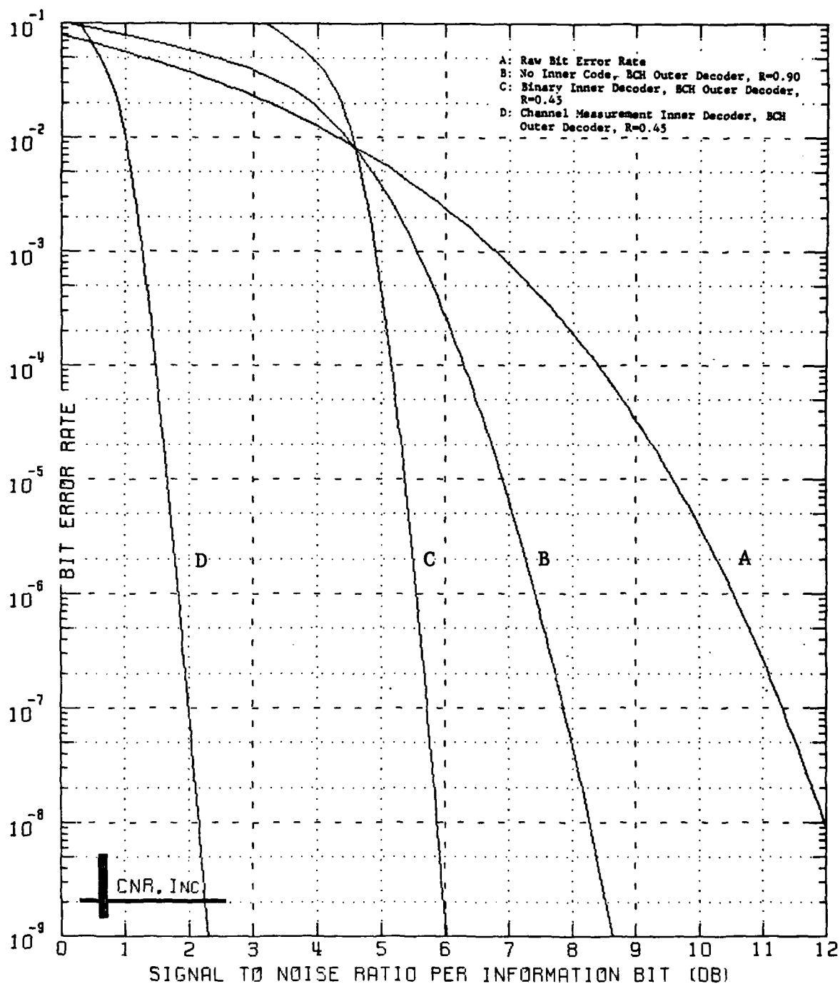
Figure 7.1 Decoded Performance of a Two-Stage Coding Approach Outer Decoder: BCH Code (240,216;7) Inner Decoder: Block Code (128,64;22) \delta=0.0 and No Erasure Information Employed
