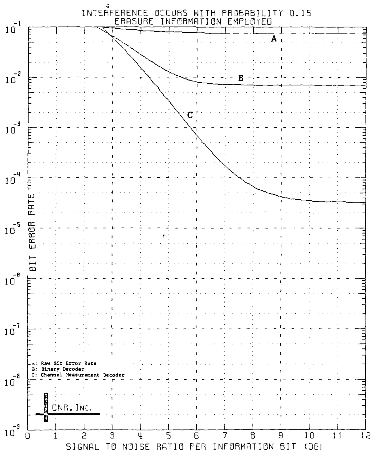
Figure 5.8 Decoded Performance of a Block Code Dimensions (24,12;8)
