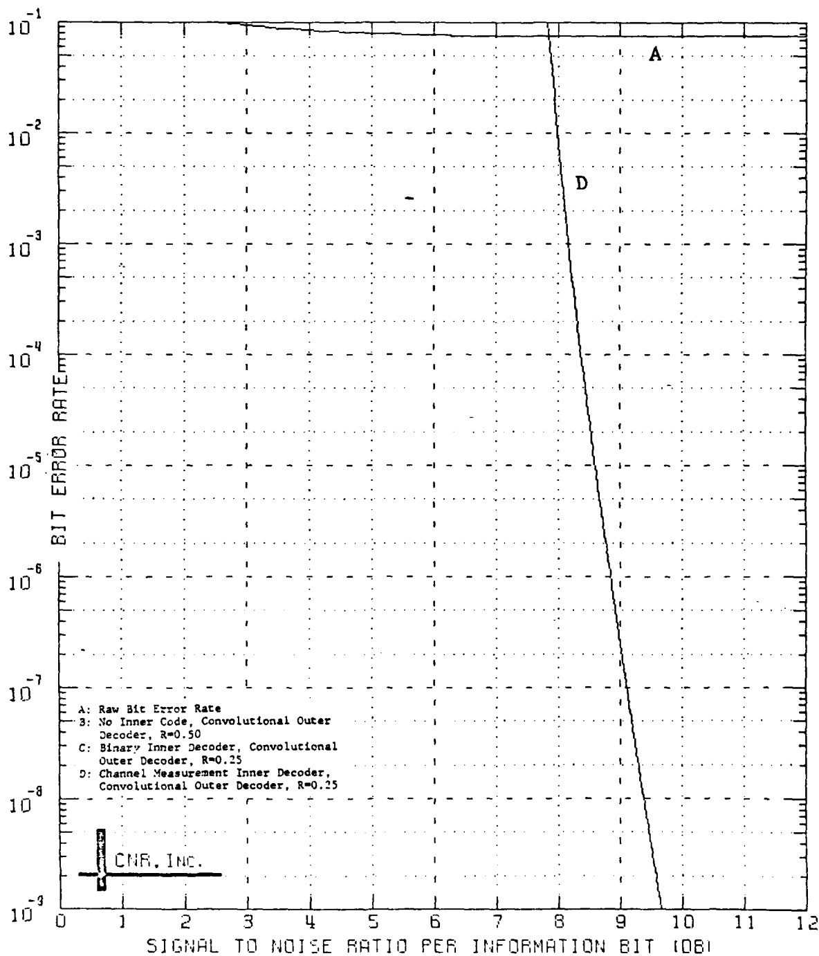
Figure 8.31 Decoded Performance of a Two-Stage Coding Approach Outer Decoder: Convolutional Code, Rate=1/2; K=7 Inner Decoder: Convolutional Code, Rate=1/2; K=7 \delta=0.15 and No Erasure Information Employed
