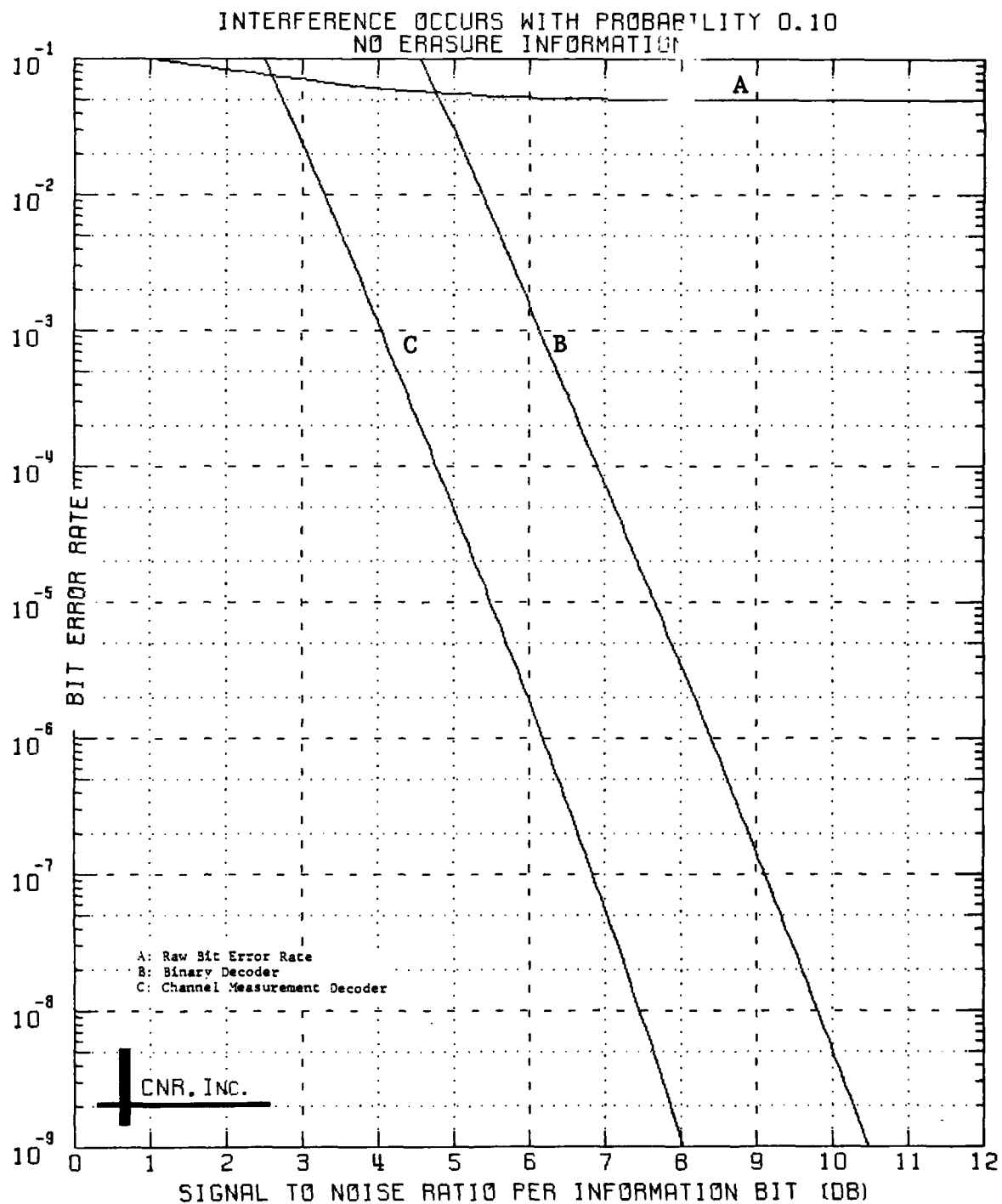
Figure 6.21 Decoded Performance of a Convolutional Code Rate 1/8; Constraint Length = 7
