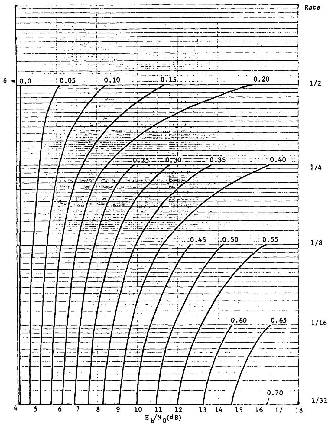
Figure 6.32 Convolutional Coding Performance with Interference Probability as a Parameter Channel Measurement Decoding-No Erasure Information
