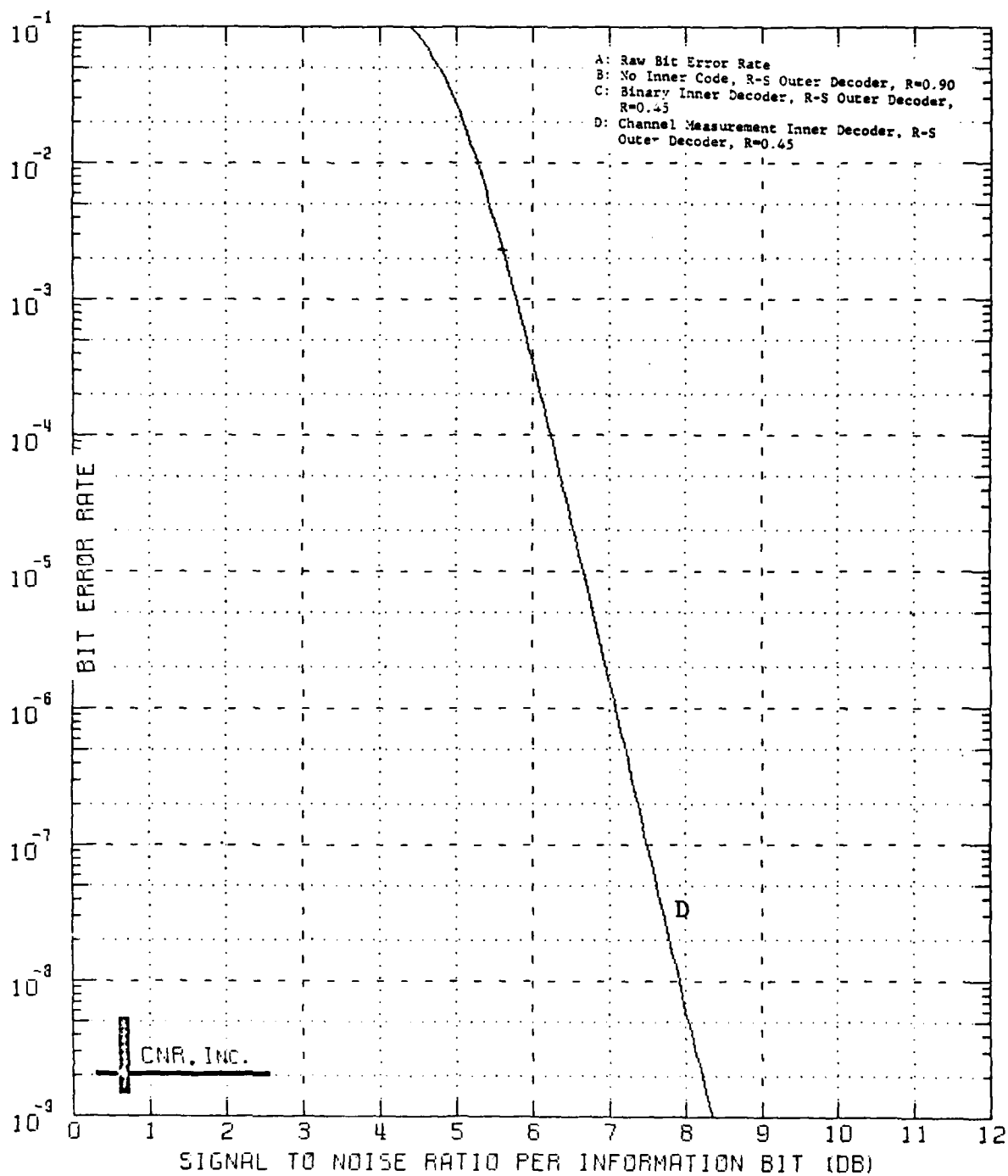
Figure 9.60 Decoded Performance of a Two-Stage Coding Approach Outer Decoder: Reed-Solomon Code (40,36;5) Bit Interleaver Employed Inner Decoder: Block Code (128,64;22) \delta=0.20 and No Erasure Information Employed
