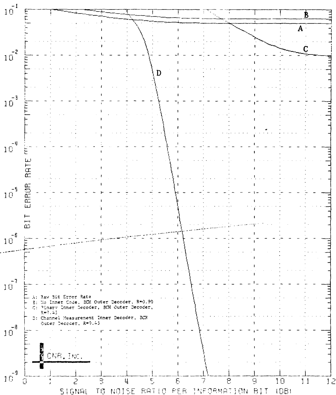
Figure 8.3 Decoded Performance of a Two-Stage Coding Approach Outer Decoder: BCH Code (240,216;7) Inner Decoder: Convolutional Code; Rate=1/2; K=7 \delta=0.10 and No Erasure Information Employed
