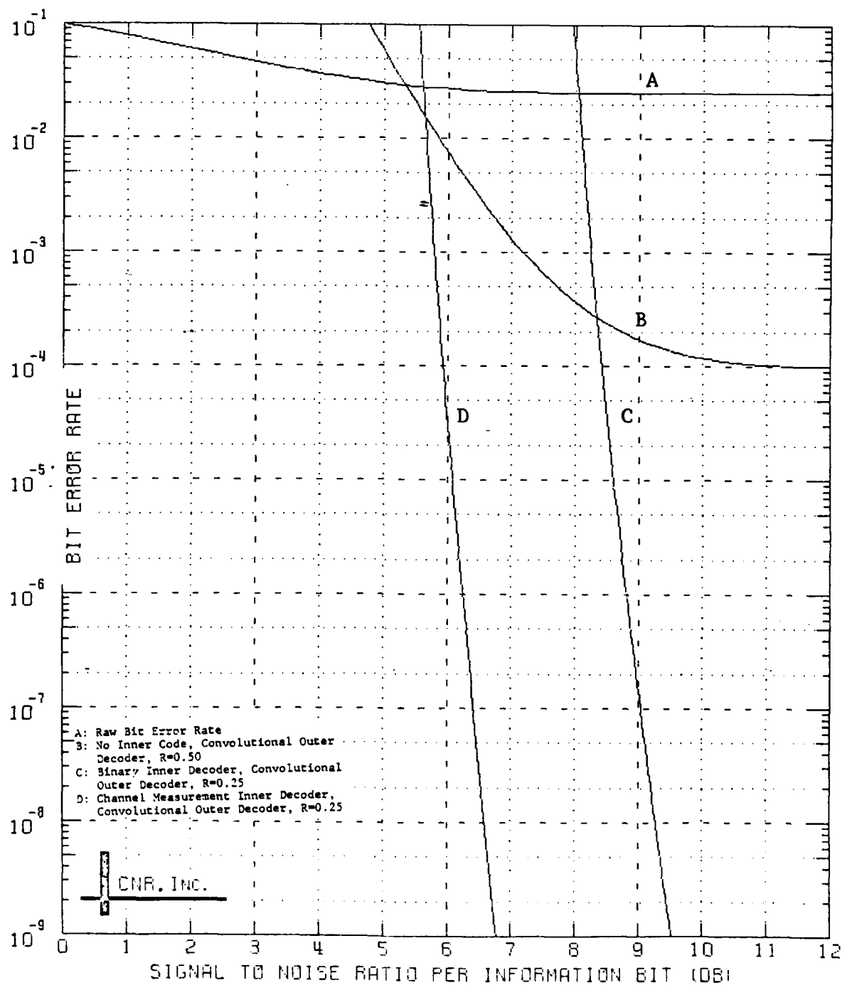
Figure 8.29 Decoded Performance of a Two-Stage Coding Approach Outer Decoder: Convolutional Code, Rate=1/2; K=7 Inner Decoder: Convolutional Code, Rate=1/2; K=7 \delta=0.05 and No Erasure Information Employed
