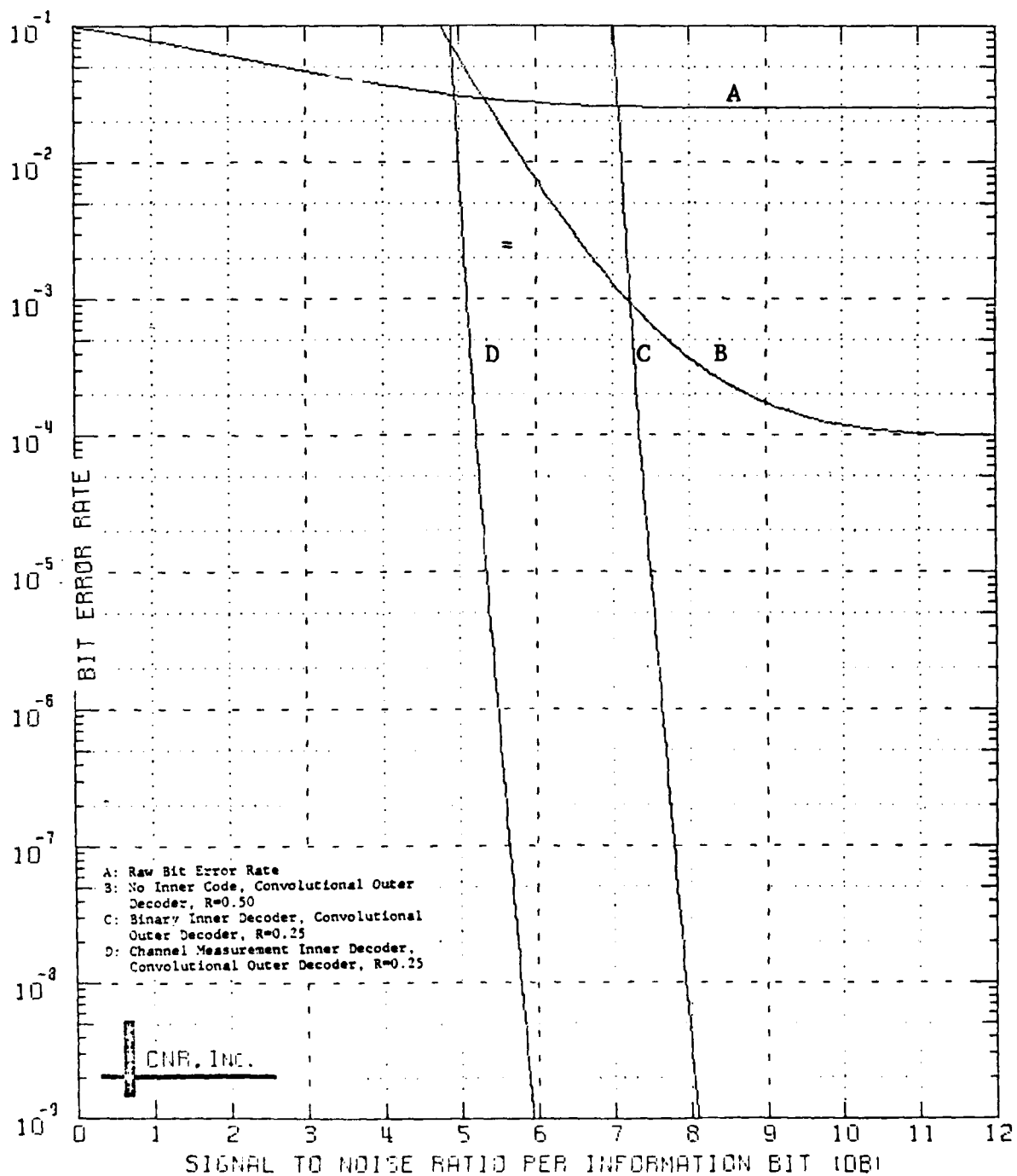
Figure 8.33 Decoded Performance of a Two-Stage Coding Approach Outer Decoder: Convolutional Code, Rate=1/2; K=7 Inner Decoder: Convolutional Code, Rate=1/2; K=7 \delta=0.05 and Erasure Information is Employed
