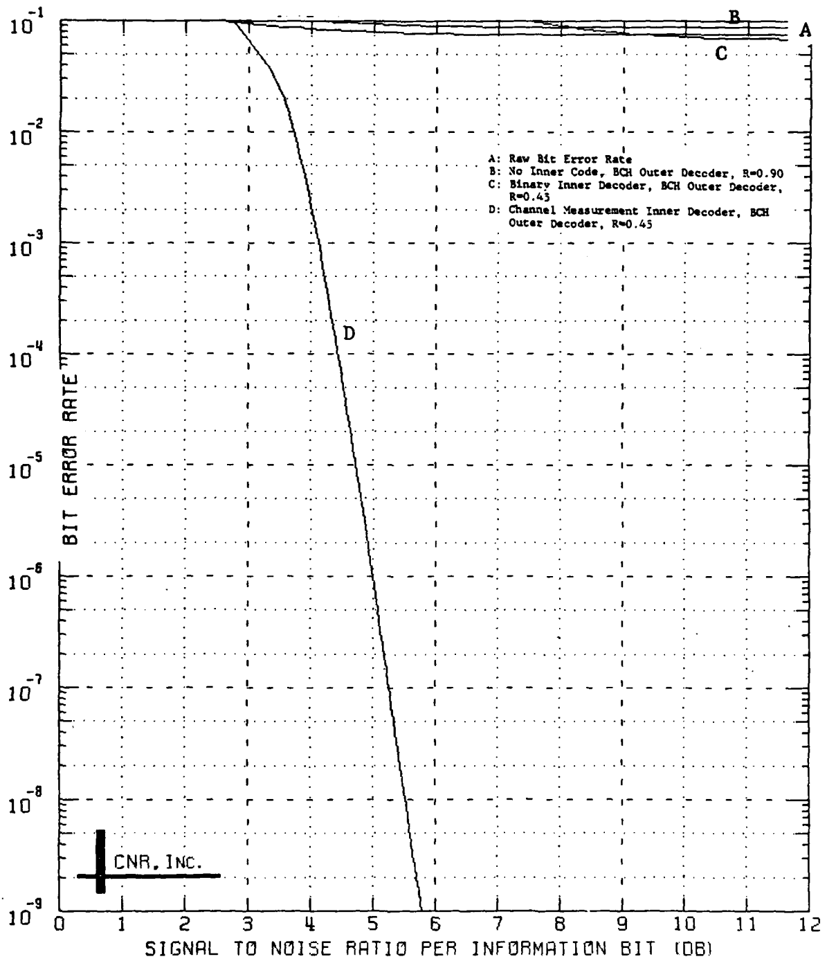
Figure 7.4 Decoded Performance of a Two-Stage Coding Approach Outer Decoder: BCH Code (240,216;7) Inner Decoder: Block Code (128,64;22) \delta=0.15 and No Erasure Information Employed
