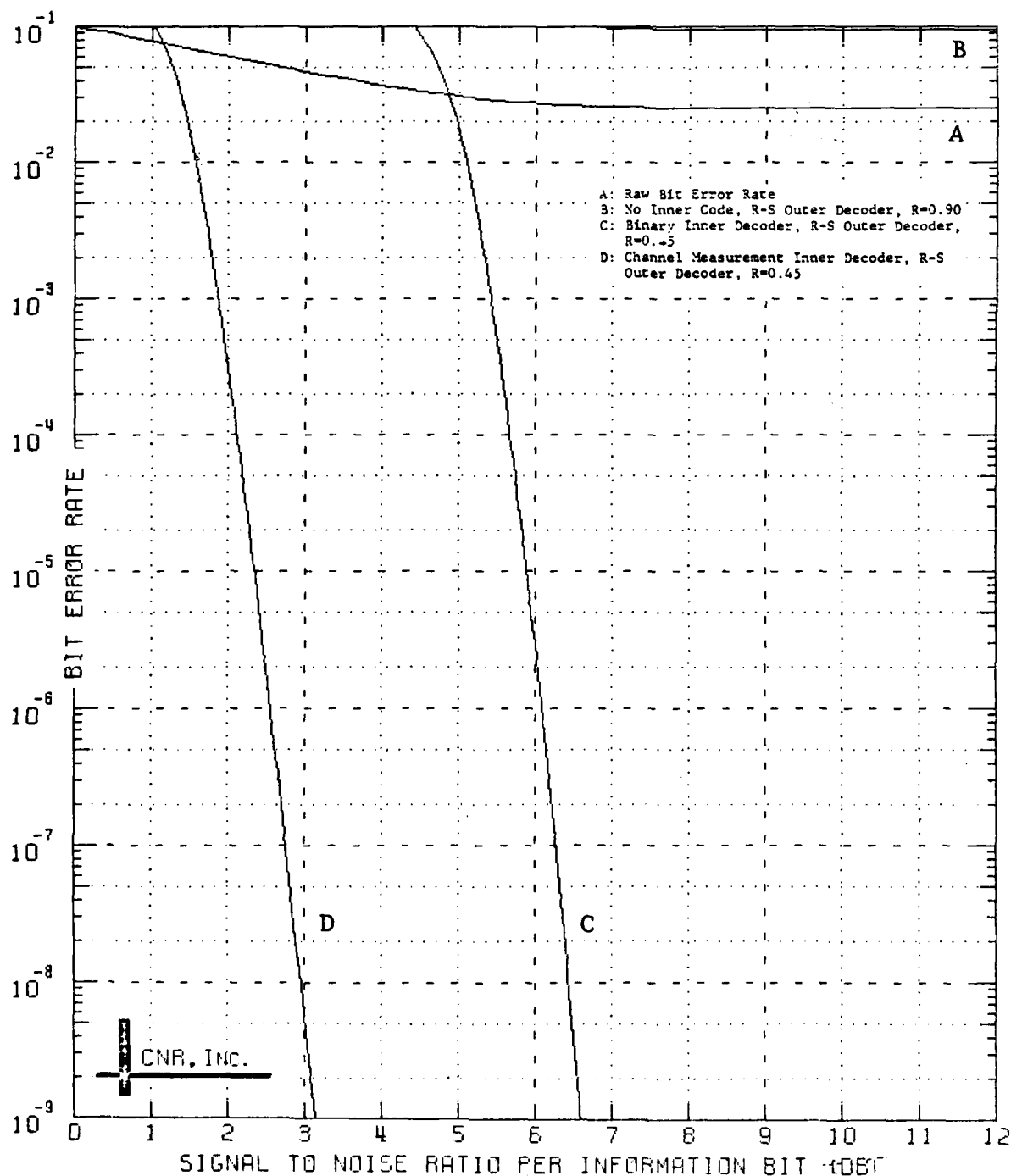
Figure 9.61 Decoded Performance of a Two-Stage Coding Approach Outer Decoder: Reed-Solomon Code (40,36;5) Bit Interleaver Employed Inner Decoder: Block Code (128,64;22) \delta=0.05 and Erasure Information is Employed
