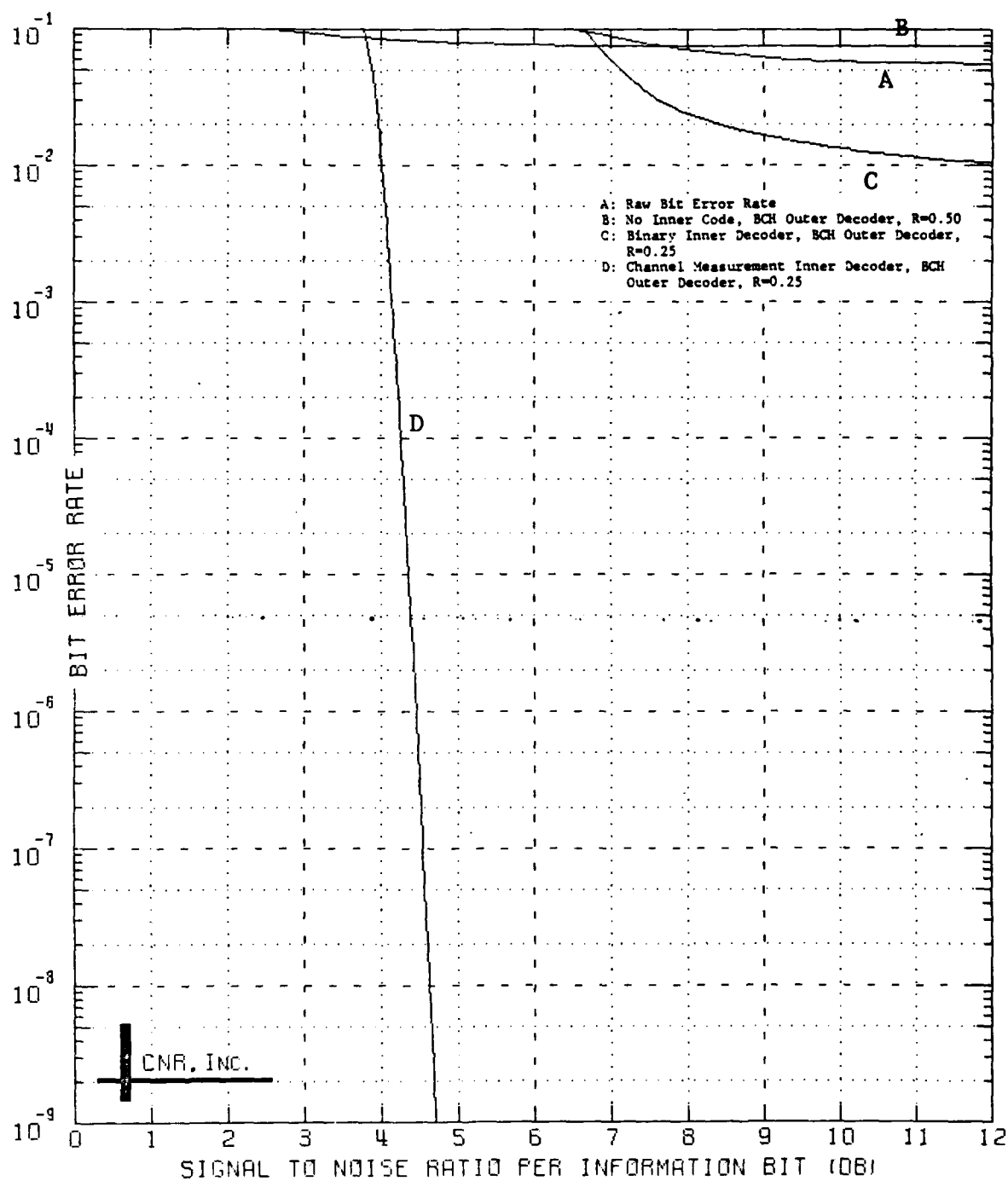
Figure 7.17 Decoded Performance of a Two-Stage Coding Approach Outer Decoder: BCH Code (128,64;22) Inner Decoder: Block Code (128,64;22) \delta=0.15 and Erasure Information is Employed
