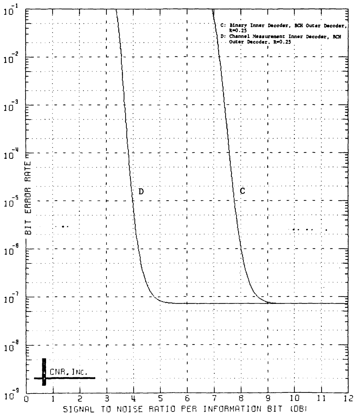
Figure 7.22 Decoded Performance of a Two-Stage Coding Approach Adaptive Technique Outer Decoder: BCH Code (128,64;22) Inner Decoder: Block Code (128,64;22) \delta=0.05 and No Erasure Information Employed
