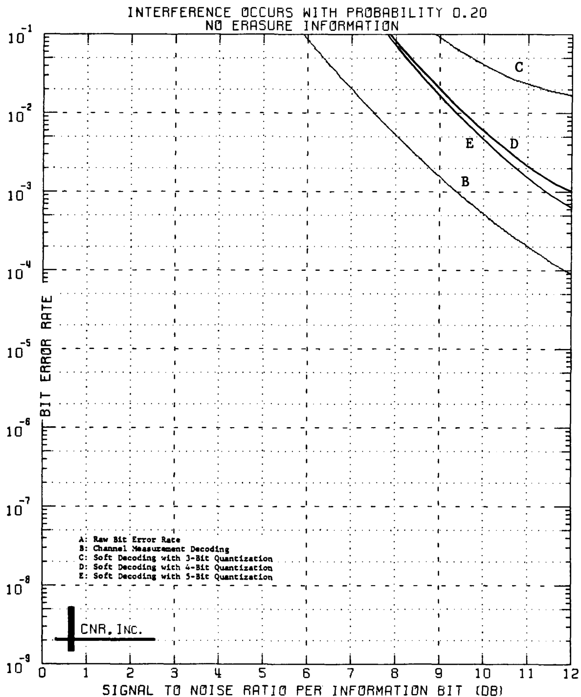
Figure 6 Decoded Performance of a Convolutional Code Rate 1/2; Constraint Length = 7; Gaussian Channel; CPSK Modulation
