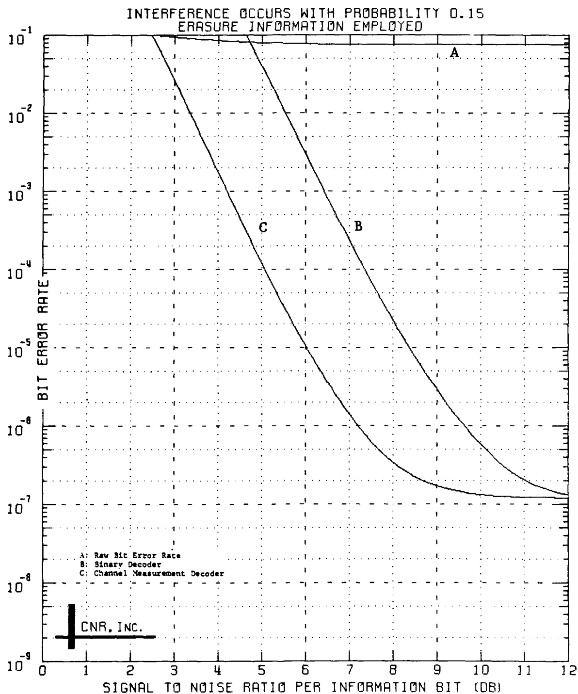
Figure 6.8 Decoded Performance of a Convolutional Code Rate 1/2; Constraint Length = 7
