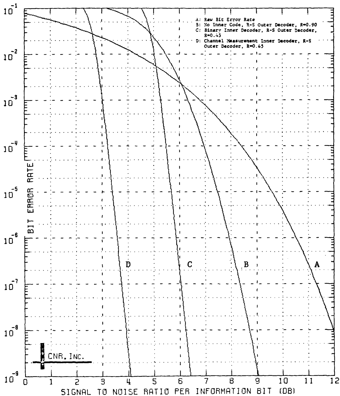
Figure 9.2 Decoded Performance of a Two-Stage Coding Approach Outer Decoder: Reed-Solomon Code (60,54;7) Bit Interleaver Employed Inner Decoder: Convolutional Code, Rate=1/2; K=7 \delta=0.00 and No Erasure Information Employed
