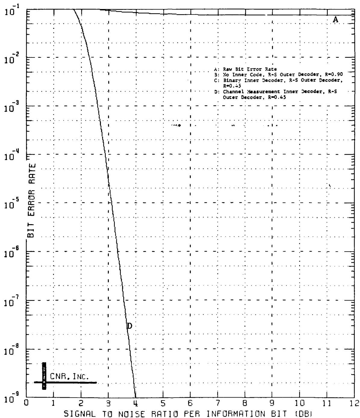
Figure 9.63 Decoded Performance of a Two-Stage Coding Approach Outer Decoder: Reed-Solomon Code (40,36;5) Bit Interleaver Employed Inner Decoder: Block Code (128,64;22) \delta=0.15 and Erasure Information is Employed
