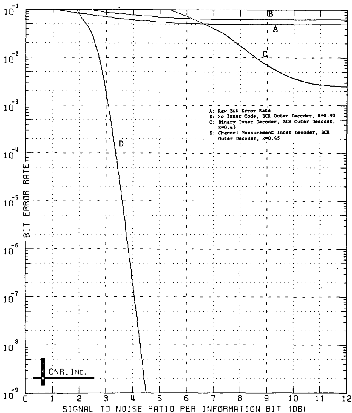
Figure 7.3 Decoded Performance of a Two-Stage Coding Approach Outer Decoder: BCH Code (240,216;7) Inner Decoder: Block Code (128,64;22) \delta=0.10 and No Erasure Information Employed
