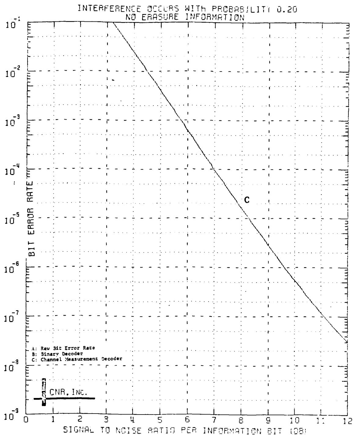
Figure 5.14 Decoded Performance of a Block Code Dimensions (128,64;22)
