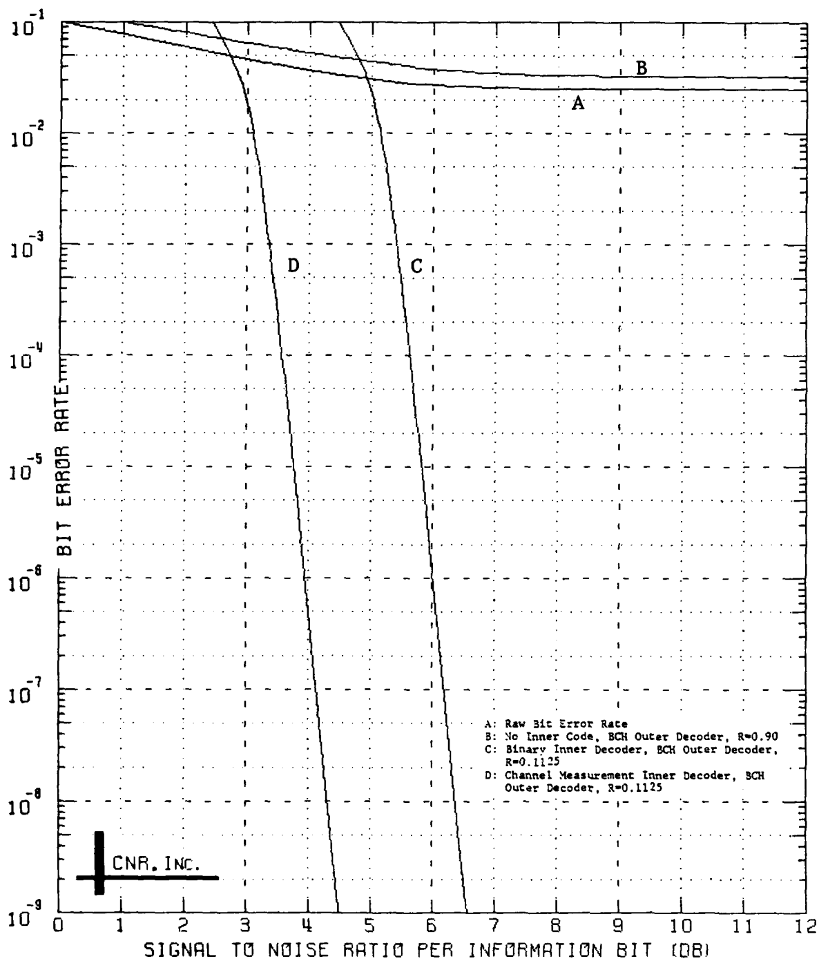
Figure 8.20 Decoded Performance of a Two-Stage Coding Approach Outer Decoder: BCH Code (240,216;7) Inner Decoder: Convolutional Code; Rate=1/8; K=7 \delta=0.05 and No Erasure Information Employed
