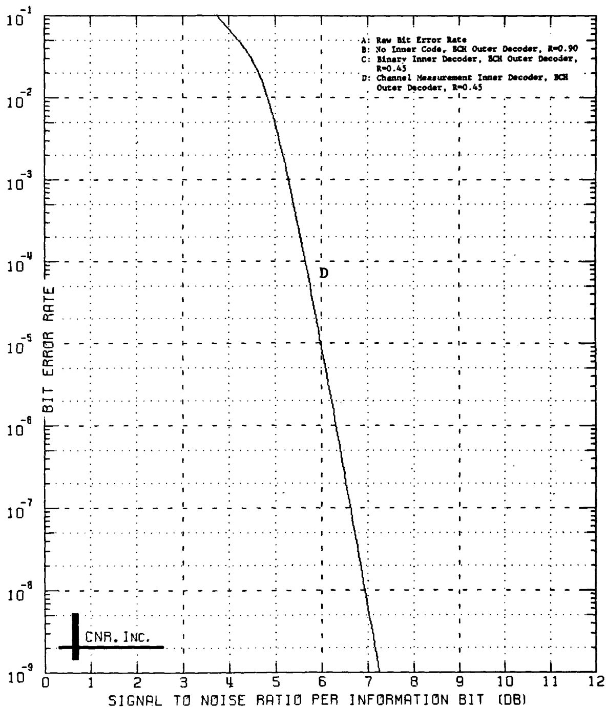
Figure 7.5 Decoded Performance of a Two-Stage Coding Approach Outer Decoder: BCH Code (240,216;7) Inner Decoder: Block Code (128,64;22) \delta=0.20 and No Erasure Information Employed
