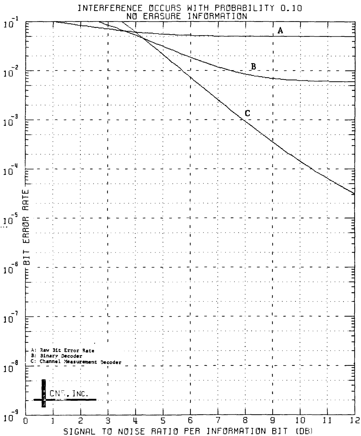
Figure 5.3 Decoded Performance of a Block Code Dimensions (24,12;8)
