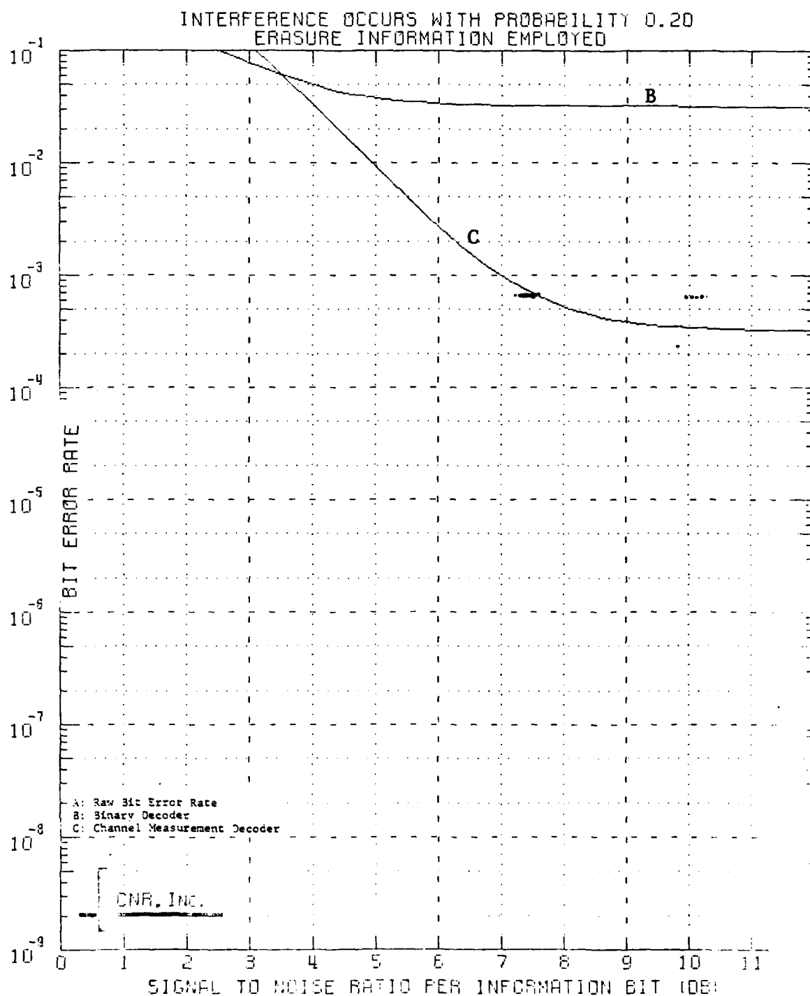
Figure 5.9 Decoded Performance of a Block Code Dimensions (24,12;8)
