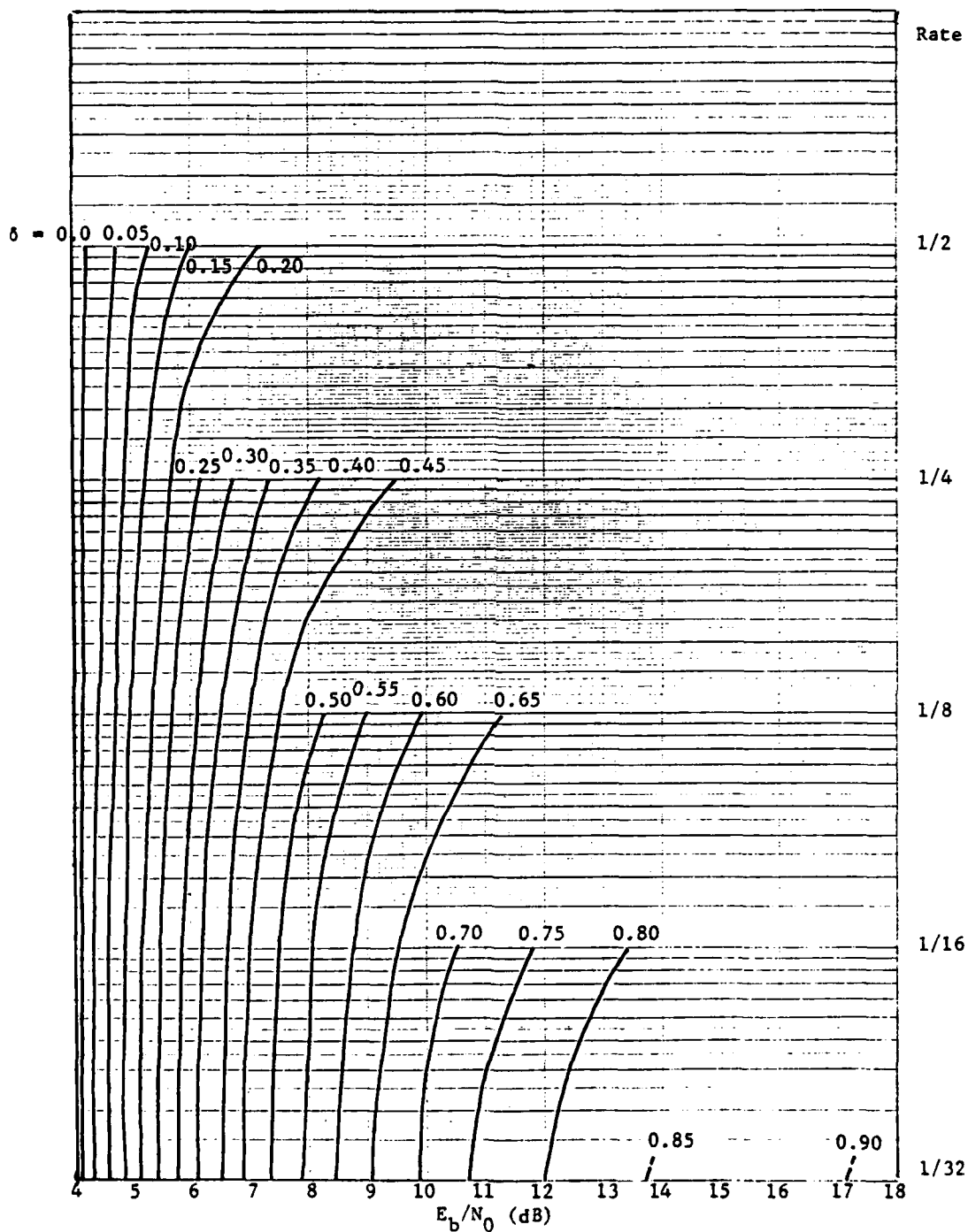
Figure 6.34 Convolutional Coding Performance with Interference Probability as a Parameter Channel Measurement Decoding-Erasurc Information Available
