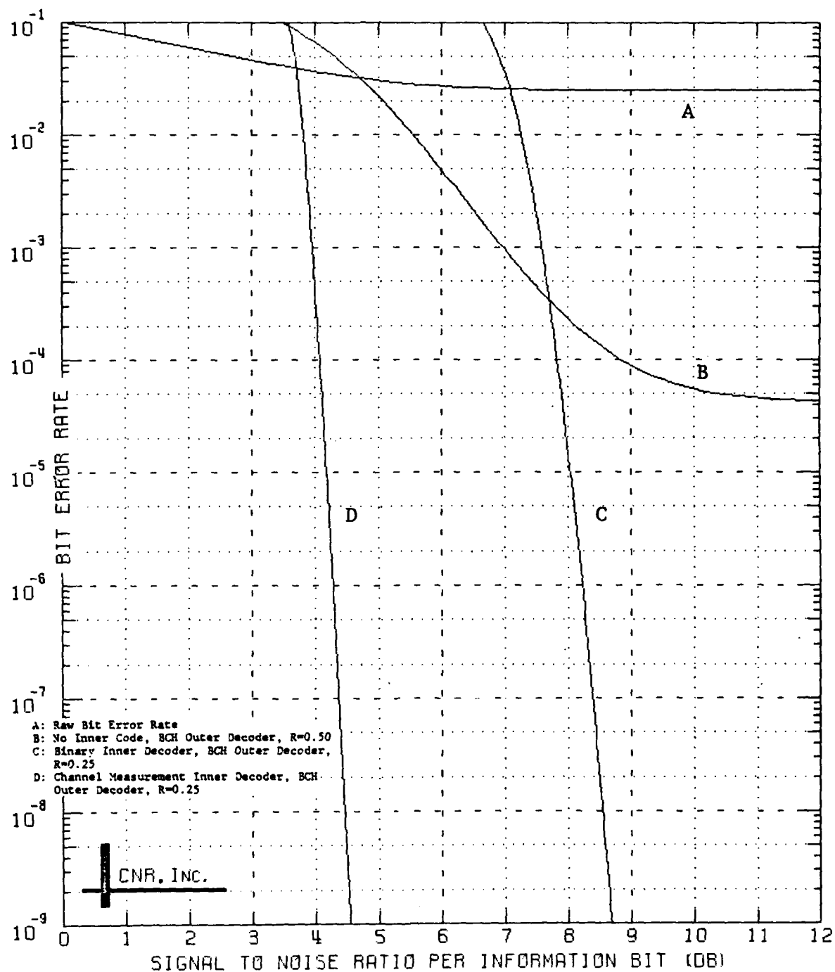
Figure 7.11 Decoded Performance of a Two-Stage Coding Approach Outer Decoder: BCH Code (128,64;22) Inner Decoder: Block Code (128,64;22) \delta=0.05 and No Erasure Information Employed
