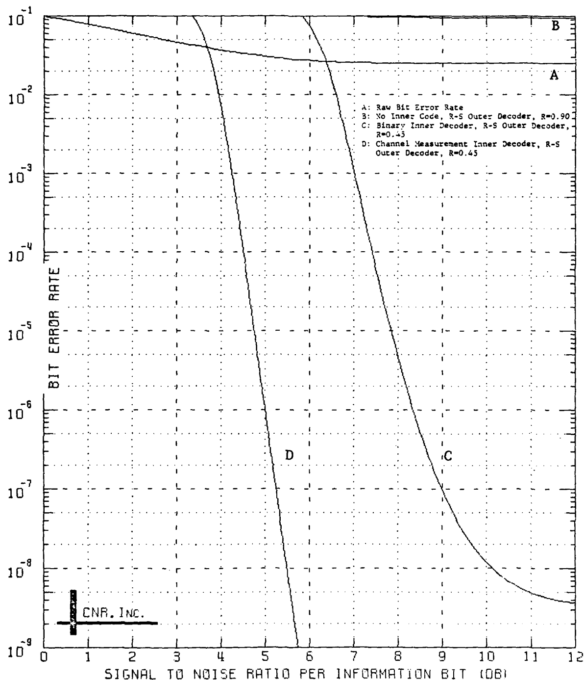
Figure 9.3 Decoded Performance of a Two-Stage Coding Approach Outer Decoder: Reed-Solomon Code (60,54;7) Bit Interleaver Employed Inner Decoder: Convolutional Code, Rate=1/2; K=7 \delta=0.05 and No Erasure Information Employed
