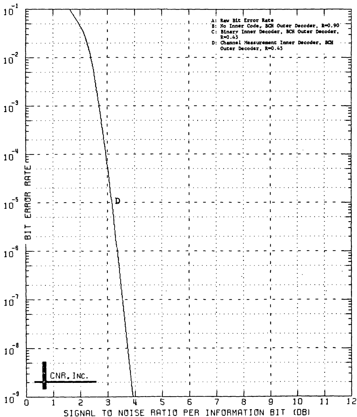
Figure 7.9 Decoded Performance of a Two-Stage Coding Approach Outer Decoder: BCH Code (240,216;7) Inner Decoder: Block Code (128,64;22) \delta=0.20 and Erasure Information is Employed
