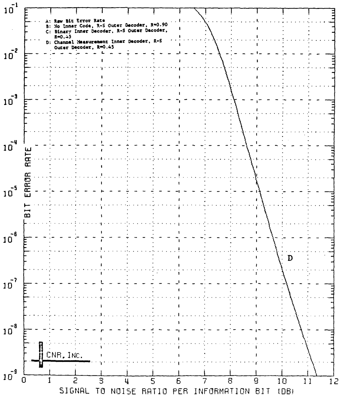
Figure 9.15 Decoded Performance of a Two-Stage Coding Approach Outer Decoder: Reed-Solomon Code (60,54;7) Symbol Interleaver Employed Inner Decoder: Convolutional Code, Rate=1/2; K=7 \delta=0.20 and No Erasure Information Employed
