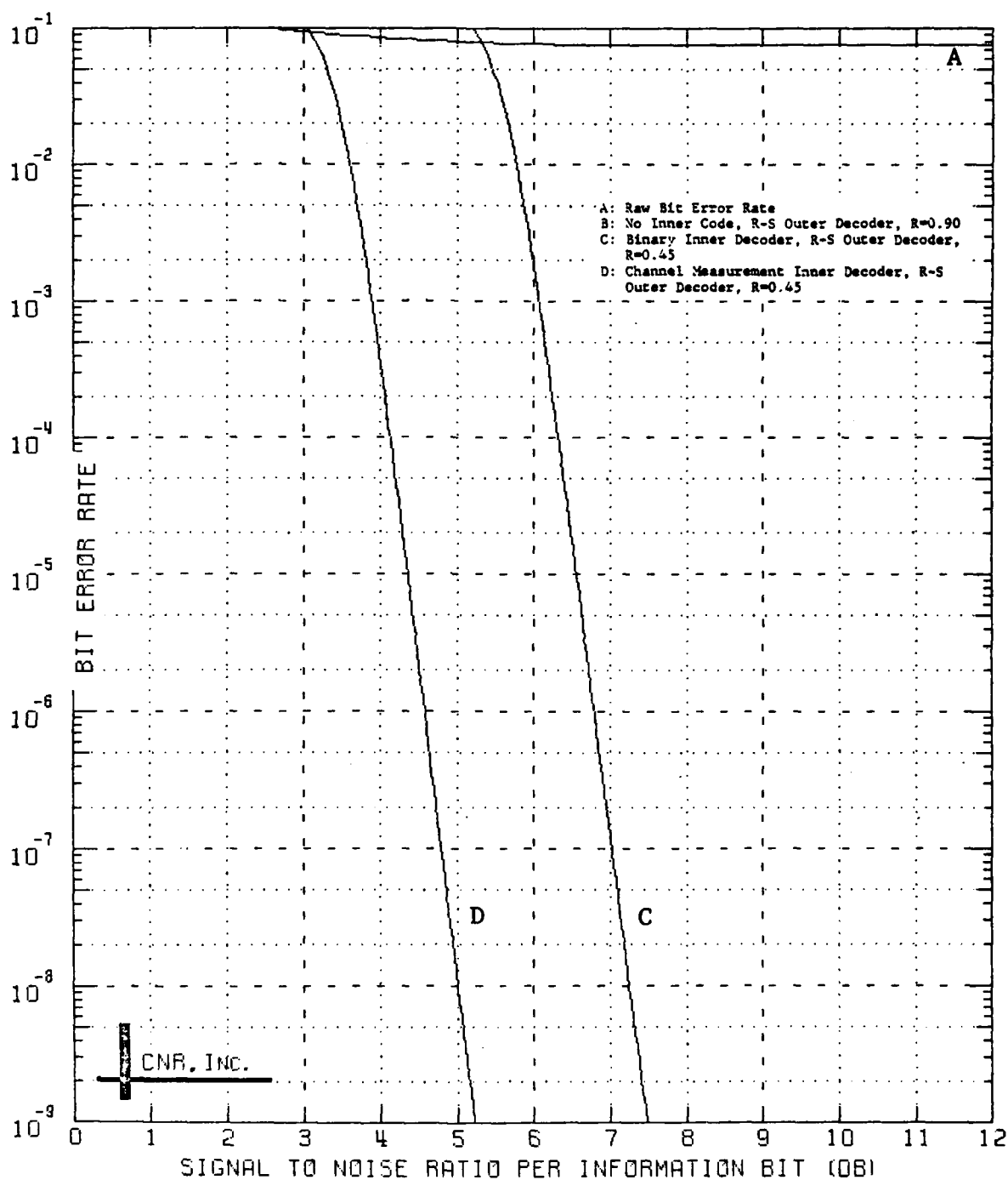
Figure 9.18 Decoded Performance of a Two-Stage Coding Approach Outer Decoder: Reed-Solomon Code (60,54;7) Symbol Interleaver Employed Inner Decoder: Convolutional Code, Rate=1/2; K=7 \delta=0.15 and Erasure Information is Employed
