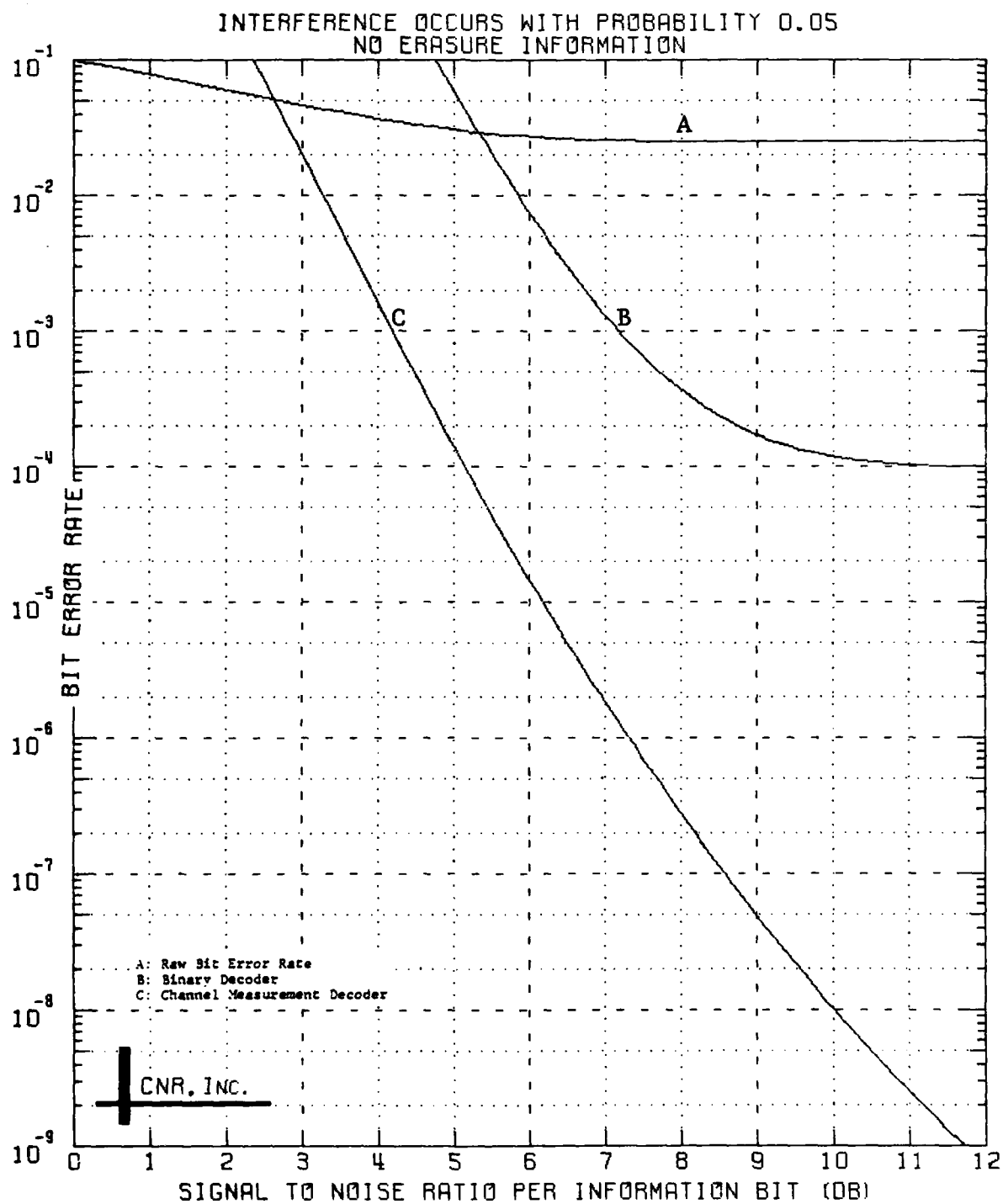
Figure 6.2 Decoded Performance of a Convolutional Code Rate 1/2; Constraint Length = 7
