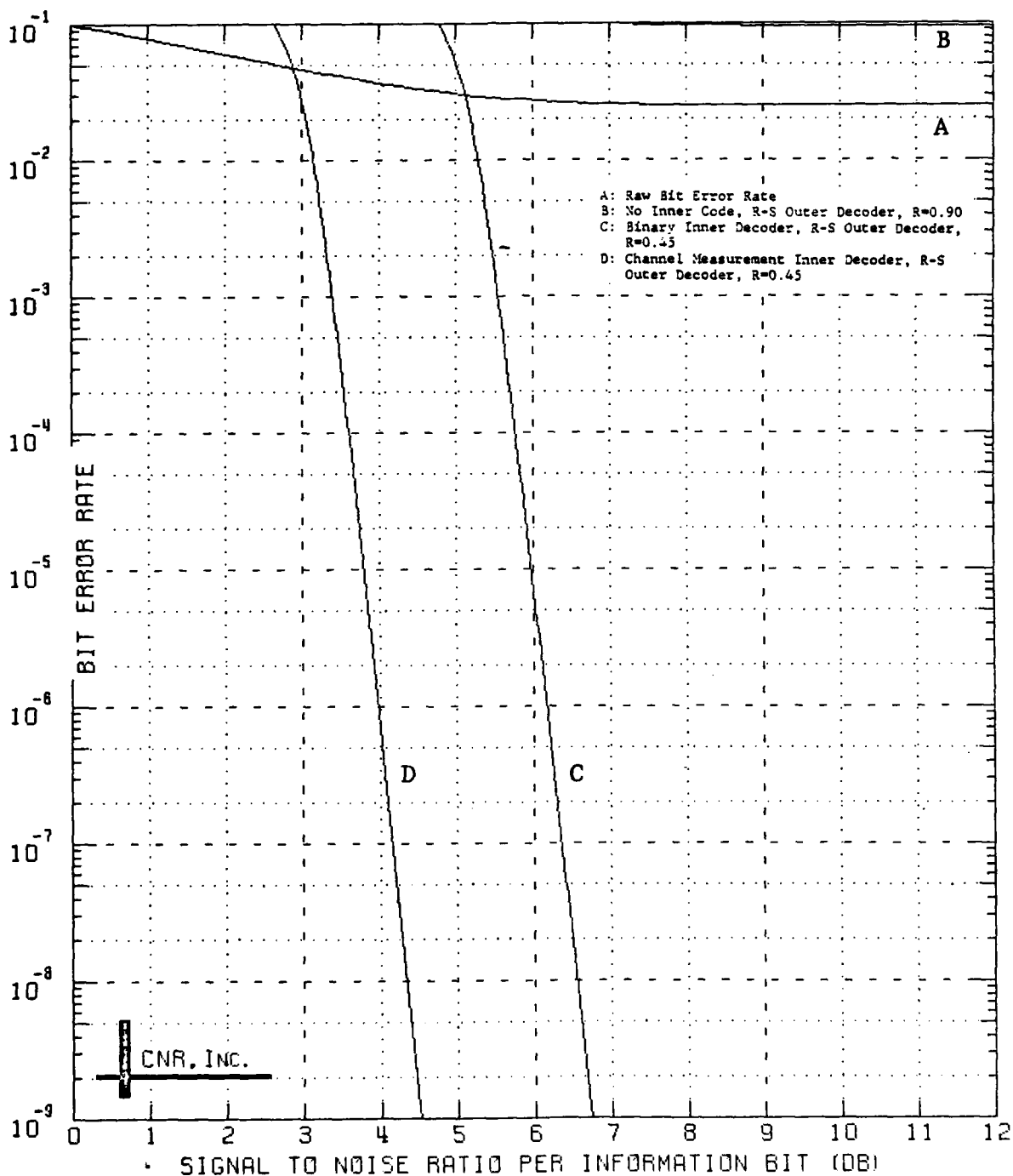
Figure 9.7 Decoded Performance of a Two-Stage Coding Approach Outer Decoder: Reed-Solomon Code (60,54;7) Bit Interleaver Employed Inner Decoder: Convolutional Code, Rate=1/2; K=7 \delta=0.05 and Erasure Information is Employed
