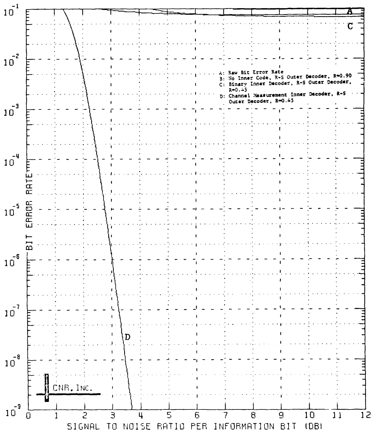
Figure 9.72 Decoded Performance of a Two-Stage Coding Approach Outer Decoder: Reed-Solomon Code (40,36;5) Symbol Interleaver Employed Inner Decoder: Block Code (128,64;22) \delta=0.15 and Erasure Information is Employed
