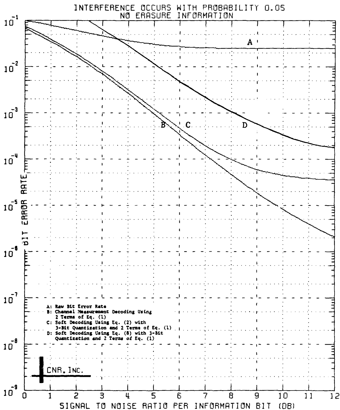
Figure 12 Decoded Performance of a Convolutional Code Rate 1/2; Constraint Length = 3; Gaussian Channel; CPSK Modulation
