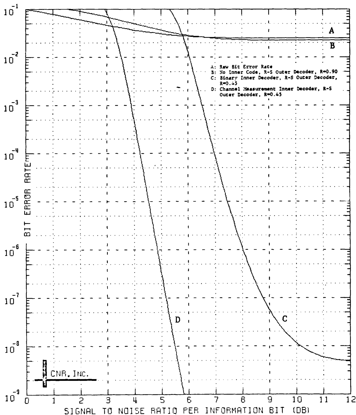
Figure 9.30 Decoded Performance of a Two-Stage Coding Approach Outer Decoder: Reed-Solomon Code (40,36;5) Symbol Interleaver Employed Inner Decoder: Convolutional Code, Rate=1/2; K=7 \delta=0.05 and No Erasure Information Employed
