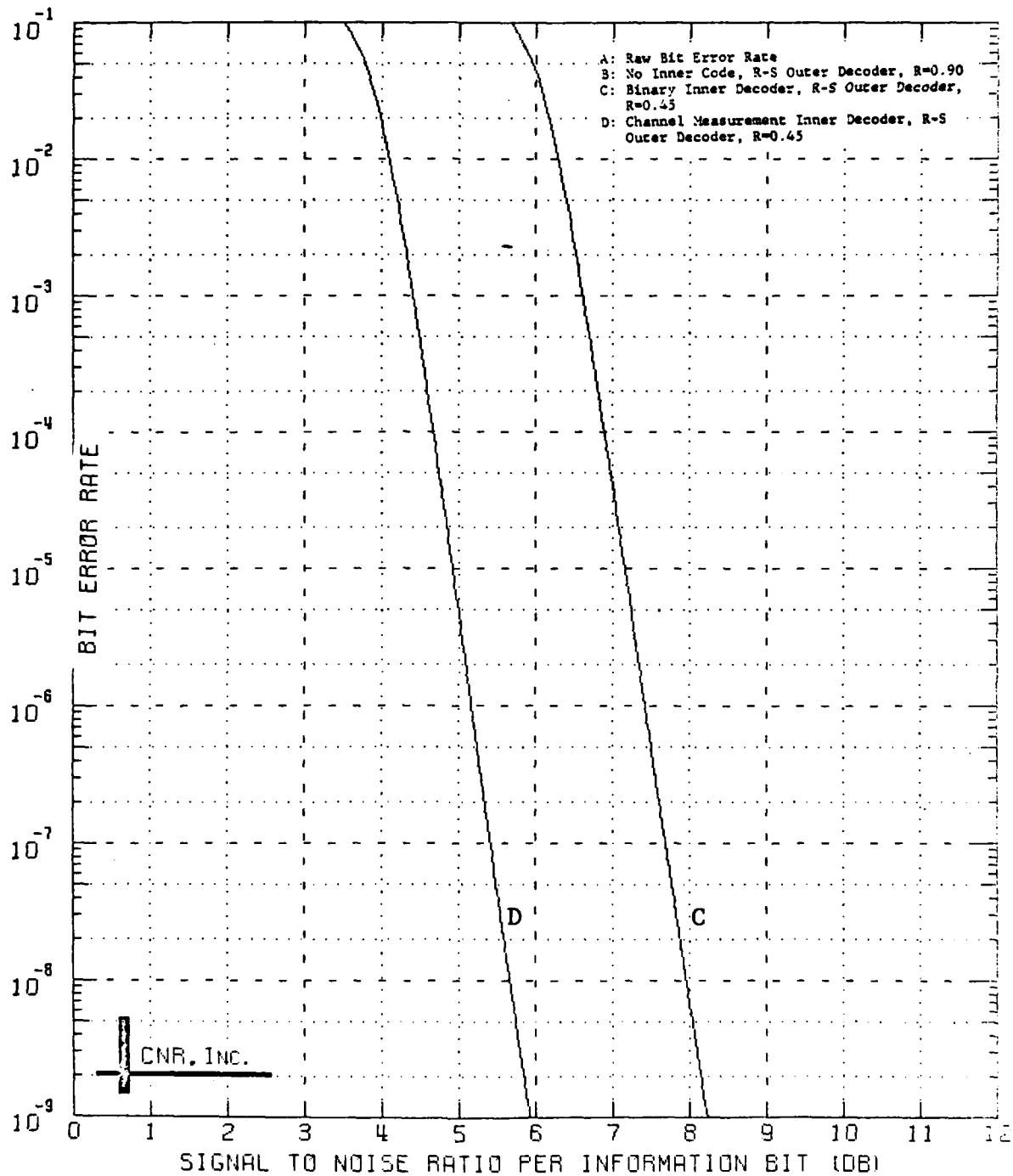
Figure 9.19 Decoded Performance of a Two-Stage Coding Approach Outer Decoder: Reed-Solomon Code (60,54;7) Symbol Interleaver Employed Inner Decoder: Convolutional Code, Rate=1/2; K=7 \delta=0.20 and Erasure Information is Employed
