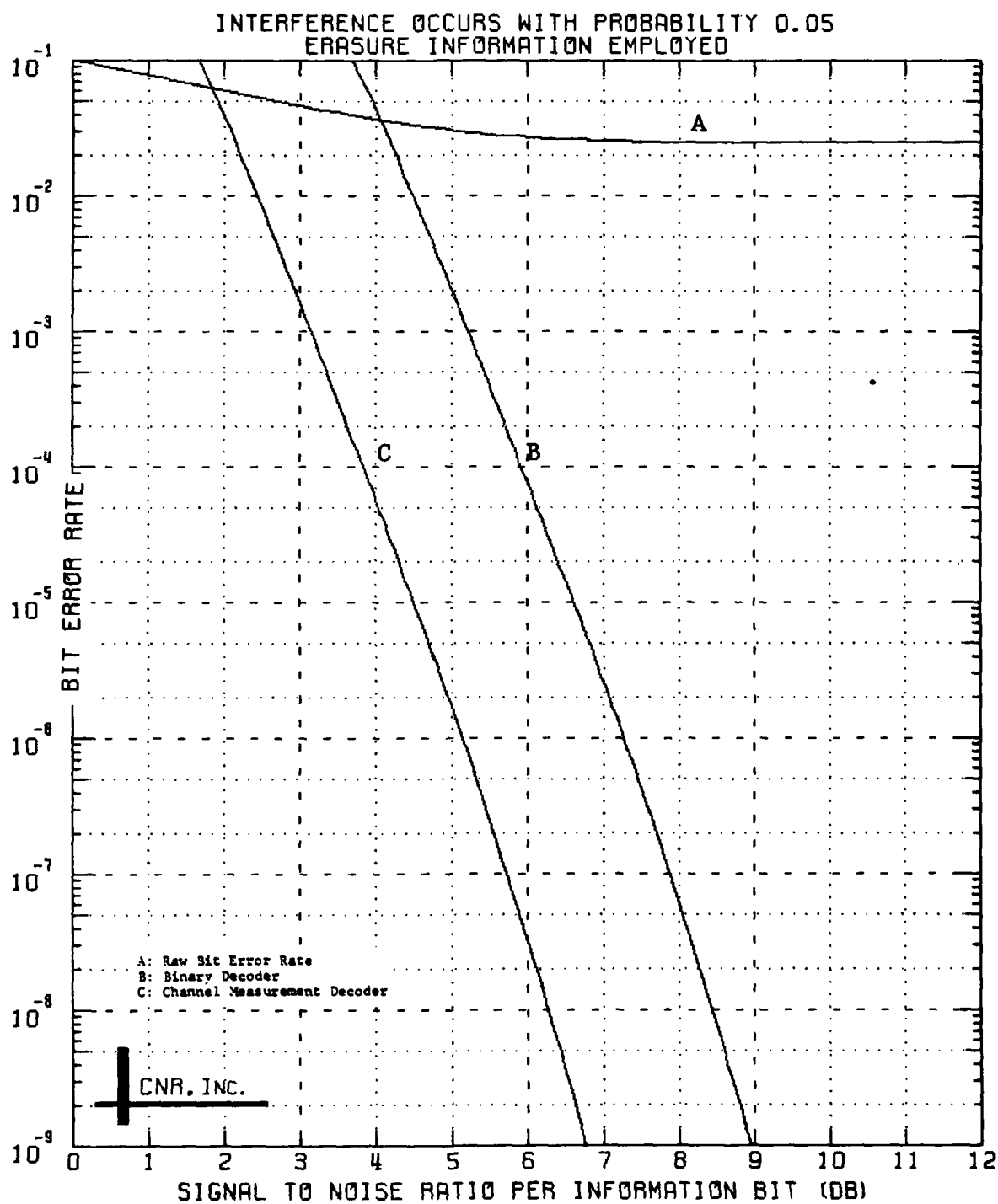
Figure 6.15 Decoded Performance of a Convolutional Code Rate 1/4; Constraint Length = 7
