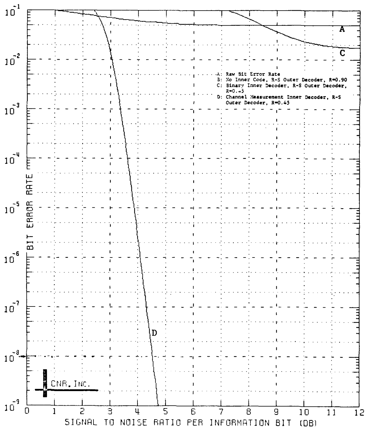
Figure 9.40 Decoded Performance of a Two-Stage Coding Approach Outer Decoder: Reed-Solomon Code (60,54;7) Bit Interleaver Employed Inner Decoder: Block Code (128,64;22) \delta=0.10 and No Erasure Information Employed
