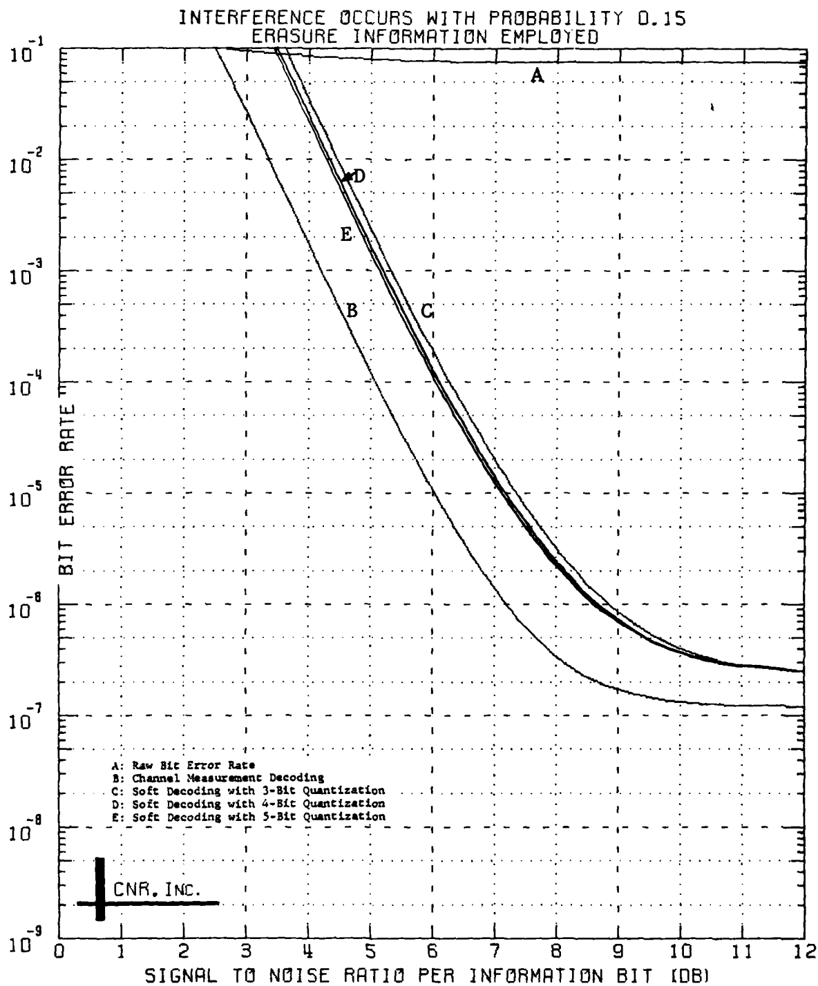
Figure 9 Decoded Performance of a Convolutional Code Rate 1/2; Constraint Length = 7; Gaussian Channel; CPSK Modulation
