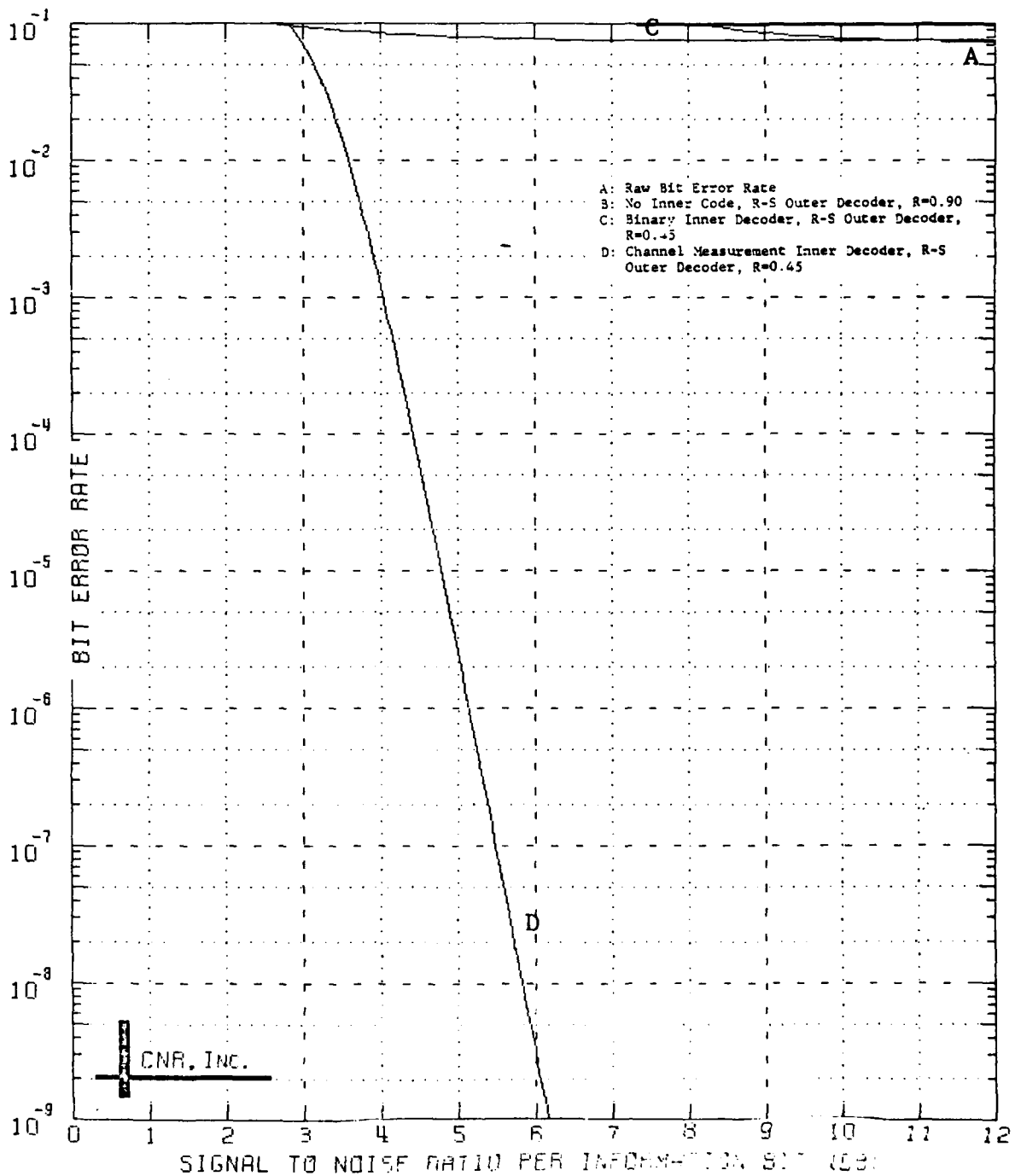
Figure 9.68 Decoded Performance of a Two-Stage Coding Approach Outer Decoder: Reed-Solomon Code (40,36;5) Symbol Interleaver Employed Inner Decoder: Block Code (128,64;22) \delta=0.15 and No Erasure Information Employed
