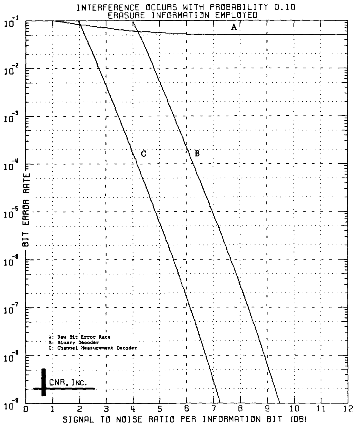
Figure 6.16 Decoded Performance of a Convolutional Code Rate 1/4; Constraint Length = 7
