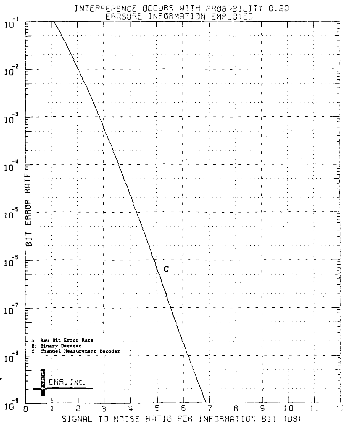
Figure 5.18 Decoded Performance of a Block Code Dimensions (128,64;22)
