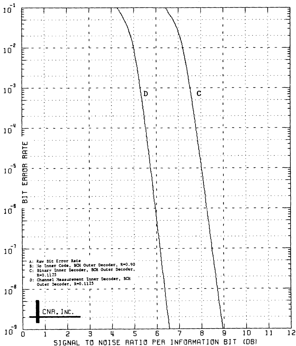
Figure 8.23 Decoded Performance of a Two-Stage Coding Approach Outer Decoder: BCH Code (240,216;7) Inner Decoder: Convolutional Code; Rate=1/8; K=7 \delta=0.20 and No Erasure Information Employed
