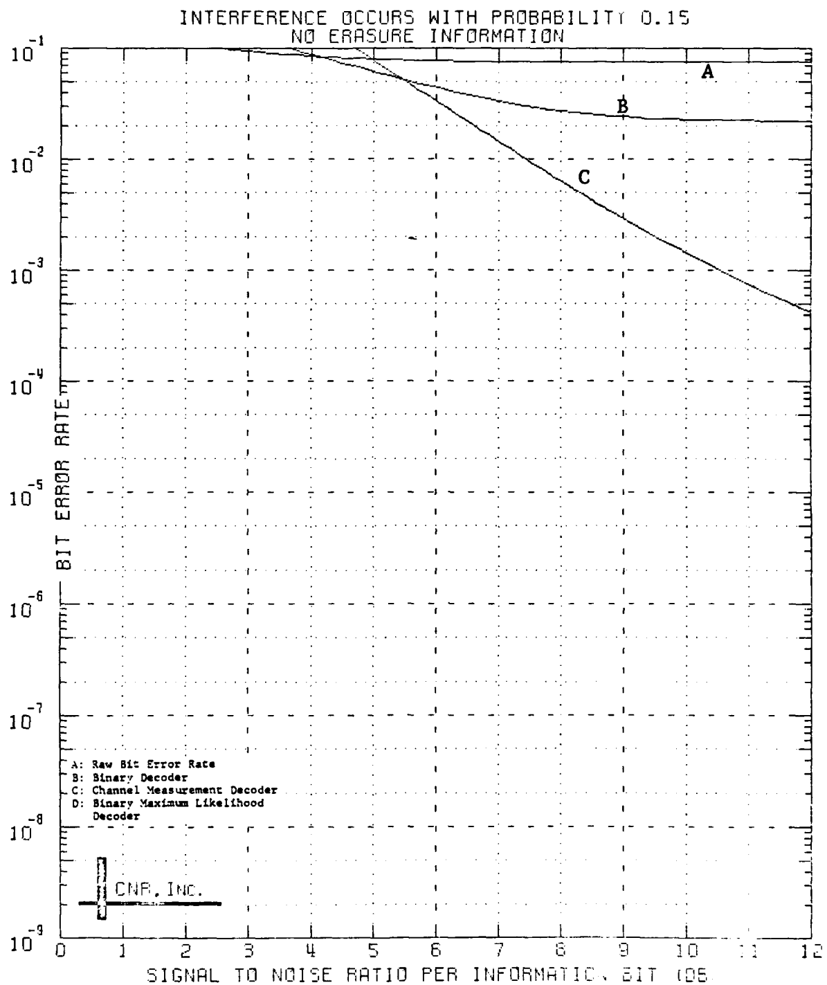
Figure 5.22 Decoded Performance of a Block Code Dimensions (24,12;8)
