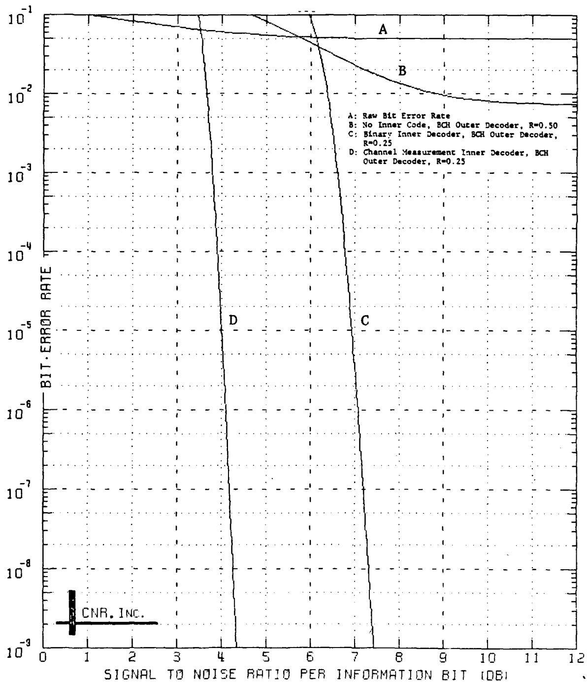
Figure 7.16 Decoded Performance of a Two-Stage Coding Approach Outer Decoder: BCH Code (128,64;22) Inner Decoder: Block Code (128,64;22) \delta=0.10 and Erasure Information is Employed
