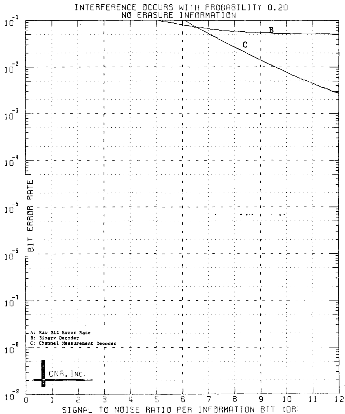
Figure 5.5 Decoded Performance of a Block Code Dimensions (24,12;8)
