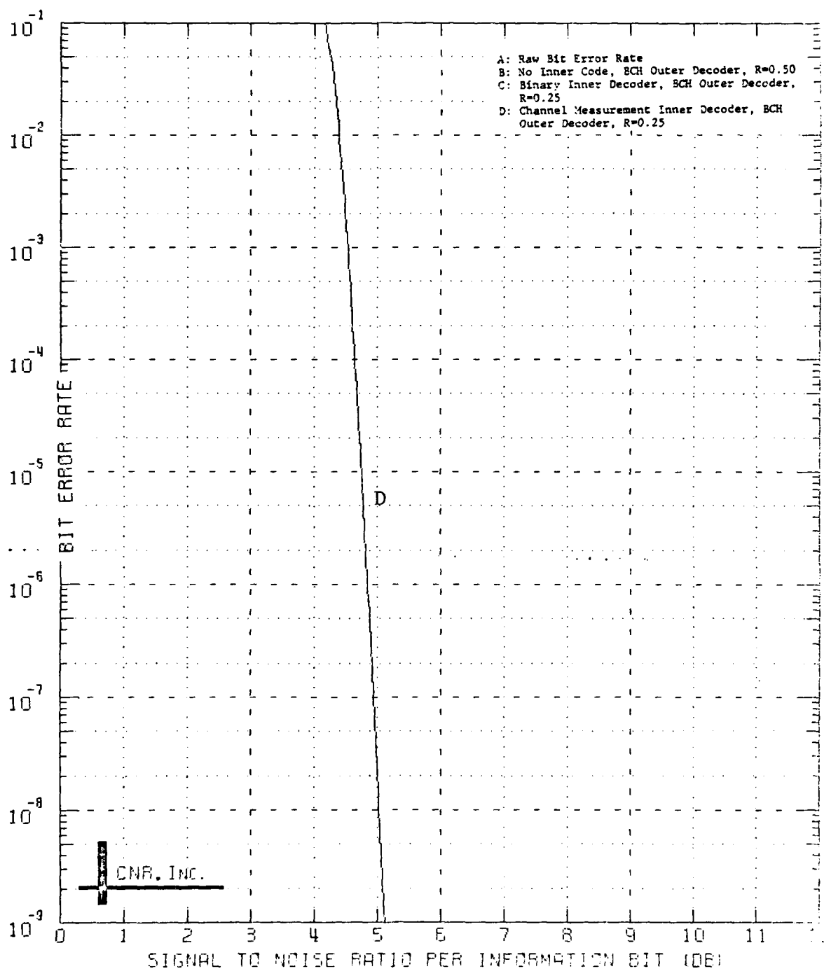
Figure 7.18 Decoded Performance of a Two-Stage Coding Approach Outer Decoder: BCH Code (128,64;22) Inner Decoder: Block Code (128,64;22) \delta=0.20 and Erasure Information is Employed
