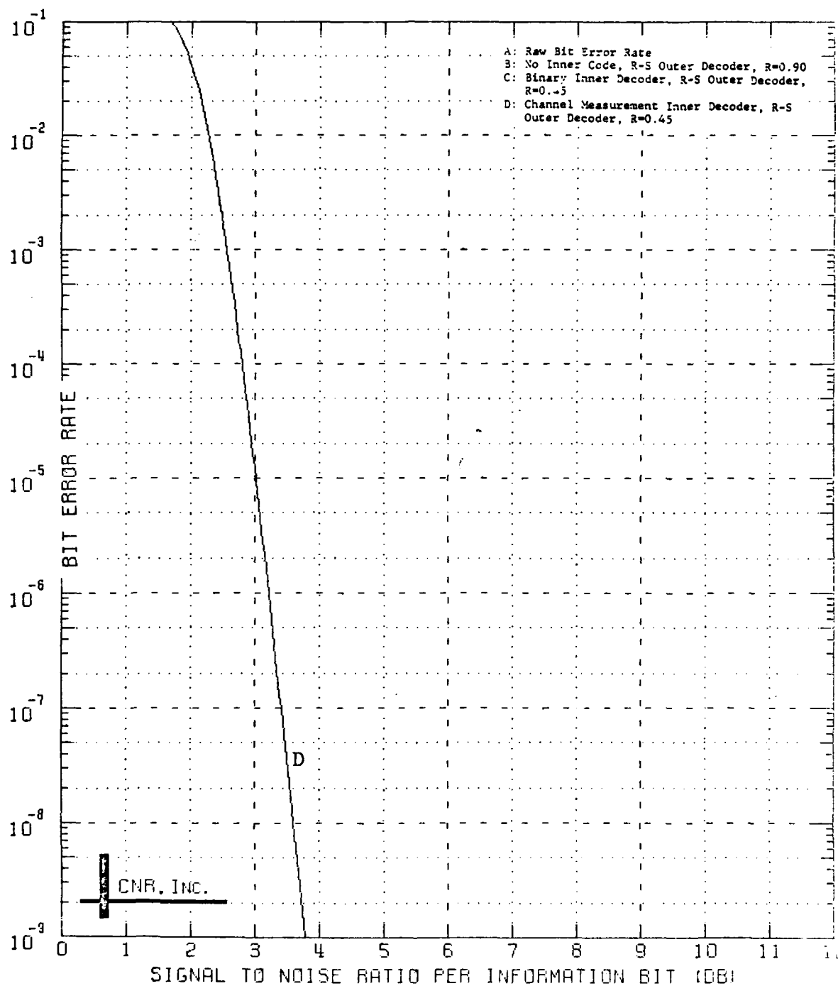
Figure 9.55 Decoded Performance of a Two-Stage Coding Approach Outer Decoder: Reed-Solomon Code (60,54;7) Symbol Interleaver Employed Inner Decoder: Block Code (128,64;22) \delta=0.20 and Erasure Information is Employed
