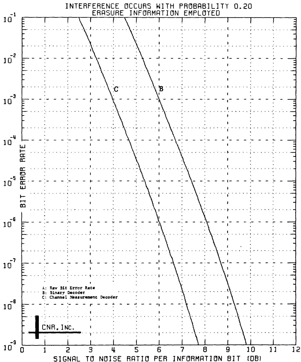
Figure 6.27 Decoded Performance of a Convolutional Code Rate 1/8; Constraint Length = 7
