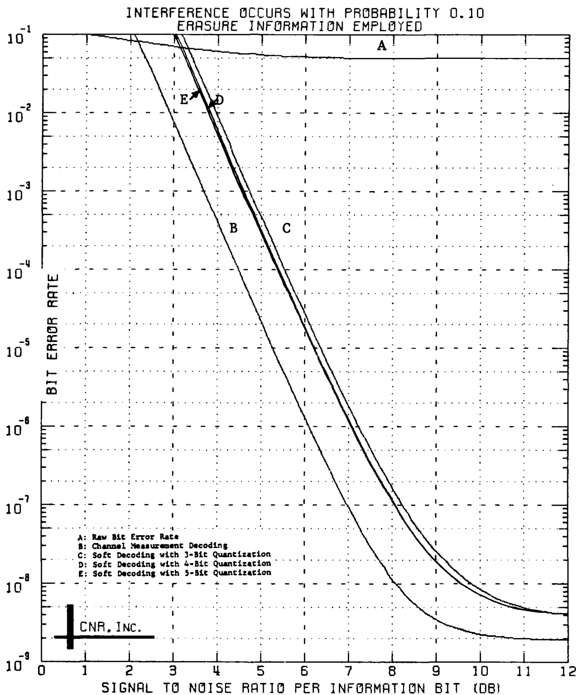
Figure 8 Decoded Performance of a Convolutional Code Rate 1/2; Constraint Length = 7; Gaussian Channel; CPSK Modulation
