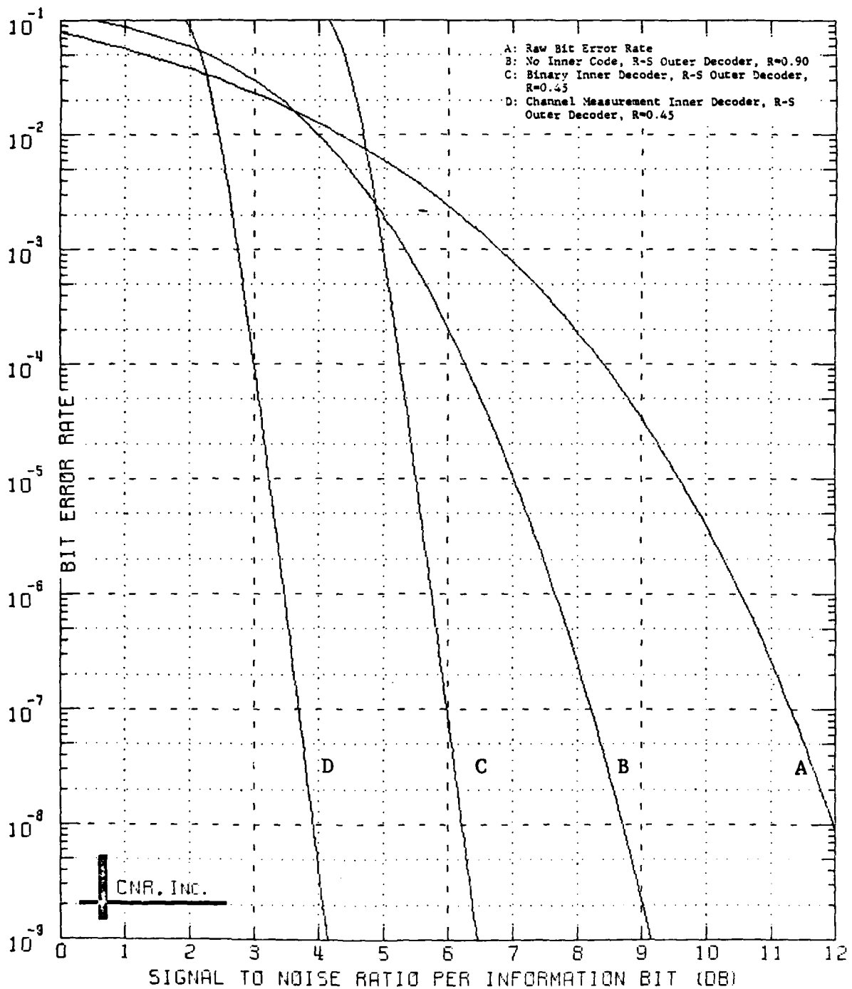
Figure 9.29 Decoded Performance of a Two-Stage Coding Approach Outer Decoder: Reed-Solomon Code (40,36;5) Symbol Interleaver Employed Inner Decoder: Convolutional Code, Rate=1/2; K=7 \delta=0.00 and No Erasure Information Employed
