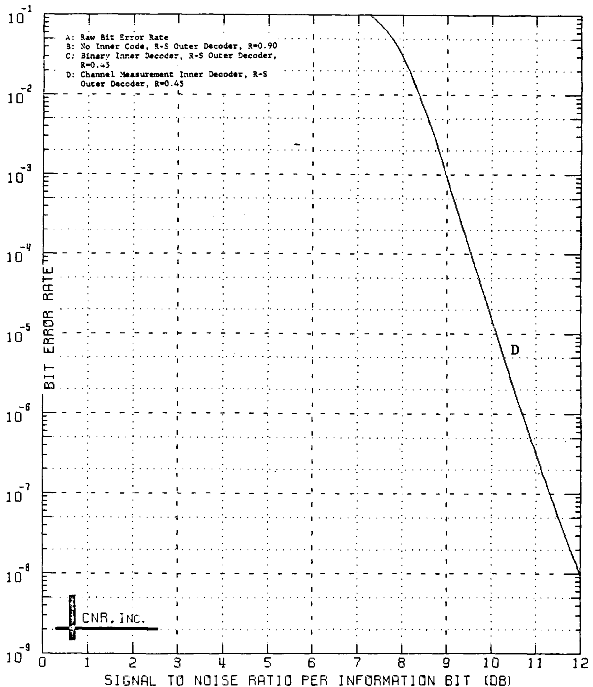
Figure 9.6 Decoded Performance of a Two-Stage Coding Approach Outer Decoder: Reed-Solomon Code (60,54;7) Bit Interleaver Employed Inner Decoder: Convolutional Code, Rate=1/2; K=7 \delta=0.20 and No Erasure Information Employed
