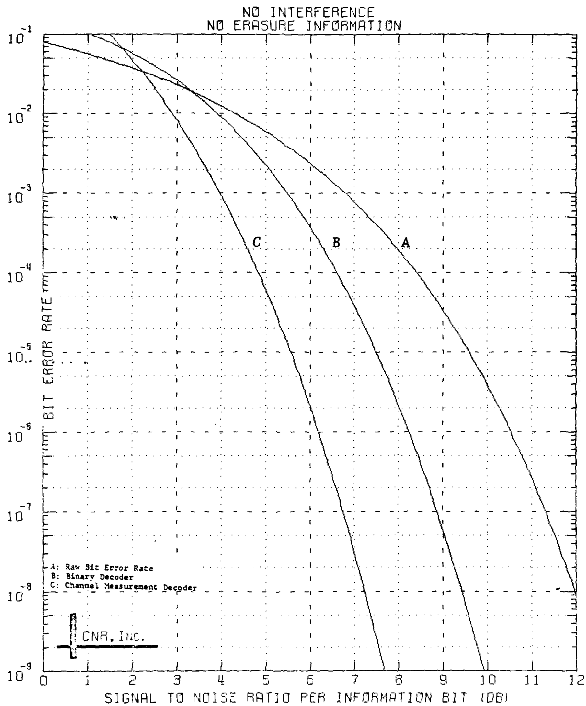
Figure 5.1 Decoded Performance of a Block Code Dimensions (24,12;8)
