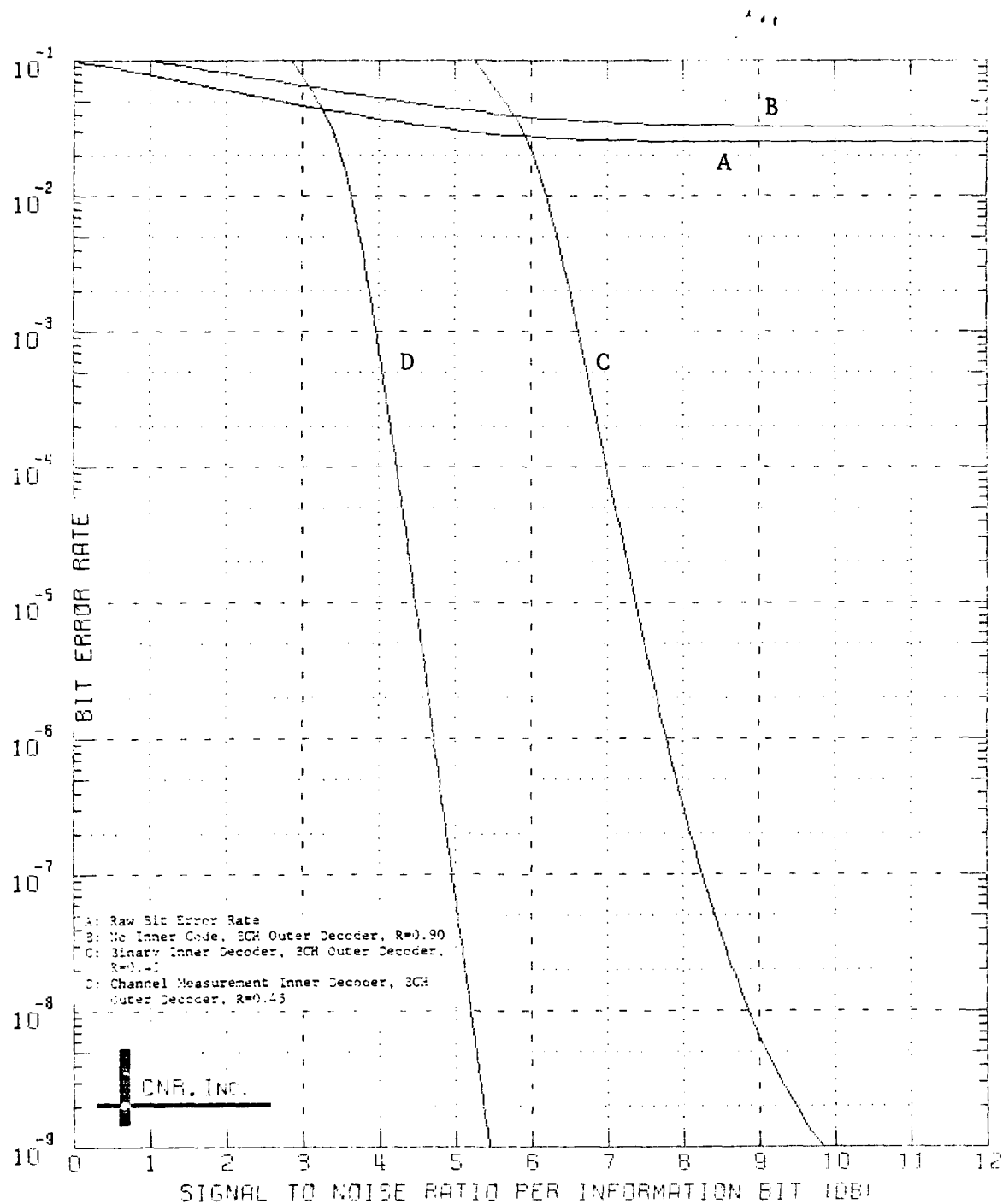
Figure 8.2 Decoded Performance of a Two-Stage Coding Approach Outer Decoder: BCH Code (240,216;7) Inner Decoder: Convolutional Code; Rate=1/2; K=7 \delta=0.05 and No Erasure Information Employed
