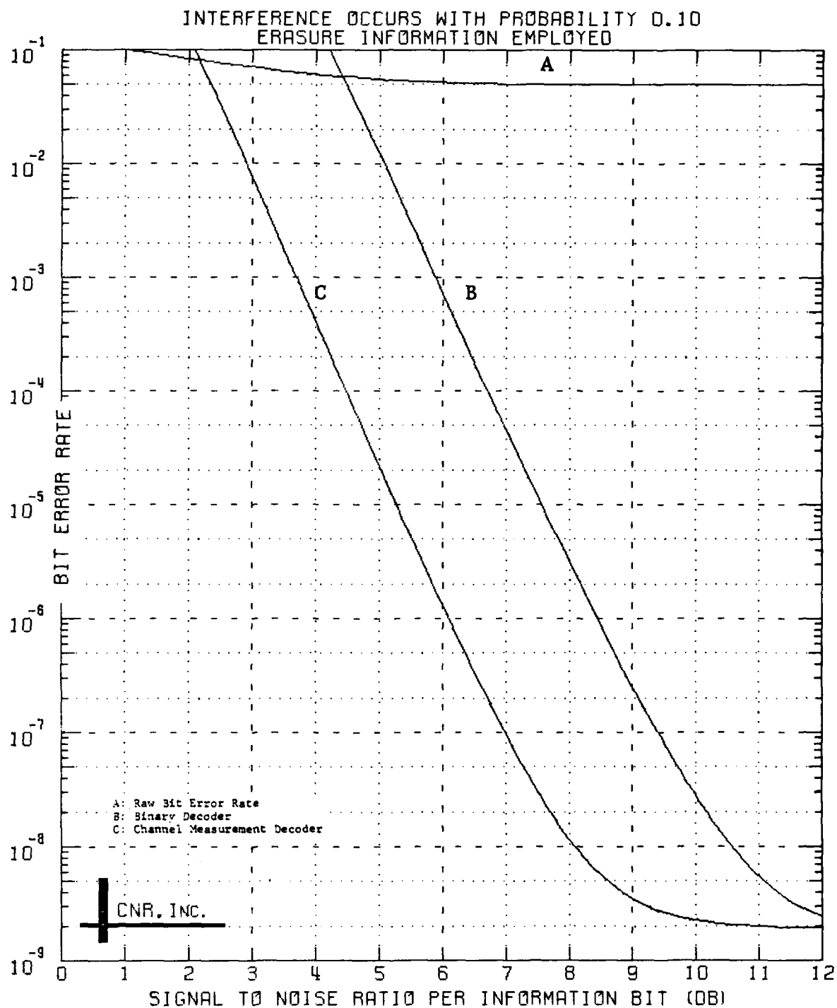
Figure 6.7 Decoded Performance of a Convolutional Code Rate 1/2; Constraint Length = 7
