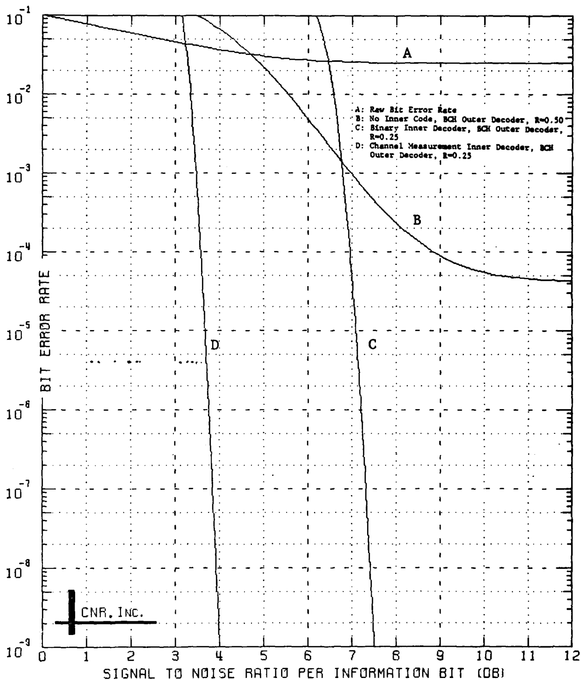
Figure 7.15 Decoded Performance of a Two-Stage Coding Approach Outer Decoder: BCH Code (128,64;22) Inner Decoder: Block Code (128,64;22) \delta=0.05 and Erasure Information is Employed
