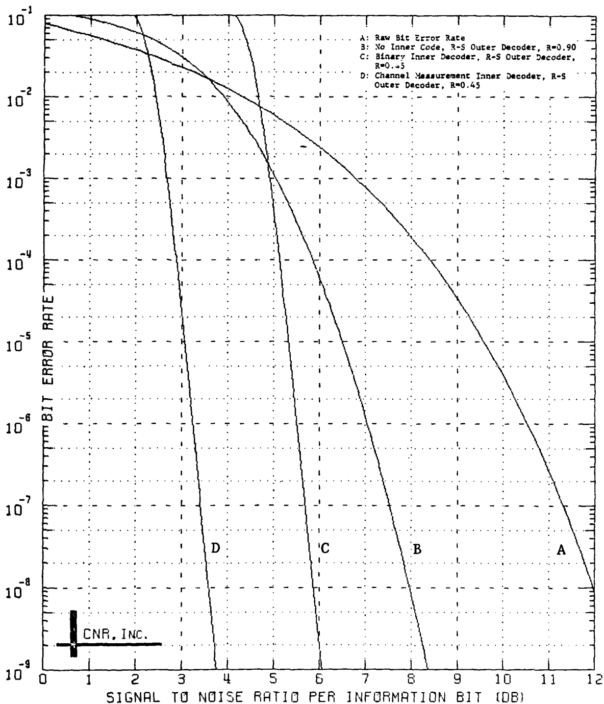
Figure 9.11 Decoded Performance of a Two-Stage Coding Approach Outer Decoder: Reed-Solomon Code (60,54;7) Symbol Interleaver Employed Inner Decoder: Convolutional Code, Rate=1/2; K=7 \delta=0.00 and No Erasure Information is Employed
