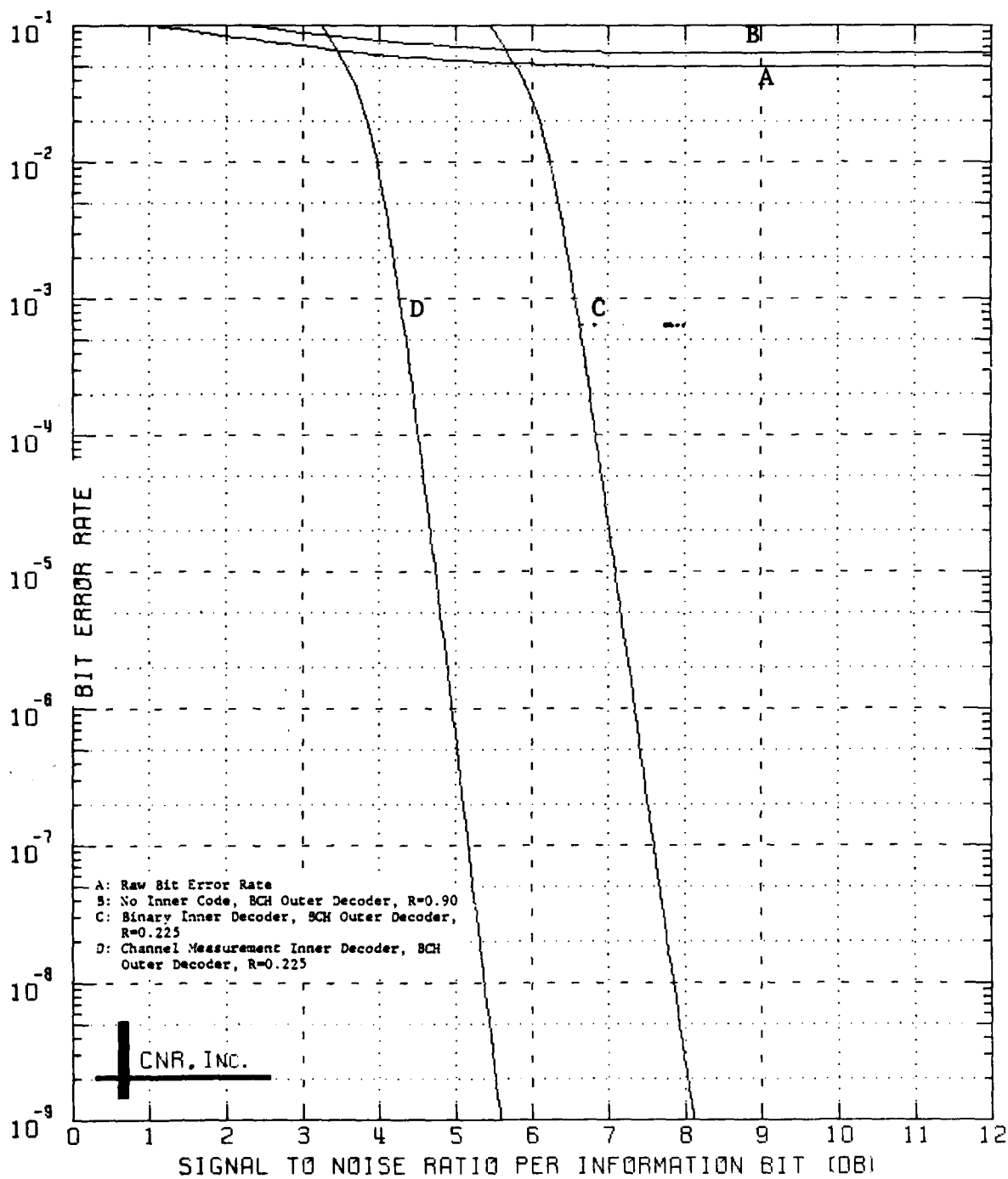
Figure 8.12 Decoded Performance of a Two-Stage Coding Approach Outer Decoder: BCH Code (240,216;7) Inner Decoder: Convolutional Code; Rate=1/4; K=7 \delta=0.10 and No Erasure Information Employed
