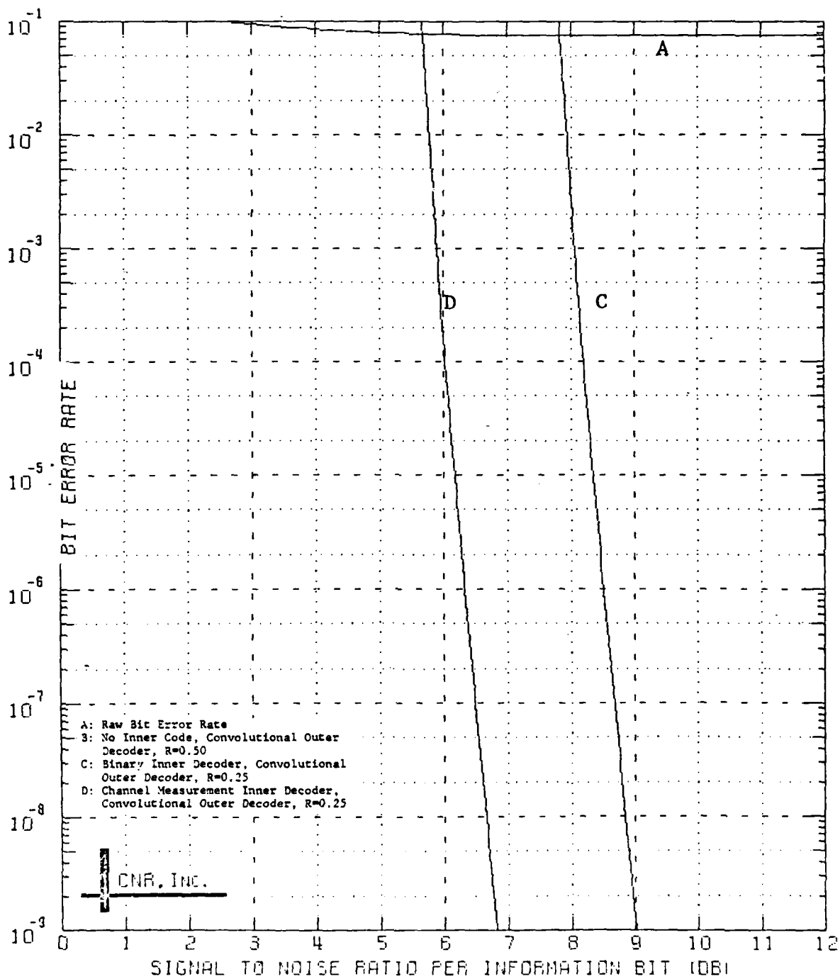
Figure 8.35 Decoded Performance of a Two-Stage Coding Approach Outer Decoder: Convolutional Code, Rate=1/2; K=7 Inner Decoder: Convolutional Code, Rate=1/2; K=7 \delta=0.15 and Erasure Information is Employed
