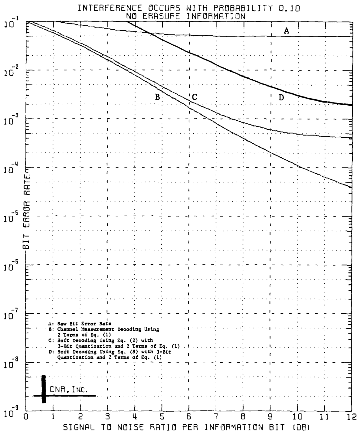
Figure 13 Decoded Performance of a Convolutional Code Rate 1/2; Constraint Length = 3; Gaussian Channel; CPSK Modulation
