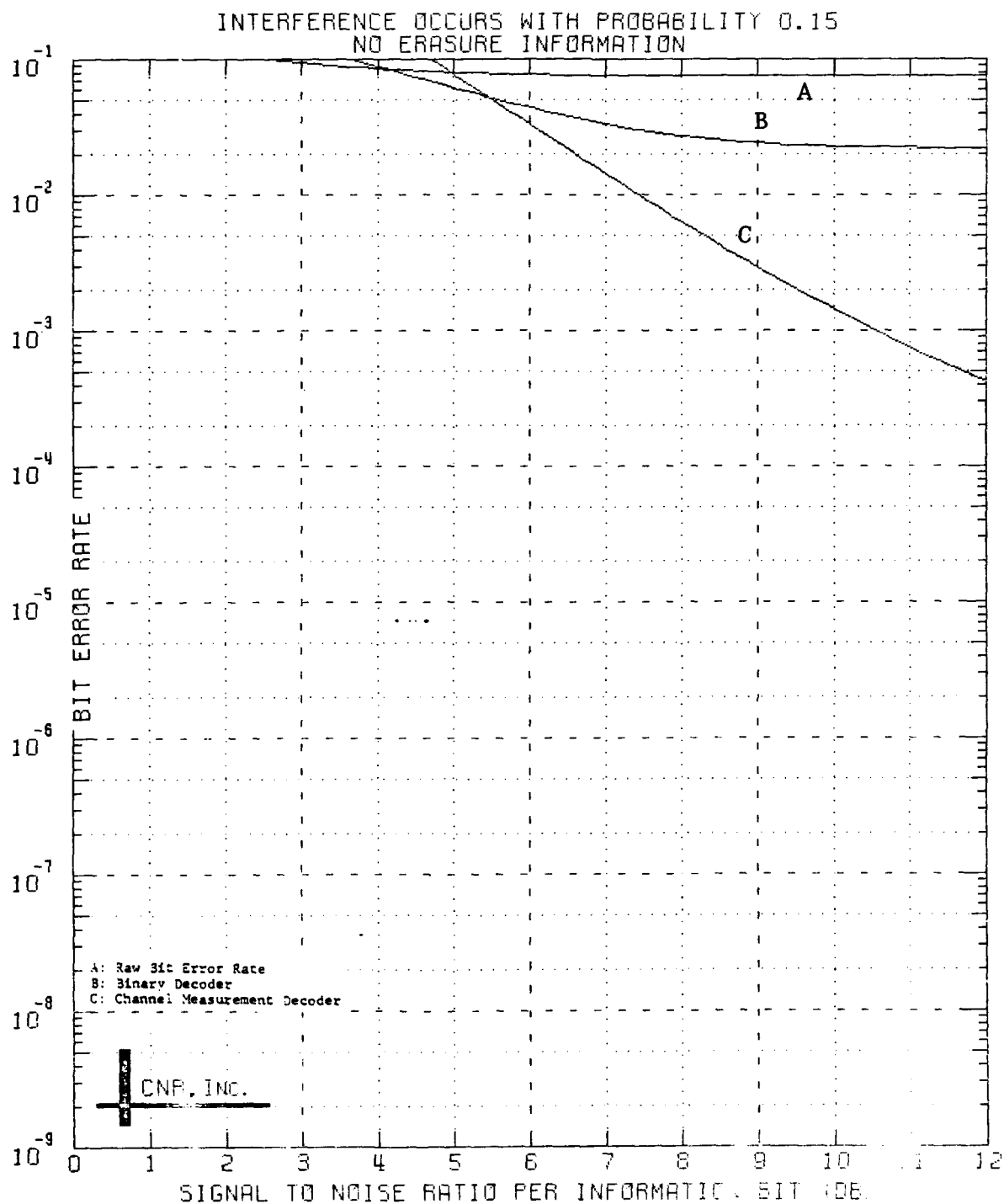
Figure 5.4 Decoded Performance of a Block Code Dimensions (24,12;8)
