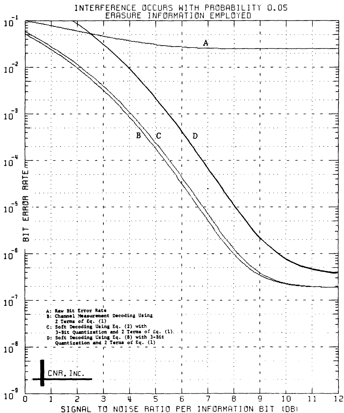
Figure 14 Decoded Performance of a Convolutional Code Rate 1/2; Constraint Length = 3; Gaussian Channel; CPSK Modulation
