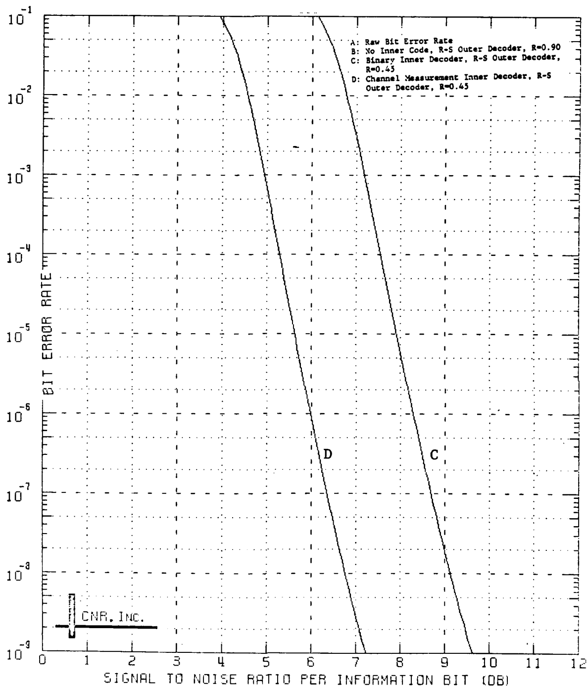
Figure 9.28 Decoded Performance of a Two-Stage Coding Approach Outer Decoder: Reed-Solomon Code (40,36;5) Bit Interleaver Employed Inner Decoder: Convolutional Code, Rate=1/2; K=7 \delta=0.20 and Erasure Information is Employed
