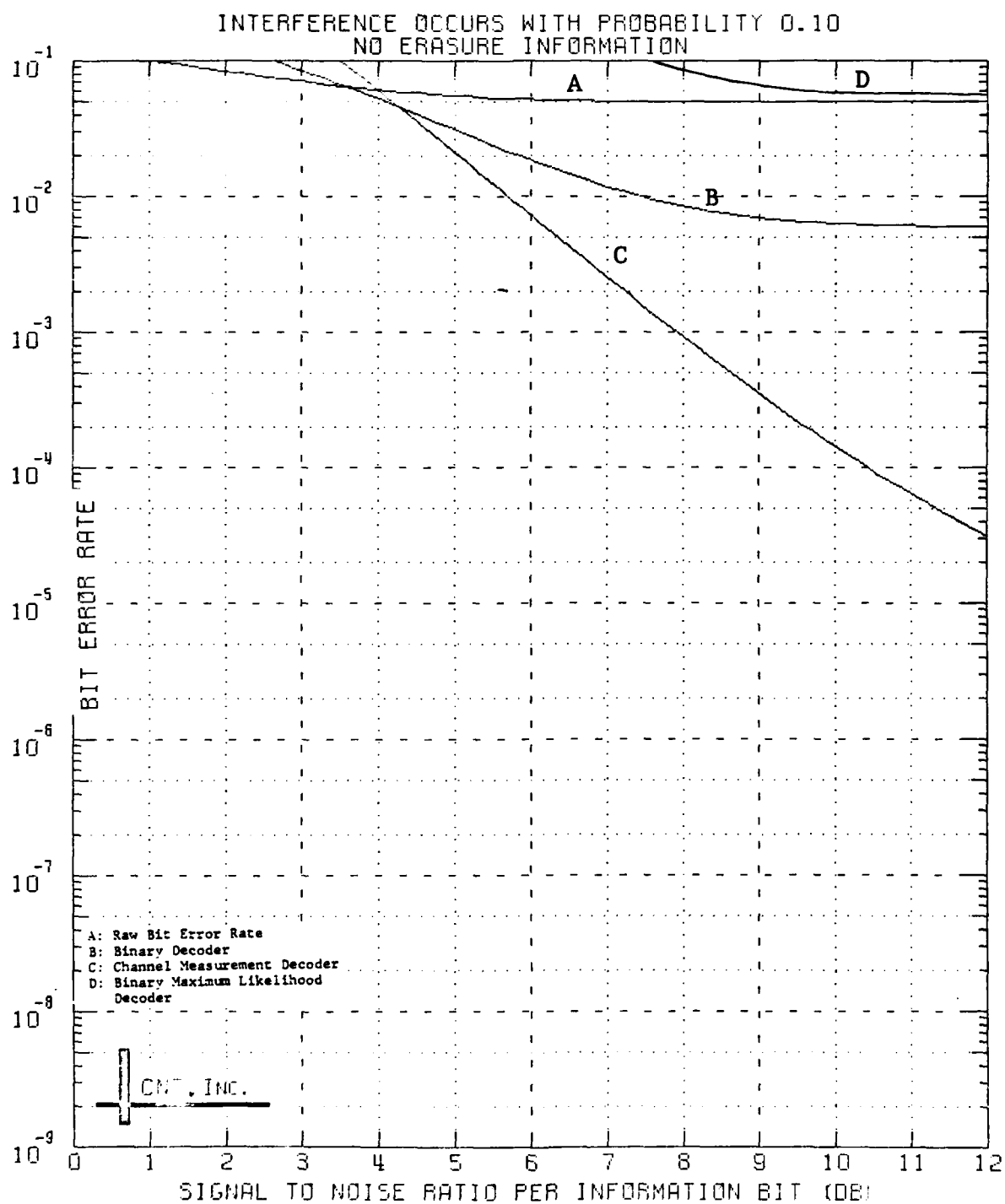
Figure 5.21 Decoded Performance of a Block Code Dimensions (24,12;8)
