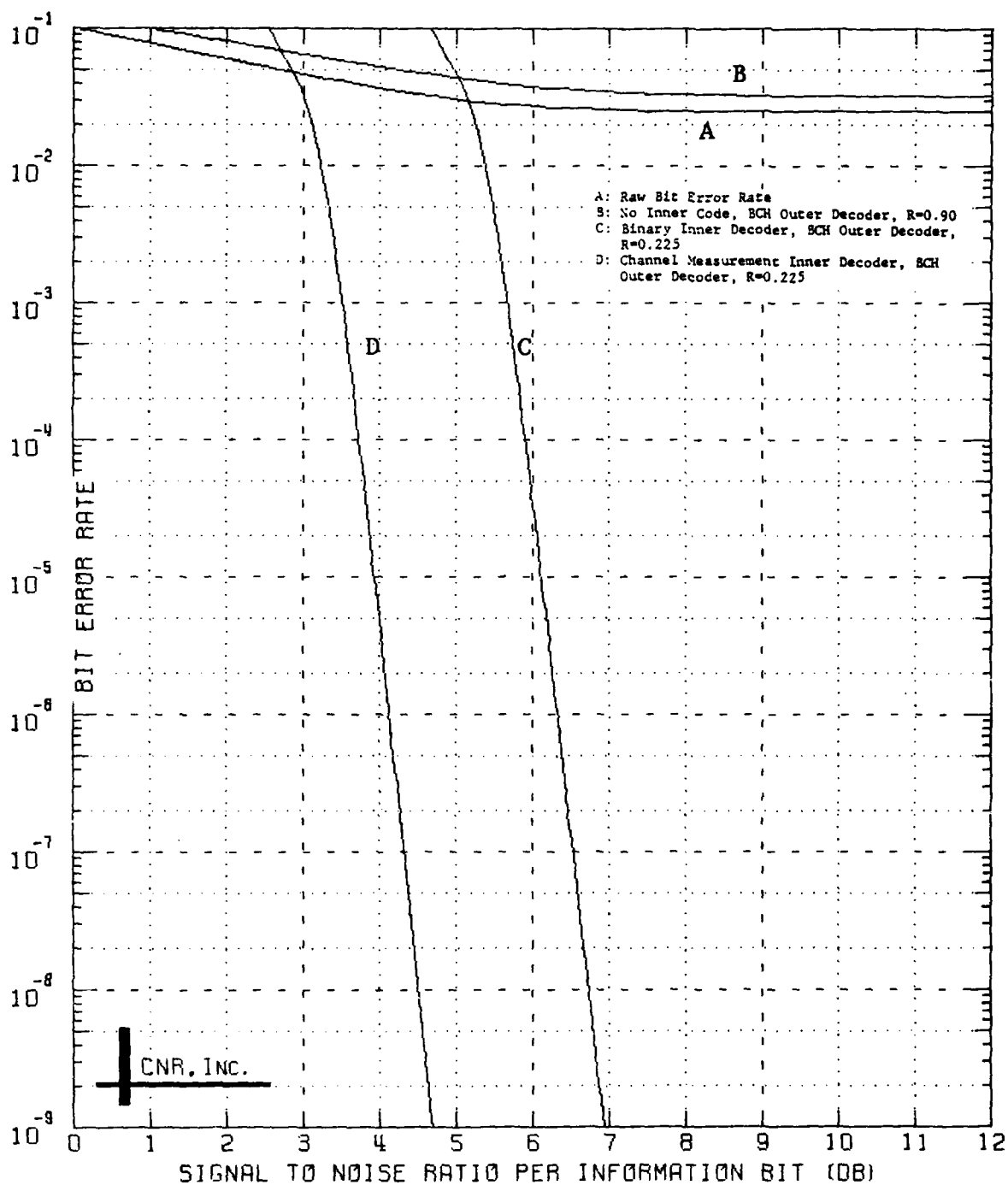
Figure 8.11 Decoded Performance of a Two-Stage Coding Approach Outer Decoder: BCH Code (240,216;7) Inner Decoder: Convolutional Code; Rate=1/4; K=7 \delta=0.05 and No Erasure Information Employed
