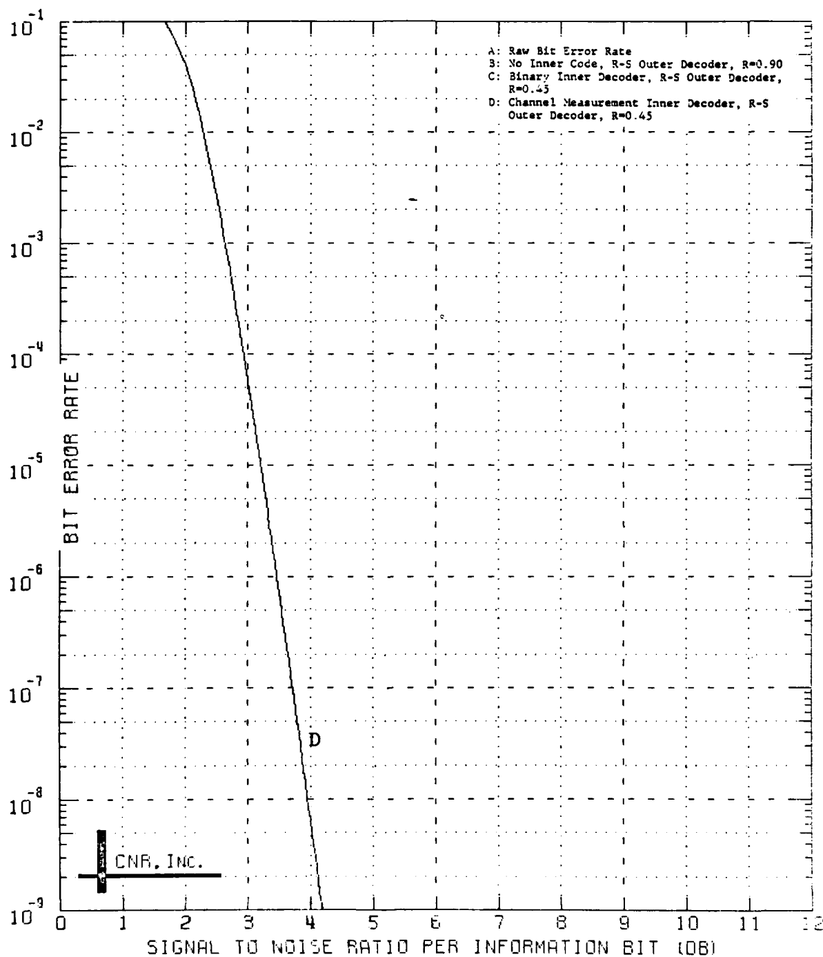
Figure 9.73 Decoded Performance of a Two-Stage Coding Approach Outer Decoder: Reed-Solomon Code (40,36;5) Symbol Interleaver Employed Inner Decoder: Block Code (128,64;22) \delta=0.20 and Erasure Information is Employed
