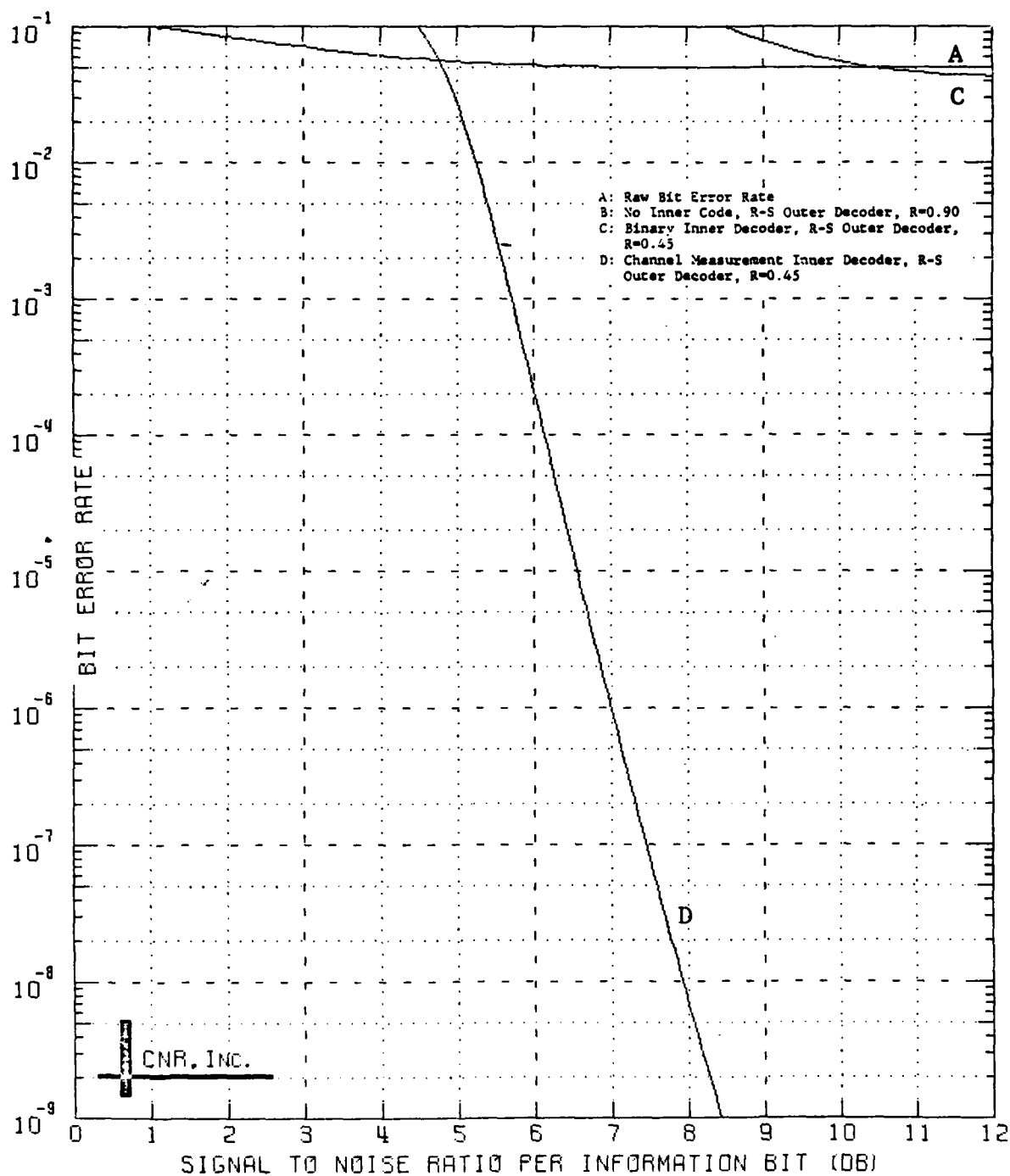
Figure 9.22 Decoded Performance of a Two-Stage Coding Approach Outer Decoder: Reed-Solomon Code (40,36;5) Bit Interleaver Employed Inner Decoder: Convolutional Code, Rate=1/2; K=7 \delta=0.10 and No Erasure Information Employed
