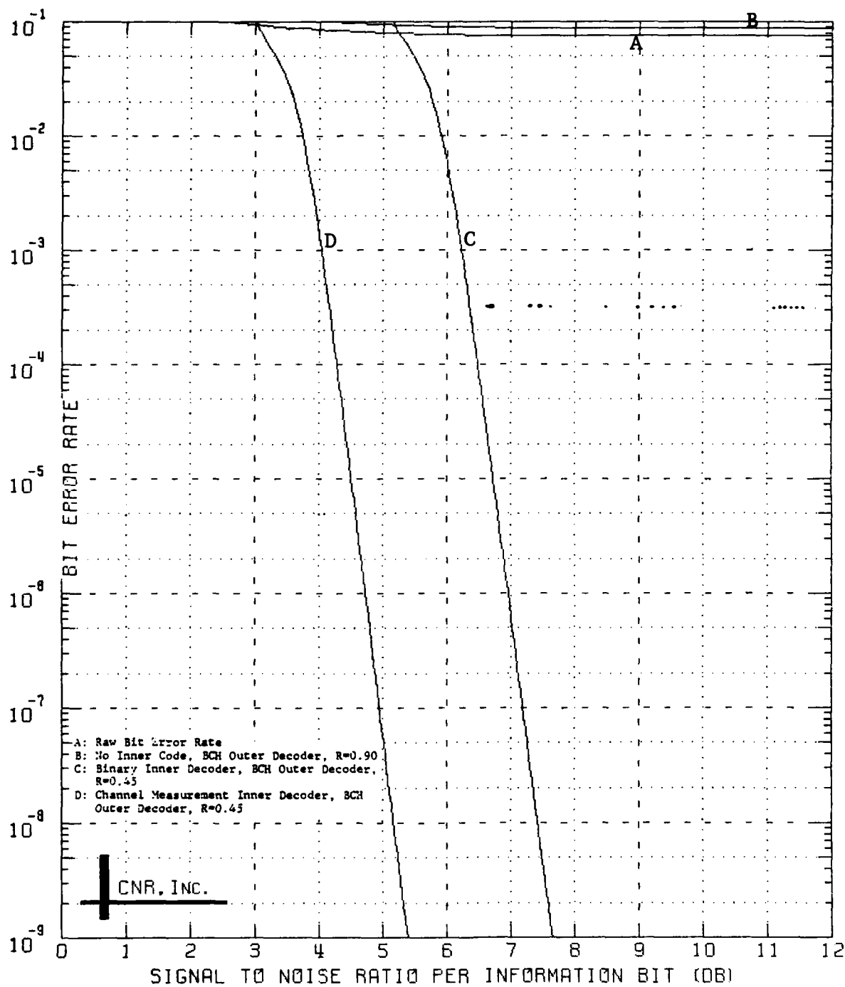
Figure 8.8 Decoded Performance of a Two-Stage Coding Approach Outer Decoder: BCH Code (240,216;7) Inner Decoder: Convolutional Code; Rate=1/2; K=7 \delta=0.15 and Erasure Information is Employed
