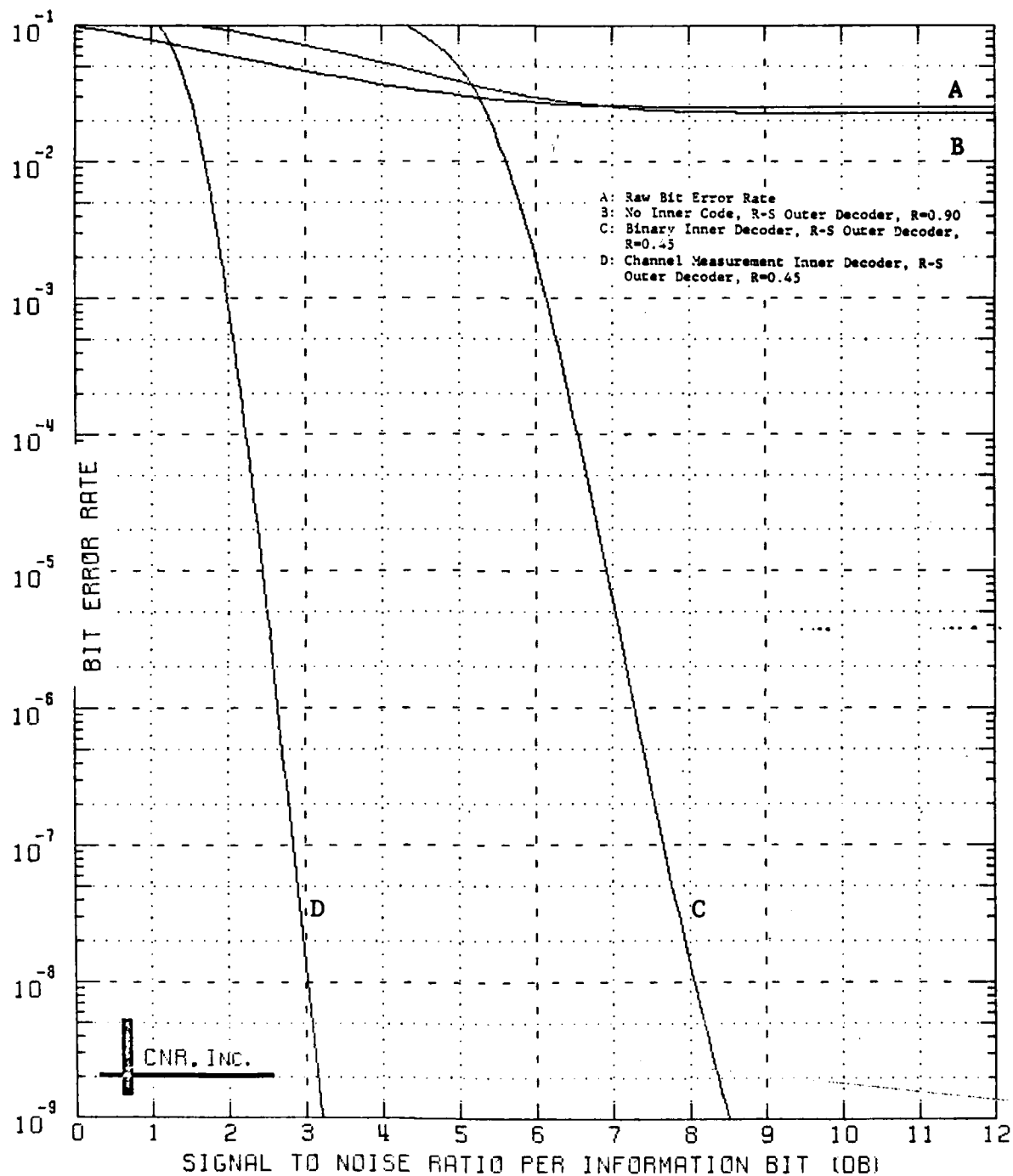
Figure 9.48 Decoded Performance of a Two-Stage Coding Approach Outer Decoder: Reed-Solomon Code (60,54;7) Symbol Interleaver Employed Inner Decoder: Block Code (128,64;22) \delta=0.05 and No Erasure Information Employed
