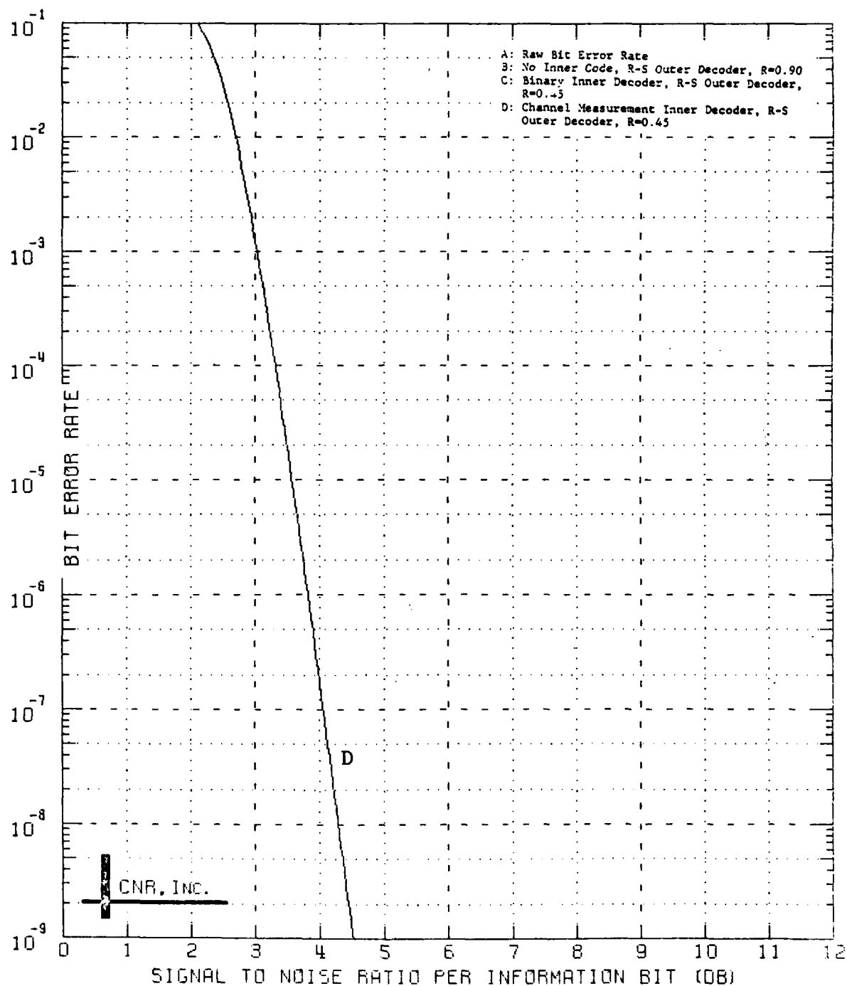
Figure 9.64 Decoded Performance of a Two-Stage Coding Approach Outer Decoder: Reed-Solomon Code (40,36;5) Bit Interleaver Employed Inner Decoder: Block Code (128,64;22) \delta = 0.20 and Erasure Information is Employed
