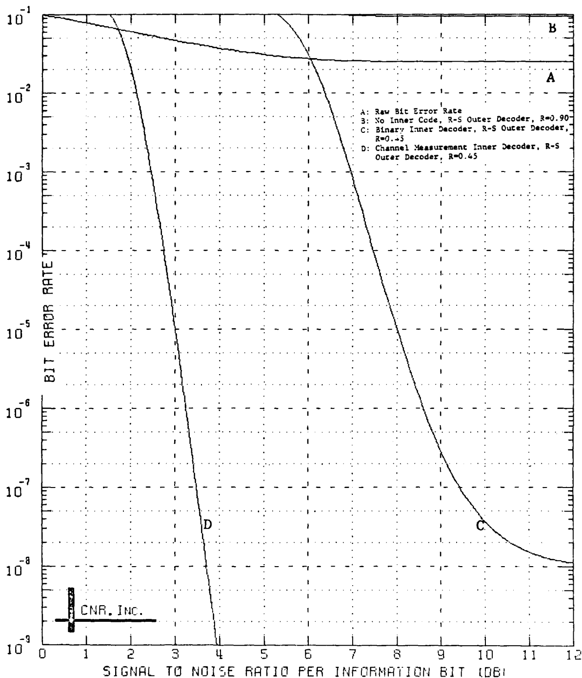
Figure 9.57 Decoded Performance of a Two-Stage Coding Approach Outer Decoder: Reed-Solomon Code (40,36;5) Bit Interleaver Employed Inner Decoder: Block Code (128,64;22) \delta=0.05 and No Erasure Information Employed
