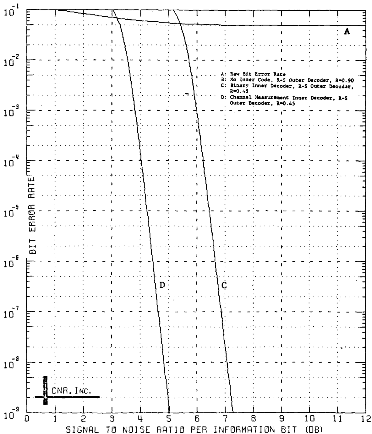
Figure 9.8 Decoded Performance of a Two-Stage Coding Approach Outer Decoder: Reed-Solomon Code (60,54;7) Bit Interleaver Employed Inner Decoder: Convolutional Code, Rate=1/2; K=7 \delta=0.10 and Erasure Information is Employed
