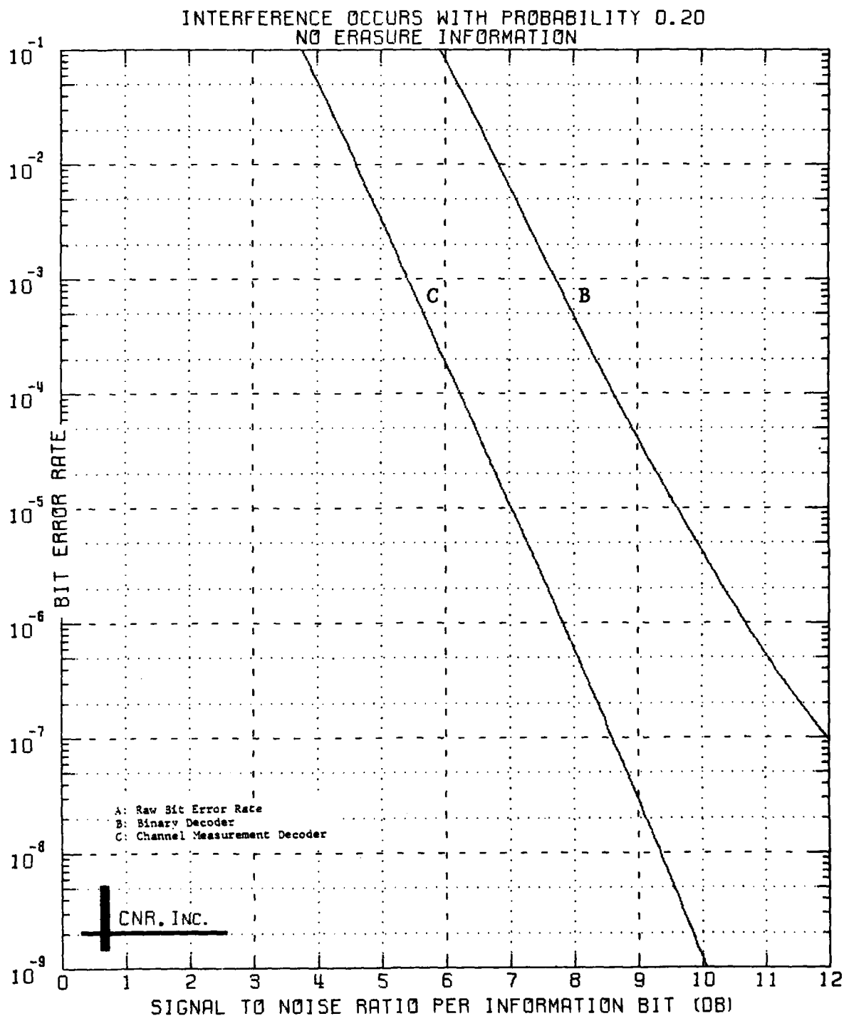
Figure 6.23 Decoded Performance of a Convolutional Code Rate 1/8; Constraint Length = 7
