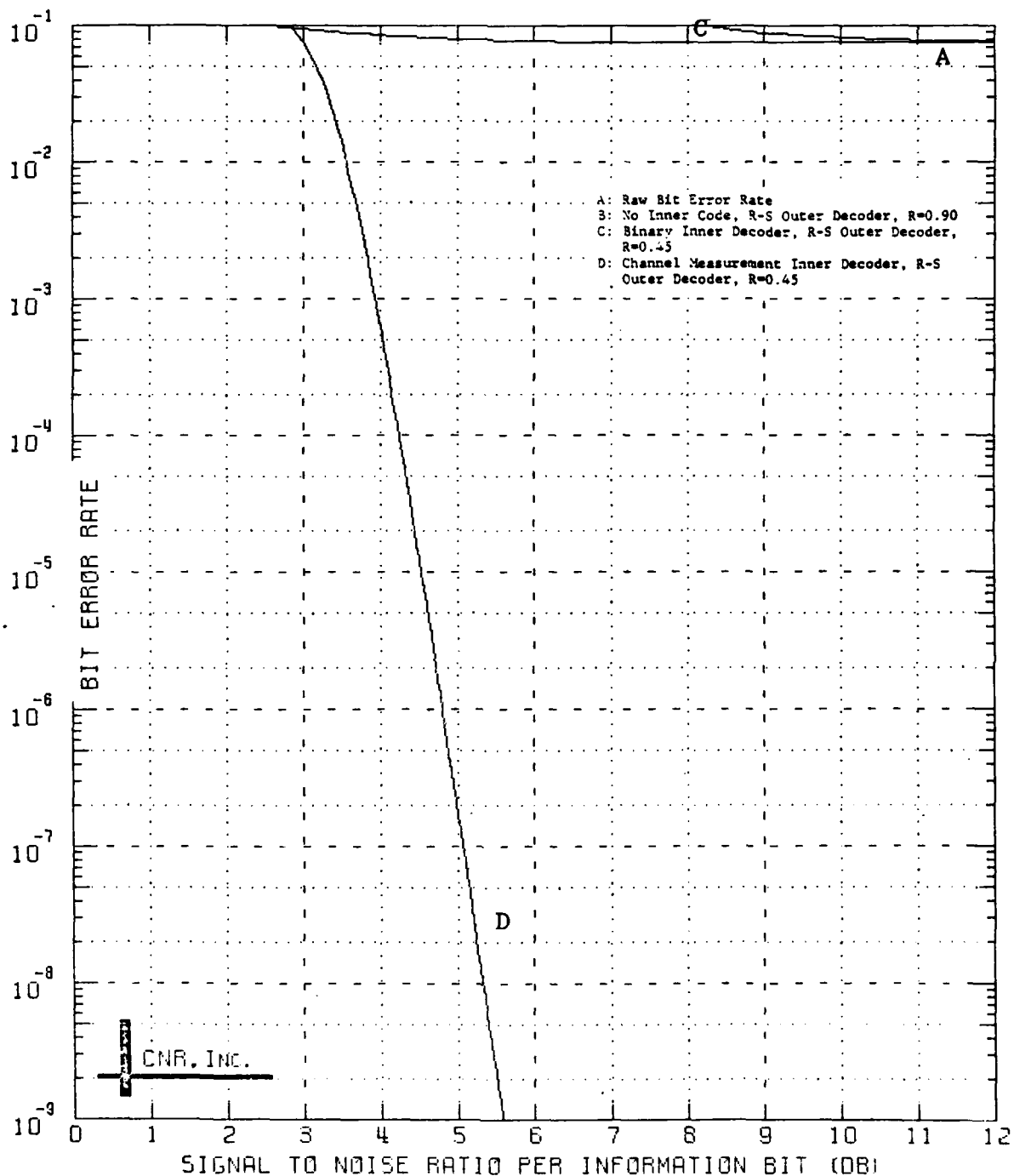
Figure 9.50 Decoded Performance of a Two-Stage Coding Approach Outer Decoder: Reed-Solomon Code (60,54;7) Symbol Interleaver Employed Inner Decoder: Block Code (128,64;22) \delta=0.15 and No Erasure Information Employed
