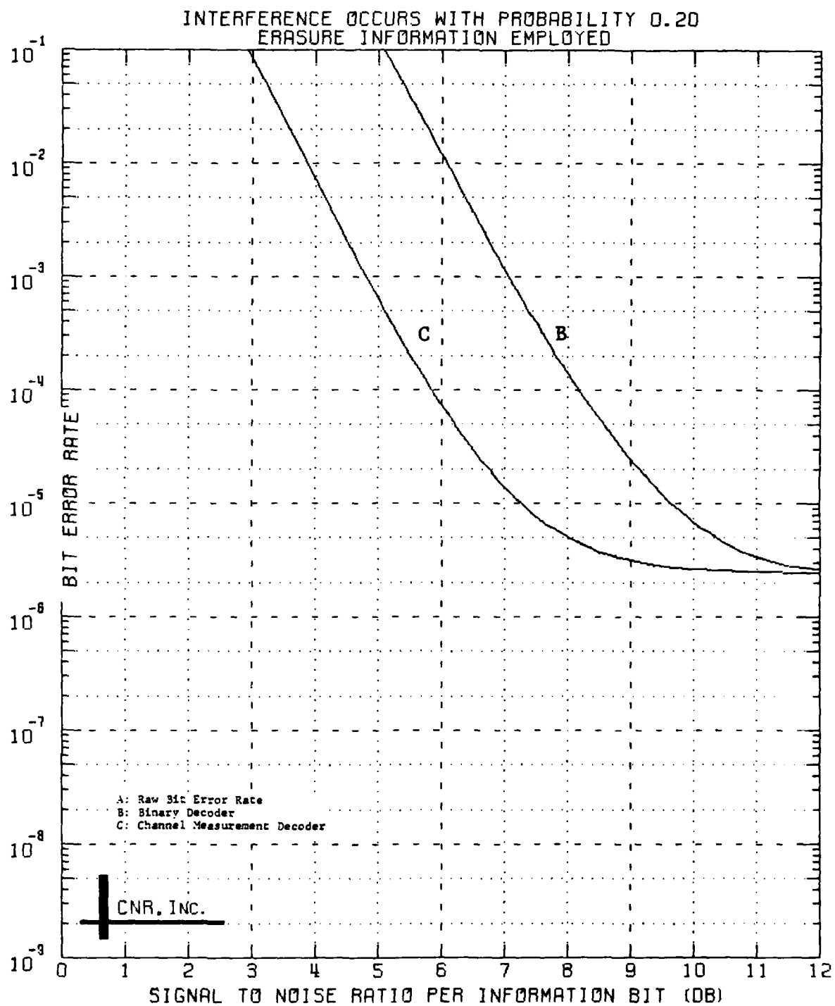
Figure 6.9 Decoded Performance of a Convolutional Code Rate 1/2; Constraint Length = 7.
