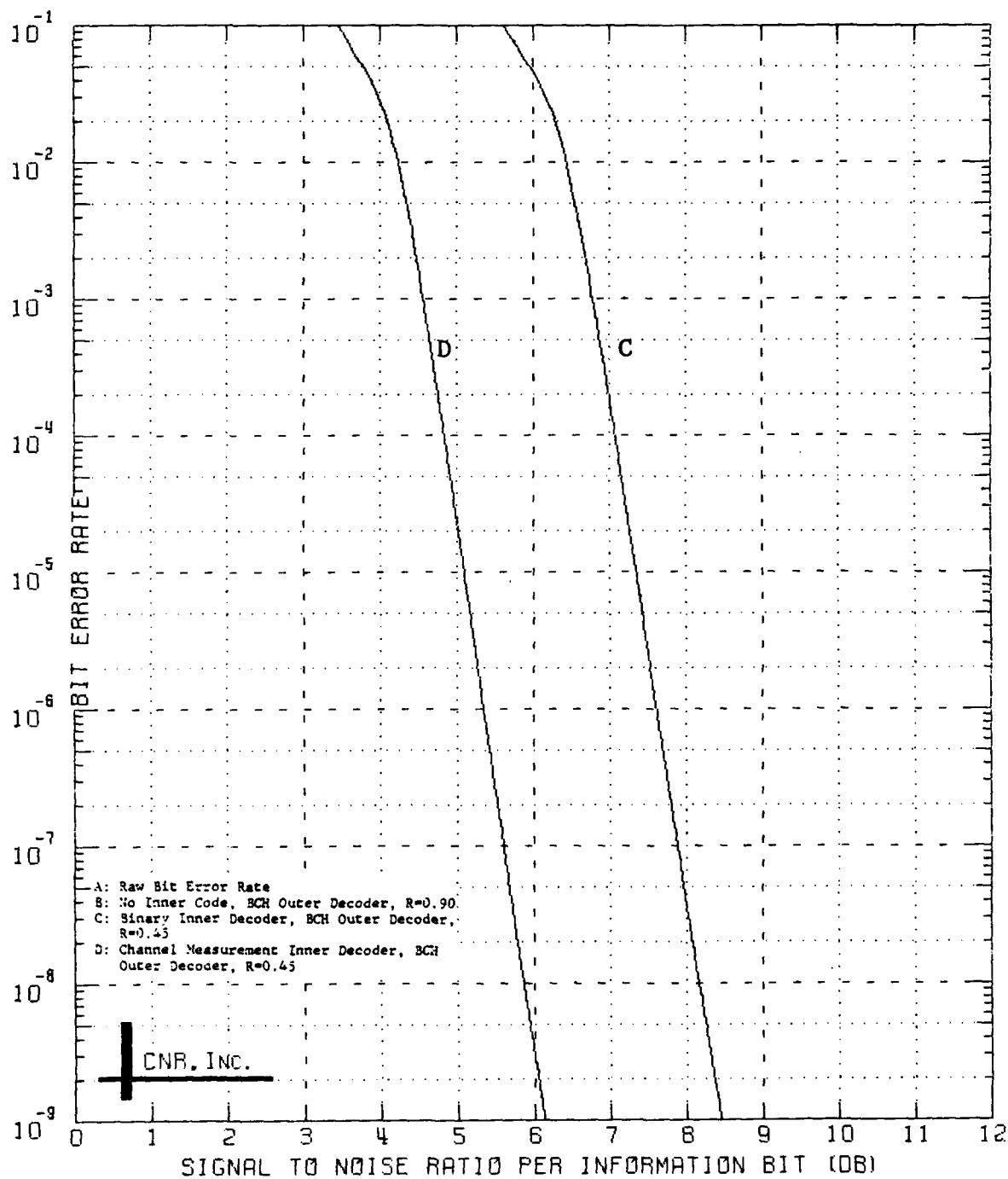
Figure 8.9 Decoded Performance of a Two-Stage Coding Approach Outer Decoder: BCH Code (240,216;7) Inner Decoder: Convolutional Code; Rate=1/2; K=7 \delta=0.20 and Erasure Information is Employed
