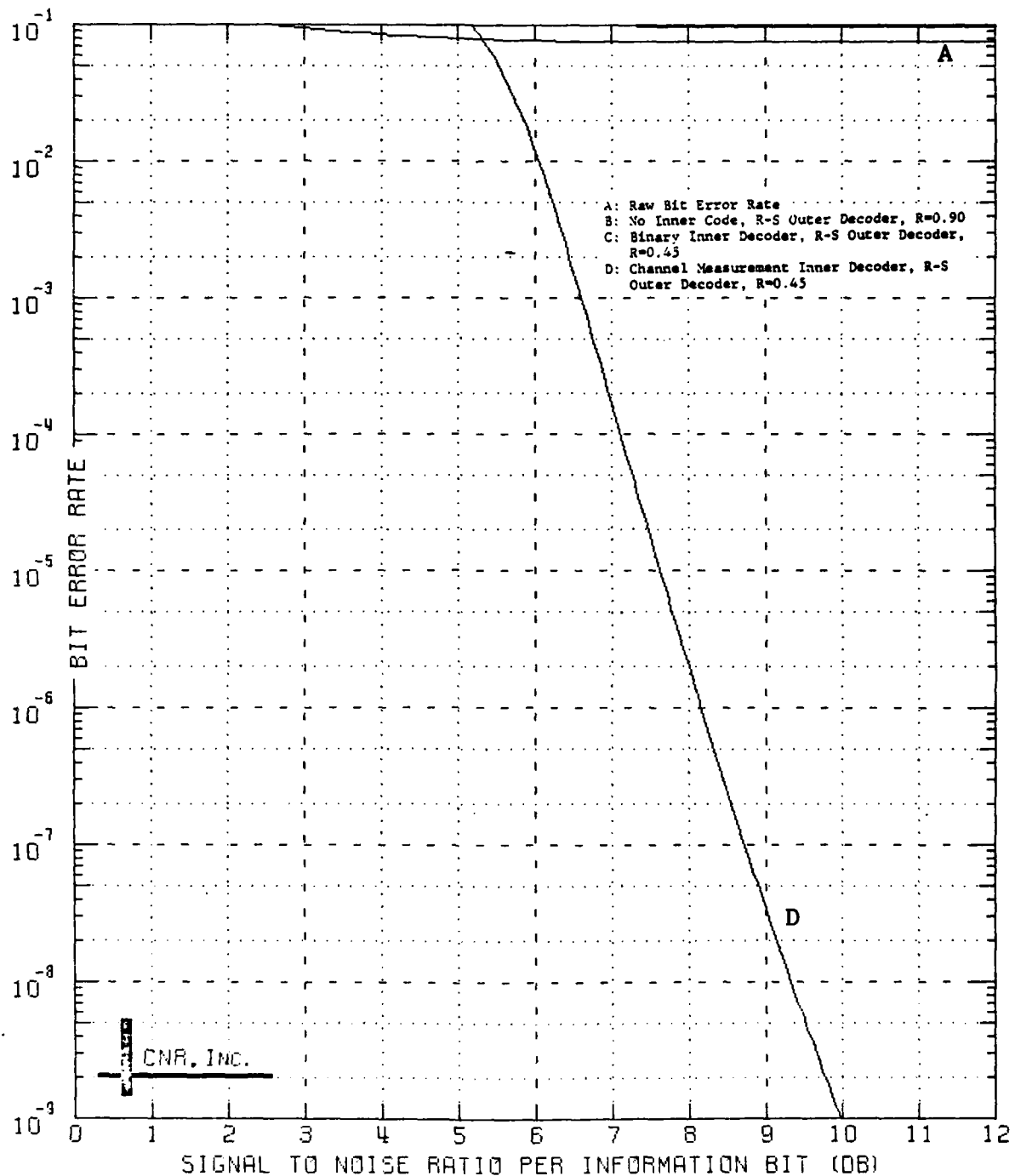
Figure 9.32 Decoded Performance of a Two-Stage Coding Approach Outer Decoder: Reed-Solomon Code (40,36;5) Symbol Interleaver Employed Inner Decoder: Convolutional Code, Rate=1/2; K=7 \delta=0.15 and No Erasure Information Employed
