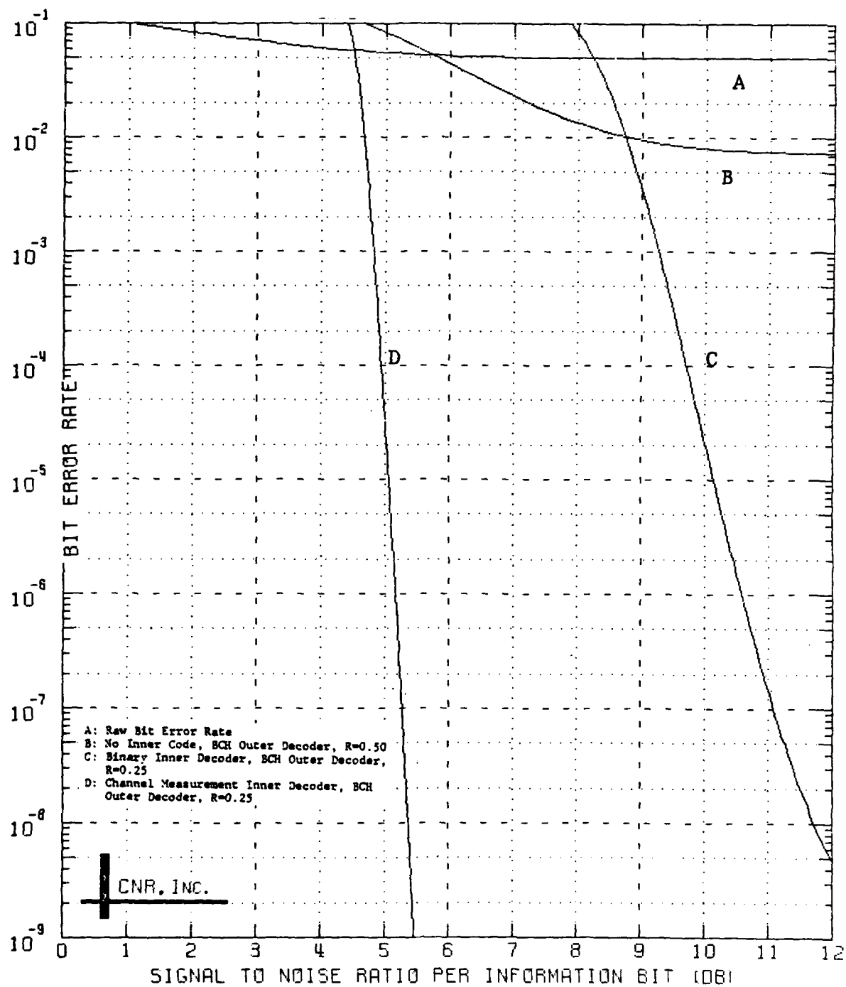
Figure 7.12 Decoded Performance of a Two-Stage Coding Approach Outer Decoder: BCH Code (128,64;22) Inner Decoder: Block Code (128,64;22) \delta=0.10 and No Erasure Information Employed
