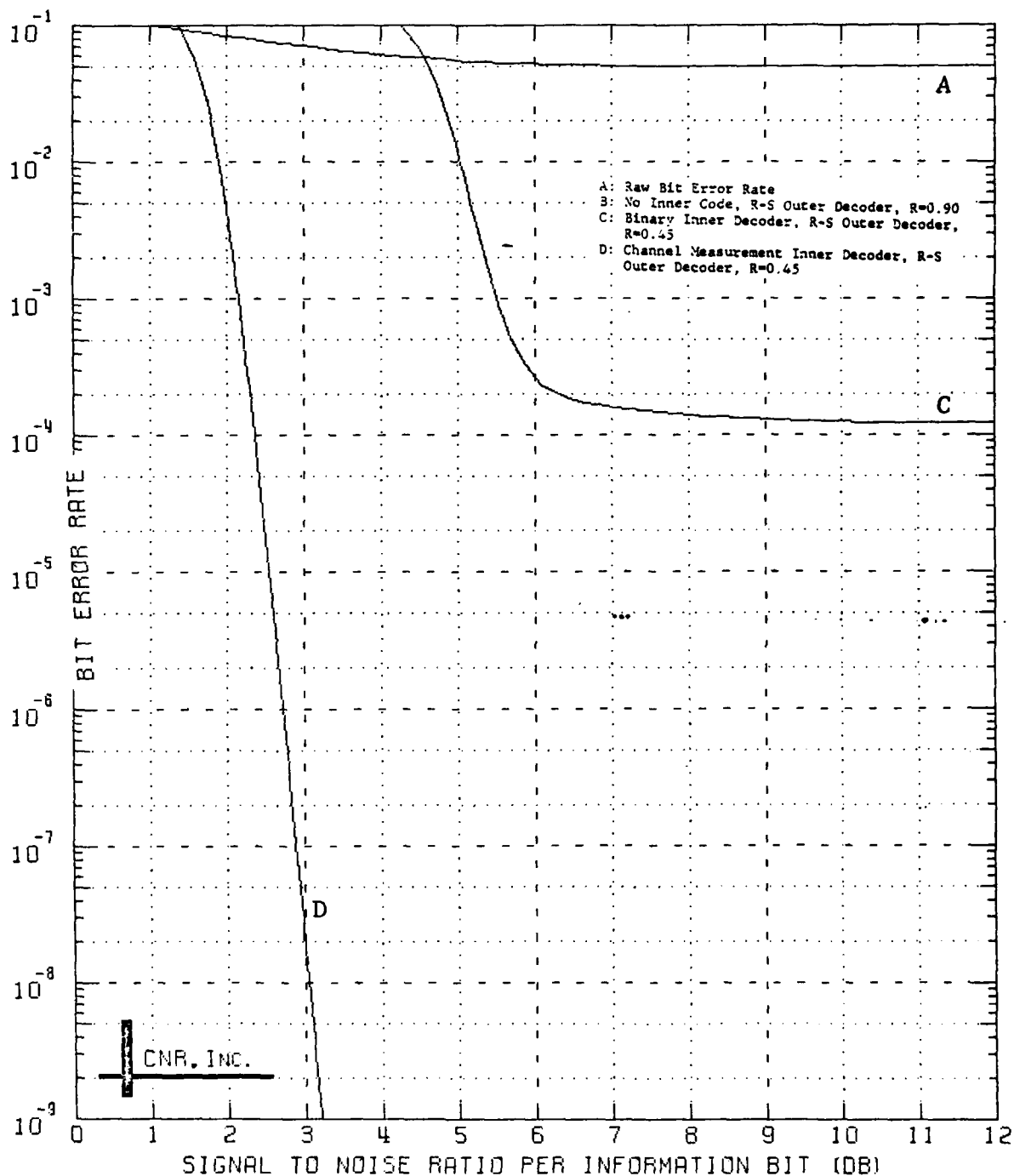
Figure 9.44 Decoded Performance of a Two-Stage Coding Approach Outer Decoder: Reed-Solomon Code (60,54;7) Bit Interleaver Employed Inner Decoder: Block Code (128,64;22) \delta=0.10 and Erasure Information is Employed
