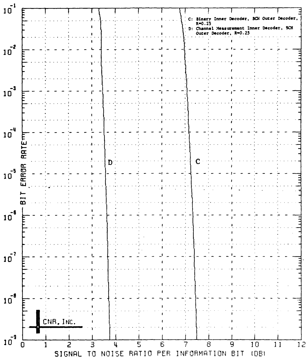
Figure 7.21 Decoded Performance of a Two-Stage Coding Approach Adaptive Technique Outer Decoder: BCH Code (128,64;22) Inner Decoder: Block Code (128,64;22) \delta=0.00 and No Erasure Information Employed
