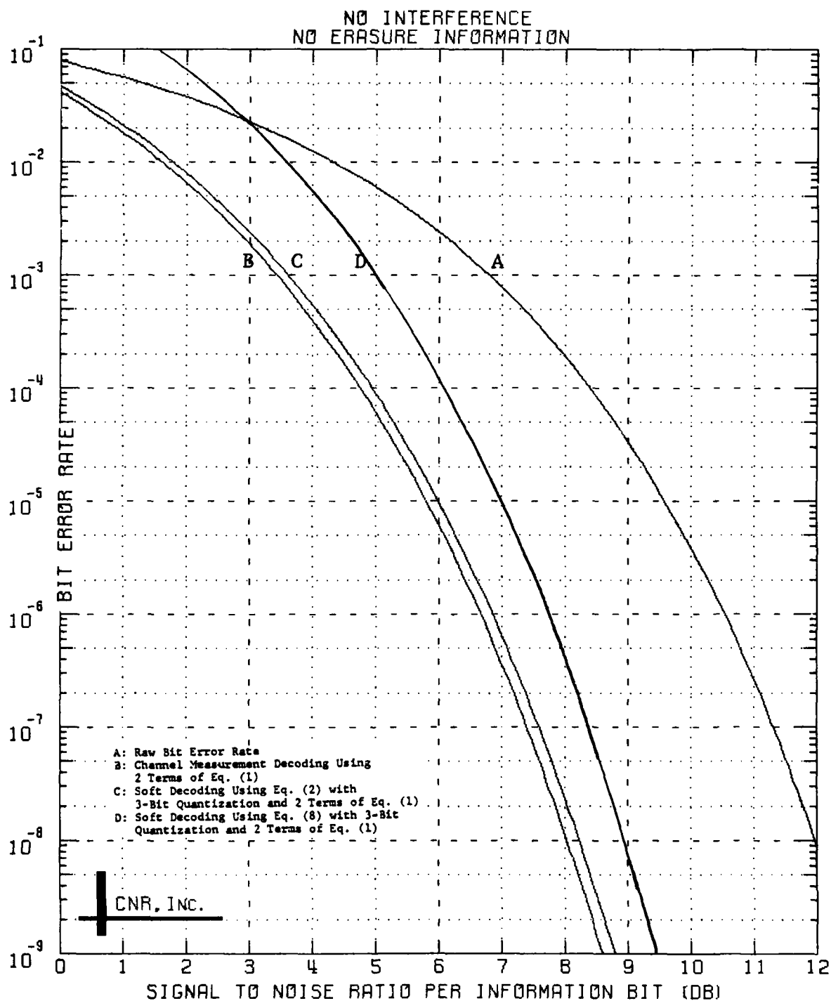
Figure 11 Decoded Performance of a Convolutional Code Rate 1/2; Constraint Length = 3; Gaussian Channel; CPSK Modulation
