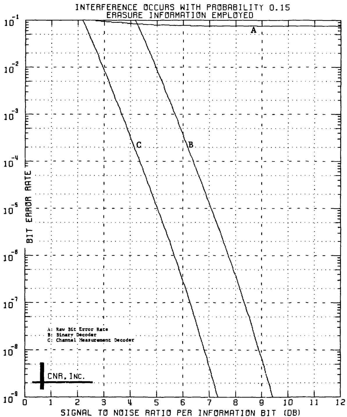
Figure 6.26 Decoded Performance of a Convolutional Code Rate 1/8; Constraint Length = 7
