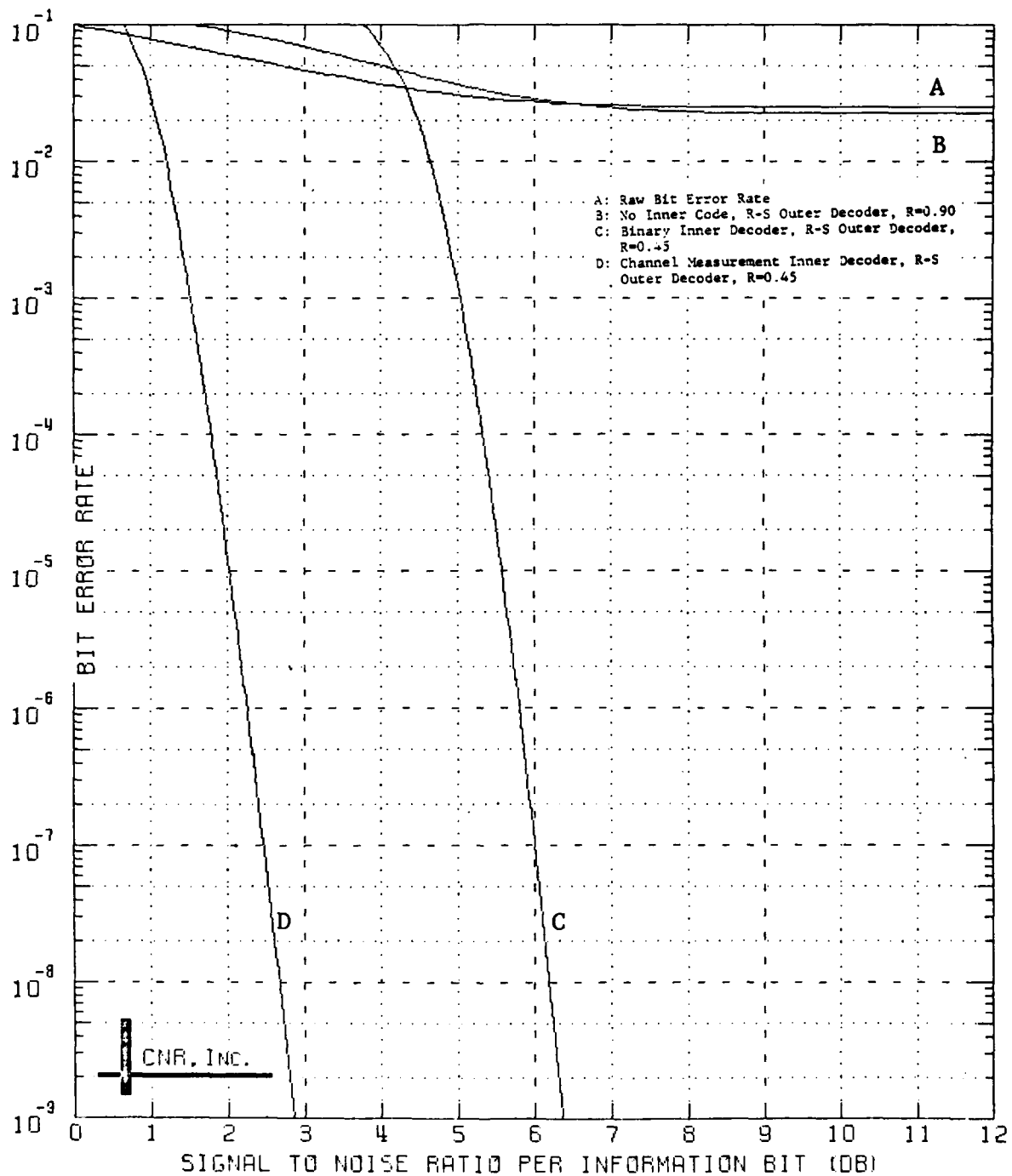
Figure 9.70 Decoded Performance of a Two-Stage Coding Approach Outer Decoder: Reed-Solomon Code (40,36;5) Symbol Interleaver Employed Inner Decoder: Block Code (128,64;22) \delta=0.05 and Erasure Information Employed
