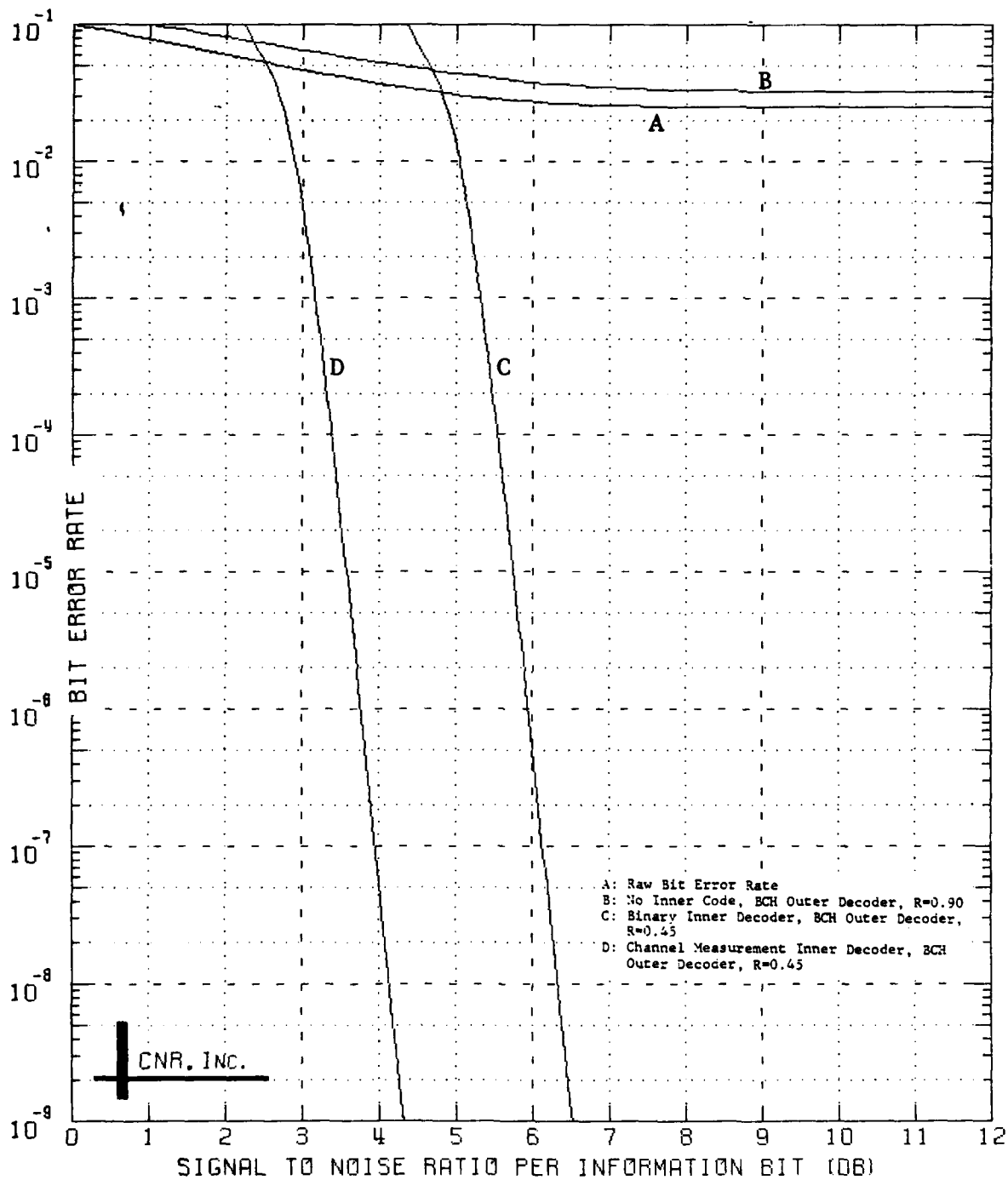
Figure 8.6 Decoder Performance of a Two-Stage Coding Approach Outer Decoder: BCH Code (240,216;7) Inner Decoder: Convolutional Code; Rate=1/2; K=7 \delta=0.05 and Erasure Information is Employed
