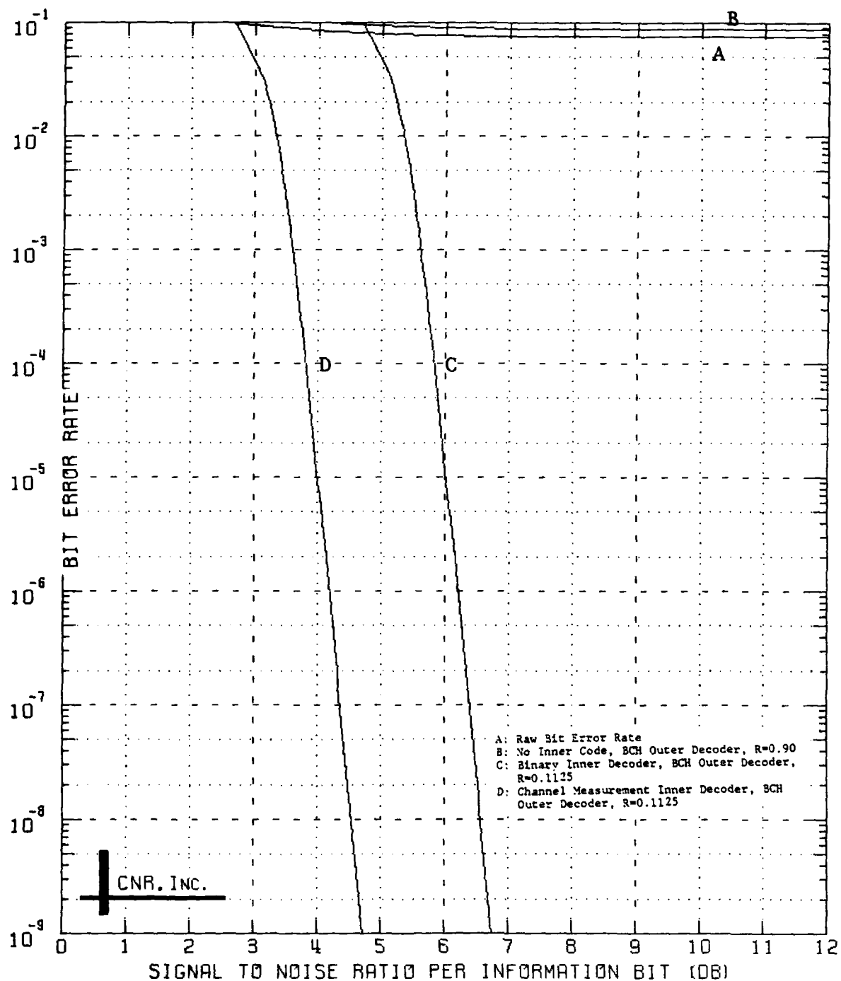
Figure 8.26 Decoded Performance of a Two-Stage Coding Approach Outer Decoder: BCH Code (240,216;7) Inner Decoder: Convolutional Code; Rate=1/8; K=7 \delta=0.15 and Erasure Information is Employed
