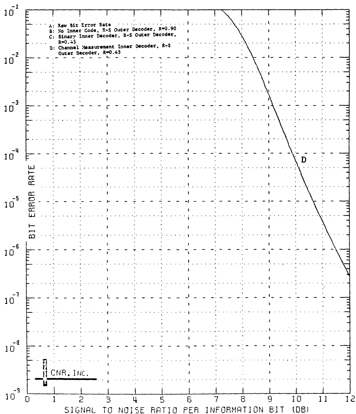
Figure 9.24 Decoded Performance of a Two-Stage Coding Approach Outer Decoder: Reed-Solomon Code (40,36;5) Bit Interleaver Employed Inner Decoder: Convolutional Code, Rate=1/2; K=7 \delta=0.20 and No Erasure Information Employed
