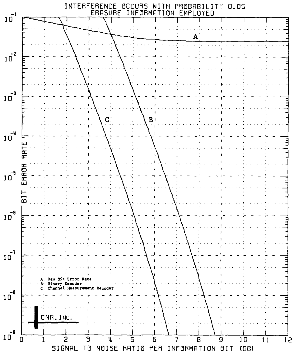
Figure 6.24 Decoded Performance of a Convolutional Code Rate 1/8; Constraint Length = 7
