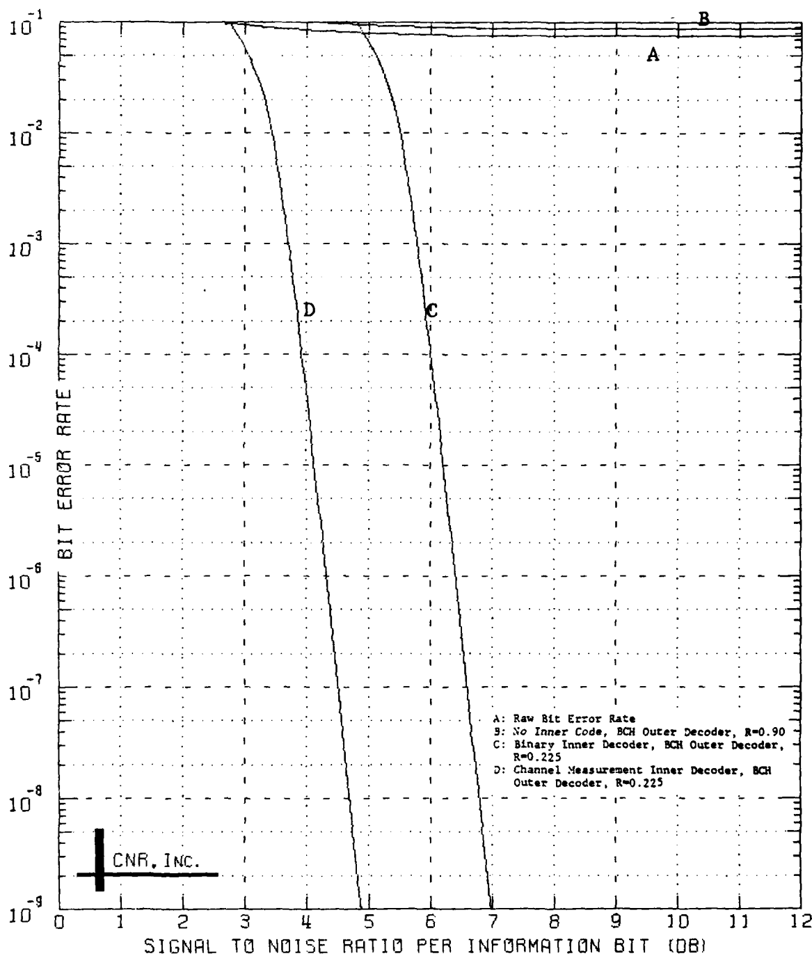
Figure 8.17 Decoded Performance of a Two-Stage Coding Approach Outer Decoder: BCH Code (240,216;7) Inner Decoder: Convolutional Code; Rate=1/4; K=7 \delta=0.15 and Erasure Information is Employed
