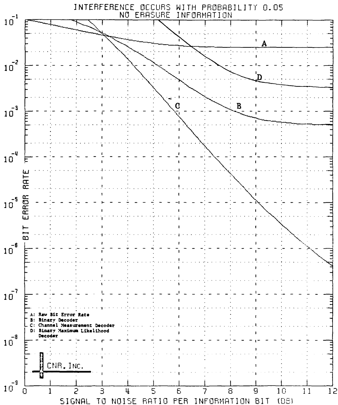
Figure 5.20 Decoded Performance of a Block Code Dimensions (24,12;8)
