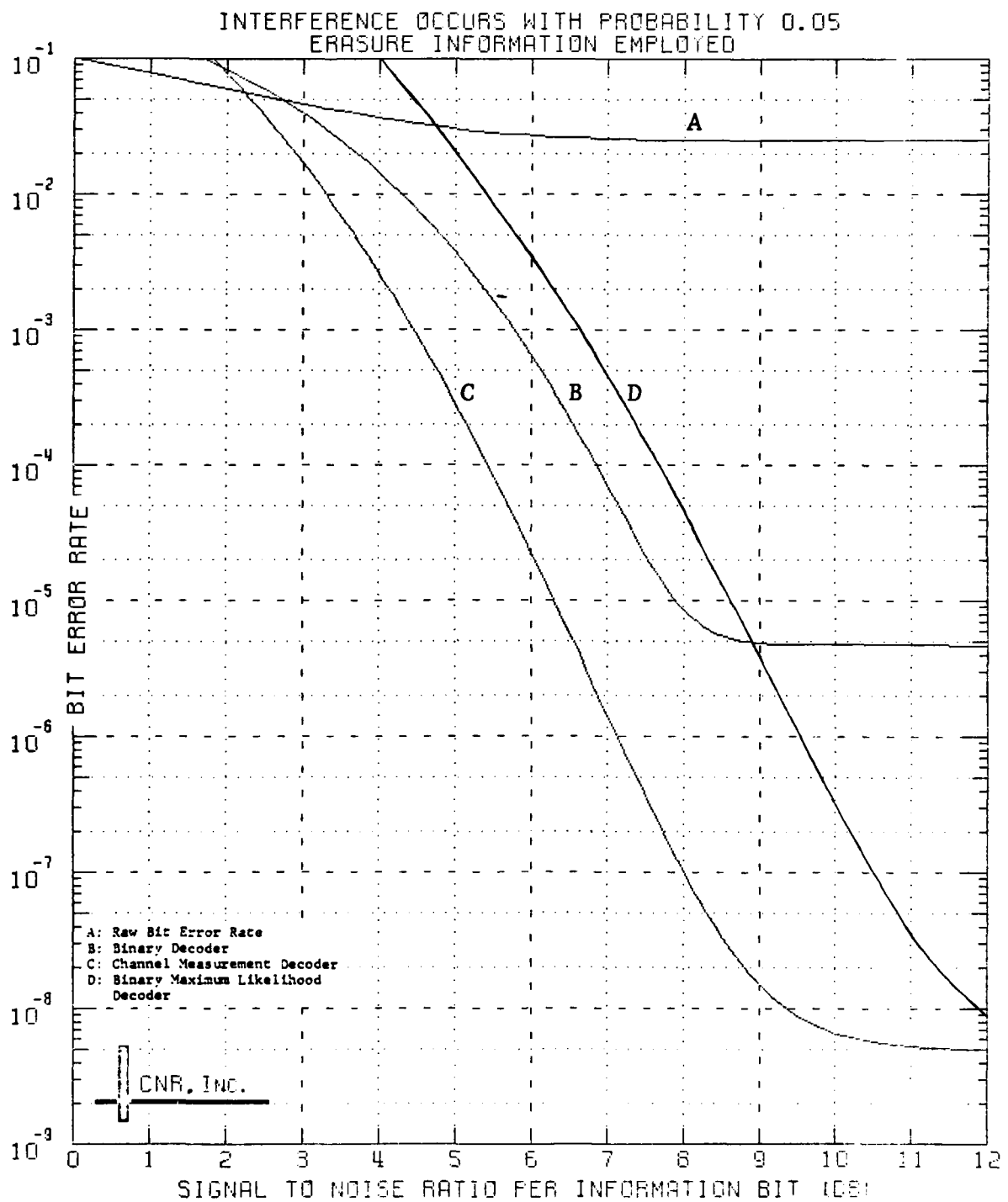
Figure 5.24 Decoded Performance of a Block Code Dimensions (24,12;8)
