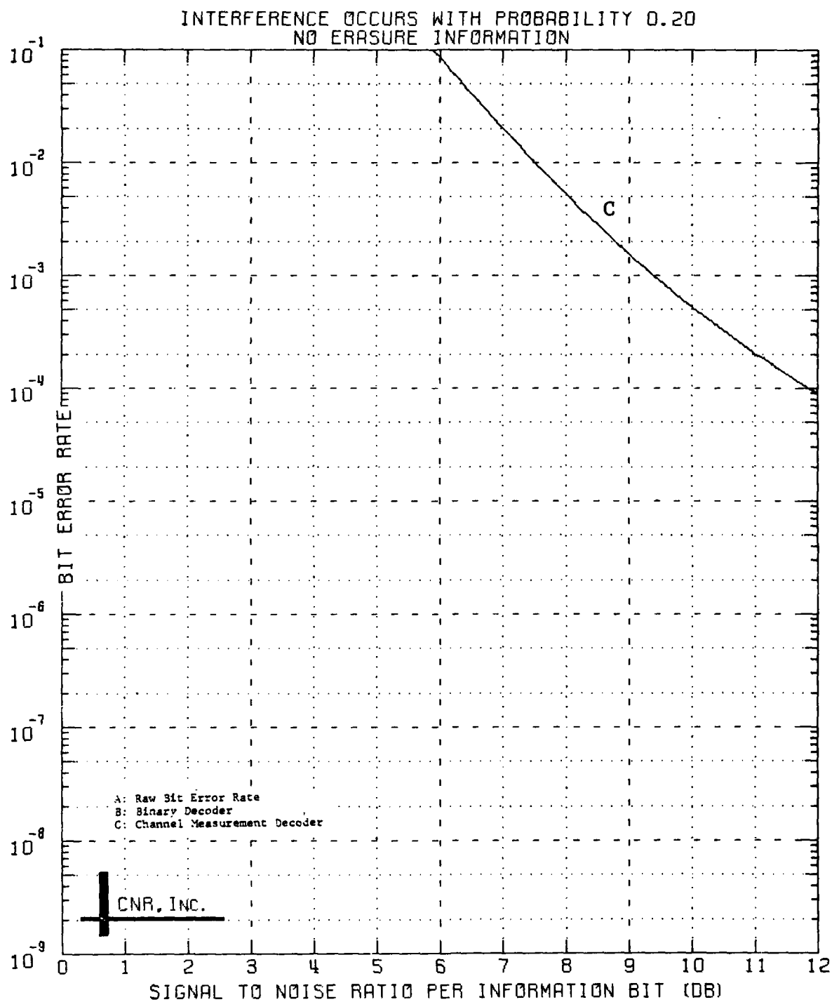
Figure 6.5 Decoded Performance of a Convolutional Code Rate 1/2; Constraint Length = 7
