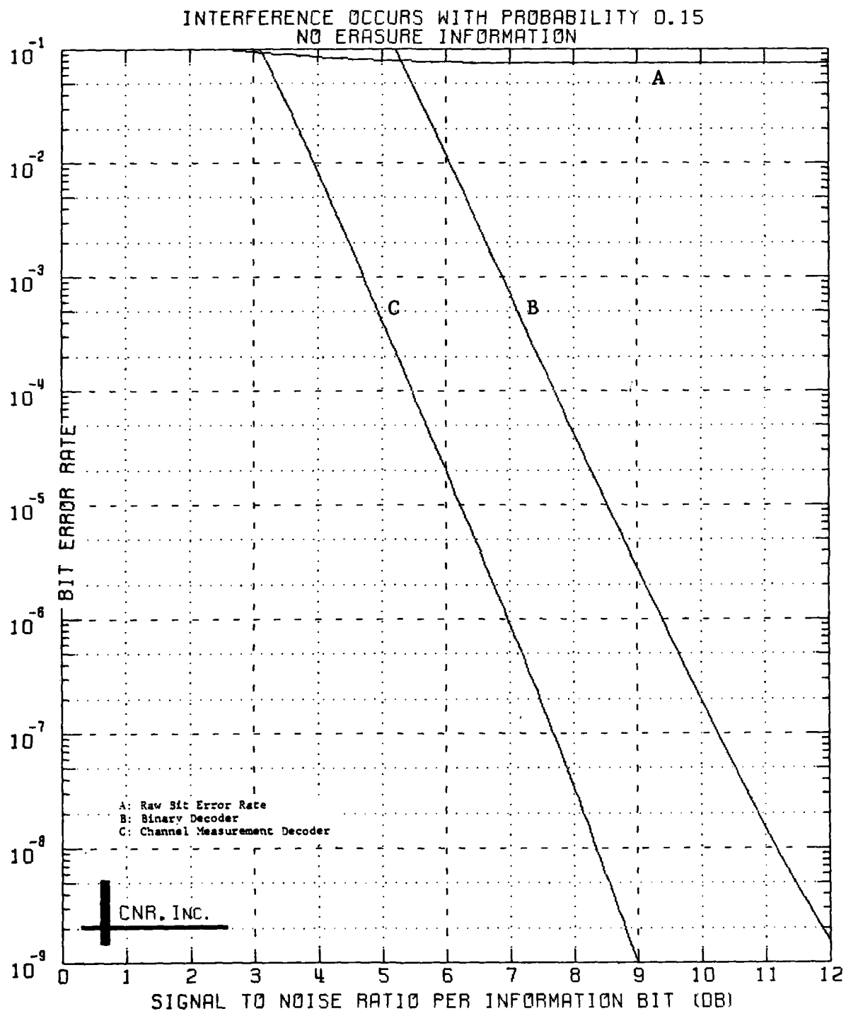
Figure 6.22 Decoded Performance of a Convolutional Code Rate 1/8; Constraint Length = 7
