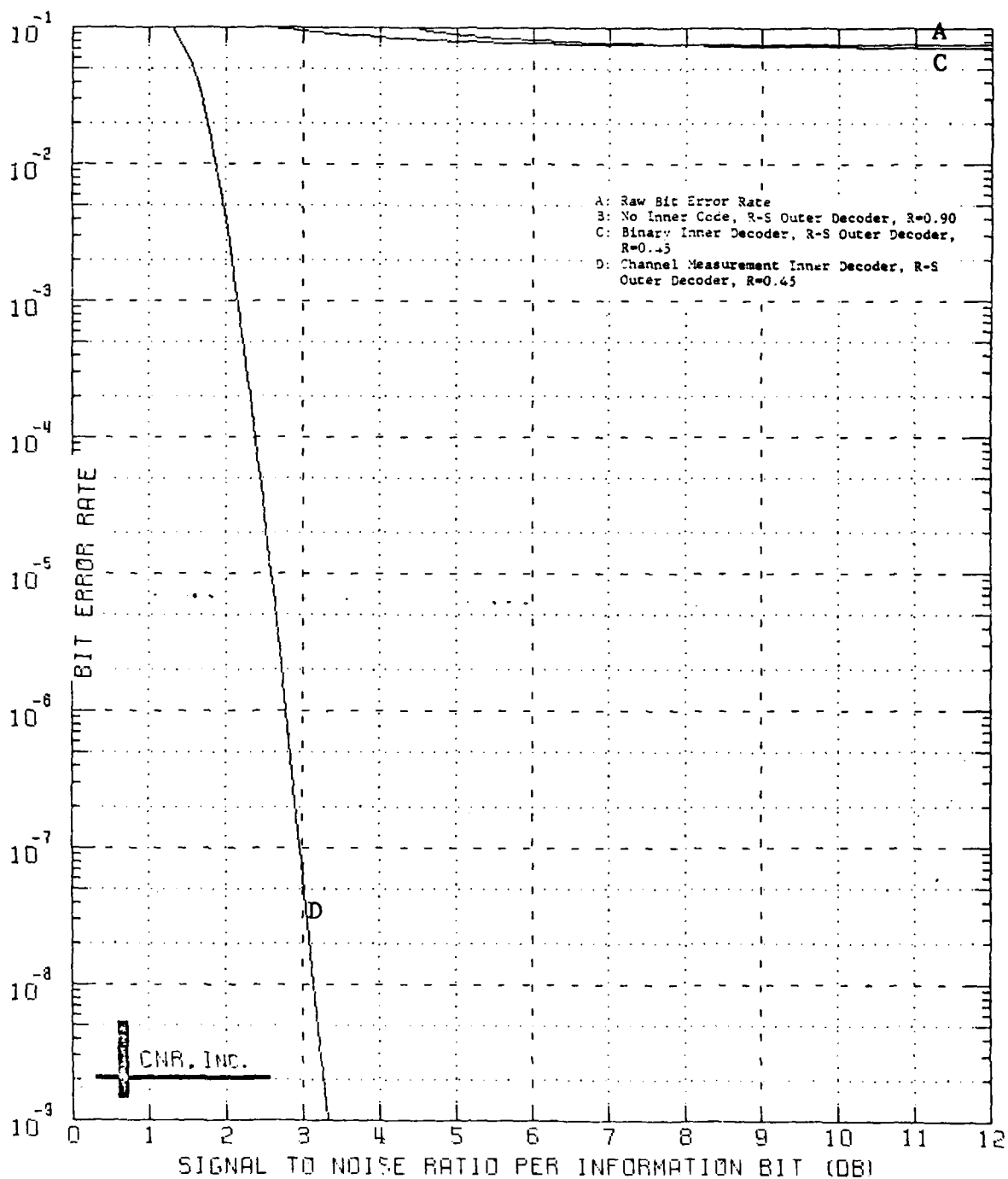
Figure 9.54 Decoded Performance of a Two-Stage Coding Approach Outer Decoder: Reed-Solomon Code (60,54;7) Symbol Interleaver Employed Inner Decoder: Block Code (128,64;22) \delta=0.15 and Erasure Information is Employed
