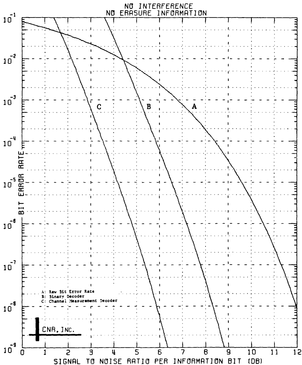
Figure 6.1 Decoded Performance of a Convolutional Code Rate 1/2; Constraint Length = 7
