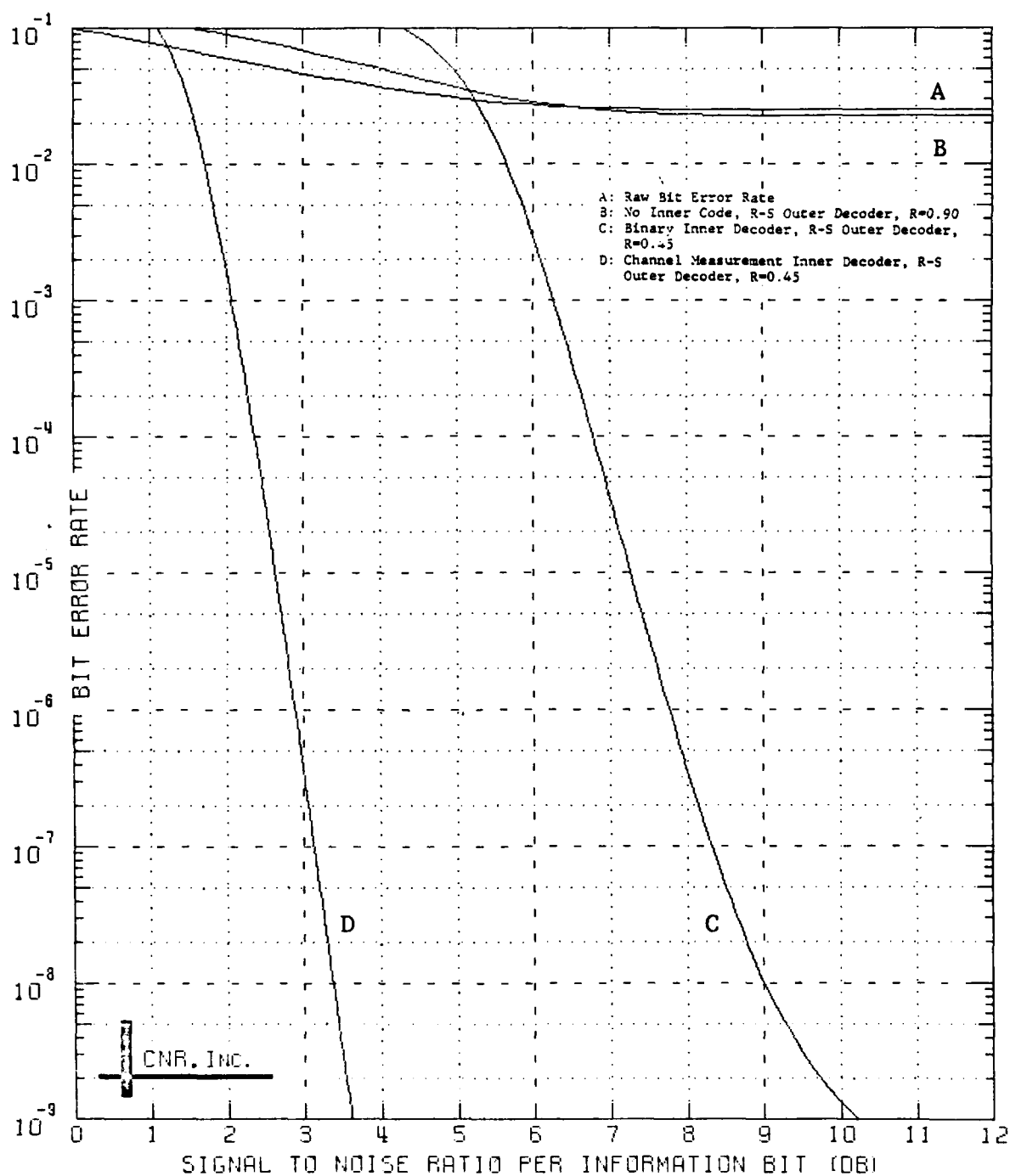
Figure 9.66 Decoded Performance of a Two-Stage Coding Approach Outer Decoder: Reed-Solomon Code (40,36;5) Symbol Interleaver Employed Inner Decoder: Block Code (128,64;22) \delta=0.05 and No Erasure Information Employed
