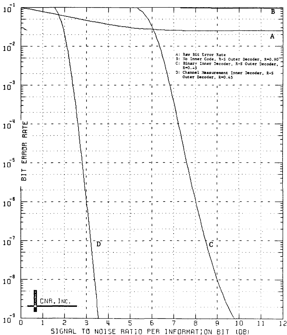
Figure 9.39 Decoded Performance of a Two-Stage Coding Approach Outer Decoder: Reed-Solomon Code (60,54;7) Bit Interleaver Employed Inner Decoder: Block Code (128,64;22) \delta=0.05 and No Erasure Information Employed
