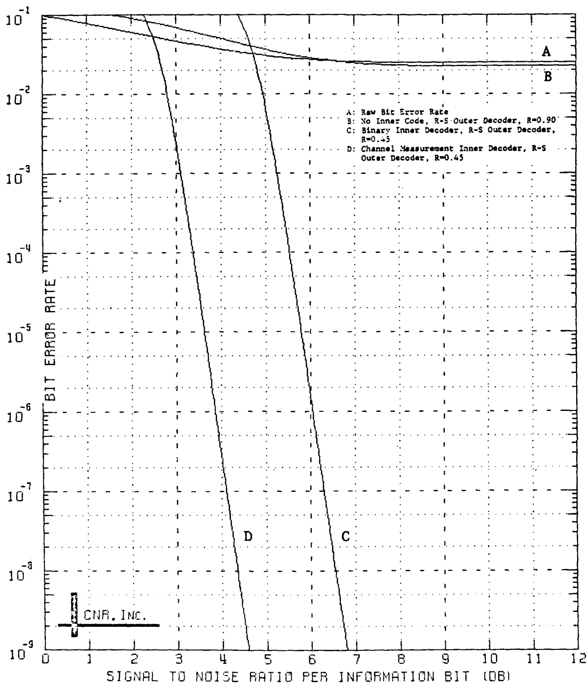
Figure 9.34 Decoded Performance of a Two-Stage Coding Approach Outer Decoder: Reed-Solomon Code (40,36;5) Symbol Interleaver Employed Inner Decoder: Convolutional Code, Rate=1/2; K=7 \delta=0.05 and Erasure Information is Employed
