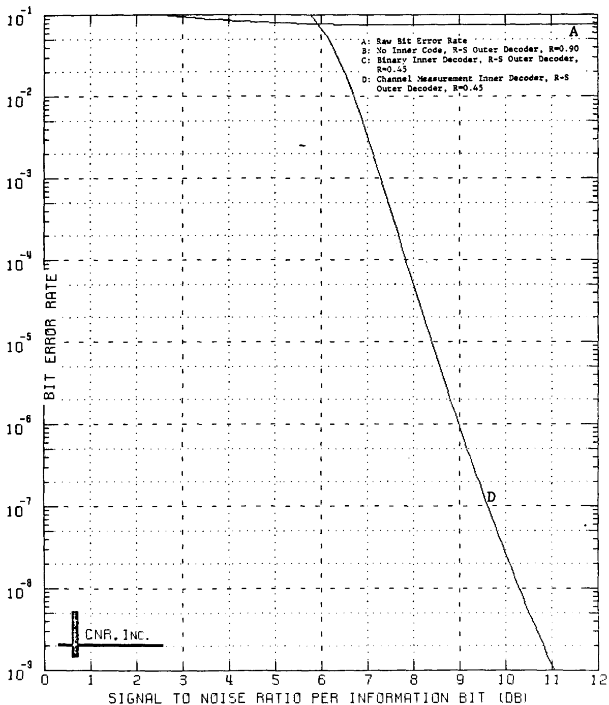
Figure 9.23 Decoded Performance of a Two-Stage Coding Approach Outer Decoder: Reed-Solomon Code (40,36;5) Bit Interleaver Employed Inner Decoder: Convolutional Code, Rate=1/2; K=7 \delta=0.15 and No Erasure Information Employed
