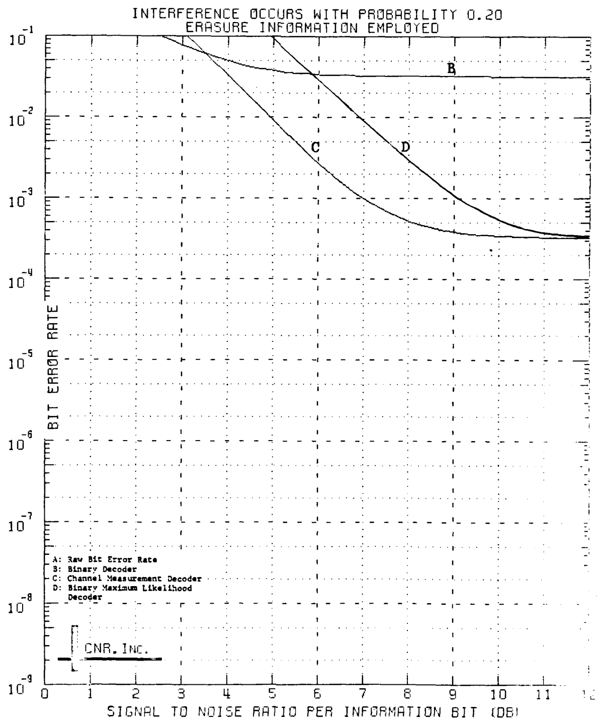
Figure 5.27 Decoded Performance of a Block Code Dimensions (24,12;8)
