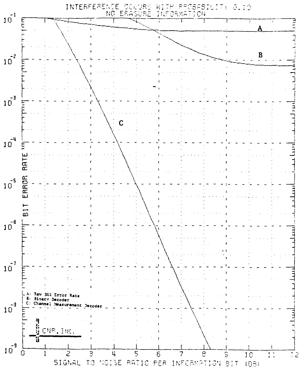
Figure 5.12 Decoded Performance of a Block Code Dimensions (128, 64; 22)
