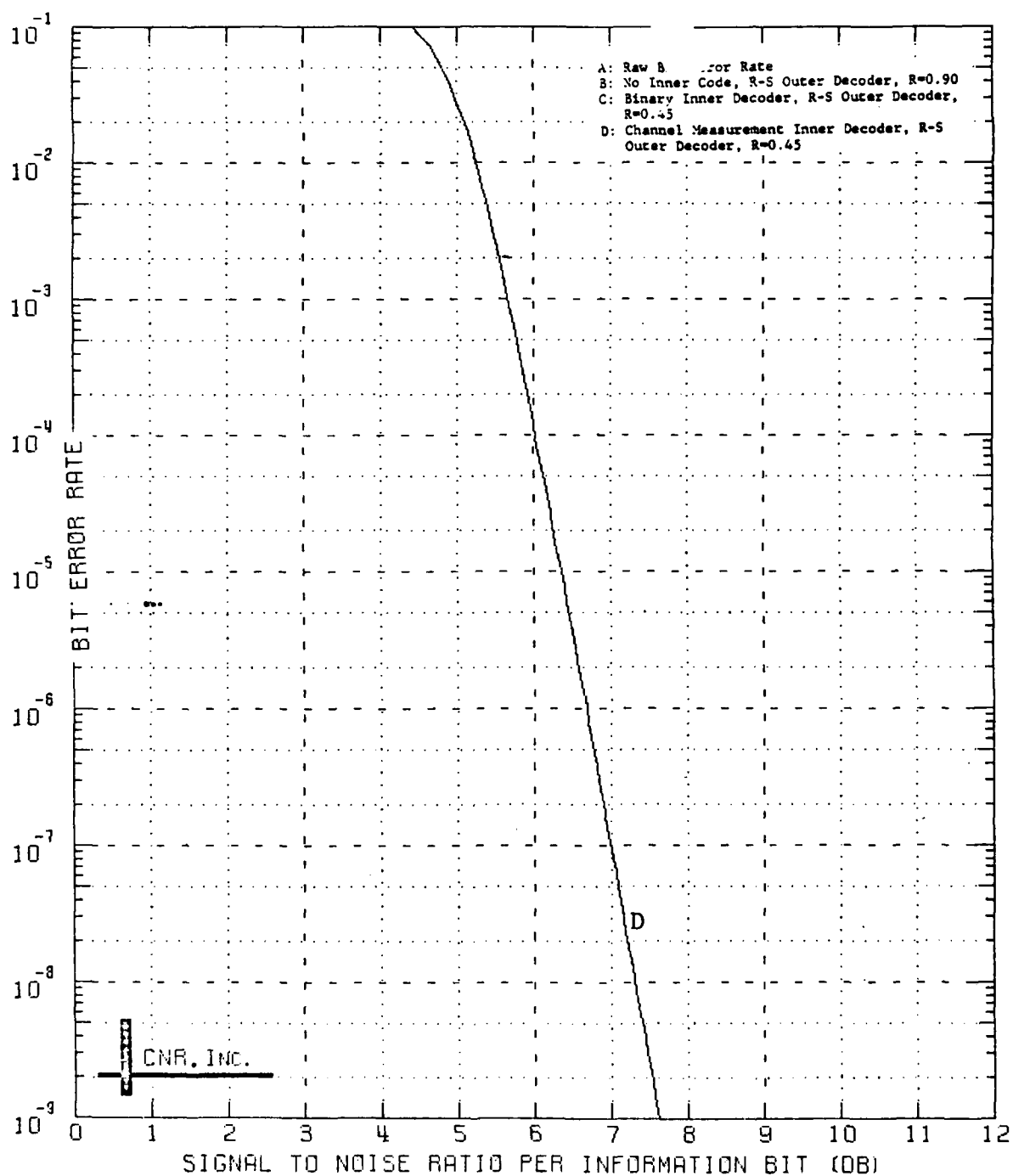
Figure 9.42 Decoded Performance of a Two-Stage Coding Approach Outer Decoder: Reed-Solomon Code (60,54;7) Bit Interleaver Employed Inner Decoder: Block Code (128,64;22) \delta=0.20 and No Erasure Information Employed
