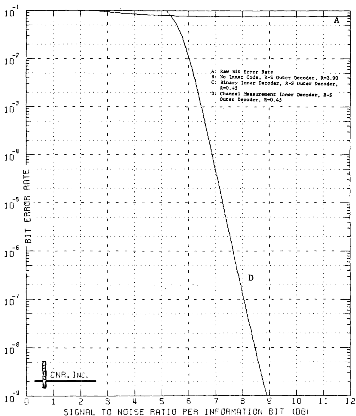
Figure 9.14 Decoded Performance of a Two-Stage Coding Approach Outer Decoder: Reed-Solomon Code (60,54;7) Symbol Interleaver Employed Inner Decoder: Convolutional Code, Rate=1/2; K=7 \delta=0.15 and No Erasure Information Employed
