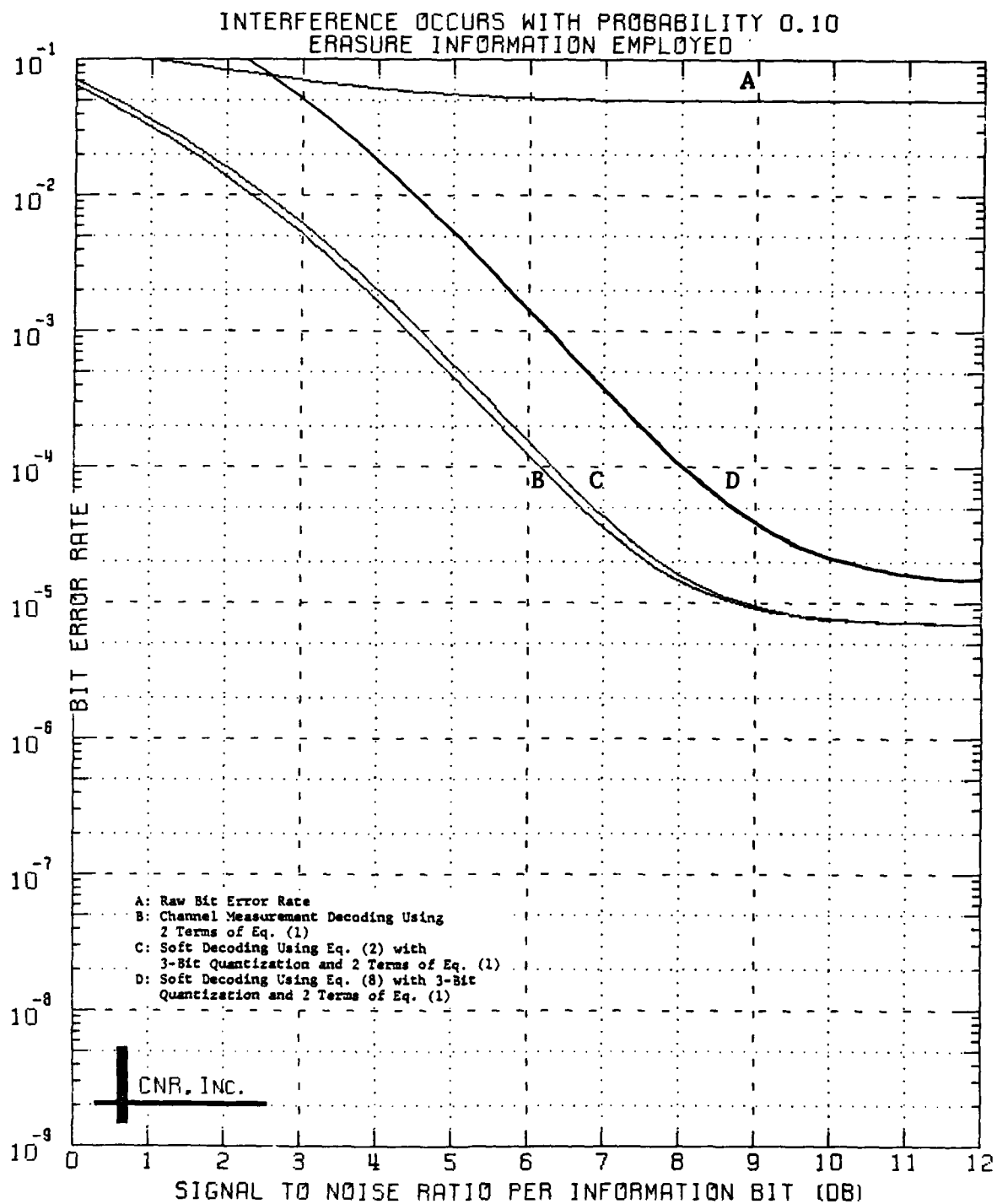
Figure 15 Decoded Performance of a Convolutional Code Rate 1/2; Constraint Length = 3; Gaussian Channel; CPSK Modulation
