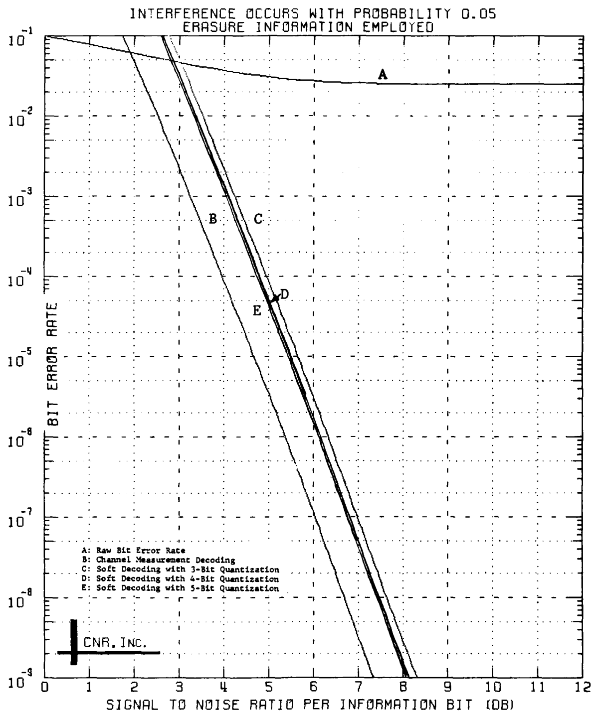
Figure 7 Decoded Performance of a Convolutional Code Rate 1/2; Constraint Length = 7; Gaussian Channel; CPSK Modulation
