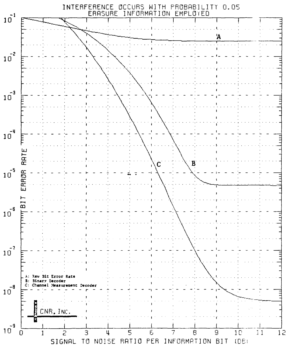
Figure 5.6 Decoded Performance of a Block Code Dimensions (24,12;8)
