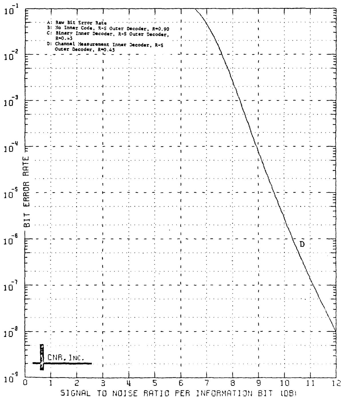
Figure 9.33 Decoded Performance of a Two-Stage Coding Approach Outer Decoder: Reed-Solomon Code (40,36;5) Symbol Interleaver Employed Inner Decoder: Convolutional Code, Rate=1/2; K=7 \delta=0.20 and No Erasure Information Employed
