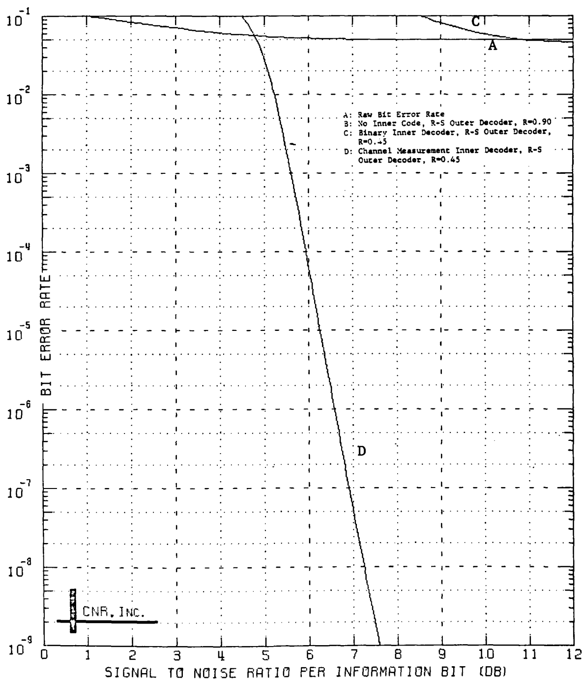
Figure 9.4 Decoded Performance of a Two-Stage Coding Approach Outer Decoder: Reed-Solomon Code (60,54;7) Bit Interleaver Employed Inner Decoder: Convolutional Code, Rate=1/2; K=7 \delta=0.10 and No Erasure Information Employed
