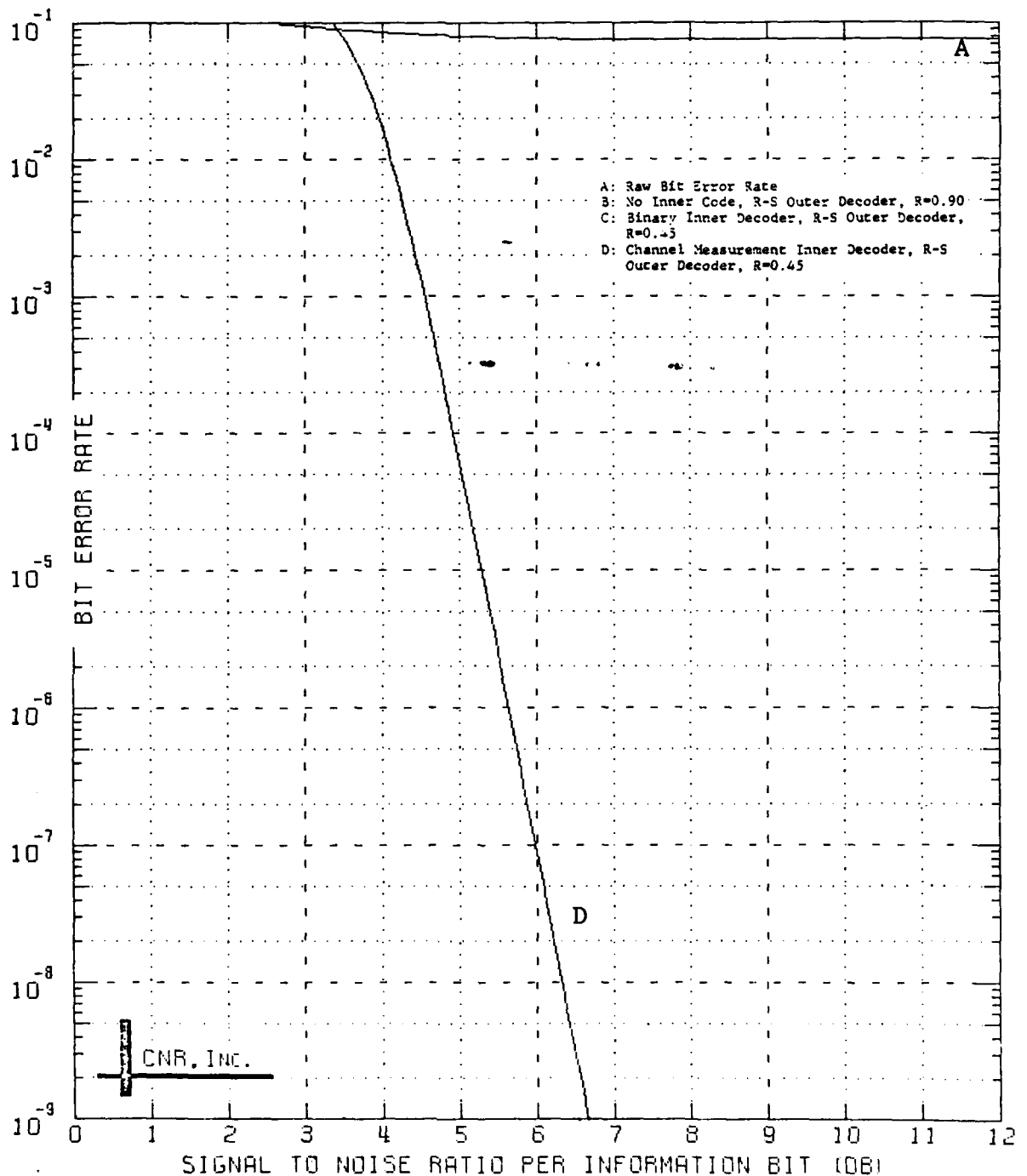
Figure 9.59 Decoded Performance of a Two-Stage Coding Approach Outer Decoder: Reed-Solomon Code (40,36;5) Bit Interleaver Employed Inner Decoder: Block Code (128,64;22) \delta=0.15 and No Erasure Information Employed
