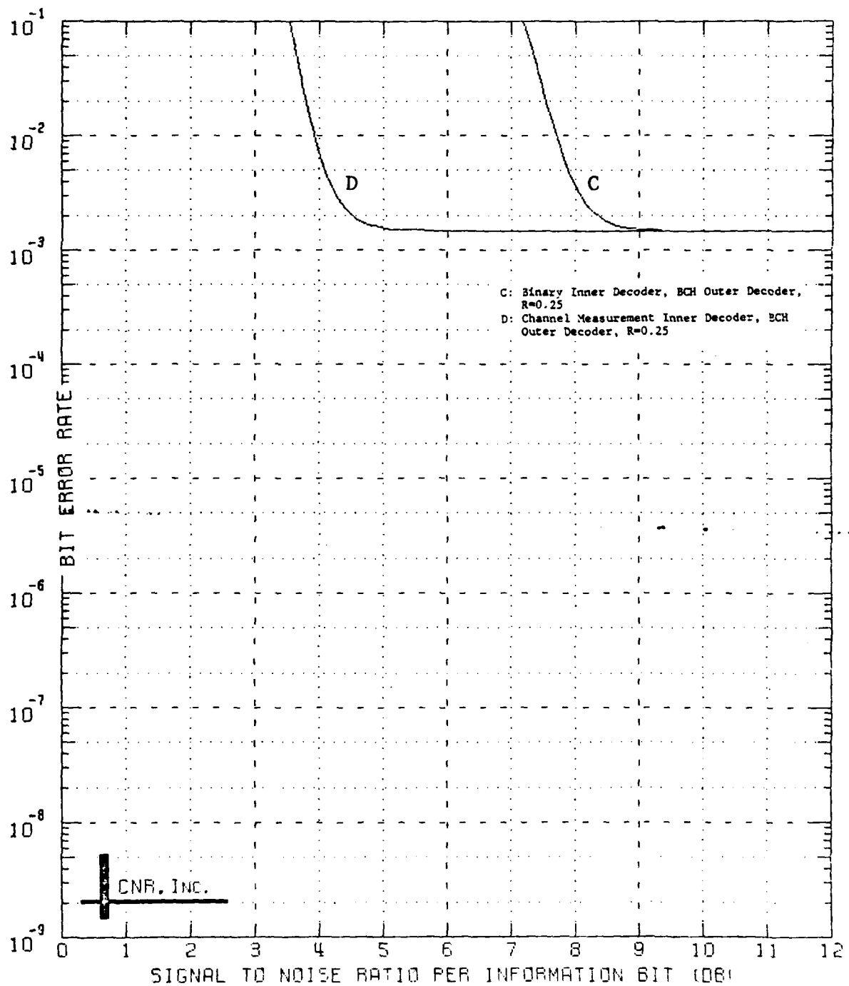
Figure 7.23 Decoded Performance of a Two-Stage Coding Approach Adaptive Technique Outer Decoder: BCH Code (128,64;22) Inner Decoder: Block Code (128,64;22) \delta=0.10 and No Erasure Information Employed
