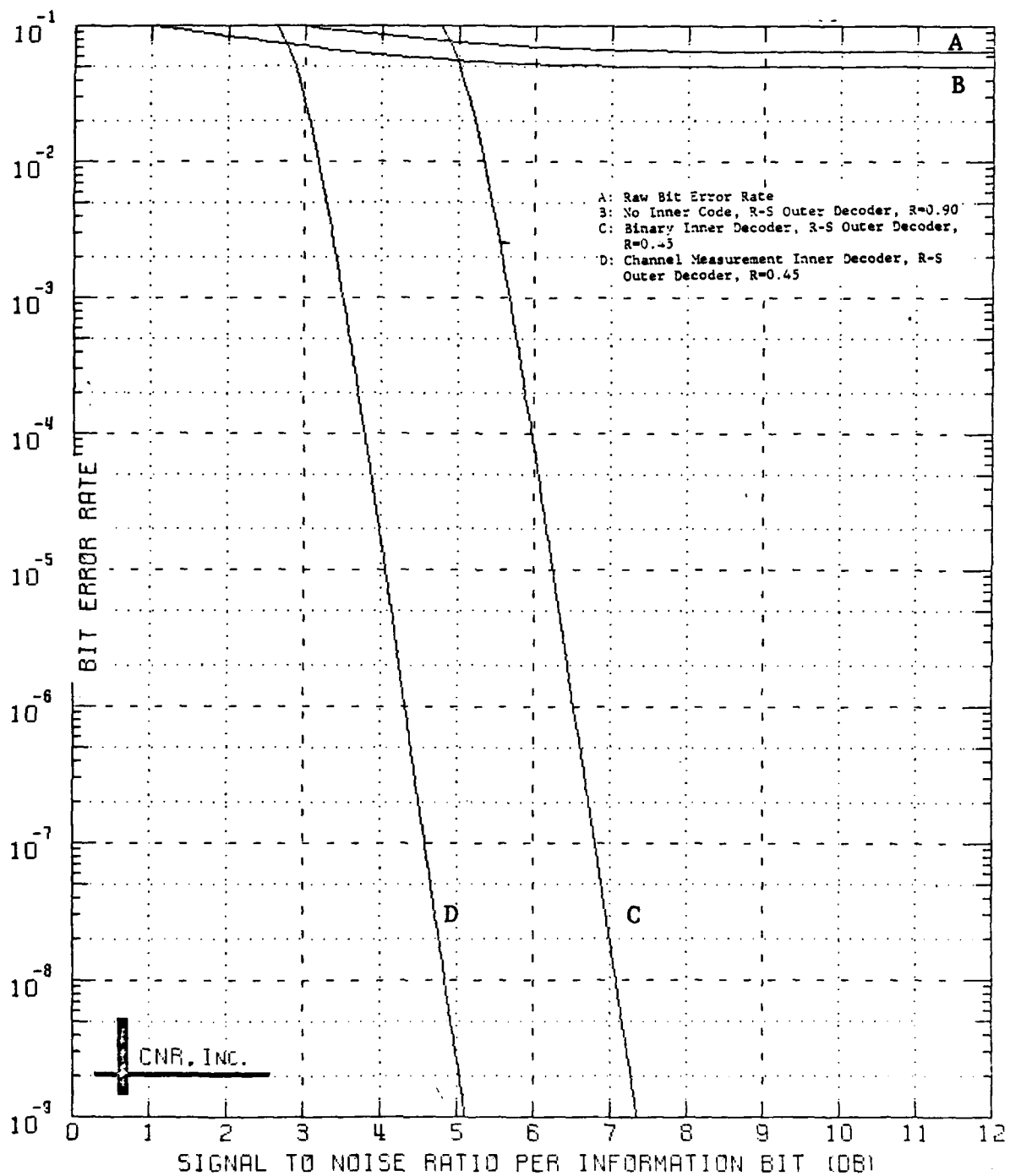
Figure 9.35 Decoded Performance of a Two-Stage Coding Approach Outer Decoder: Reed-Solomon Code (40,36;5) Symbol Interleaver Employed Inner Decoder: Convolutional Code, Rate=1/2; K=7 \delta=0.10 and Erasure Information is Employed
