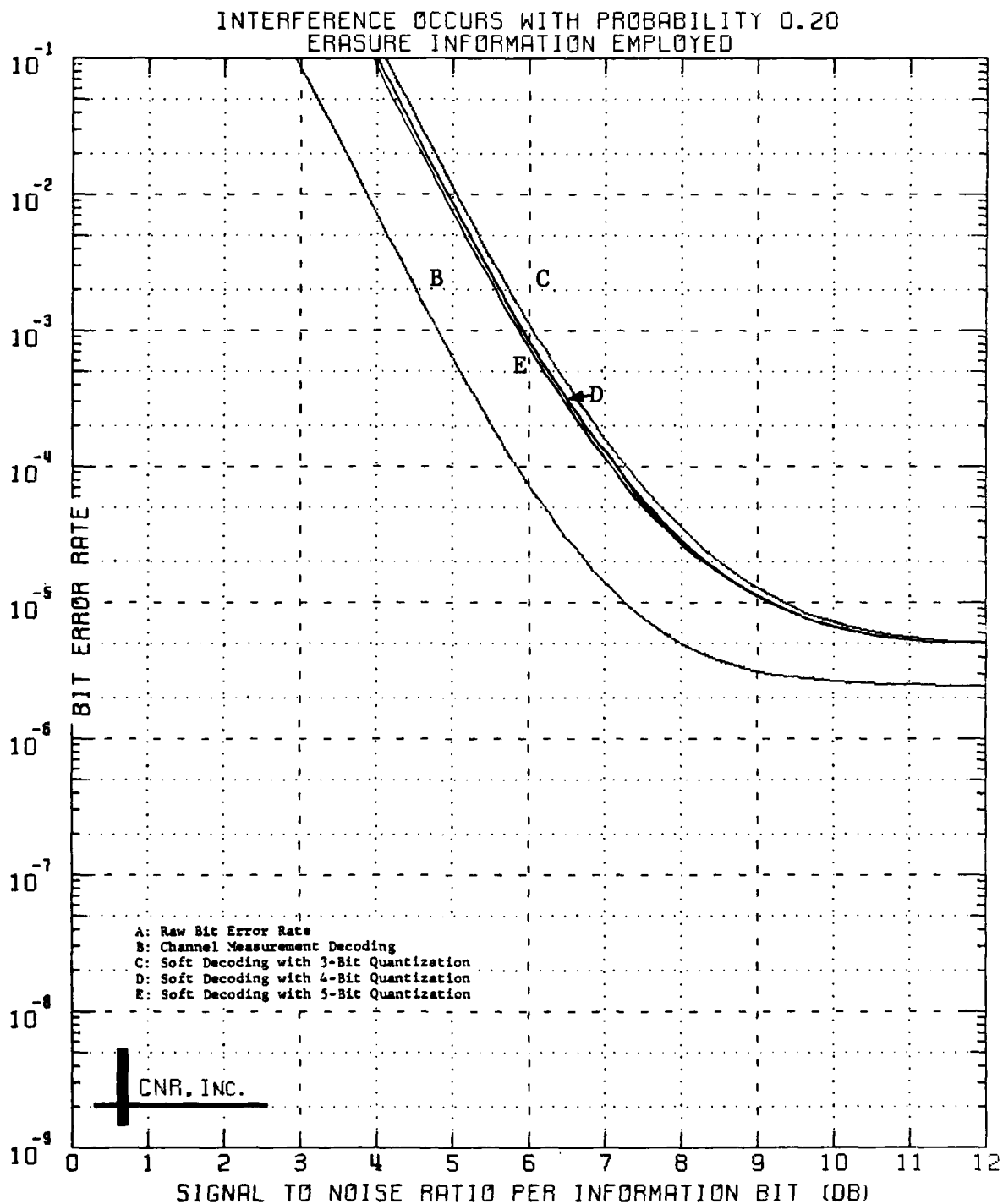
Figure 10 Decoded Performance of a Convolutional Code Rate 1/2; Constraint Length = 7; Gaussian Channel; CPSK Modulation
