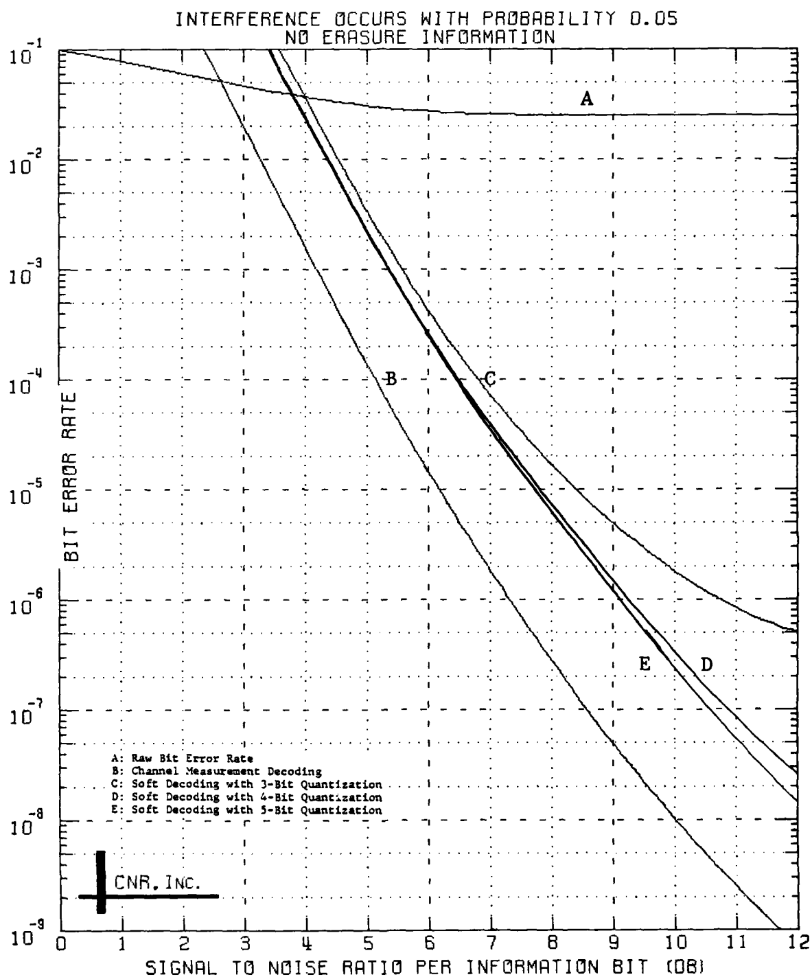
Figure 3 Decoded Performance of a Convolutional Code Rate 1/2; Constraint Length = 7; Gaussian Channel; CPSK Modulation
