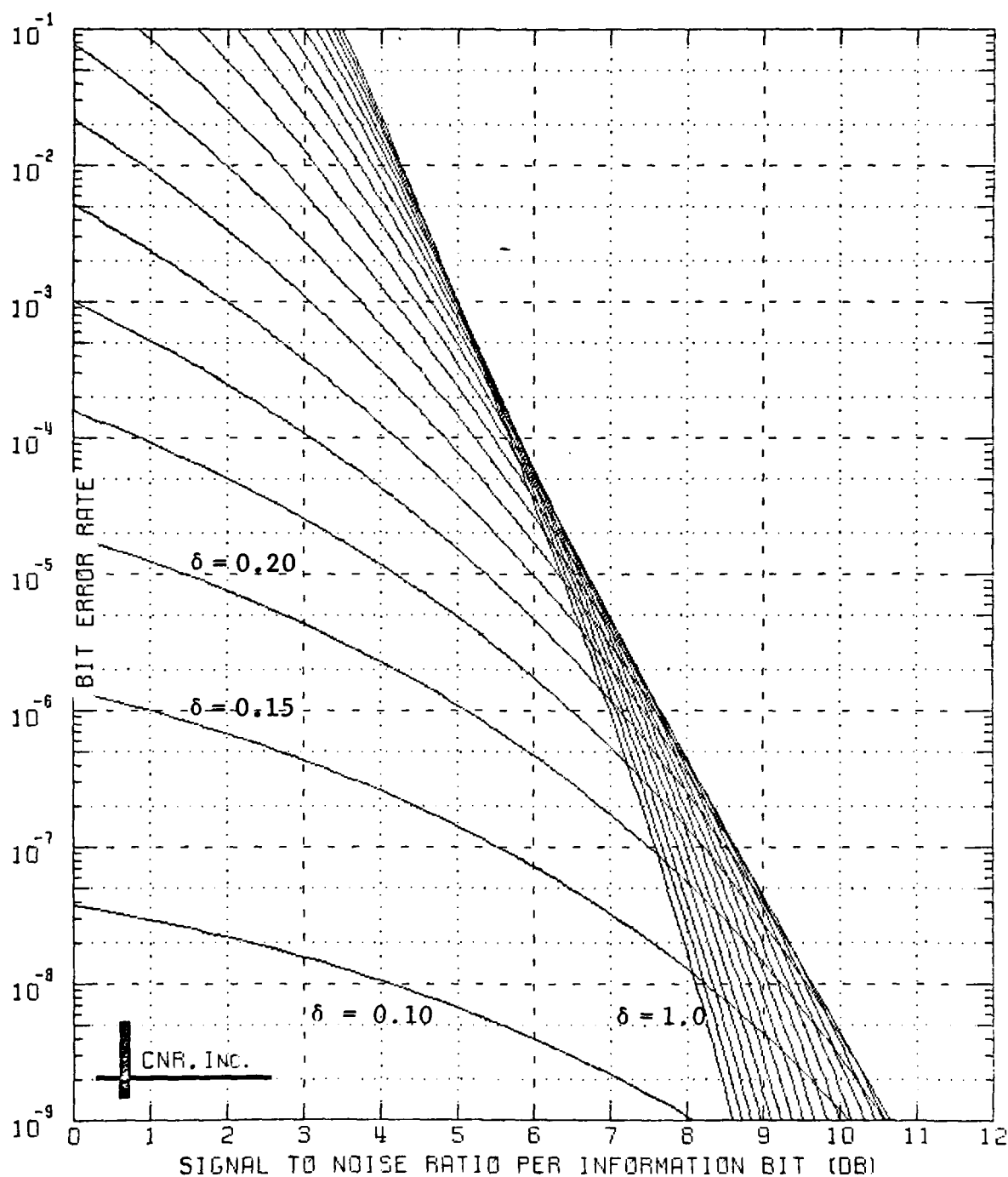
Figure 2 Rate-1/4, K=7, Binary-Decoding, Average Power-Limited Pulse Jammer Model
