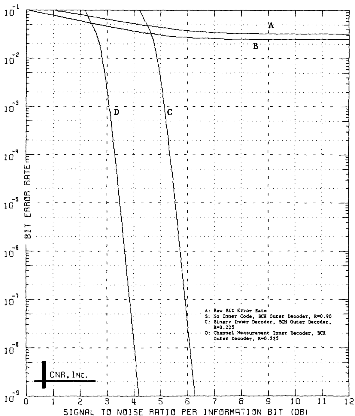
Figure 8.15 Decoded Performance of a Two-Stage Coding Approach Outer Decoder: BCH Code (240,216;7) Inner Decoder: Convolutional Code; Rate=1/4; K=7 \delta=0.05 and Erasure Information is Employed
