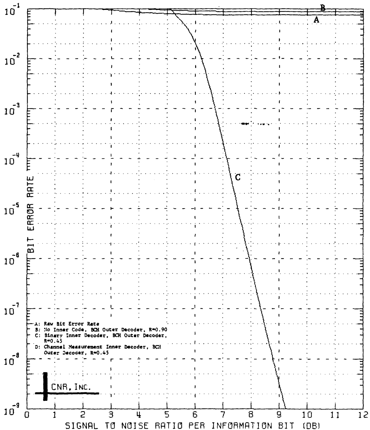
Figure 8.4 Decoded Performance of a Two-Stage Coding Approach Outer Decoder: BCH Code (240,216;7) Inner Decoder: Convolutional Code; Rate=1/2; K=7 \delta=0.15 and No Erasure Information Employed
