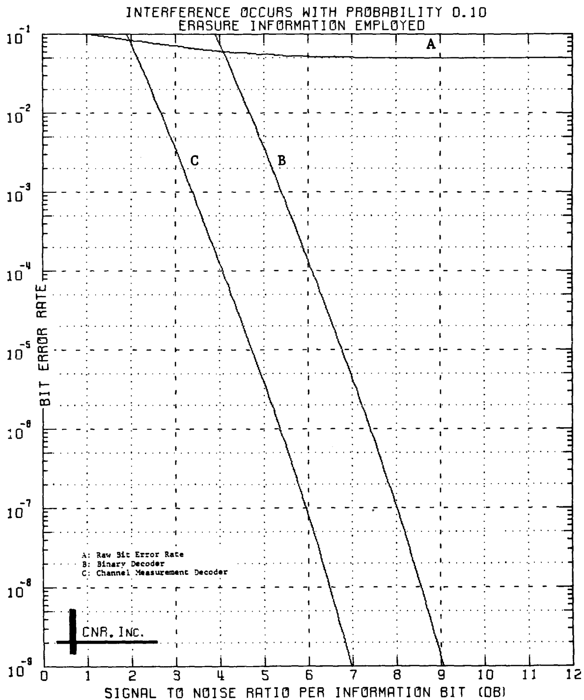
Figure 6.25 Decoded Performance of a Convolutional Code Rate 1/8; Constraint Length = 7
