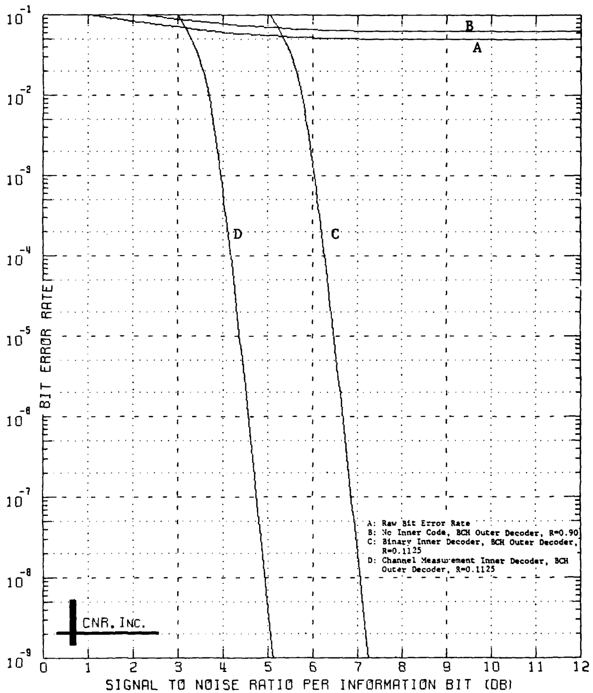
Figure 8.21 Decoded Performance of a Two-Stage Coding Approach Outer Decoder: BCH Code (240,216;7) Inner Decoder: Convolutional Code; Rate=1/8; K=7 \delta=0.10 and No Erasure Information Employed
