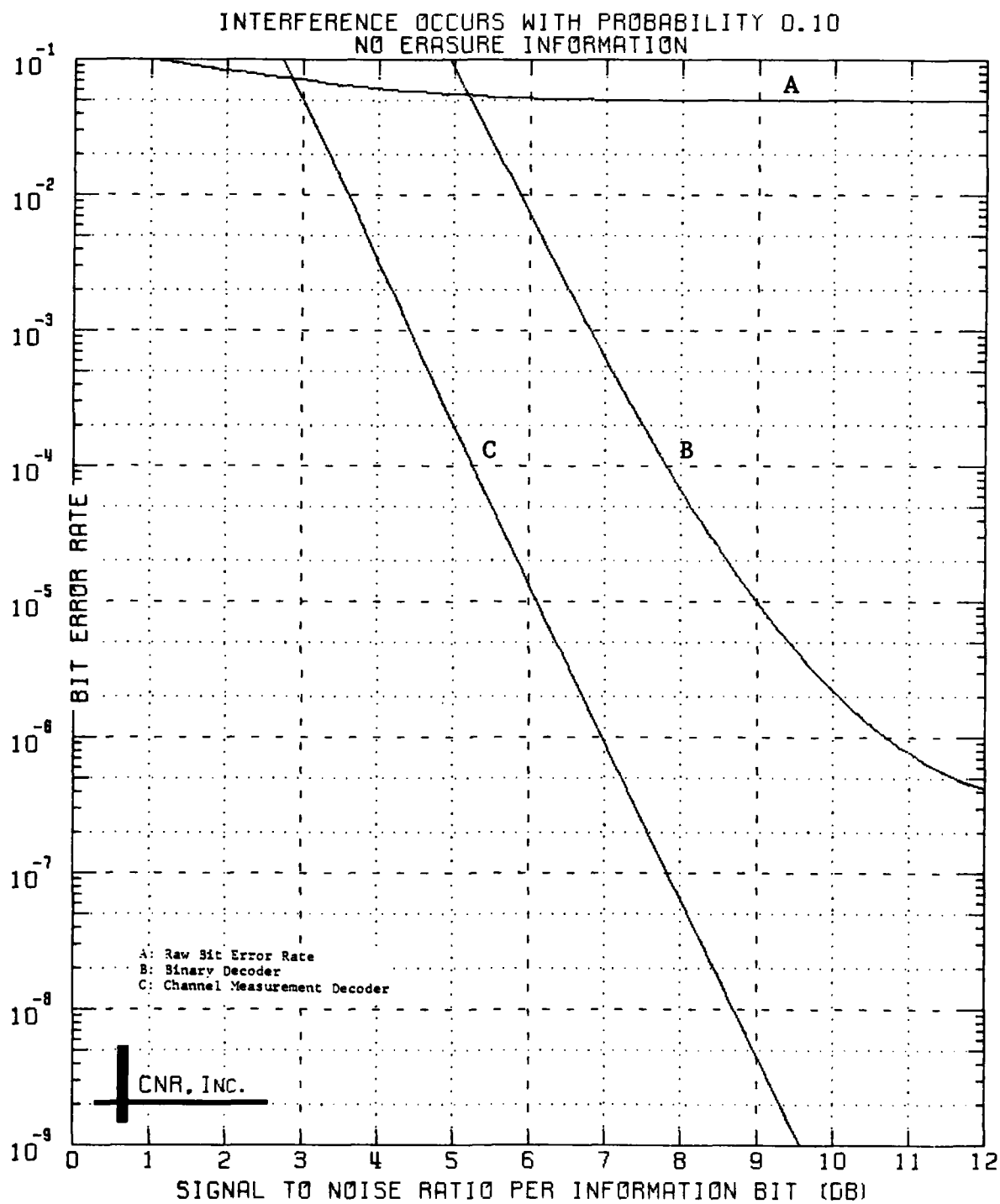
Figure 6.12 Decoded Performance of a Convolutional Code Rate 1/4; Constraint Length = 7
