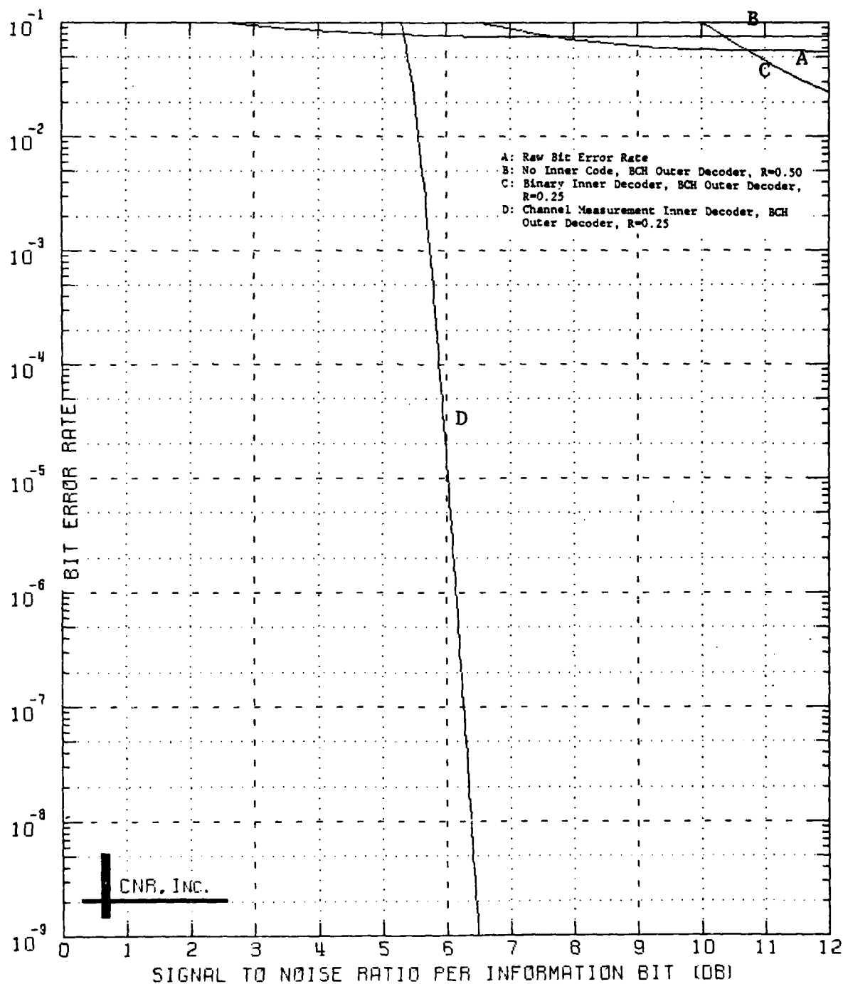
Figure 7.13 Decoded Performance of a Two-Stage Coding Approach Outer Decoder: BCH Code (128,64;22) Inner Decoder: Block Code (128,64;22) \delta=0.15 and No Erasure Information Employed
