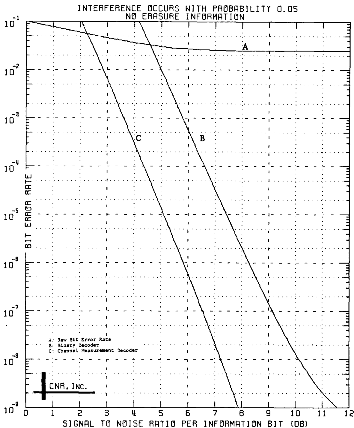
Figure 6.11 Decoded Performance of a Convolutional Code Rate 1/4; Constraint Length = 7
