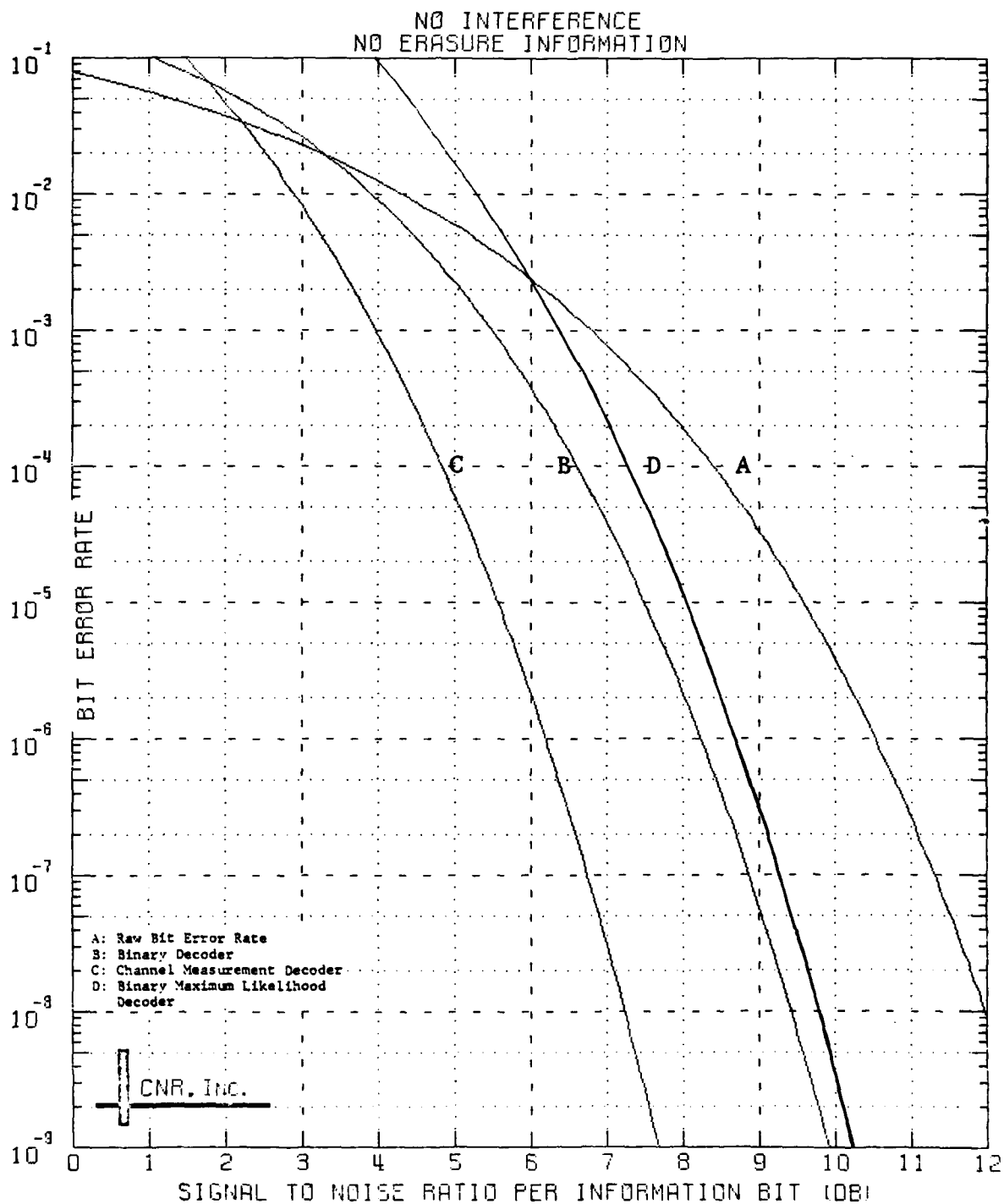
Figure 5.19 Decoded Performance of a Block Code Dimensions (24,12;8)
