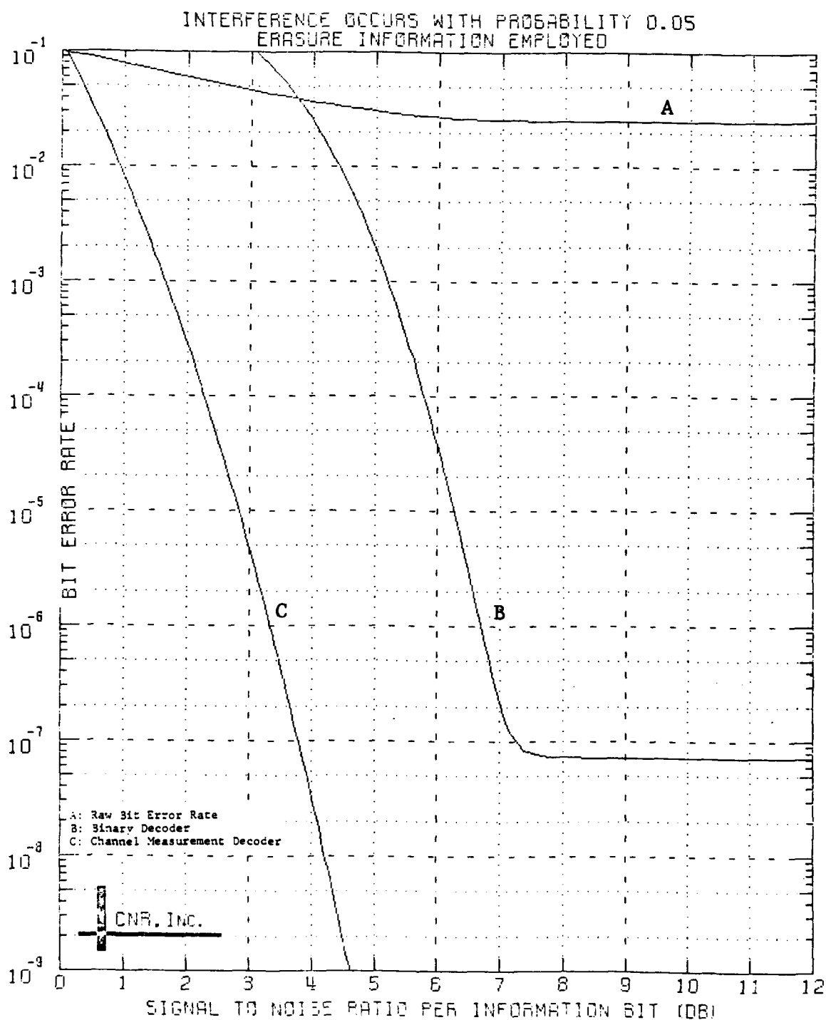
Figure 5.15 Decoded Performance of a Block Code Dimensions (128,64;22)
