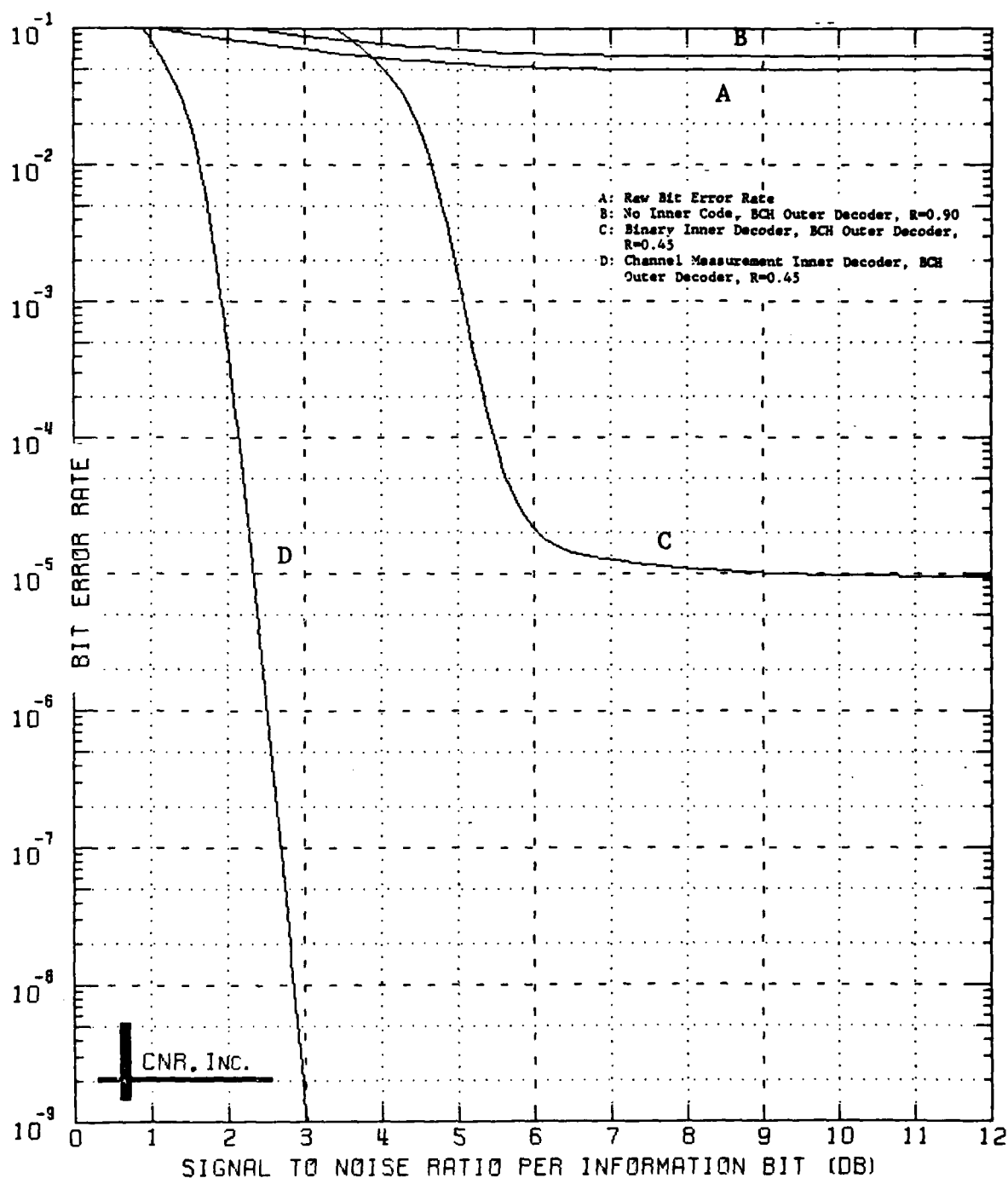
Figure 7.7 Decoded Performance of a Two-Stage Coding Approach Outer Decoder: BCH Code (240,216;7) Inner Decoder: Block Code (128,64;22) \delta=0.10 and Erasure Information is Employed
