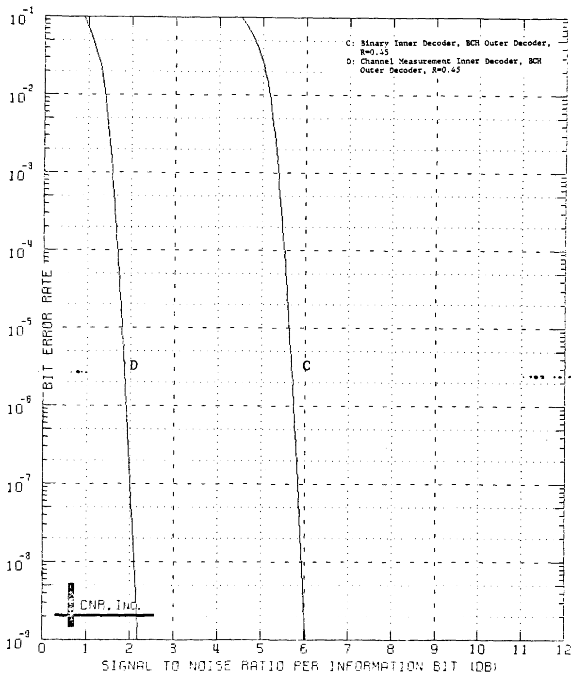
Figure 7.19 Decoded Performance of a Two-Stage Coding Approach Adaptive Technique Outer Decoder: BCH Code (240,216;7) Inner Decoder: Block Code (128,64;22) \delta=0.00 and No Erasure Information Employed
