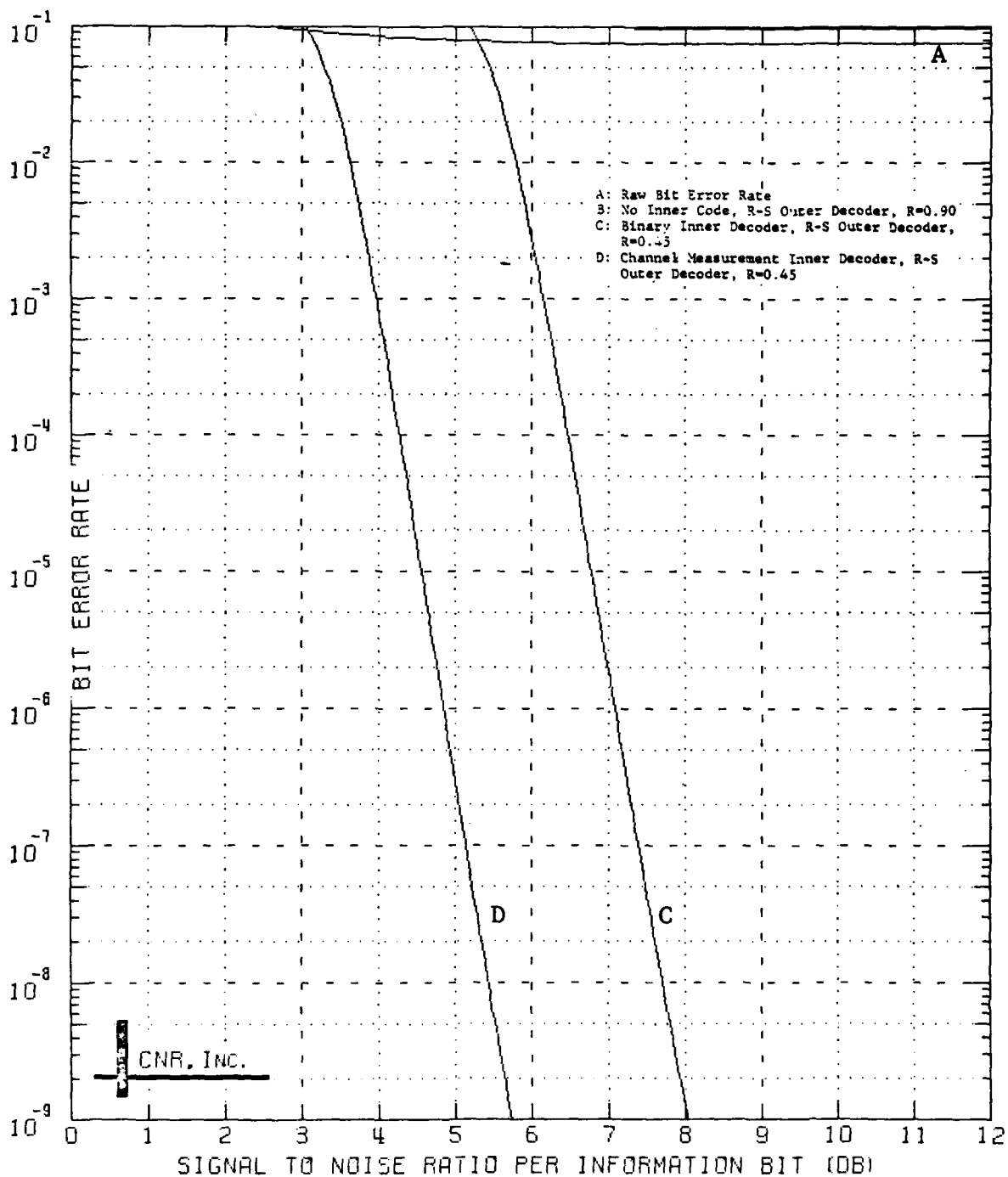
Figure 9.36 Decoded Performance of a Two-Stage Coding Approach Outer Decoder: Reed-Solomon Code (40,36;5) Symbol Interleaver Employed Inner Decoder: Convolutional Code, Rate=1/2; K=7 \delta=0.15 and Erasure Information is Employed
