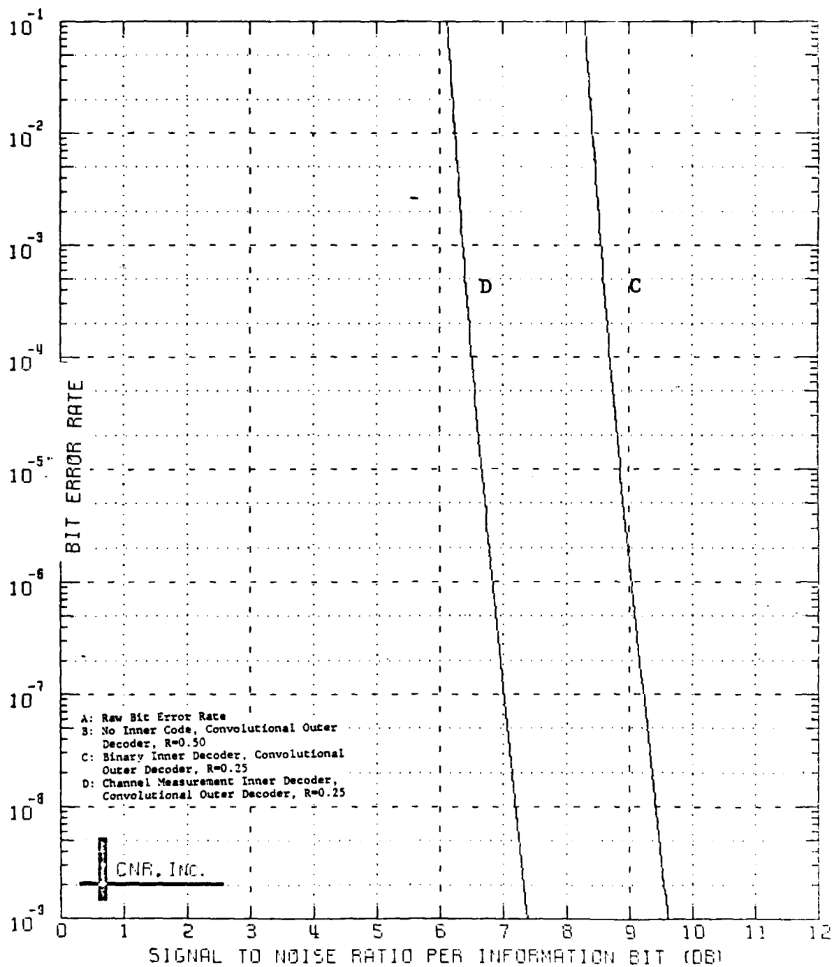
Figure 8.36 Decoded Performance of a Two-Stage Coding Approach Outer Decoder: Convolutional Code, Rate=1/2; K=7 Inner Decoder: Convolutional Code, Rate=1/2; K=7 \delta=0.20 and Erasure Information is Employed
