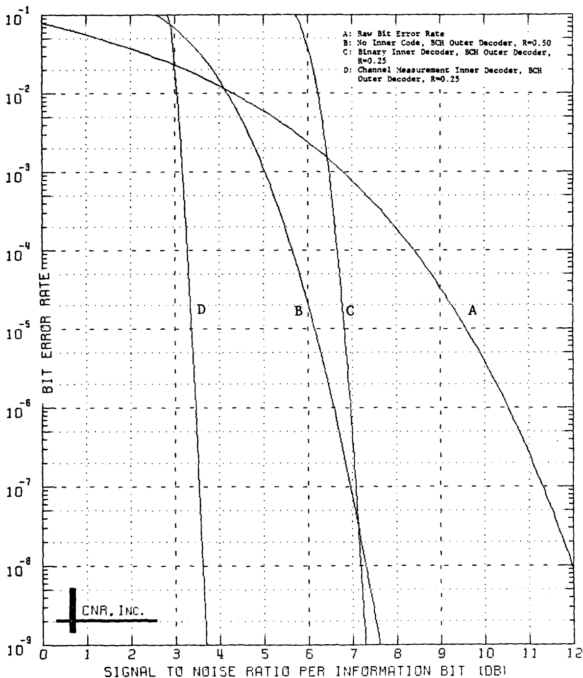
Figure 7.10 Decoded Performance of a Two-Stage Coding Approach Outer Decoder: BCH Code (128,64;22) Inner Decoder: Block Code (128,64;22) \delta=0.00 and No Erasure Information Employed
