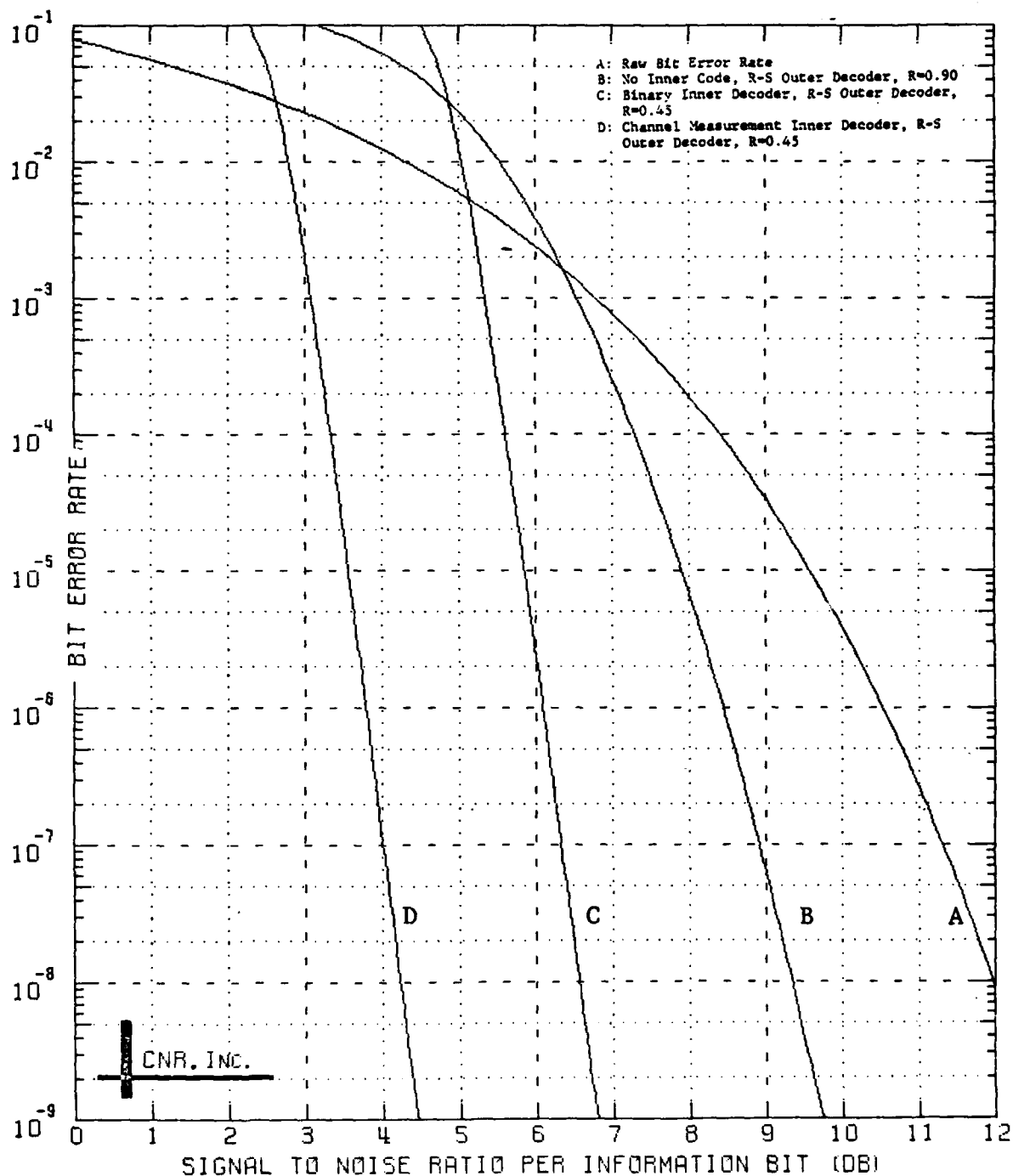
Figure 9.20 Decoded Performance of a Two-Stage Coding Approach Outer Decoder: Reed-Solomon Code (40,36;5) Bit Interleaver Employed Inner Decoder: Convolutional Code, Rate=1/2; K=7 \delta=0.00 and No Erasure Information Employed
