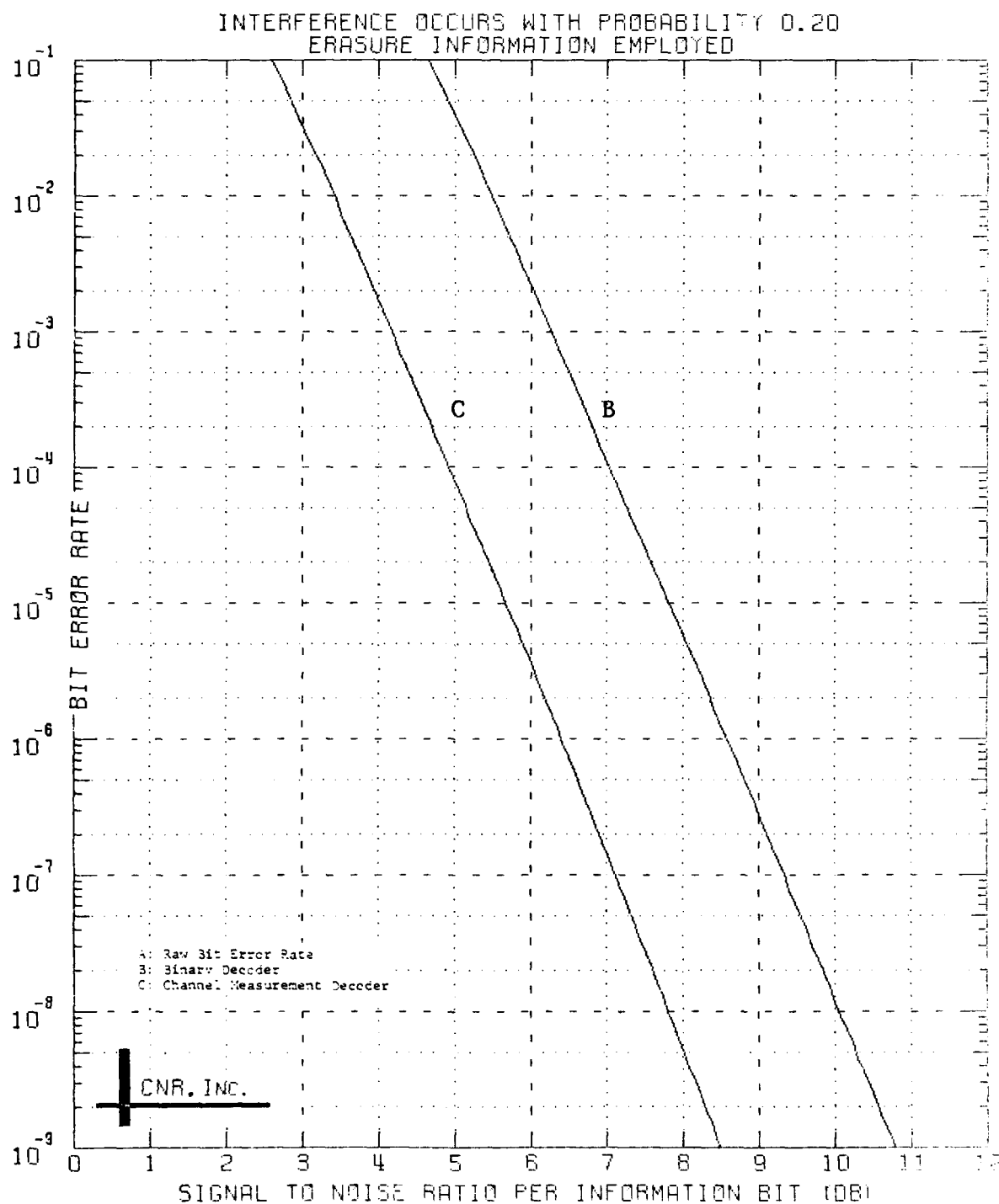
Figure 6.18 Decoded Performance of a Convolutional Code Rate 1/4; Constraint Length = 7
