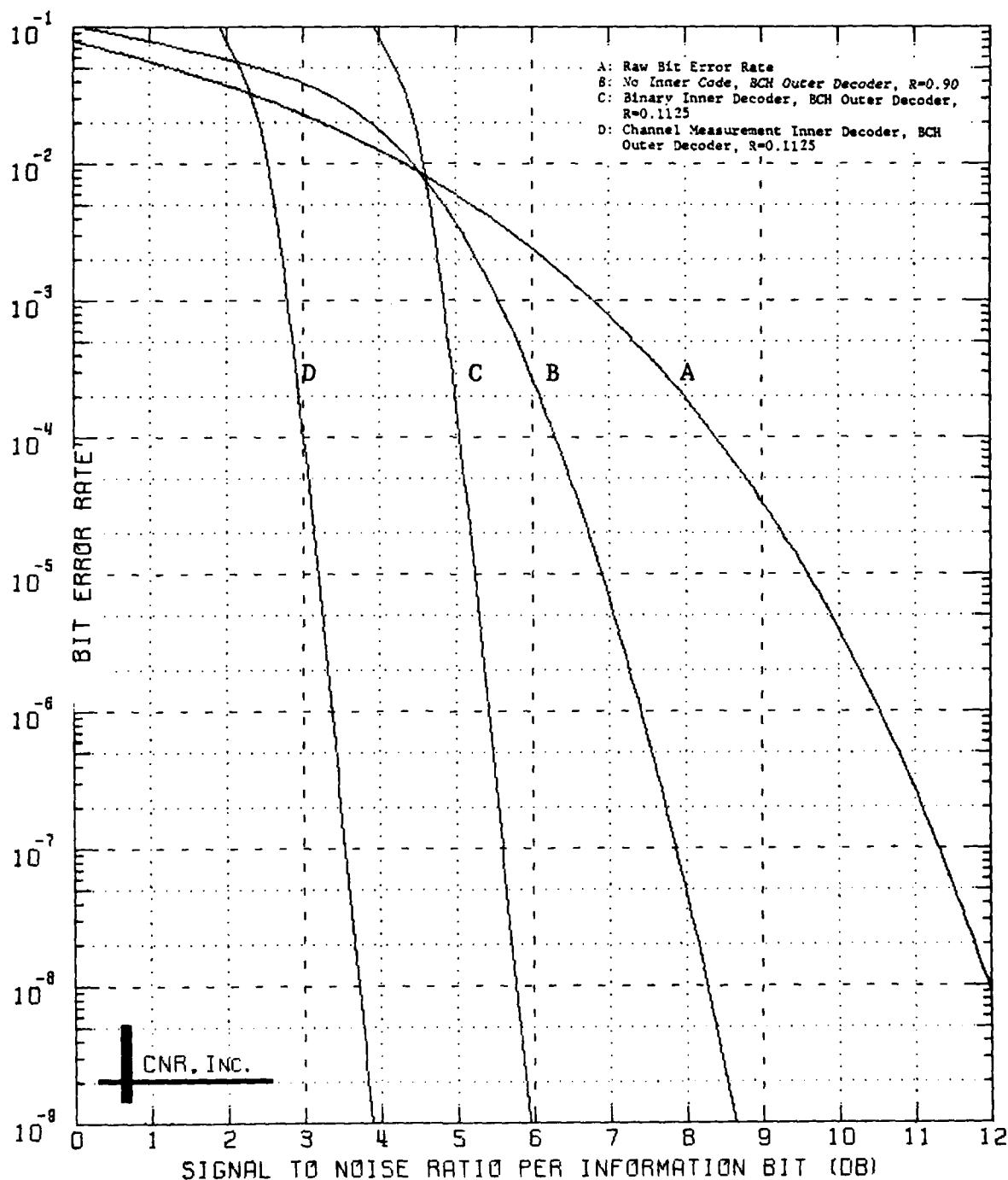
Figure 8.19 Decoded Performance of a Two-Stage Coding Approach Outer Decoder: BCH Code (240,216;7) Inner Decoder: Convolutional Code; Rate=1/8; K=7 \delta=0.00 and No Erasure Information Employed
