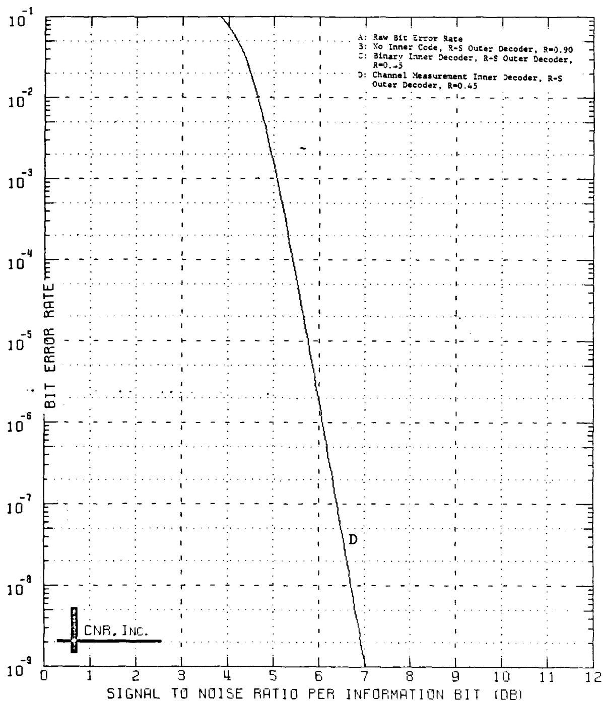
Figure 9.51 Decoded Performance of a Two-Stage Coding Approach Outer Decoder: Reed-Solomon Code (60,54;7) Symbol Interleaver Employed Inner Decoder: Block Code (128,64;22) \delta=0.20 and No Erasure Information Employed
