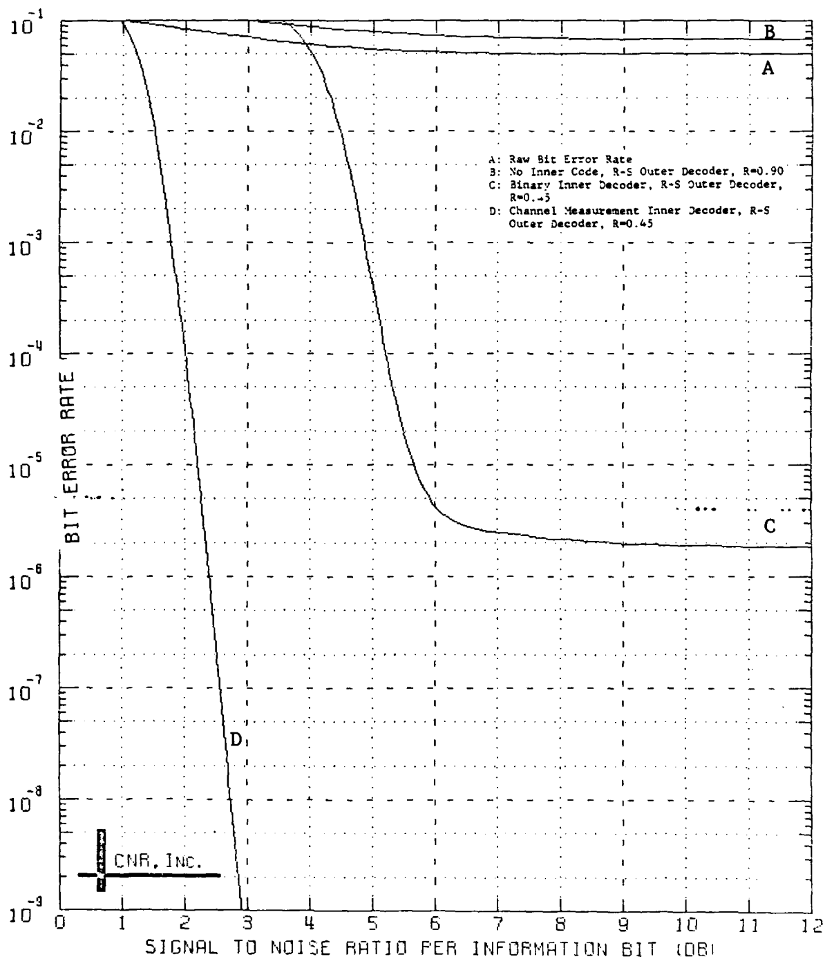
Figure 9.53 Decoded Performance of a Two-Stage Coding Approach Outer Decoder: Reed-Solomon Code (60,54;7) Symbol Interleaver Employed Inner Decoder: Block Code (128,64;22) \delta=0.10 and Erasure Information is Employed
