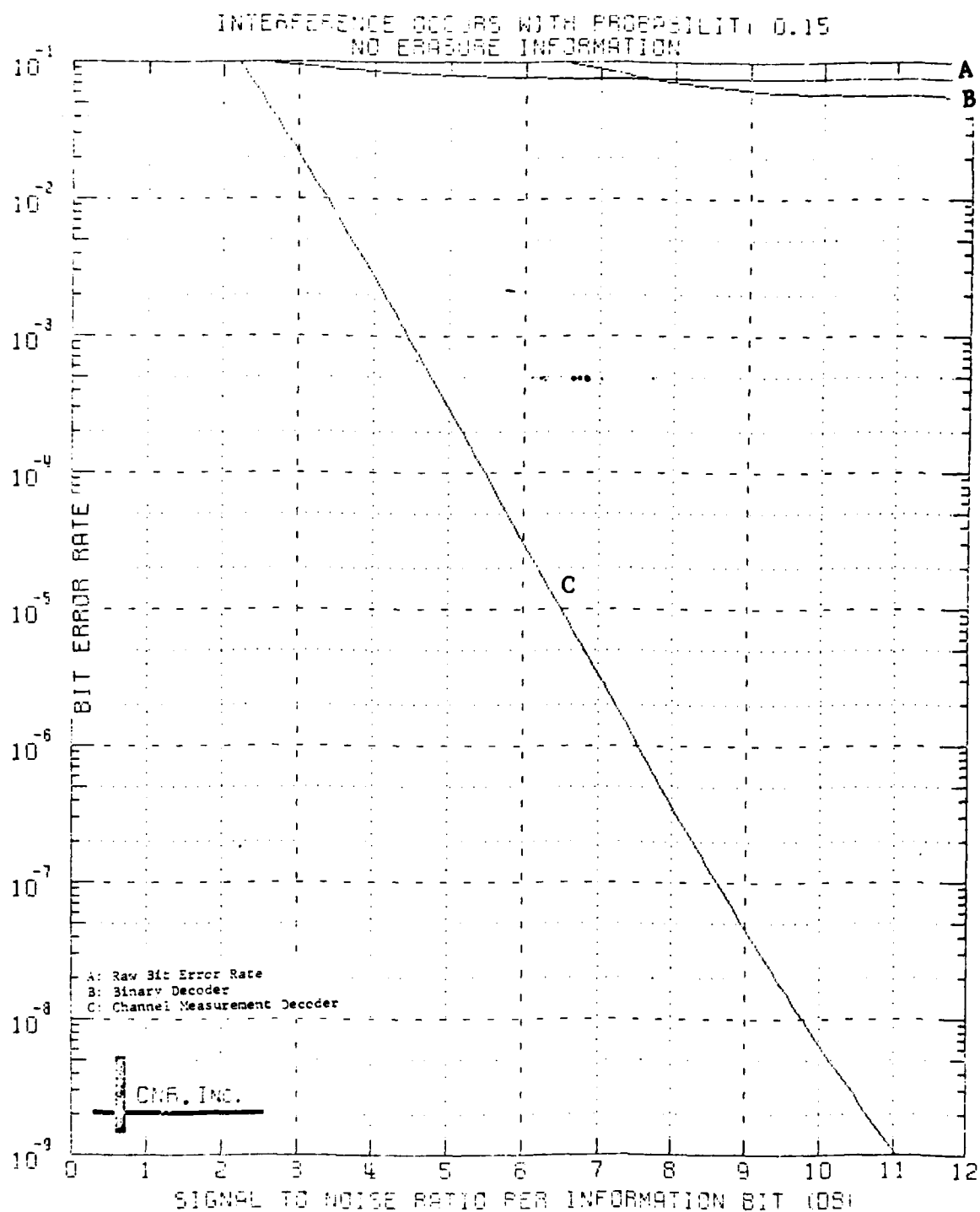
Figure 5.13 Decoded Performance of a Block Code Dimensions (128,64;22)
