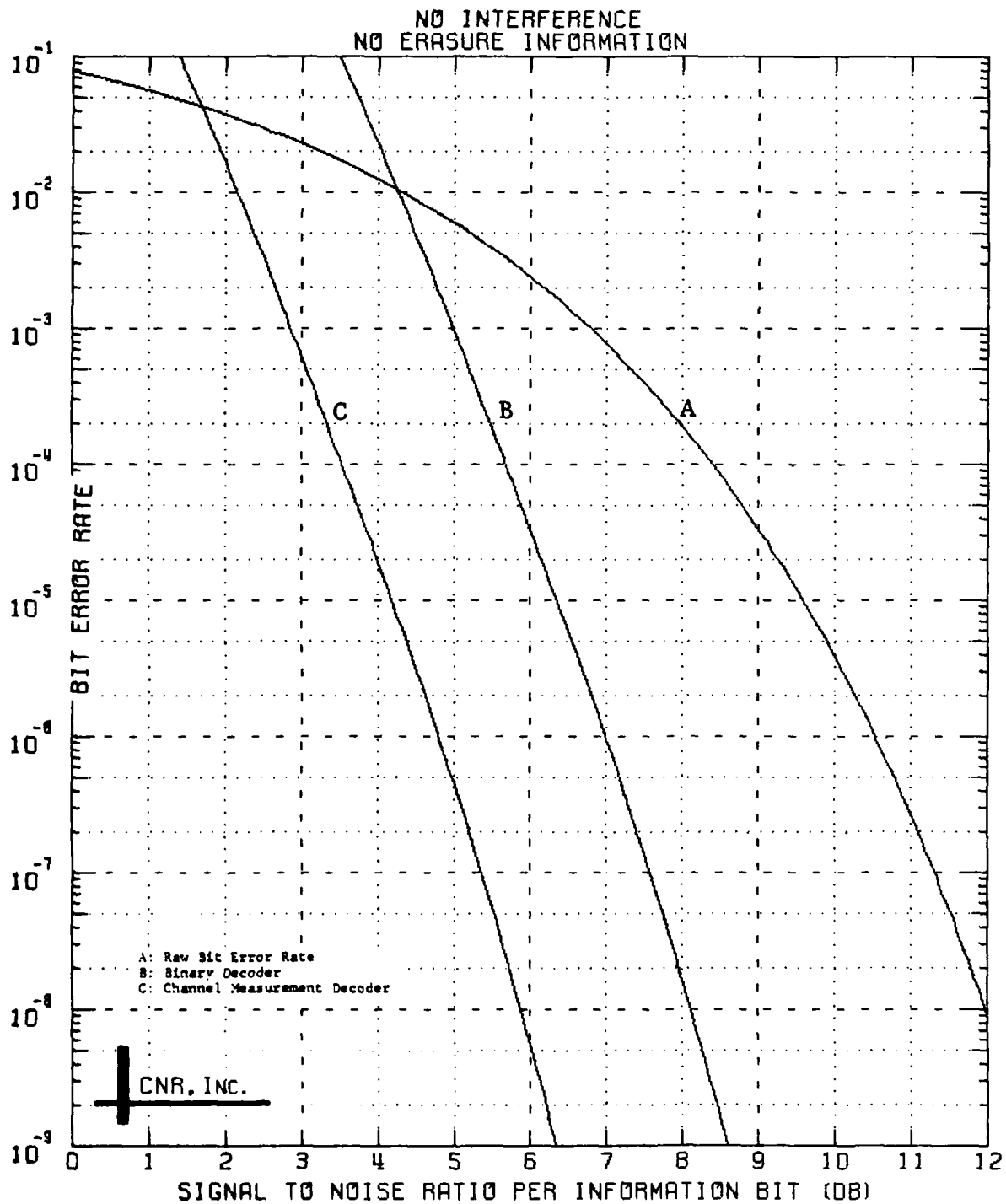
Figure 6.10 Decoded Performance of a Convolutional Code Rate 1/4; Constraint Length = 7
