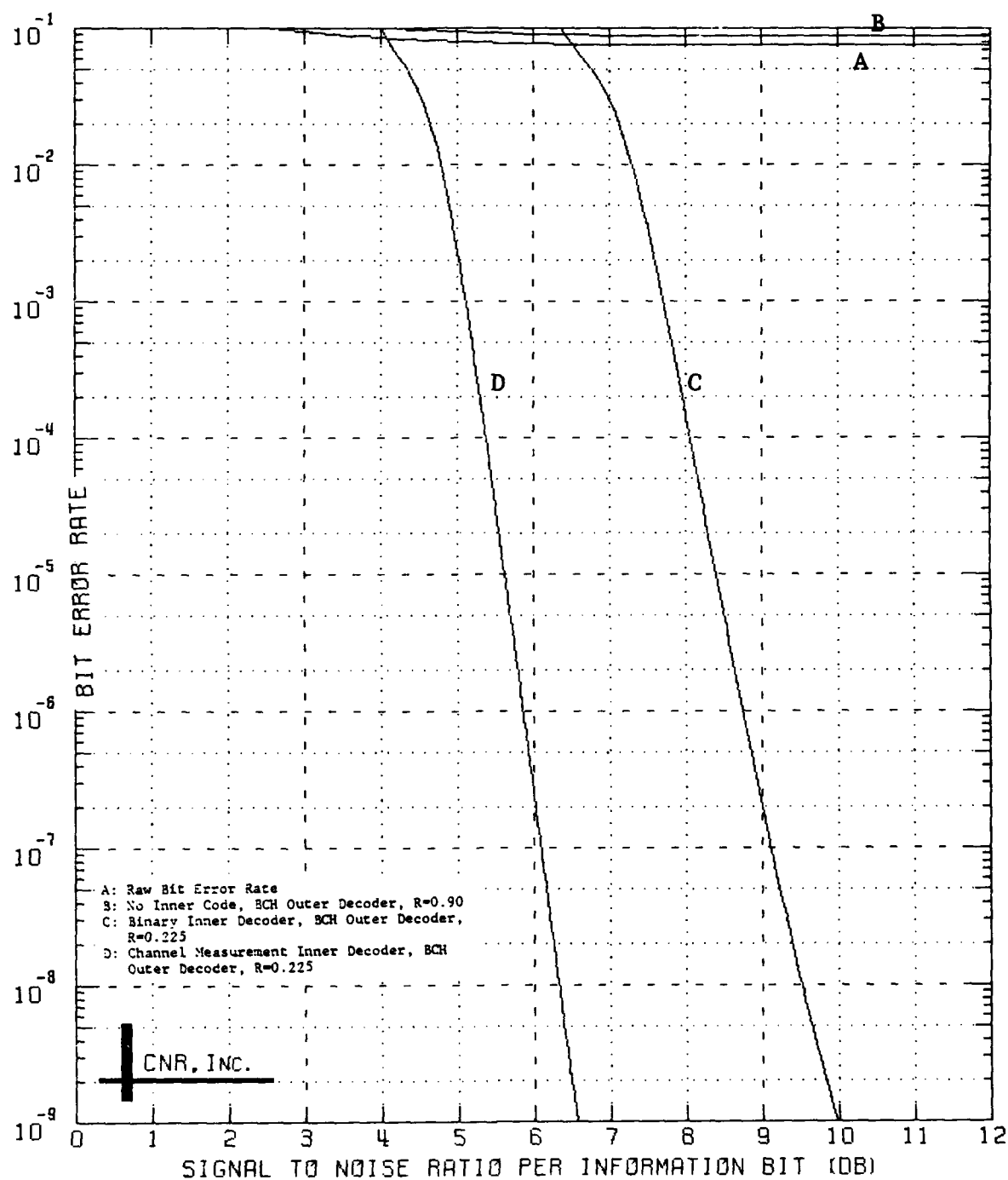
Figure 8.13 Decoded Performance of a Two-Stage Coding Approach Outer Decoder: BCH Code (240,216;7) Inner Decoder: Convolutional Code; Rate=1/4; K=7 \delta=0.15 and No Erasure Information Employed
