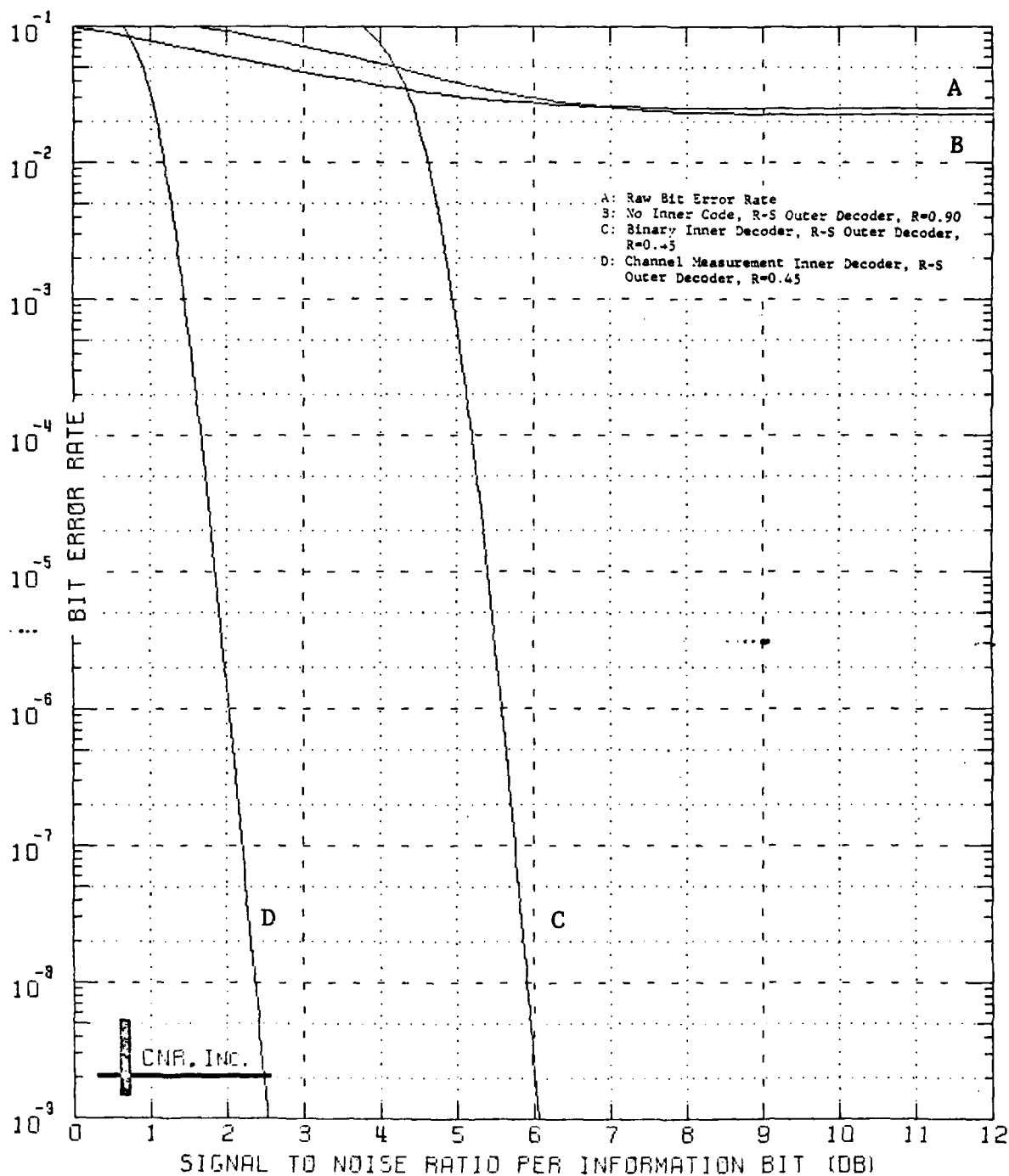
Figure 9.52 Decoded Performance of a Two-Stage Coding Approach Outer Decoder: Reed-Solomon Code (60,54;7) Symbol Interleaver Employed Inner Decoder: Block Code (128,64;22) \delta=0.05 and Erasure Information is Employed
