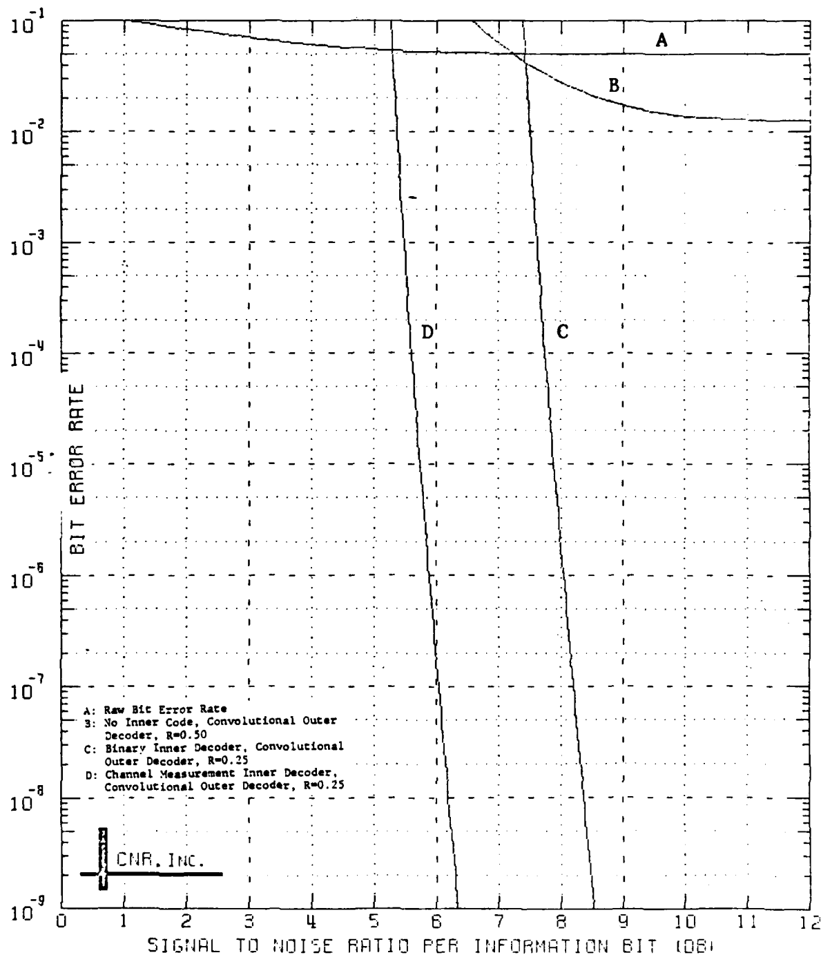
Figure 8.34 Decoded Performance of a Two-Stage Coding Approach Outer Decoder: Convolutional Code, Rate=1/2; K=7 Inner Decoder: Convolutional Code, Rate=1/2; K=7 \delta=0.10 and Erasure Information is Employed
