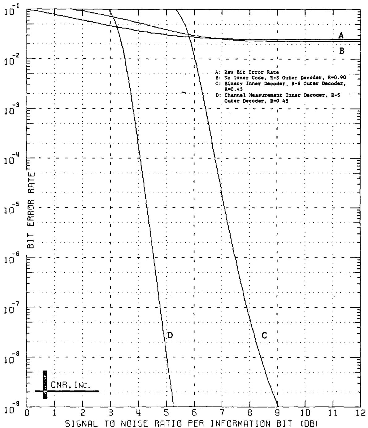
Figure 9.12 Decoded Performance of a Two-Stage Coding Approach Outer Decoder: Reed-Solomon Code (60,54;7) Symbol Interleaver Employed Inner Decoder: Convolutional Code, Rate=1/2; K=7 \delta=0.05 and No Erasure Information is Employed
