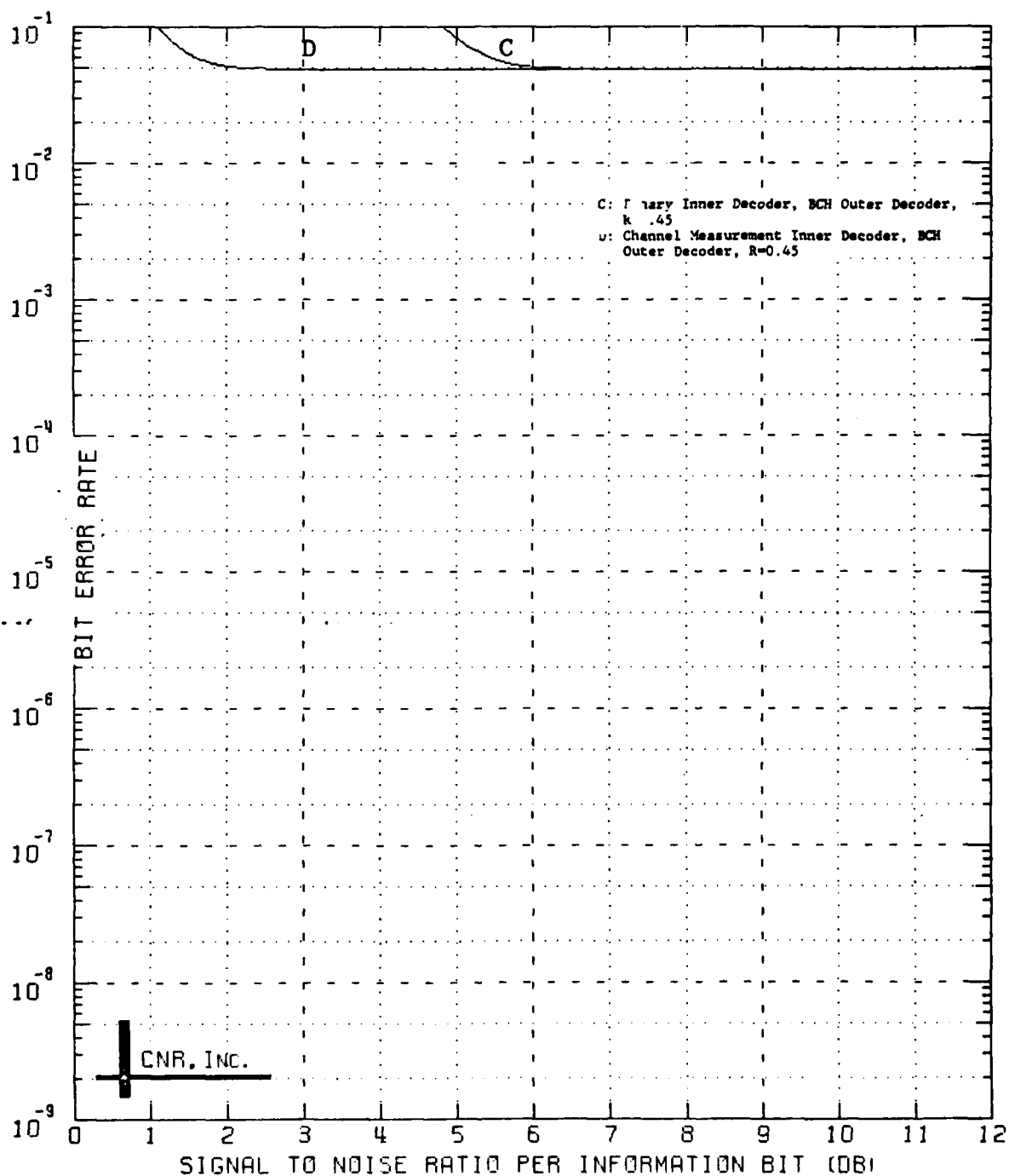
Figure 7.20 Decoded Performance of a Two-Stage Coding Approach Adaptive Technique Outer Decoder: BCH Code (240,216;7) Inner Decoder: Block Code (128,64;22) \delta=0.05 and No Erasure Information Employed
