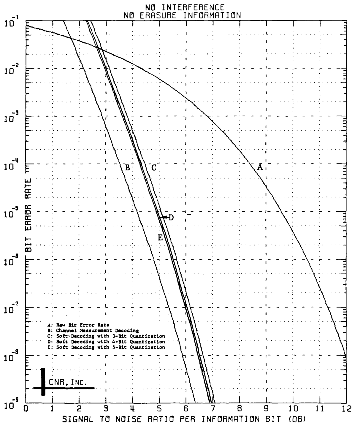
Figure 2 Decoded Performance of a Convolutional Code Rate 1/2; Constraint Length = 7; Gaussian Channel; CPSK Modulation
