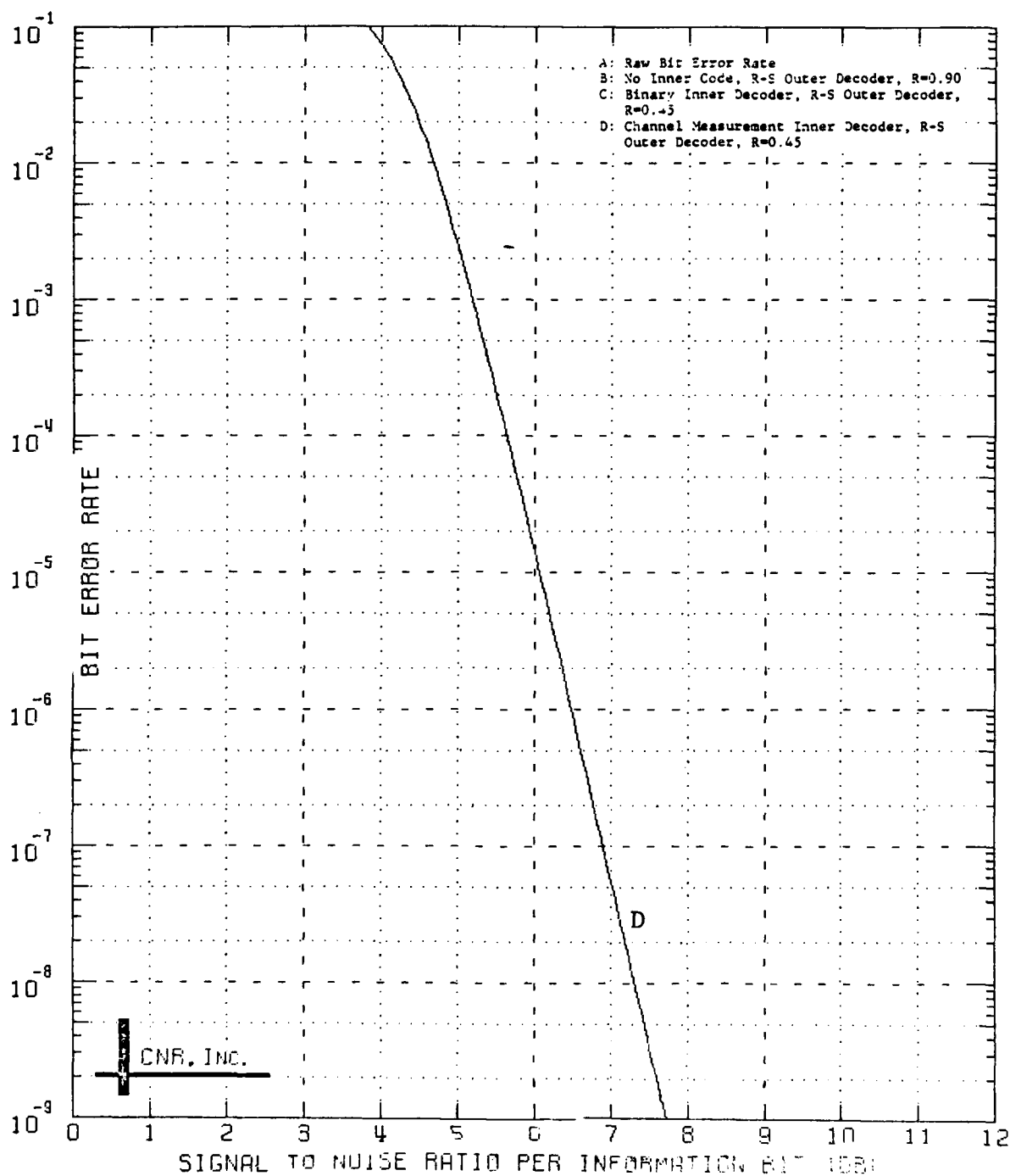
Figure 9.69 Decoded Performance of a Two-Stage Coding Approach Outer Decoder: Reed-Solomon Code (40,36;5) Symbol Interleaver Employed Inner Decoder: Block Code (128,64;22) \delta=0.20 and No Erasure Information Employed
