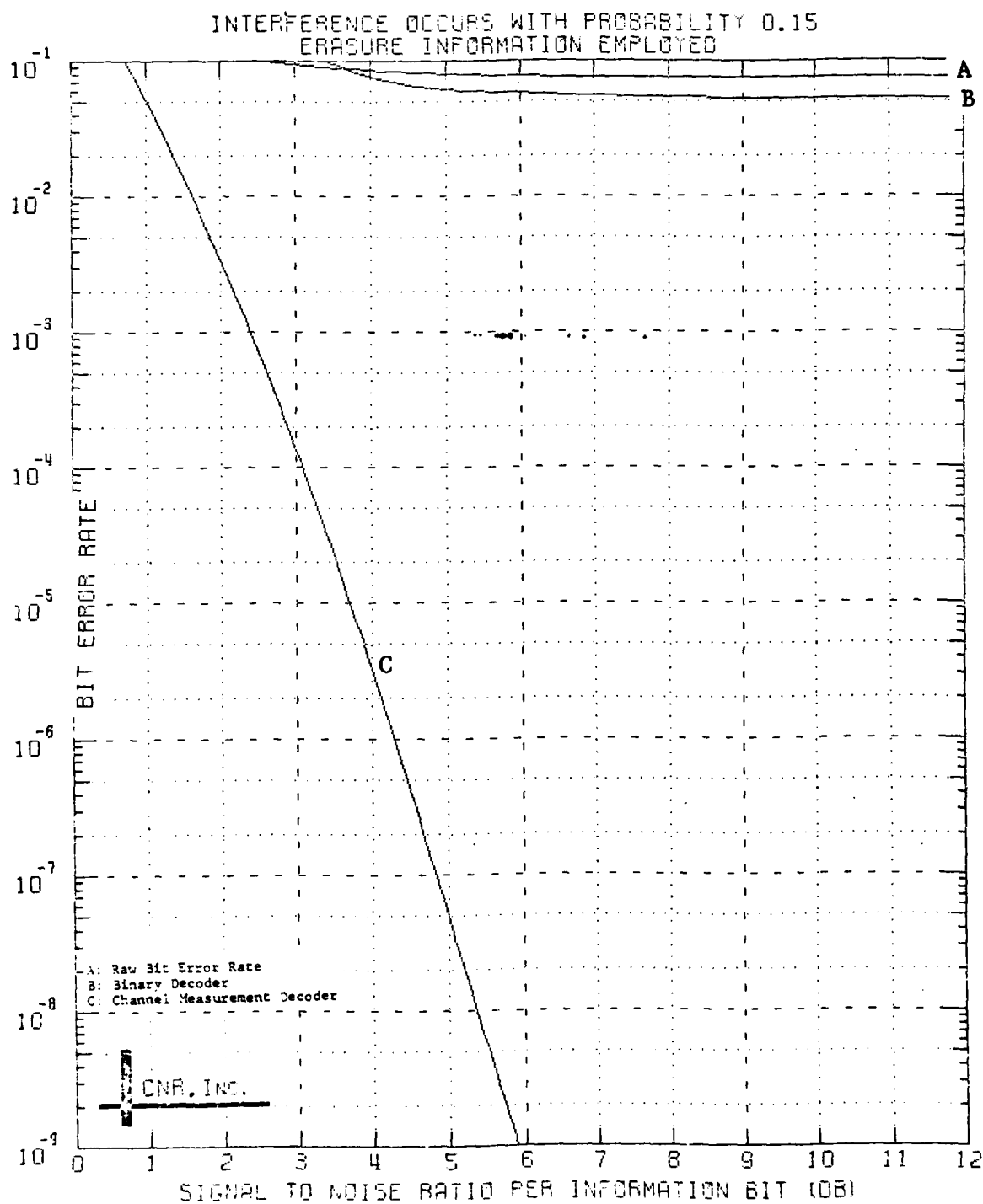
Figure 5.17 Decoded Performance of a Block Code Dimensions (128,64;22)
