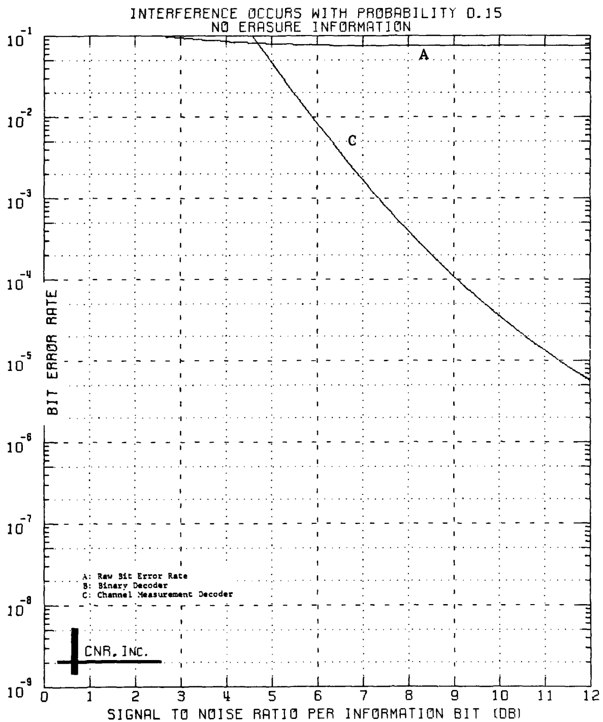
Figure 6.4 Decoded Performance of a Convolutional Code Rate 1/2; Constraint Length = 7
