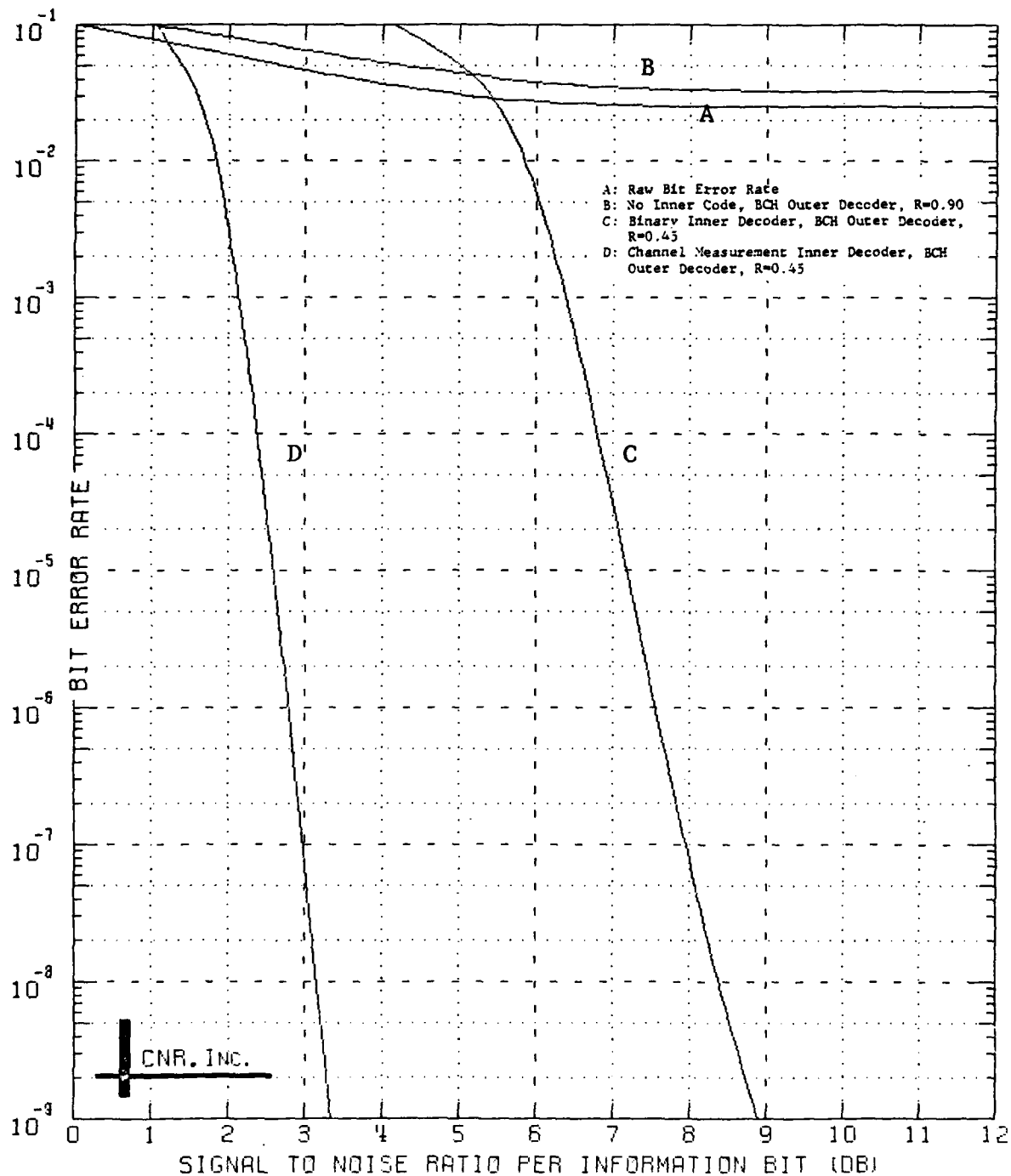
Figure 7.2 Decoded Performance of a Two-Stage Coding Approach Outer Decoder: BCH Code (240,216;7) Inner Decoder: Block Code (128,64;22) \delta=0.05 and No Erasure Information Employed
