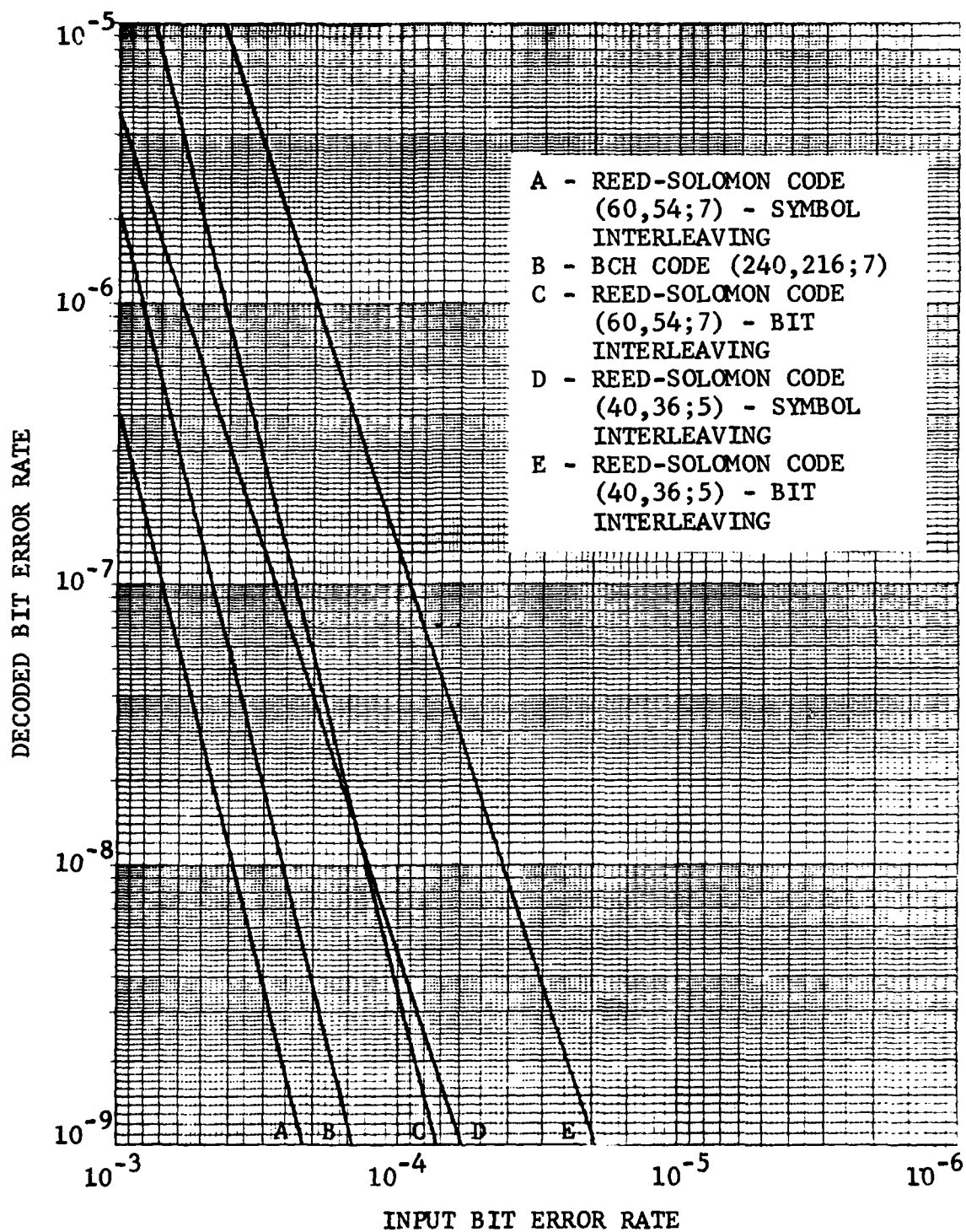
Figure 4.2 Comparison of Error Rate Performance for R = 0.9 Codes
