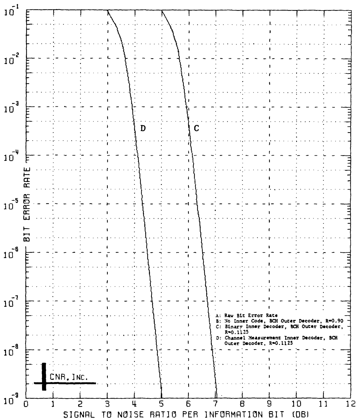
Figure 8.27 Decoded Performance of a Two-Stage Coding Approach Outer Decoder: BCH Code (240,216;7) Inner Decoder: Convolutional Code; Rate=1/8; K=7 \delta=0.20 and Erasure Information is Employed
