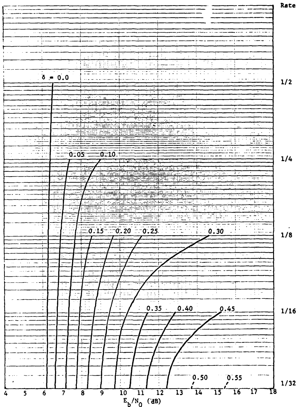
Figure 6.33 Convolutional Coding Performance with Interference Probability as a Parameter Binary Decoding-No Erasure Information
