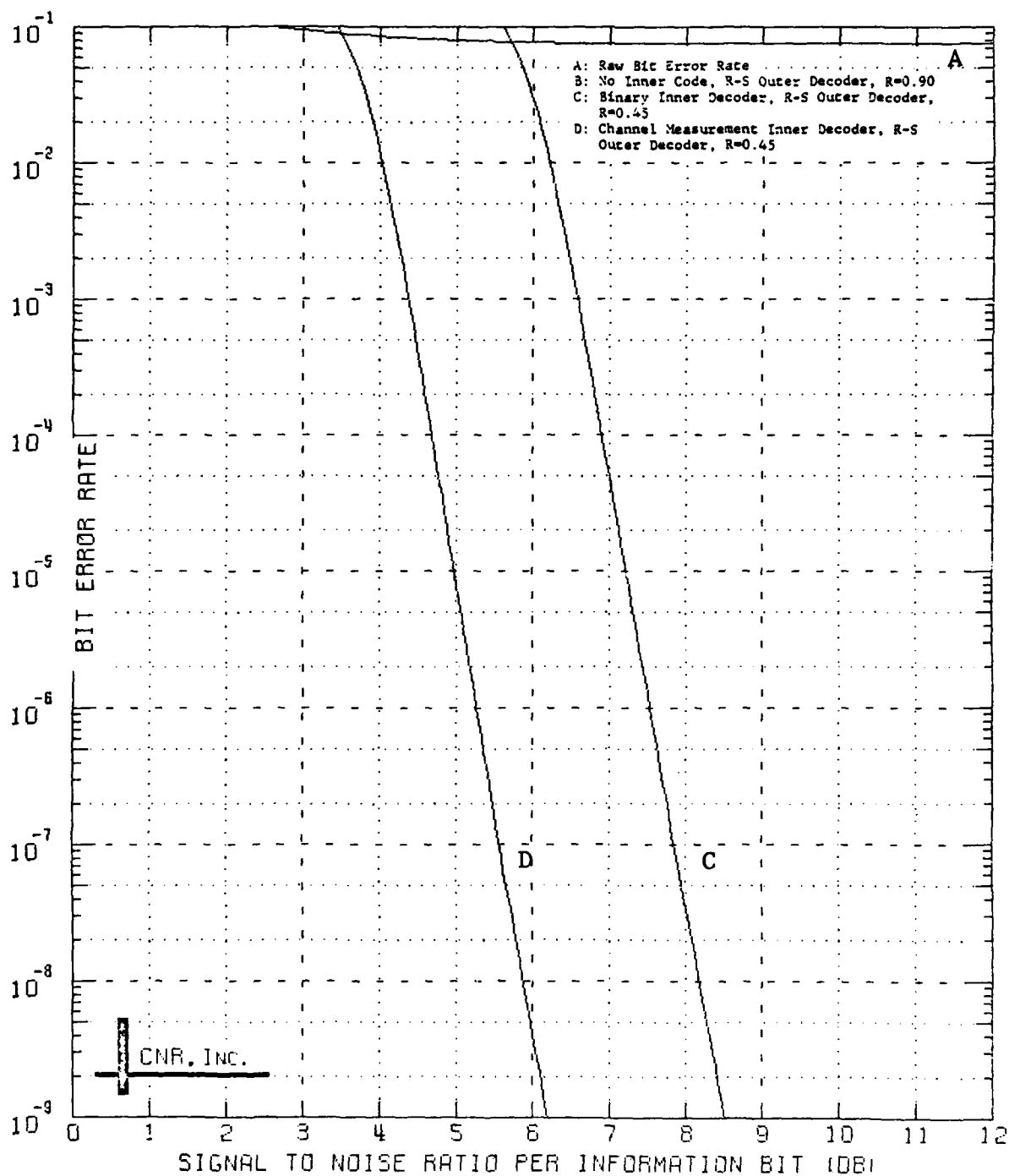
Figure 9.27 Decoded Performance of a Two-Stage Coding Approach Outer Decoder: Reed-Solomon Code (40,36;5) Bit Interleaver Employed Inner Decoder: Convolutional Code, Rate=1/2; K=7 \delta=0.15 and Erasure Information is Employed
