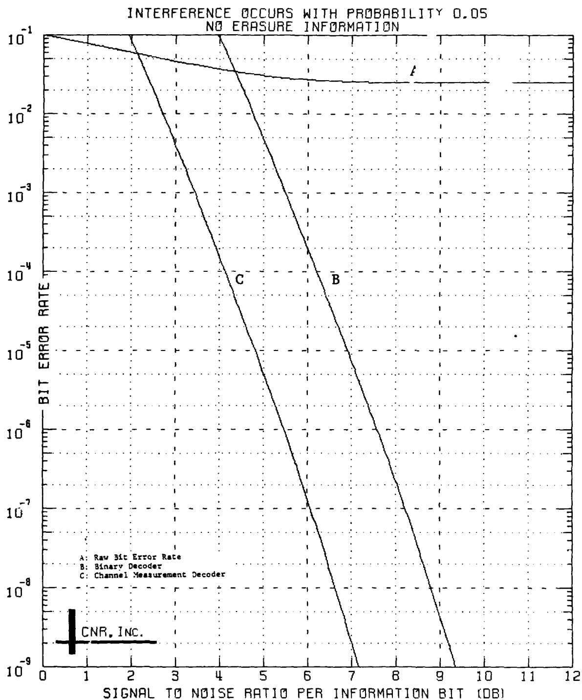
Figure 6.20 Decoded Performance of a Convolutional Code Rate 1/8; Constraint Length = 7
