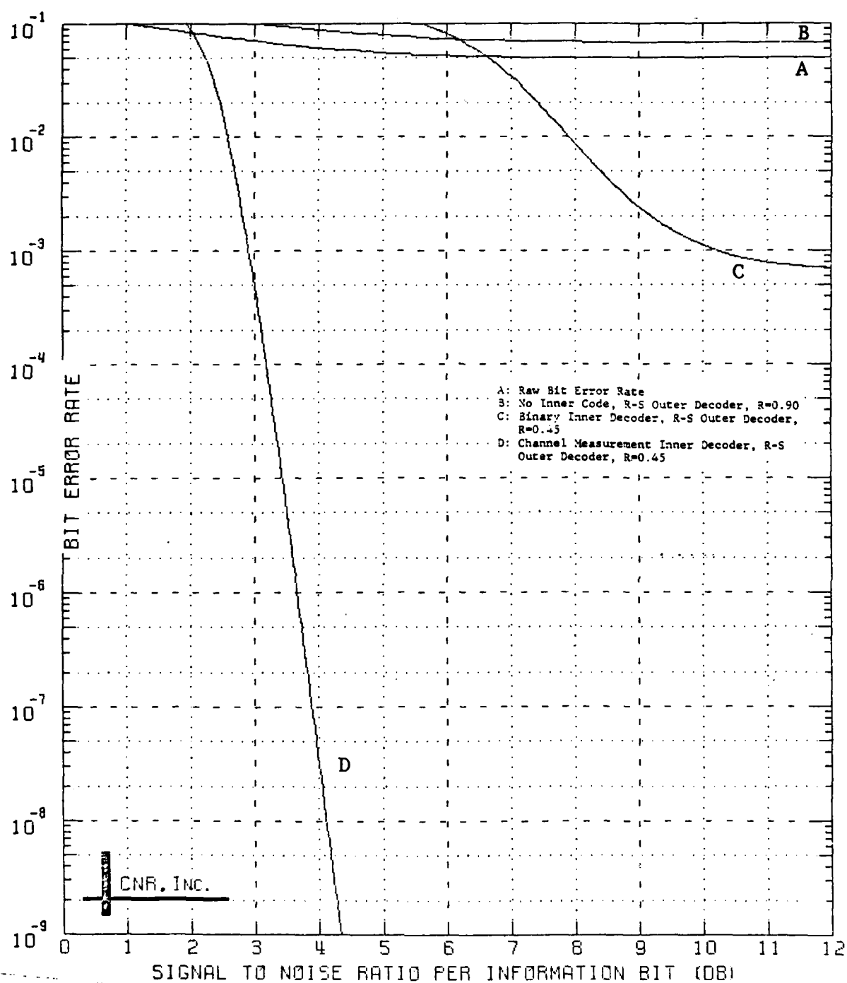
Figure 9.49 Decoded Performance of a Two-Stage Coding Approach Outer Decoder: Reed-Solomon Code (60,54;7) Symbol Interleaver Employed Inner Decoder: Block Code (128,64;22) \delta=0.10 and No Erasure Information Employed
