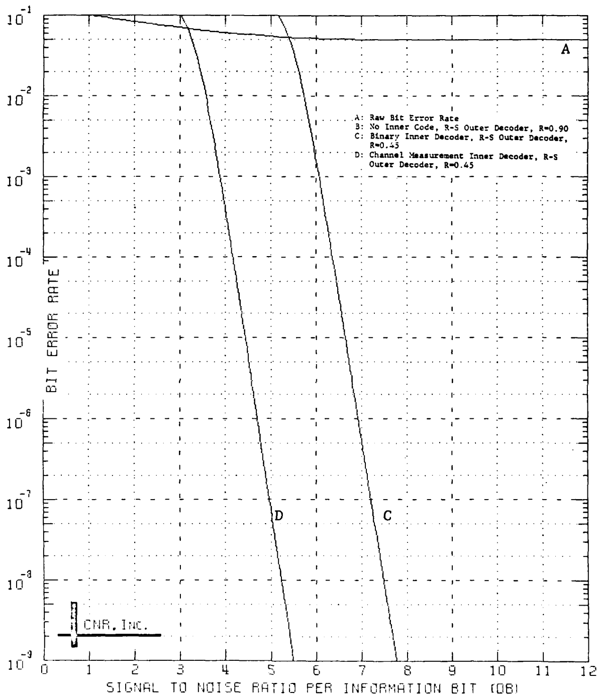
Figure 9.26 Decoded Performance of a Two-Stage Coding Approach Outer Decoder: Reed-Solomon Code (40,36;5) Bit Interleaver Employed Inner Decoder: Convolutional Code, Rate=1/2; K=7 \delta=0.10 and Erasure Information Employed
