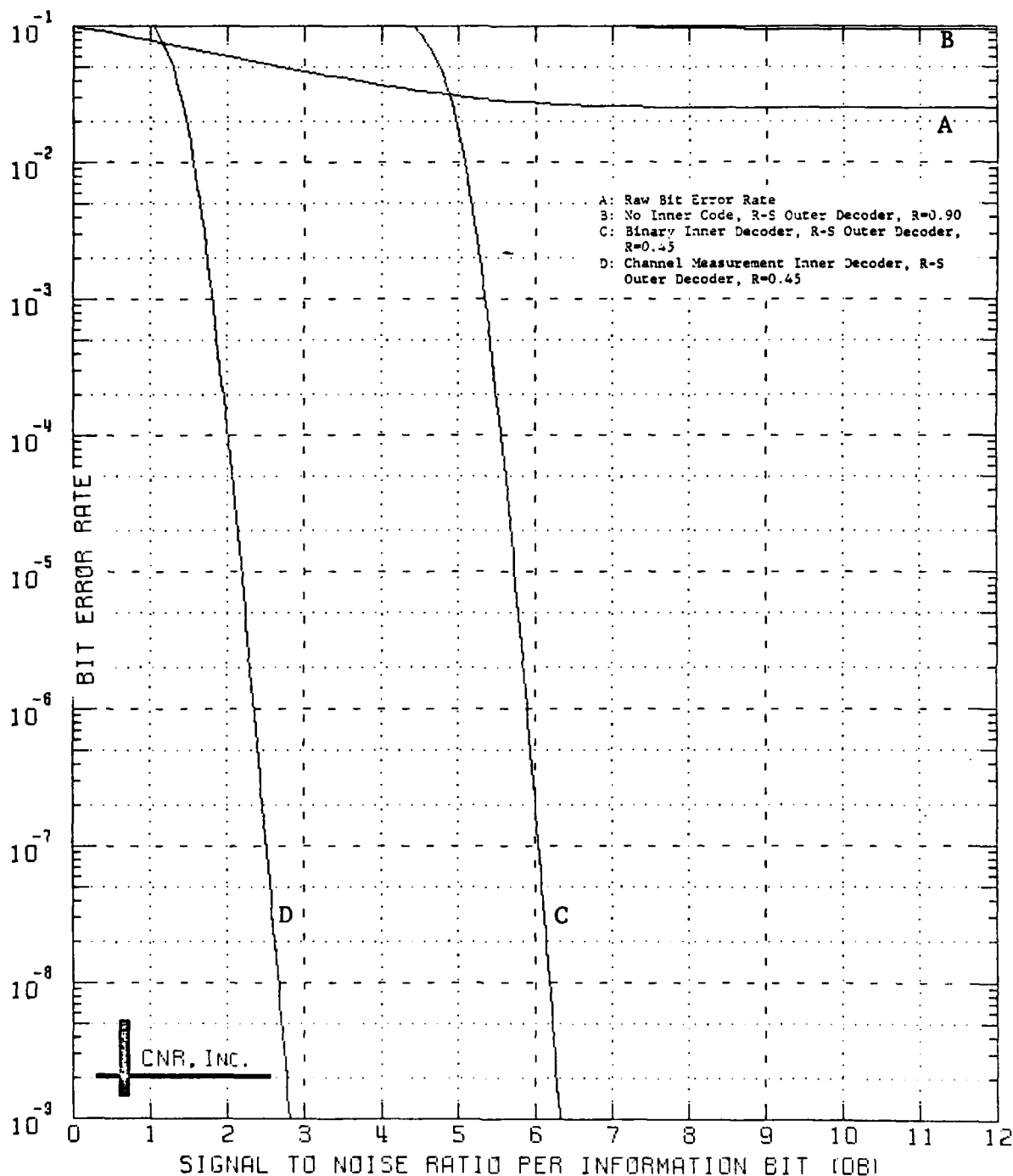
Figure 9.43 Decoded Performance of a Two-Stage Coding Approach Outer Decoder: Reed-Solomon Code (60,54;7) Bit Interleaver Employed Inner Decoder: Block Code (128,64;22) \delta=0.05 and Erasure Information is Employed
