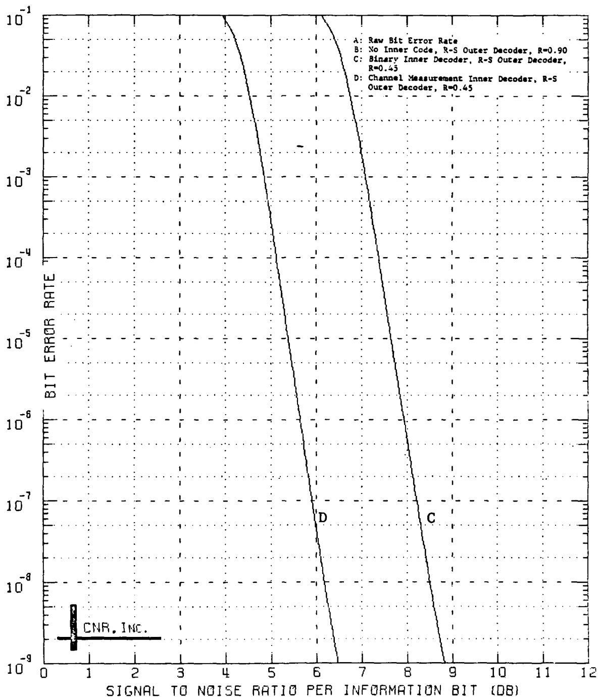
Figure 9.10 Decoded Performance of a Two-Stage Coding Approach Outer Decoder: Reed-Solomon Code (60,54;7) Bit Interleaver Employed Inner Decoder: Convolutional Code, Rate=1/2; K=7 \delta=0.20 and Erasure Information is Employed
