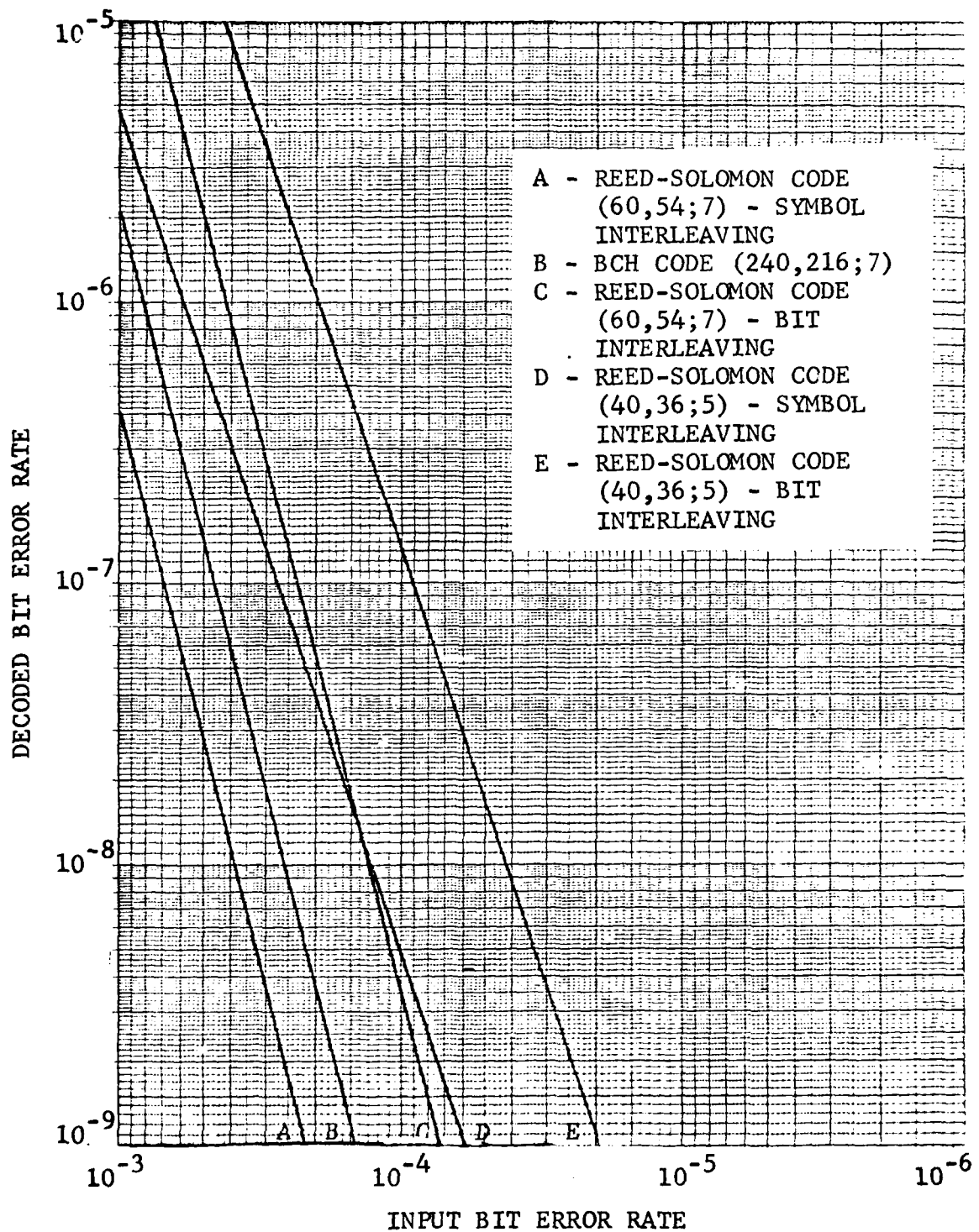
Figure 9.1 Comparison of Error Rate Performance for R = 0.9 Codes
