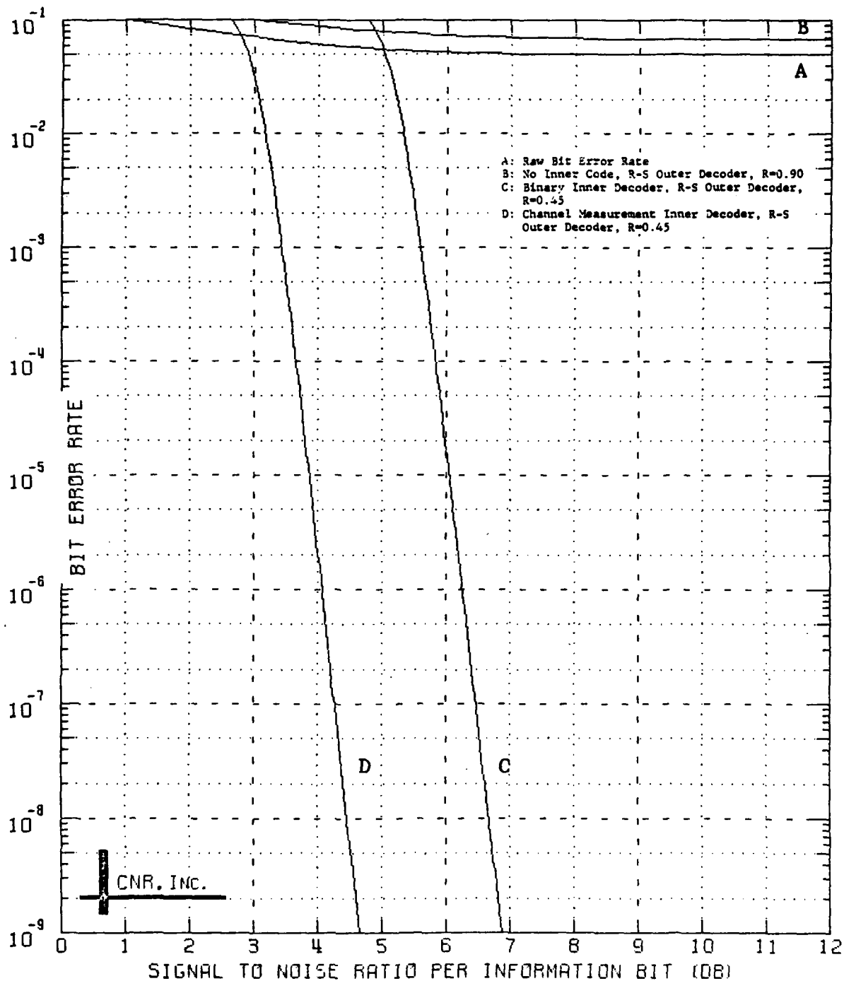
Figure 9.17 Decoded Performance of a Two-Stage Coding Approach Outer Decoder: Reed-Solomon Code (60,54;7) Symbol Interleaver Employed Inner Decoder: Convolutional Code, Rate=1/2; K=7 \delta=0.10 and Erasure Information is Employed
