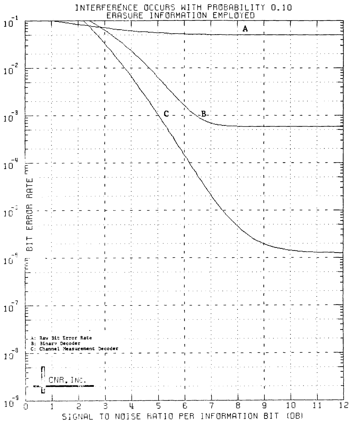
Figure 5.7 Decoded Performance of a Block Code Dimensions (24,12;8)
