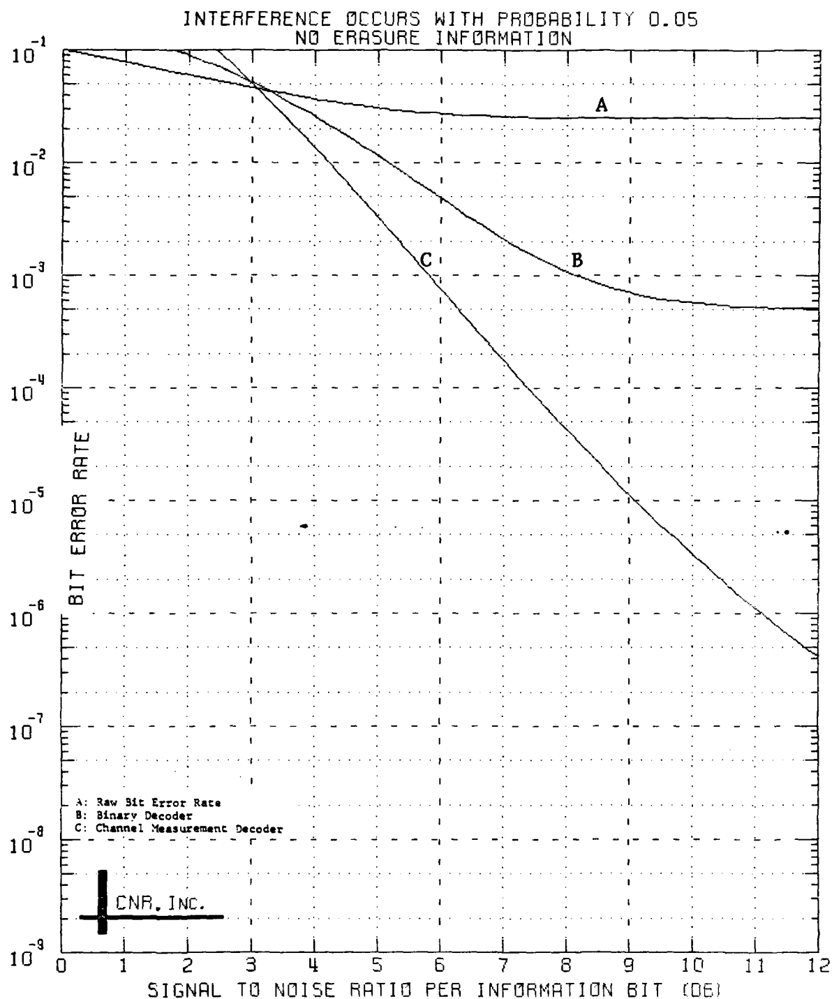
Figure 5.2 Decoded Performance of a Block Code Dimensions (24,12;8)
