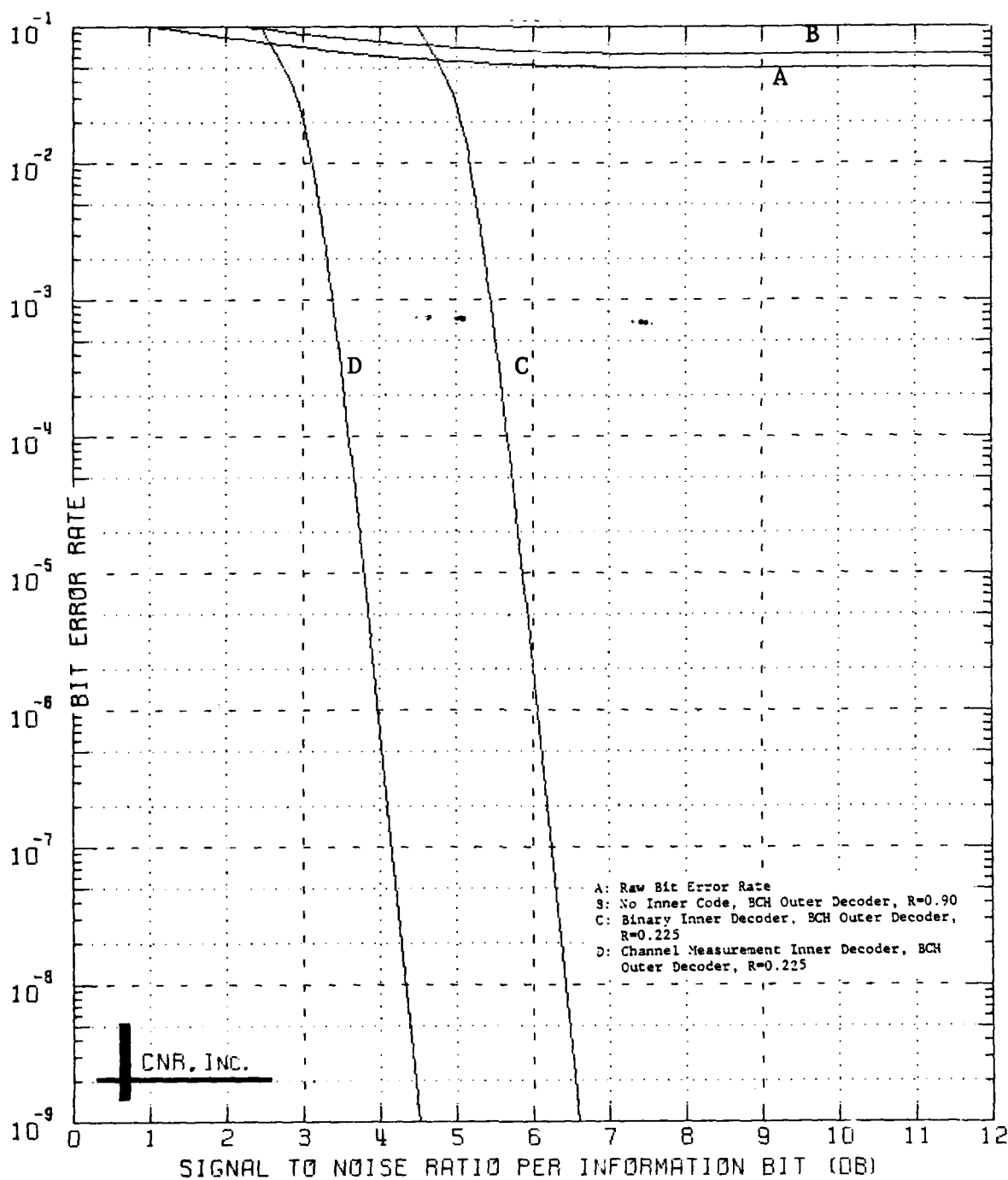
Figure 8.16 Decoded Performance of a Two-Stage Coding Approach Outer Decoder: BCH Code (240,216;7) Inner Decoder: Convolutional Code; Rate=1/4; K=7 \delta=0.10 and Erasure Information is Employed
