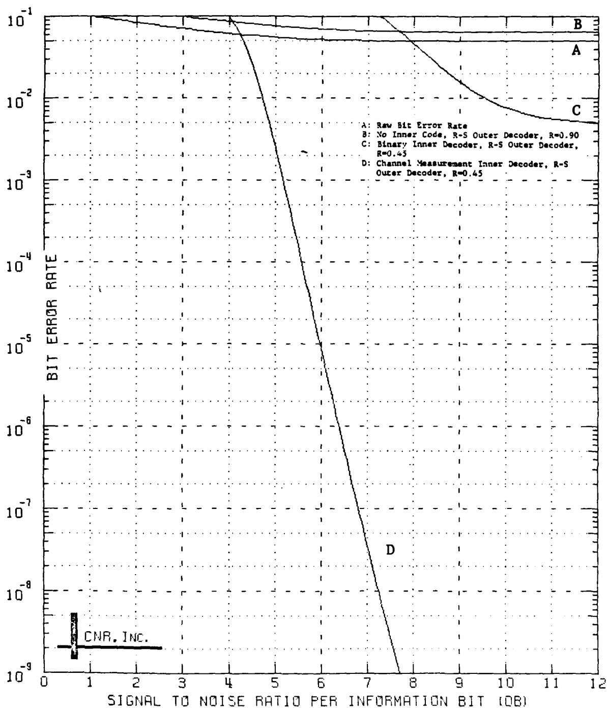
Figure 9.31 Decoded Performance of a Two-Stage Coding Approach Outer Decoder: Reed-Solomon Code (40,36;5) Symbol Interleaver Employed Inner Decoder: Convolutional Code, Rate=1/2; K=7 \delta=0.10 and No Erasure Information Employed
