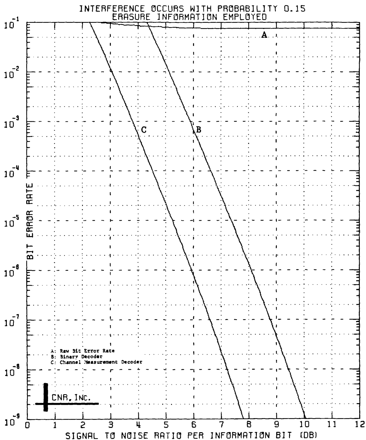
Figure 6.17 Decoded Performance of a Convolutional Code Rate 1/4; Constraint Length = 7
