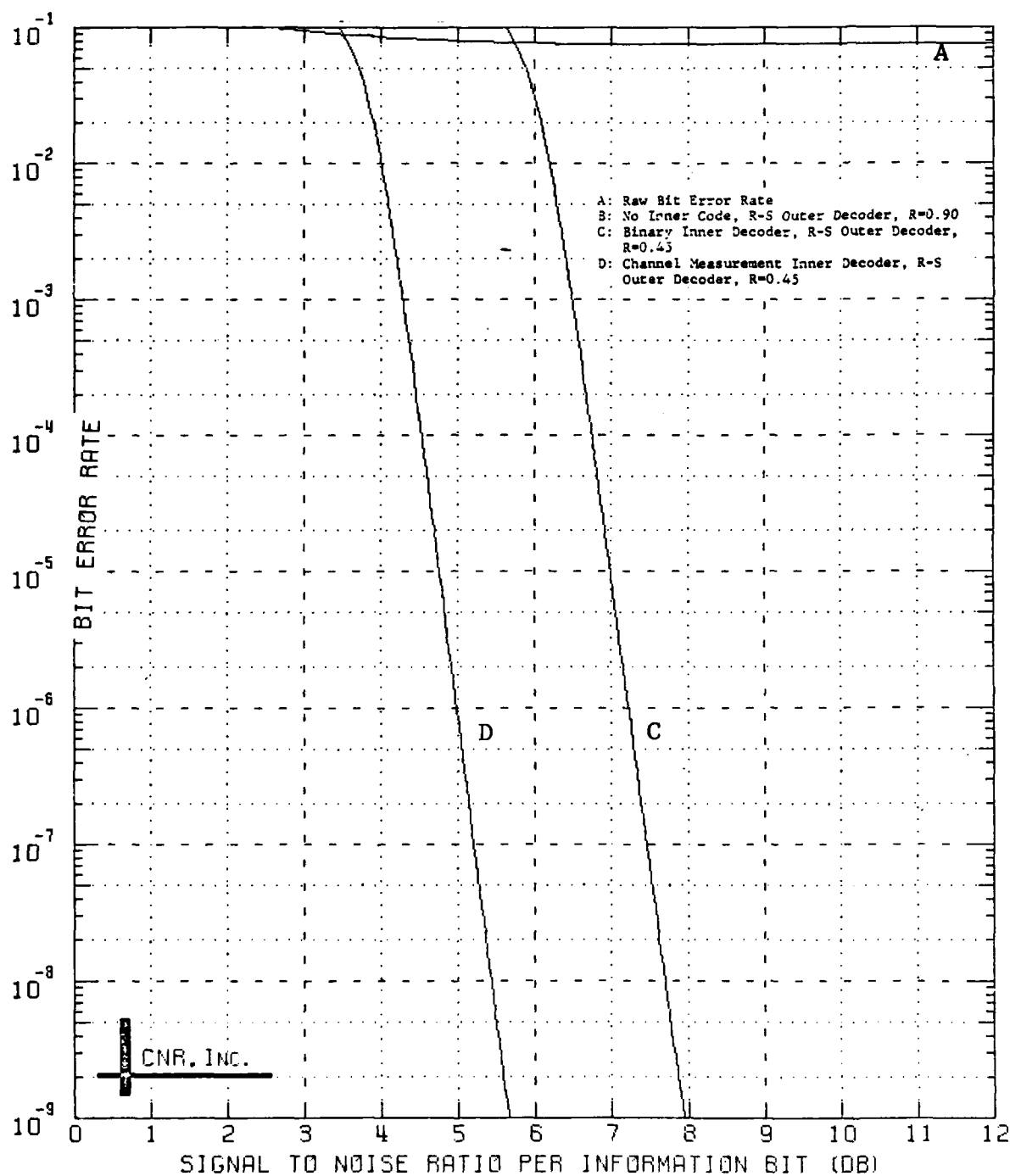
Figure 9.9 Decoded Performance of a Two-Stage Coding Approach Outer Decoder: Reed-Solomon Code (60,54;7) Bit Interleaver Employed Inner Decoder: Convolutional Code, Rate=1/2; K=7 \delta=0.15 and Erasure Information is Employed
