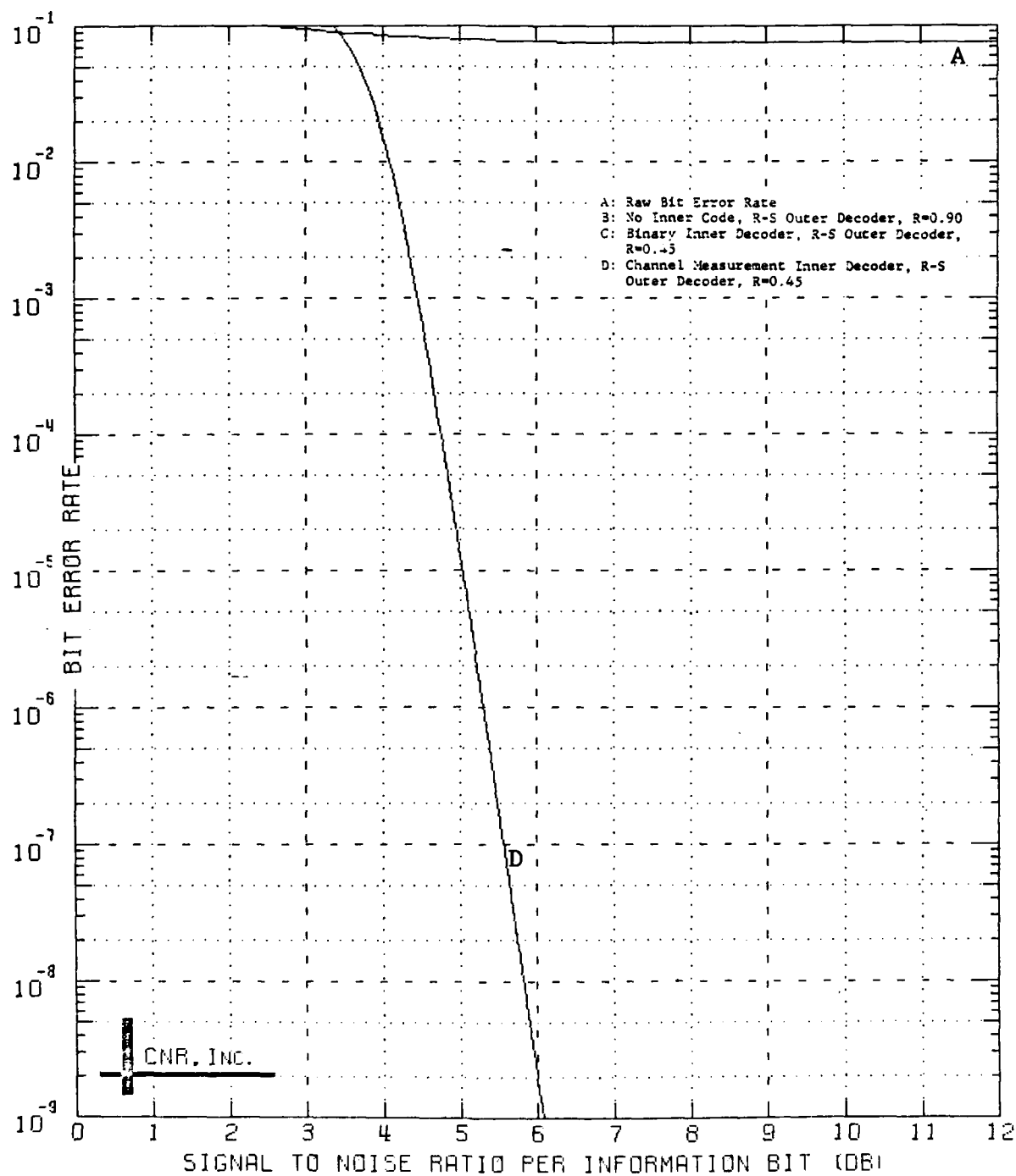
Figure 9.41 Decoded Performance of a Two-Stage Coding Approach Outer Decoder: Reed-Solomon Code (60,54;7) Bit Interleaver Employed Inner Decoder: Block Code (128,64;22) \delta=0.15 and No Erasure Information Employed
