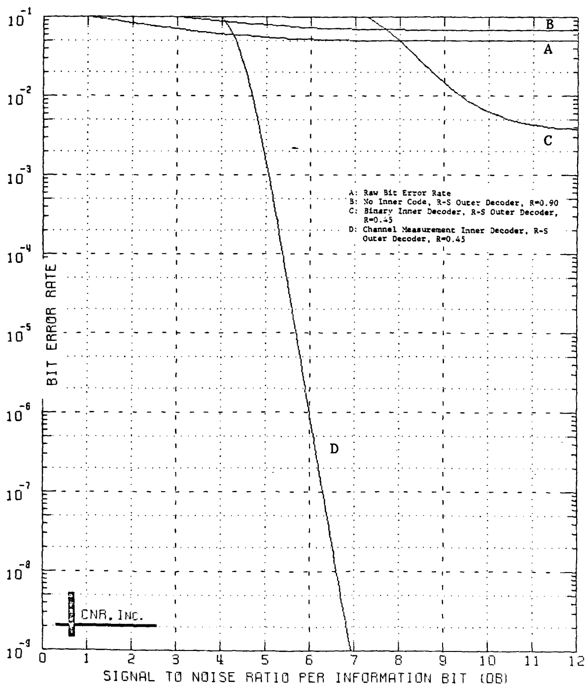
Figure 9.13 Decoded Performance of a Two-Stage Coding Approach Outer Decoder: Reed-Solomon Code (60,54;7) Symbol Interleaver Employed Inner Decoder: Convolutional Code, Rate=1/2; K=7 \delta=0.10 and No Erasure Information Employed
