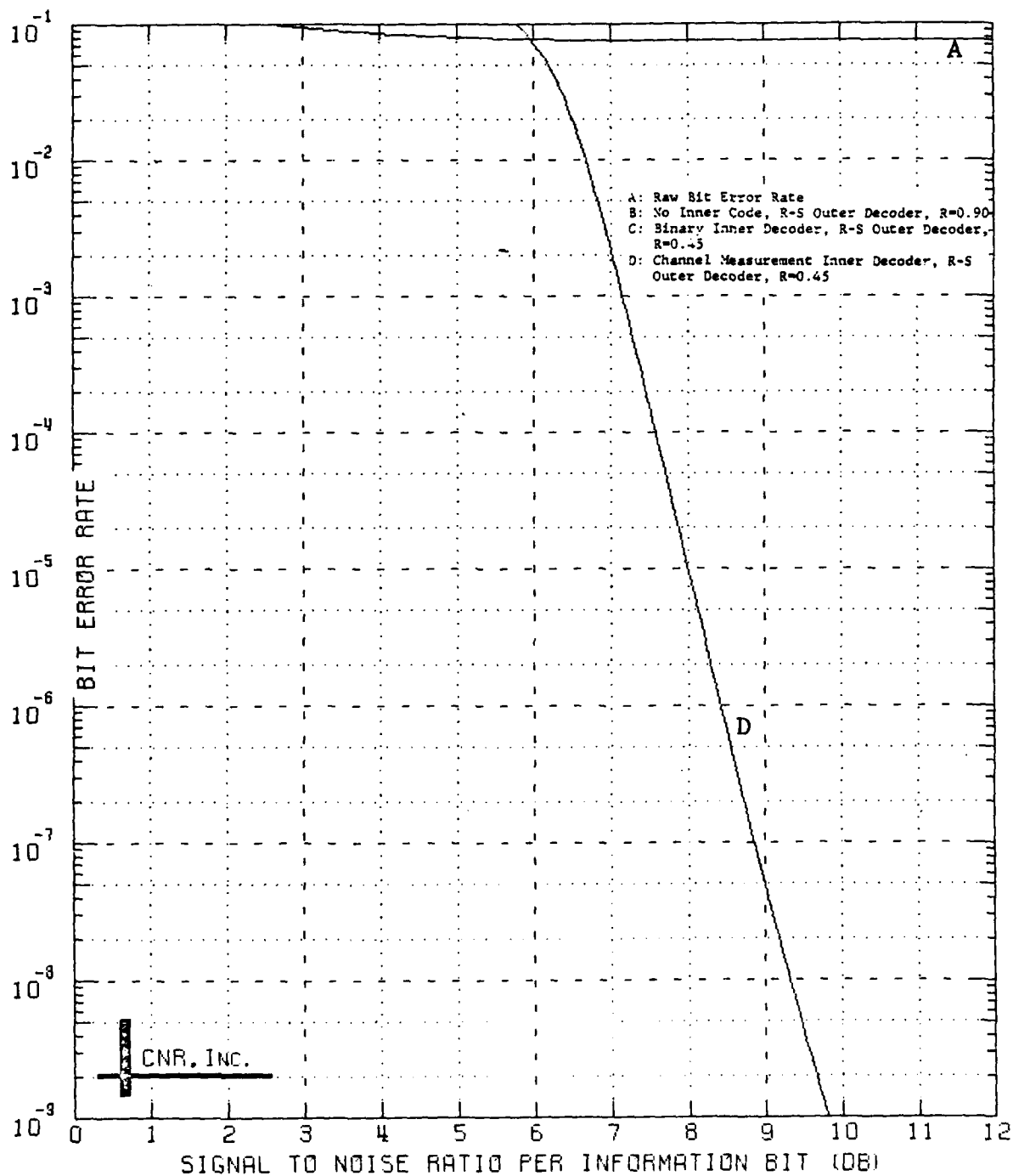
Figure 9.5 Decoded Performance of a Two-Stage Coding Approach Outer Decoder: Reed-Solomon Code (60,54;7) Bit Interleaver Employed Inner Decoder: Convolutional Code, Rate=1/2; K=7 \delta=0.15 and No Erasure Information Employed
