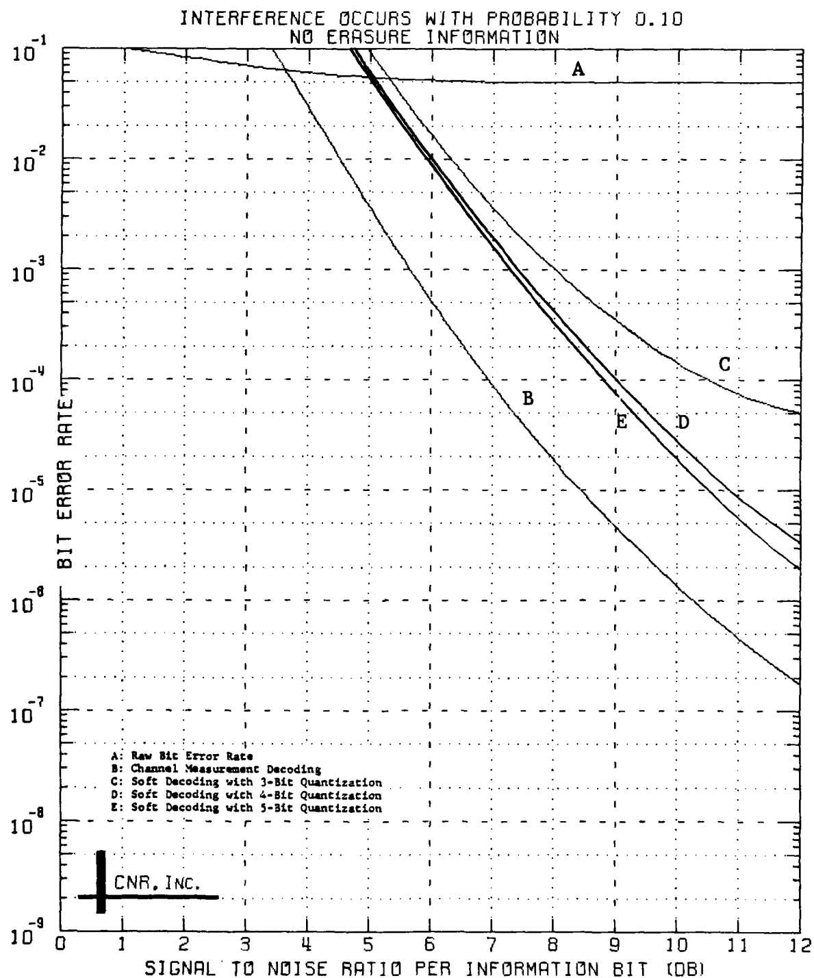
Figure 4 Decoded Performance of a Convolutional Code Rate 1/2; Constraint Length = 7; Gaussian Channel; CPSK Modulation
