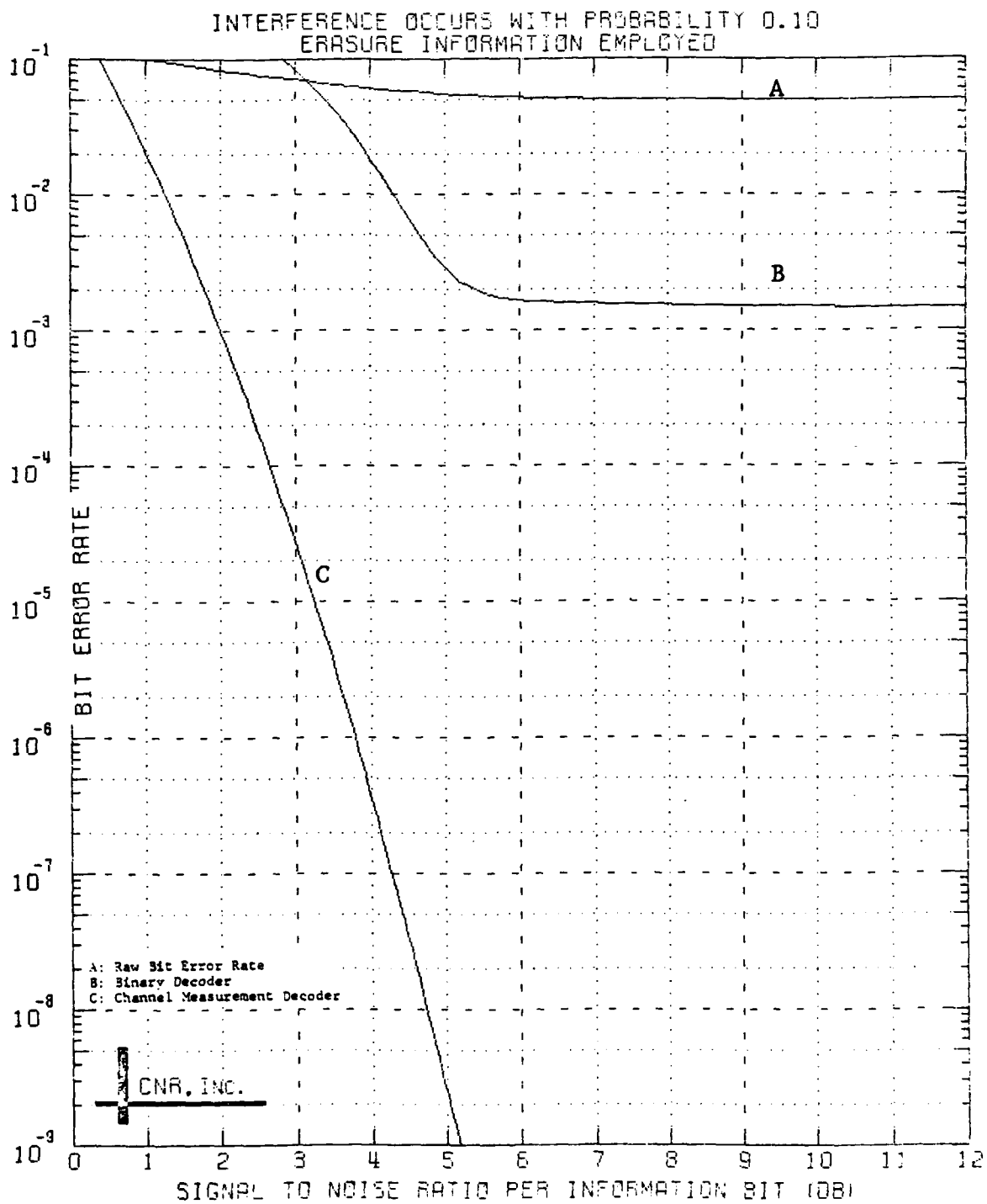
Figure 5.16 Decoded Performance of a Block Code Dimensions (128,64;22)
