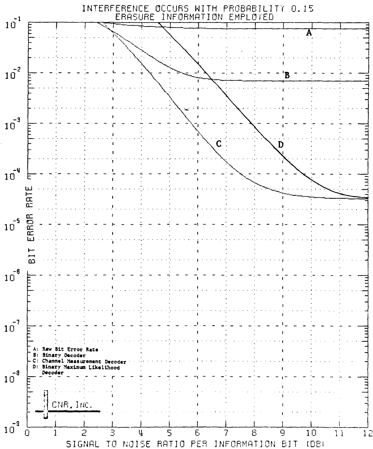
Figure 5.26 Decoded Performance of a Block Code Dimensions (24,12;8)
