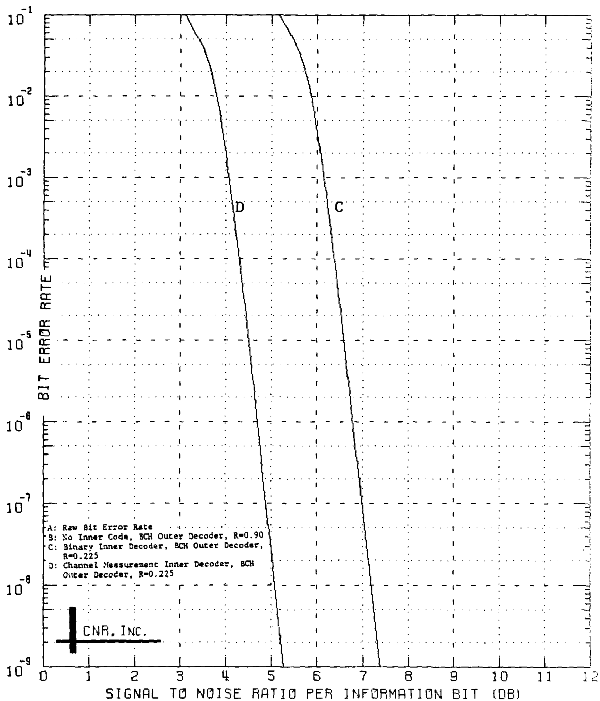
Figure 8.18 Decoded Performance of a Two-Stage Coding Approach Outer Decoder: BCH Code (240,216;7) Inner Decoder: Convolutional Code; Rate=1/4; K=7 \delta=0.20 and Erasure Information is Employed
