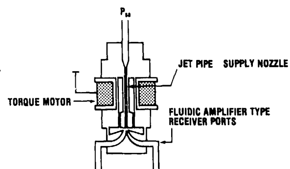
Figure 16. Bosch electrofluidic converter or amplifier (jet pipe).
