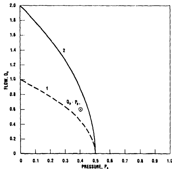
Figure 10. Fluidic amplifier output characteristics for single amplifier (1) and two amplifiers in parallel (2).
