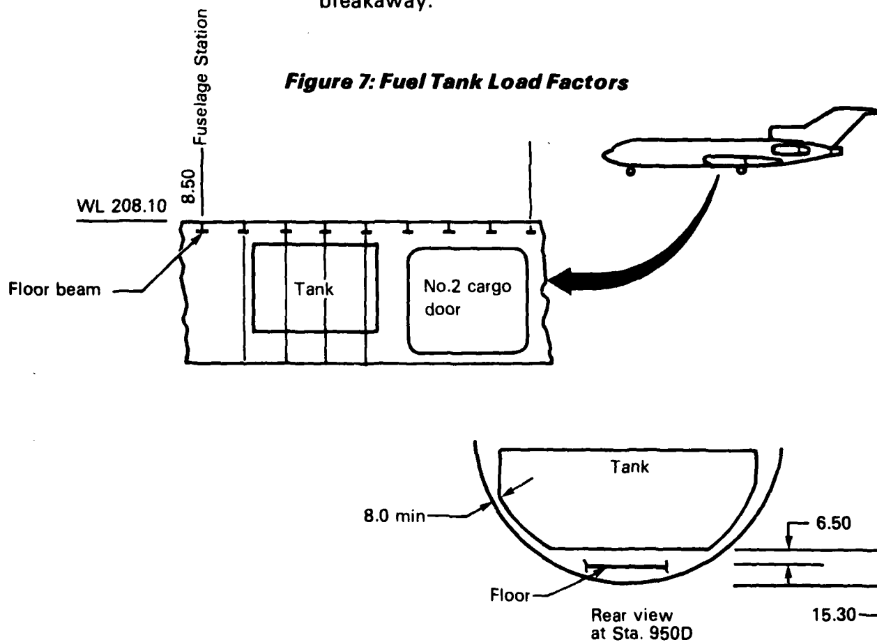
Figure 6: Cargo Compartment Tank Installation
