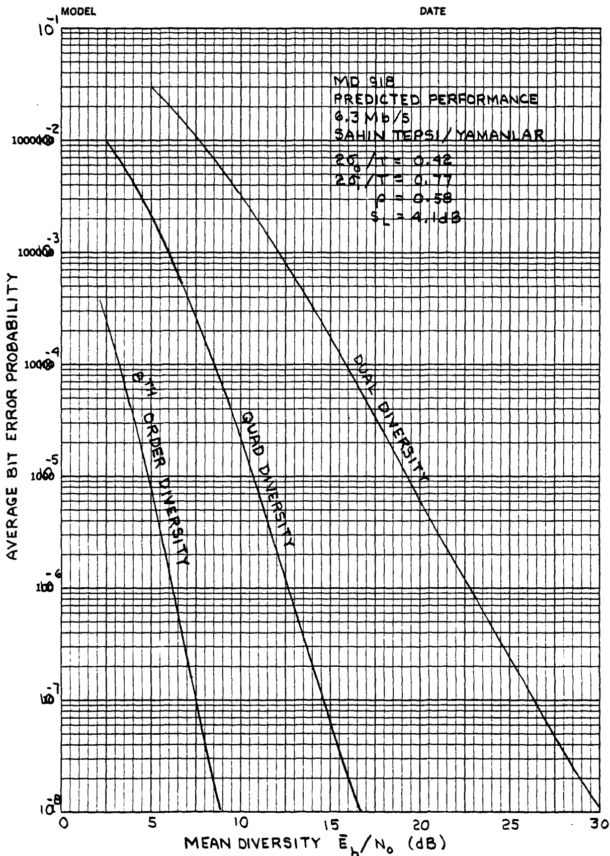
Fig. 2.10 Predicted Performance: L-Band 6.3 Mb/s
