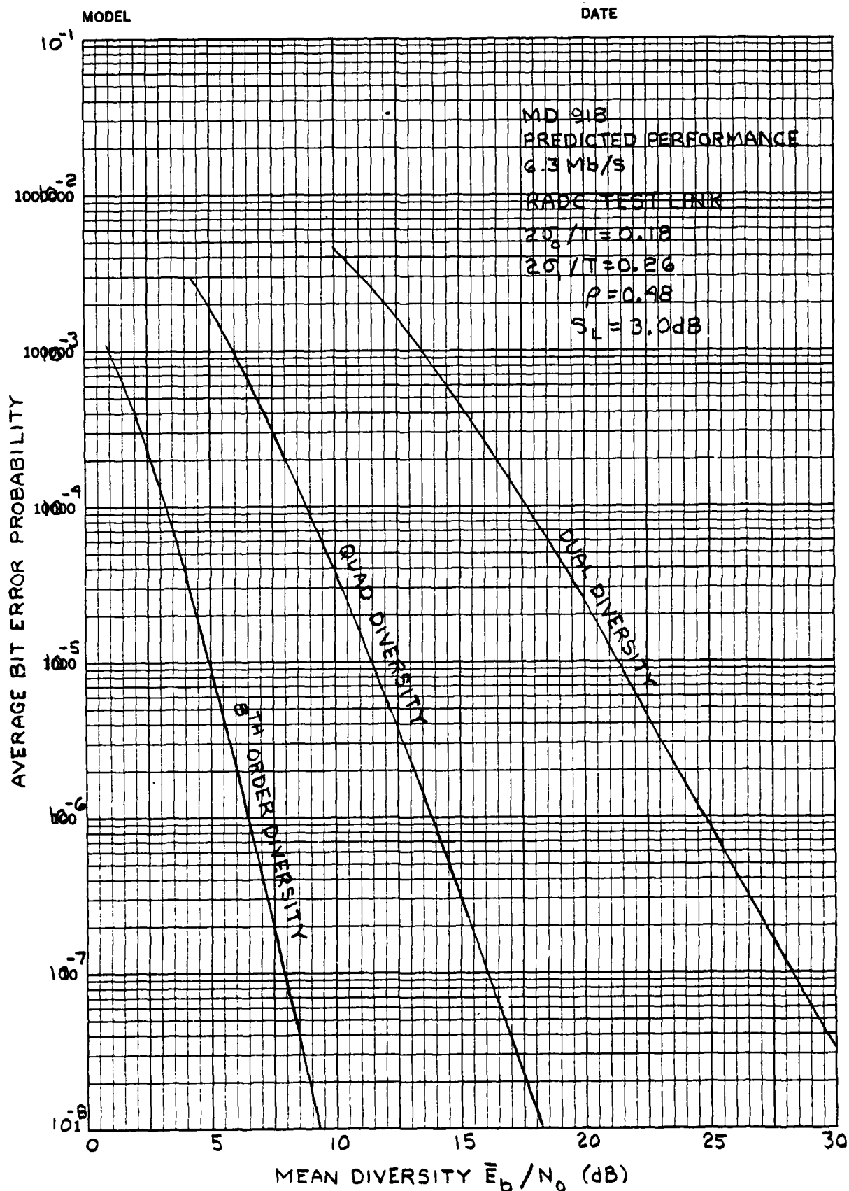
Fig. 2.8 Predicted Performance: C-Band, 6.3 Mb/s
