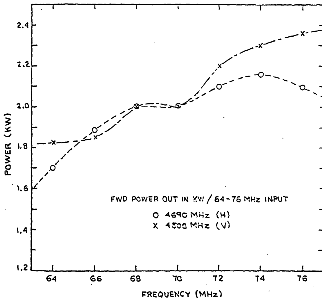
Fig. 3.3 AN/TRC-132A Transmitter Frequency Response
