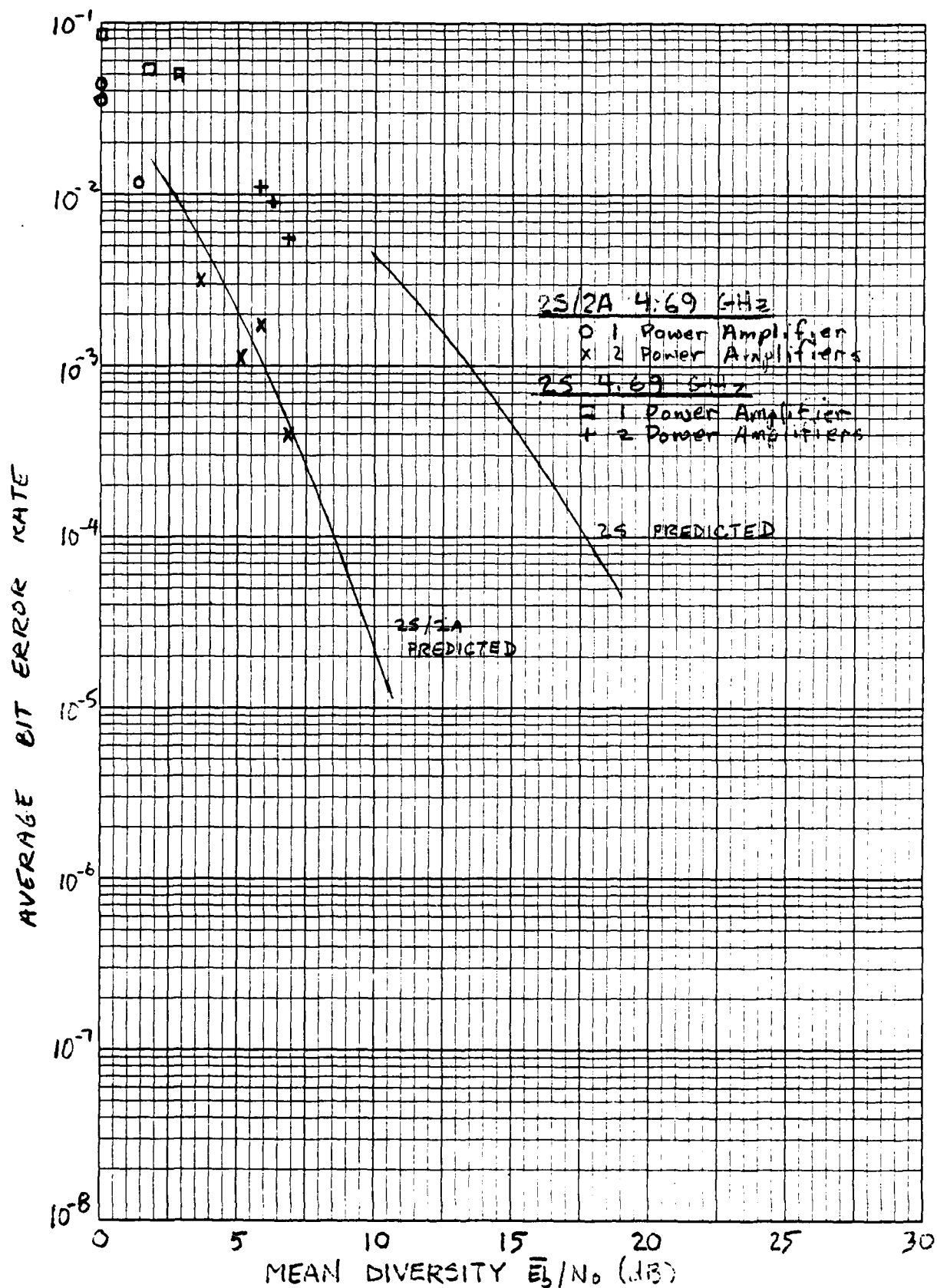
Fig. 4.17 Two Transmit Power Amplifiers on Same Frequency
