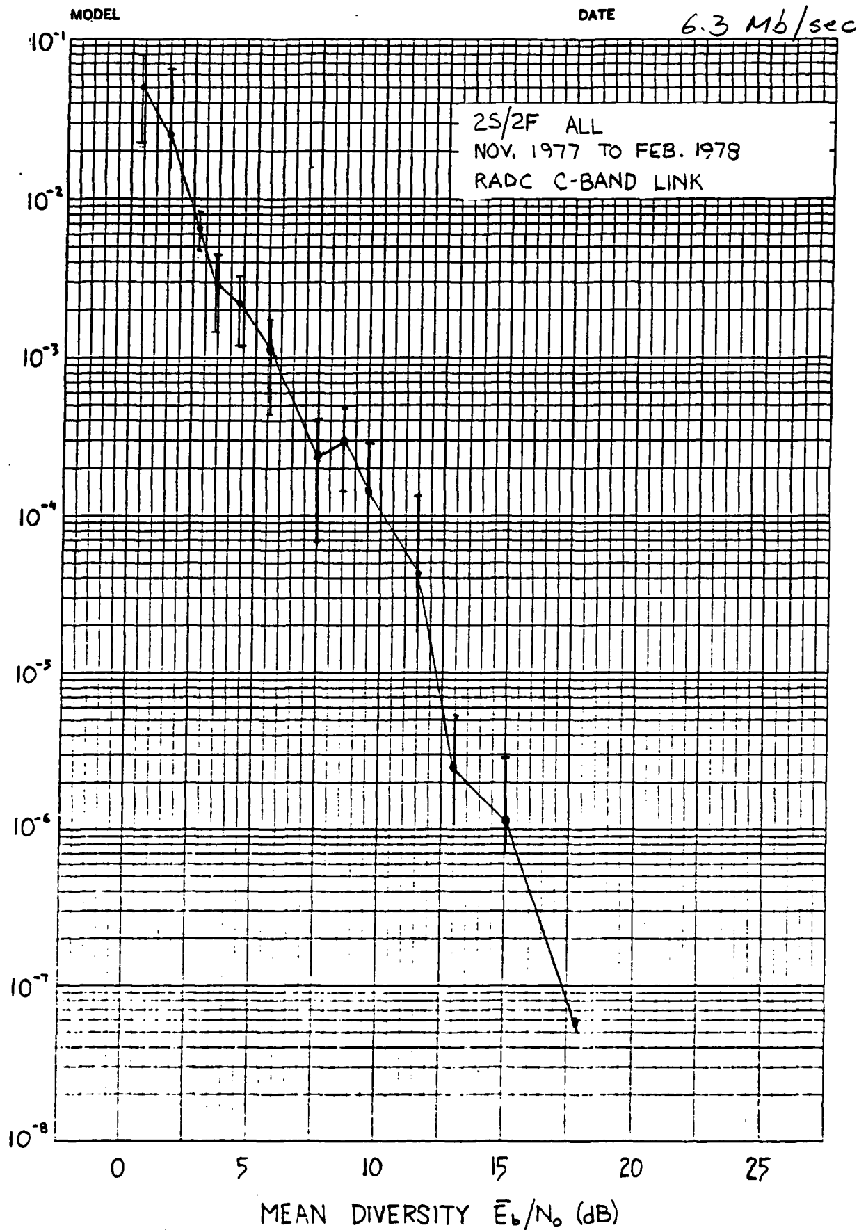
Fig. 4.10 All 2S/2F Data
