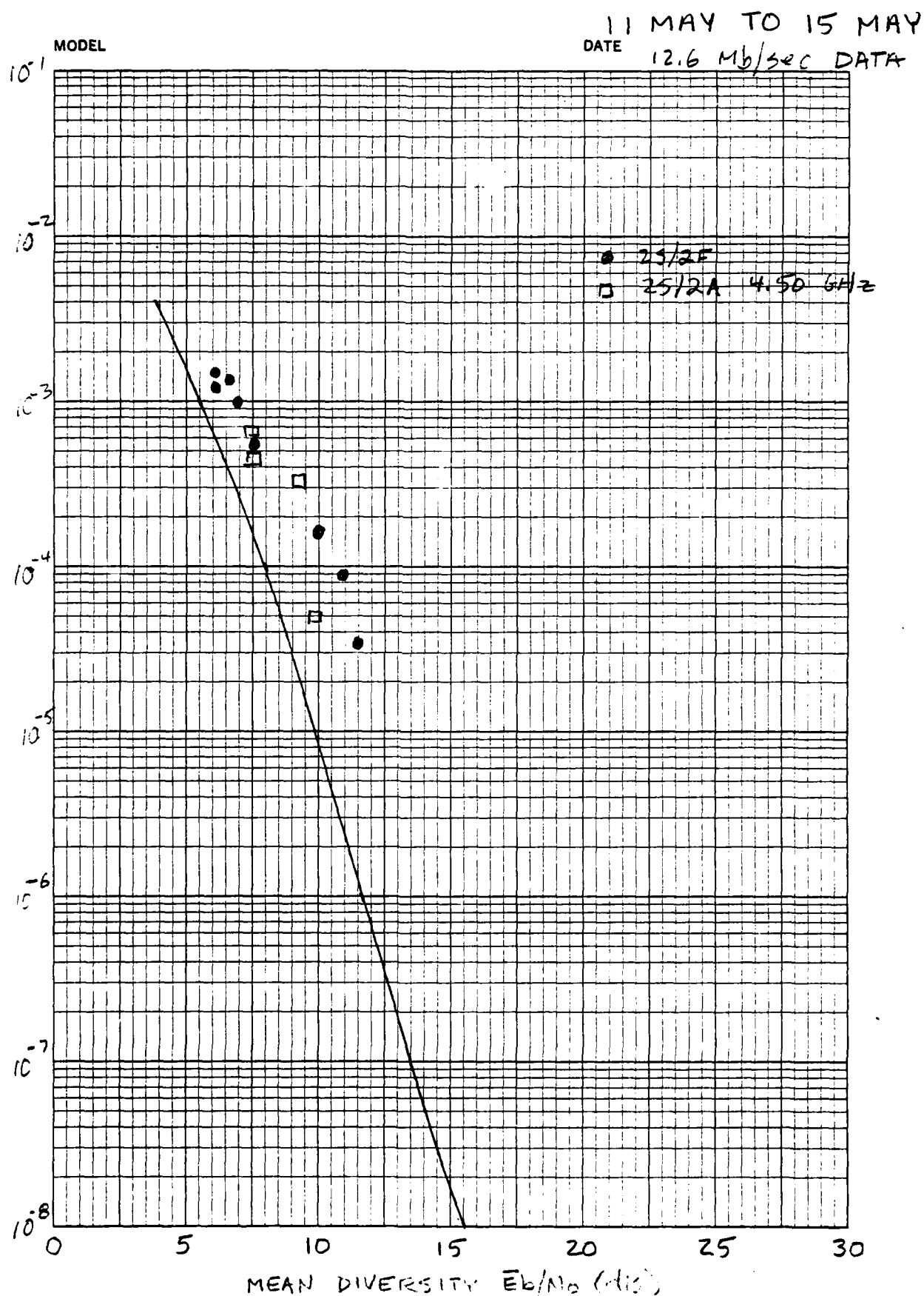
Fig. 5.6 12.6 Mb/s BER Data: 11 May to 15 May
