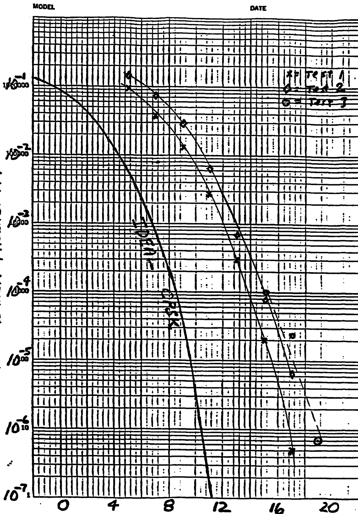
Fig 3. E_b/N_0 dB Experimental RF Loopback Results
