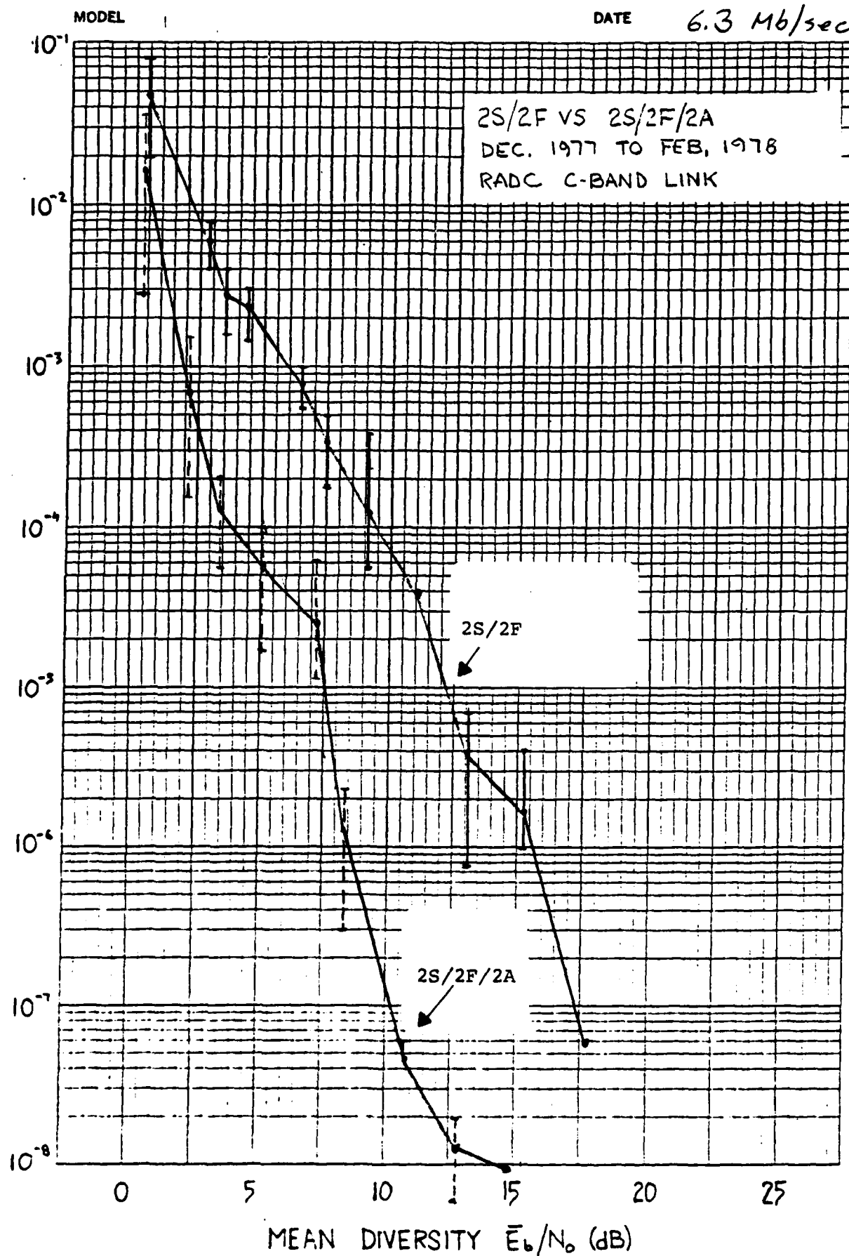
Fig. 4.13 2S/2F vs. 2S/2F/2A
