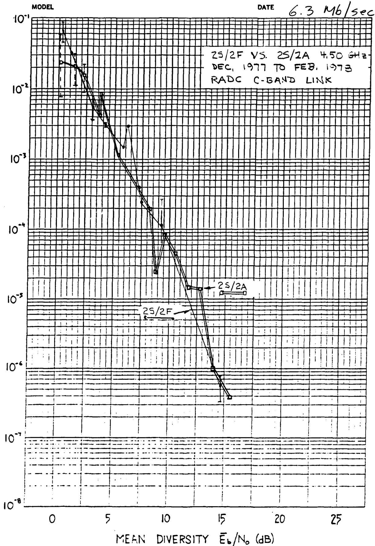
Fig. 4.12 2S/2F vs. 2S/2A 4.50 GHz
