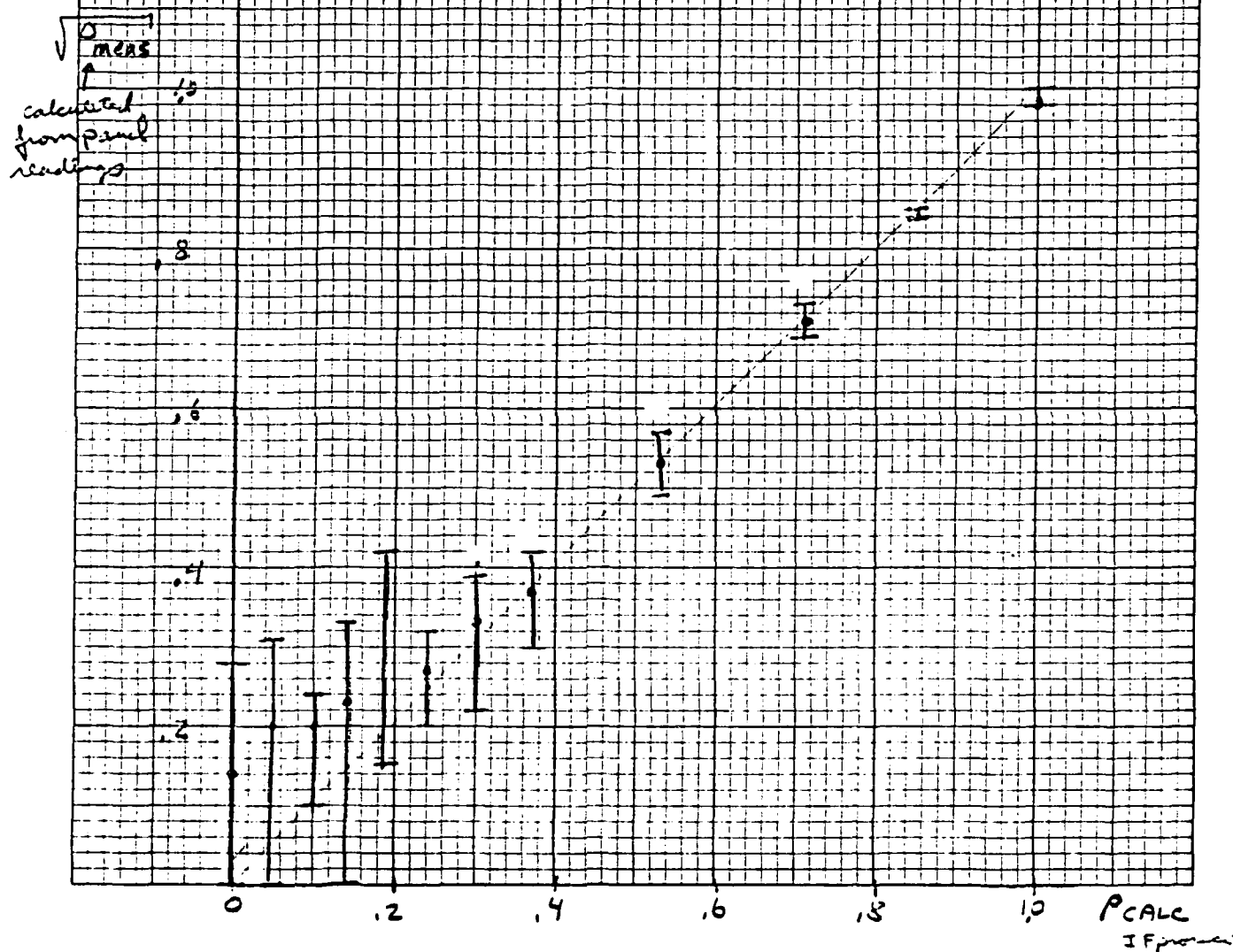
Fig. 2.13 Measured vs. Calculated Correlation Coefficient
