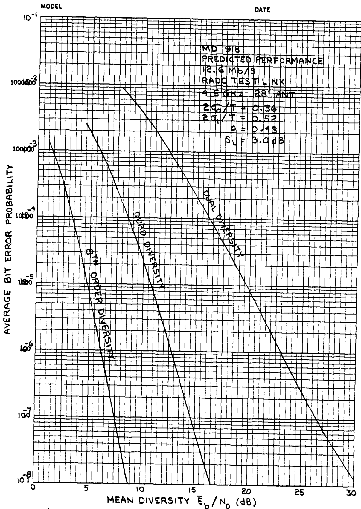
Fig. 2.9 Predicted Performance: C-Band 12.6 Mb/s
