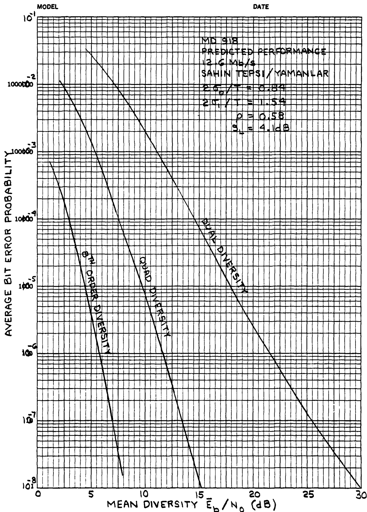
Fig. 2.11 Predicted Performance: L-Band 12.6 Mb/s
