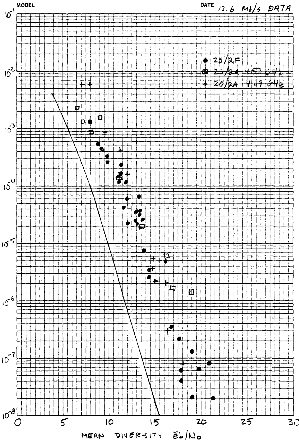
Fig. 5.7 12.6 Mb/s BER Data: After 15 May
