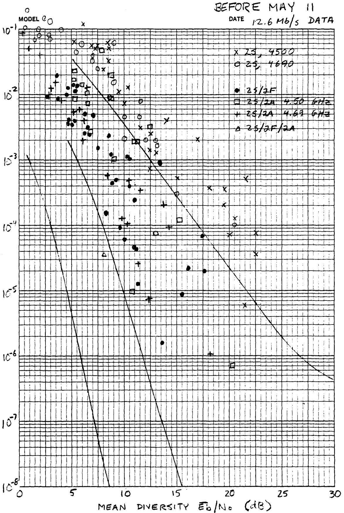
Fig. 5.5 12.6 Mb/s BER Data: Before 11 May
