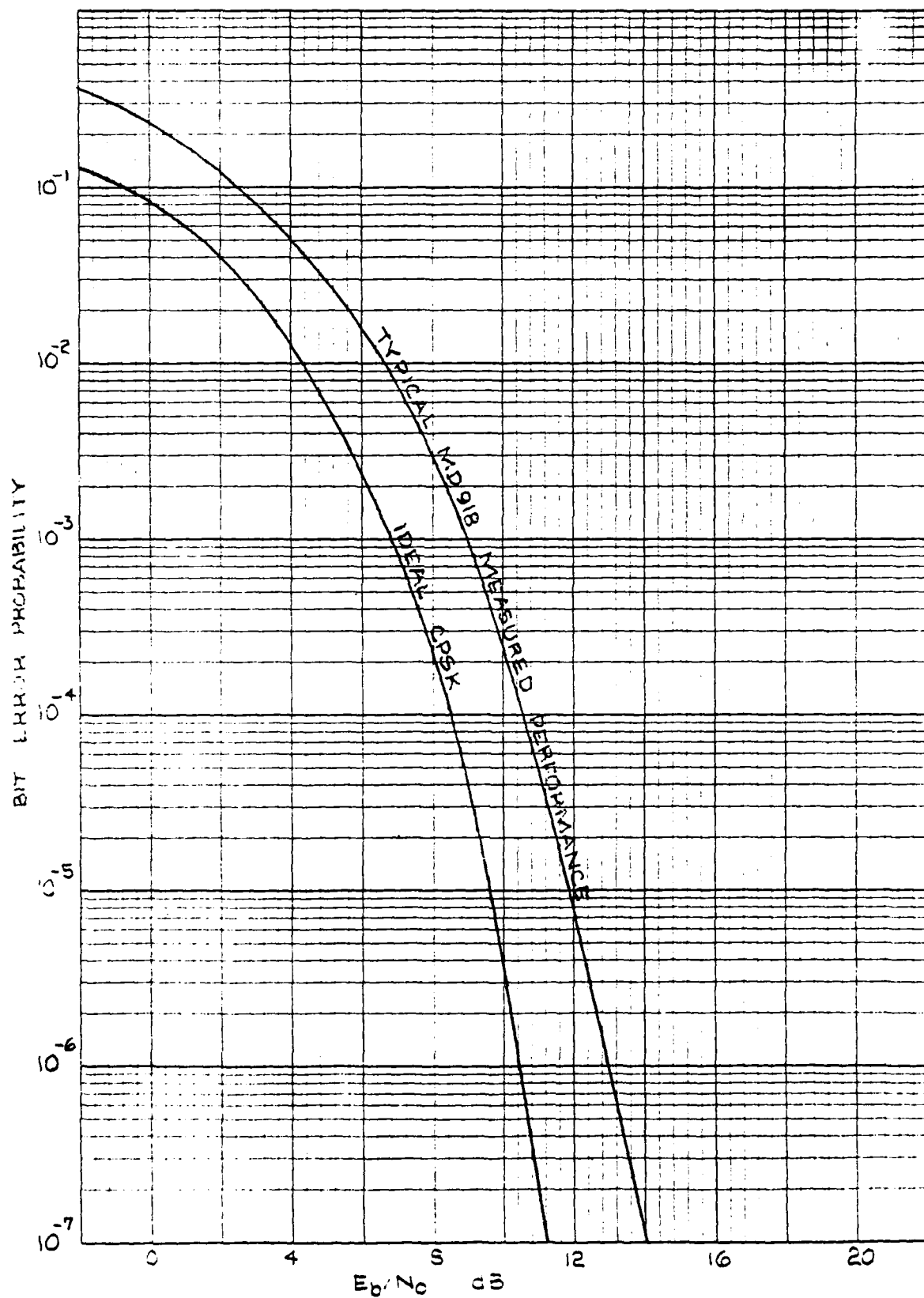
Fig. 2.1 Non Fading Performance
