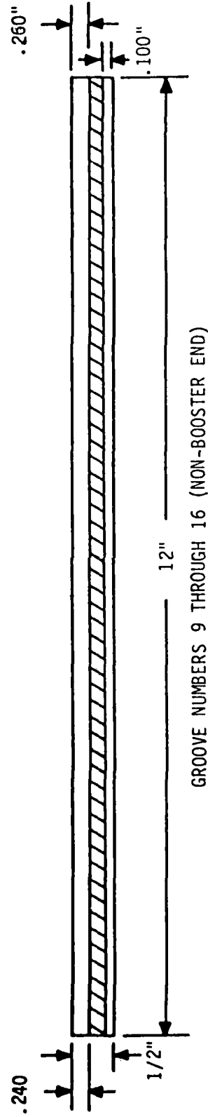
CIRCUMFERENTIAL GROOVE DETAILS FOR SSS-100 STEEL
