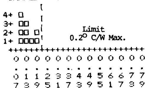
Fig. 41 Post Thermal Fatigue Thermal Impedance ( ^{\circ}\text{C/W} )
