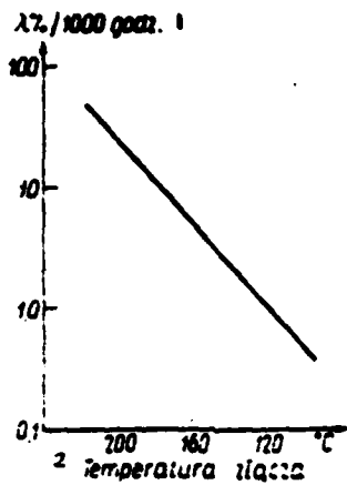
Fig. 6. A typical relationship between defect rate of elements of semiconductor (expressed in % per 1000 h) and temperature [14]. Key: 1 - h; 2 - Temperature of the joint.
