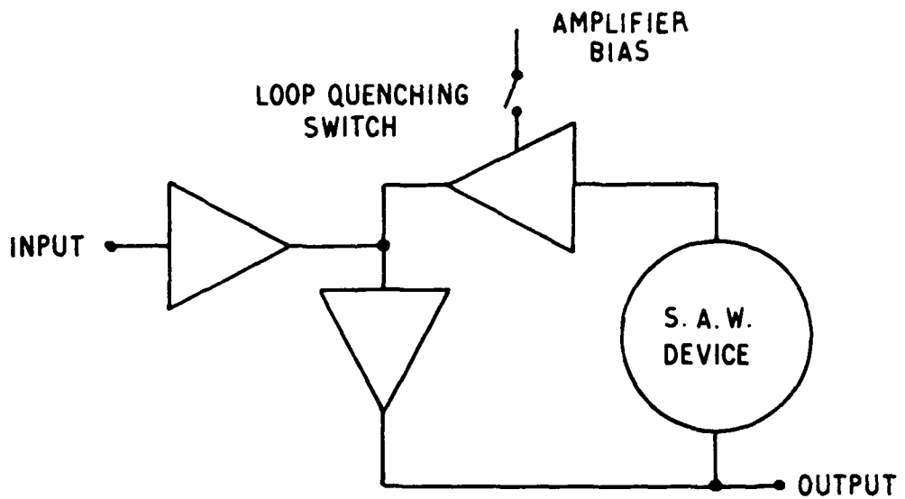
FIG. 1. TYPICAL MULTIMODE OSCILLATOR CONFIGURATION
