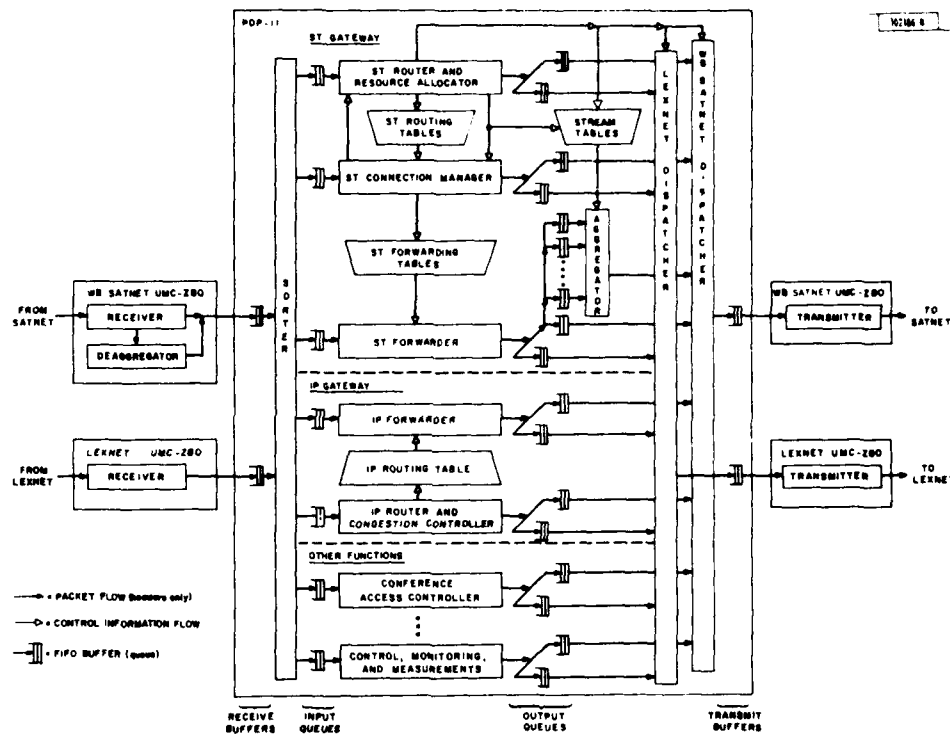
Fig. 17. Miniconcentrator functional block diagram.
