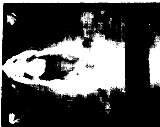
Figure 13. Schlieren Photograph, Test C6, Converging-Diverging Nozzle, L_E = 8.46 in.
