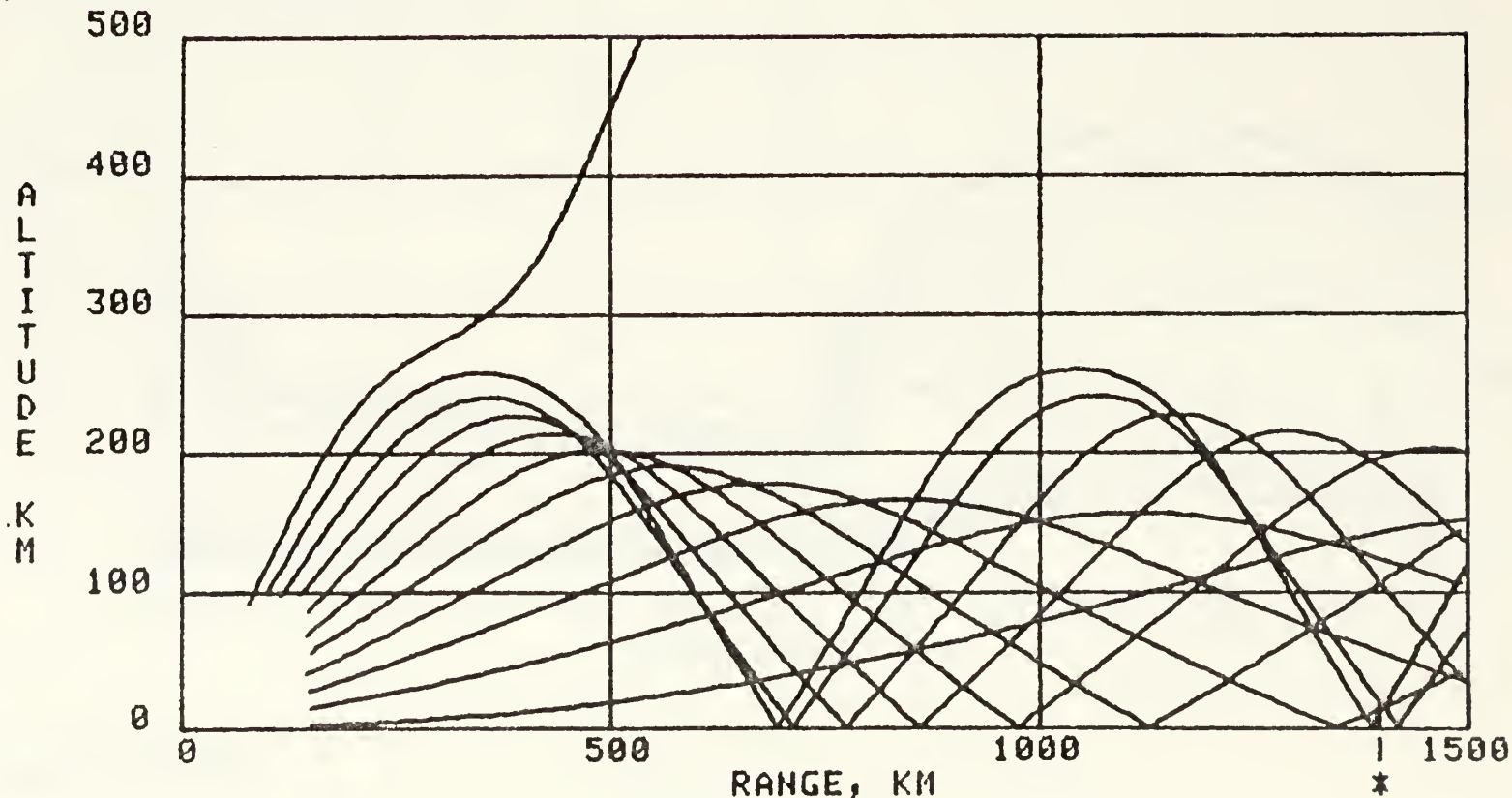
Figure 49 WWV 15 MHz 2/13/79 Ray Trace
