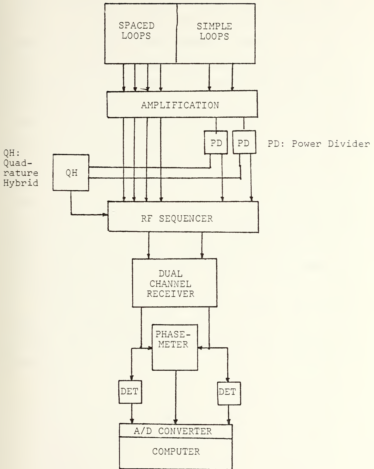
Figure 9 Block Diagram of SWRI Spaced Loop Antenna System Instrumentation
