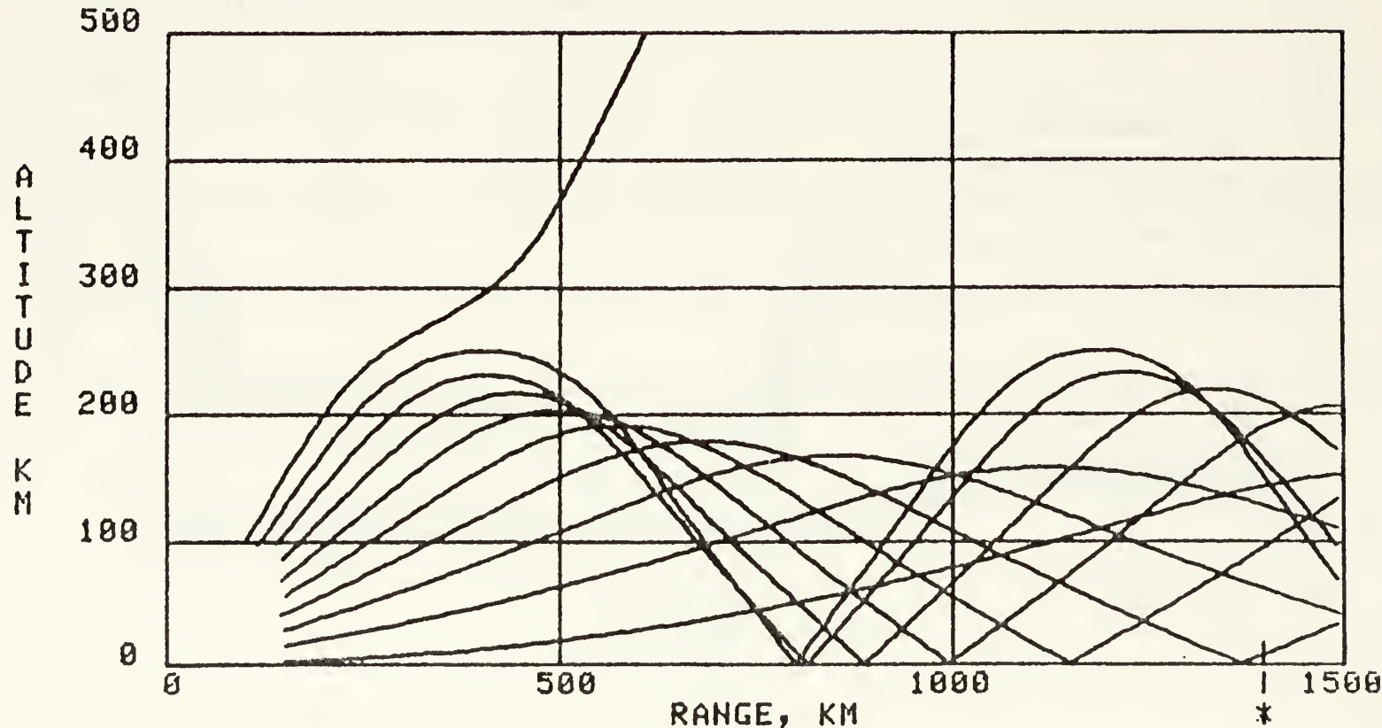
Figure 46 WWV 15 MHz 2/5/80 Ray Trace
