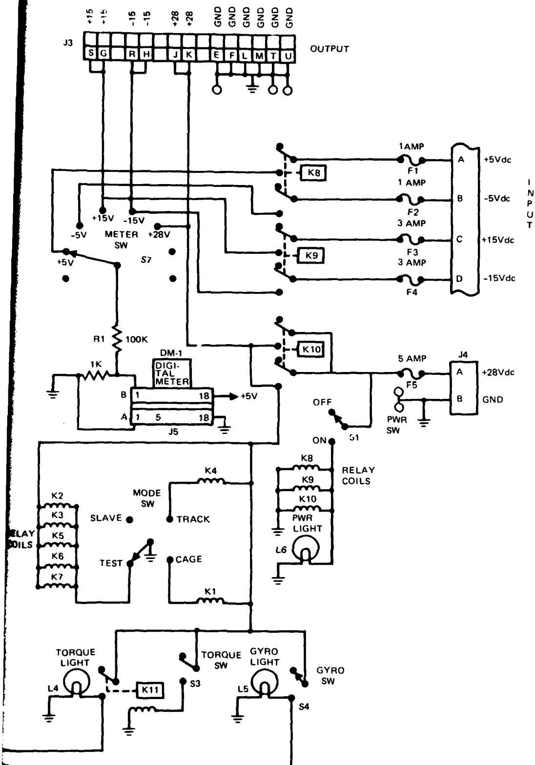
Figure 5. Control panel schematic.
