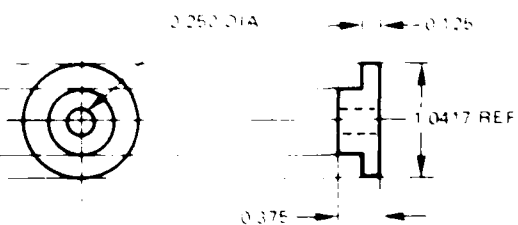
DETAIL (6) PINION
