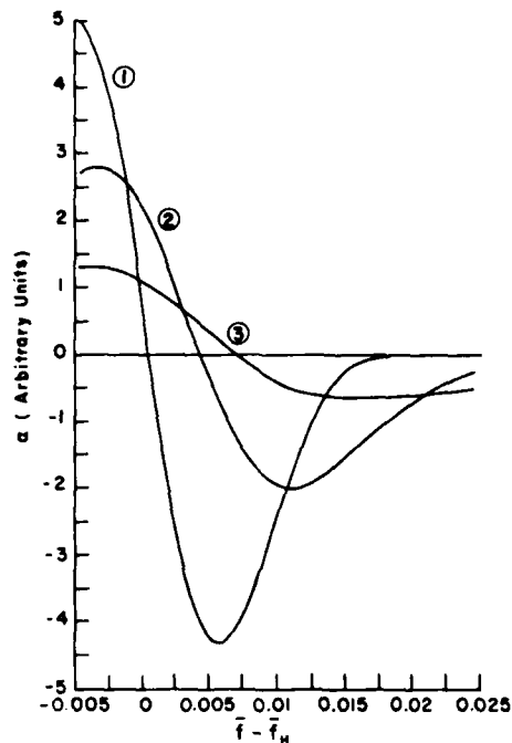
Fig. 5 - \langle \alpha \rangle as a function of (\bar{f} - \bar{f}_H) for three different values of energy spread: (1) \Delta W_b / W_{b0} = 0 , (2) \Delta W_b / W_{b0} = 0.1 and (3) \Delta W_b / W_{b0} = 0.2 . Other parameters assumed are n = s = m = 1 , r_0 = 0.48R , L/R = 0.1 , L/\lambda = 1.0 , and \beta_{10}/\beta_{z0} = 1.5 .
