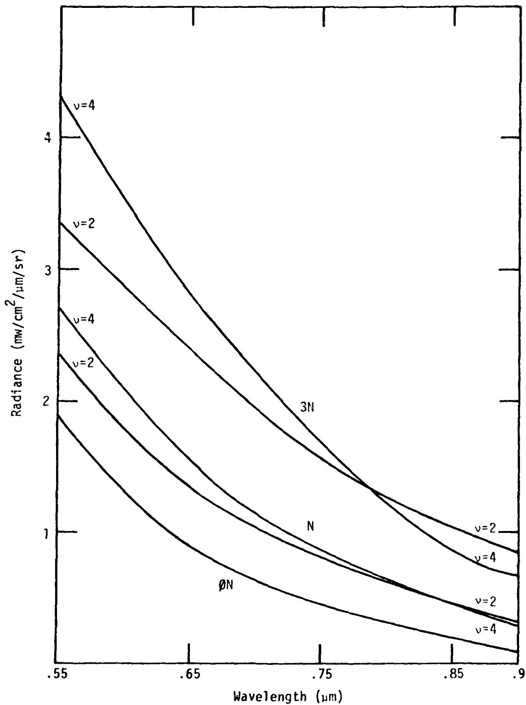
Figure 5. Theoretical Radiance Versus Wavelength as Function of Aerosol Content and Size Distribution (Nadir-viewing with Sun Zenith Angle of 63°).
