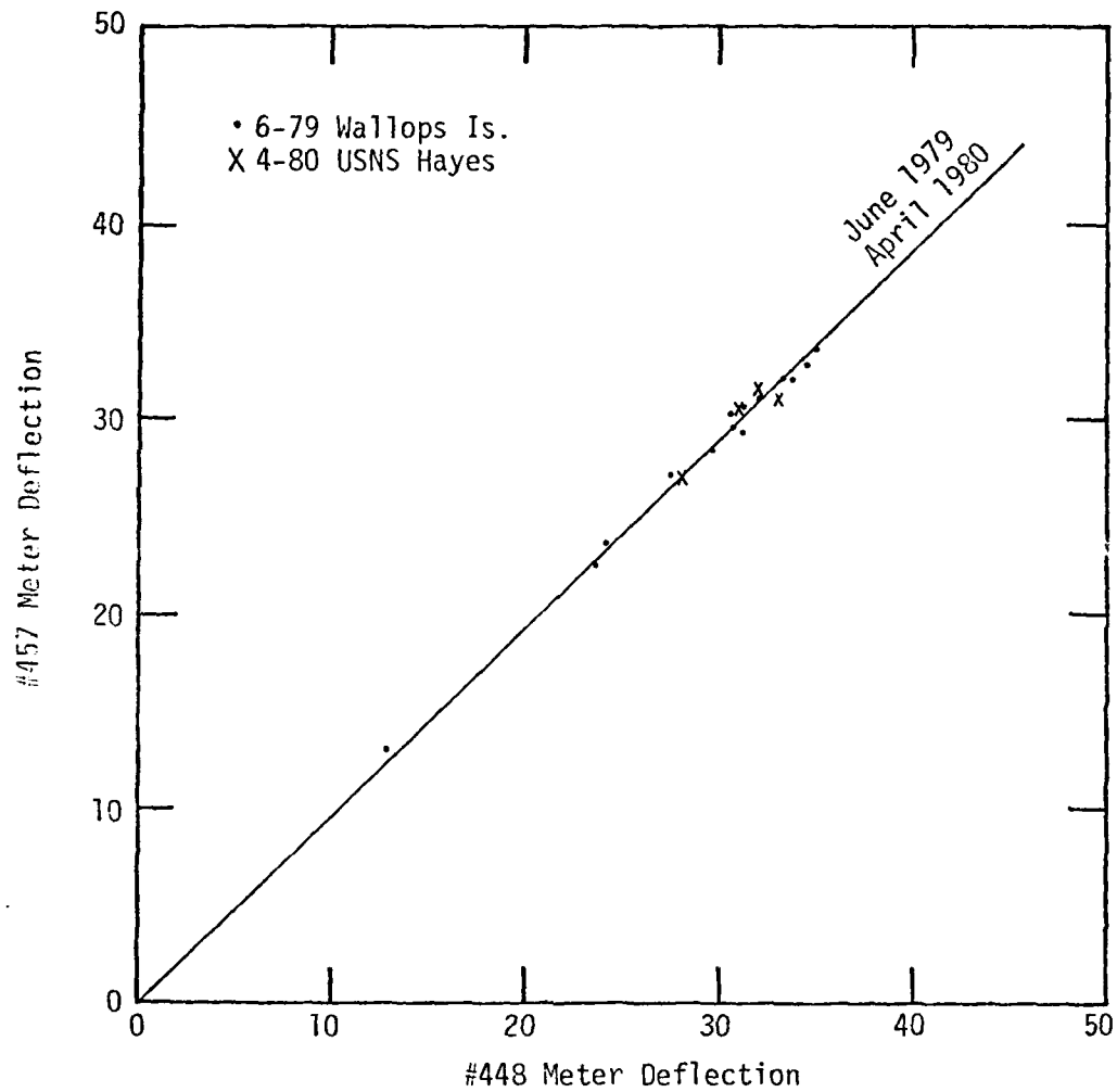
Figure 1. Comparison of NRL Sunphotometers (500 nm).
