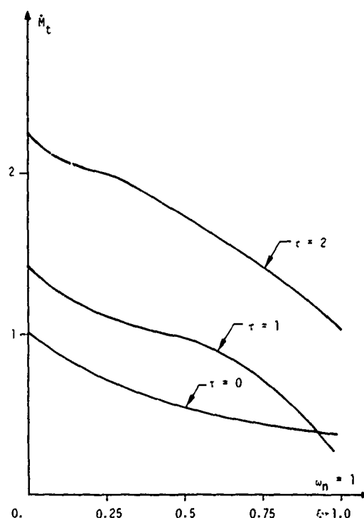
Fig. 9. Relationships among \hat{\omega}_t , \xi , \omega_n , and \tau shown in (10b).
