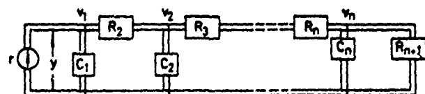
Fig. 2 Multiport RC ladder network
