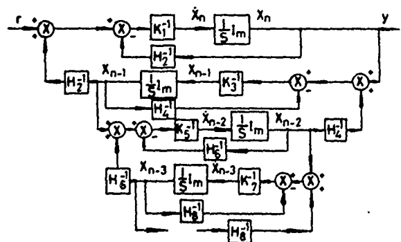
Fig. 1 Block diagram representation of the block-state equation in eqn. 8
