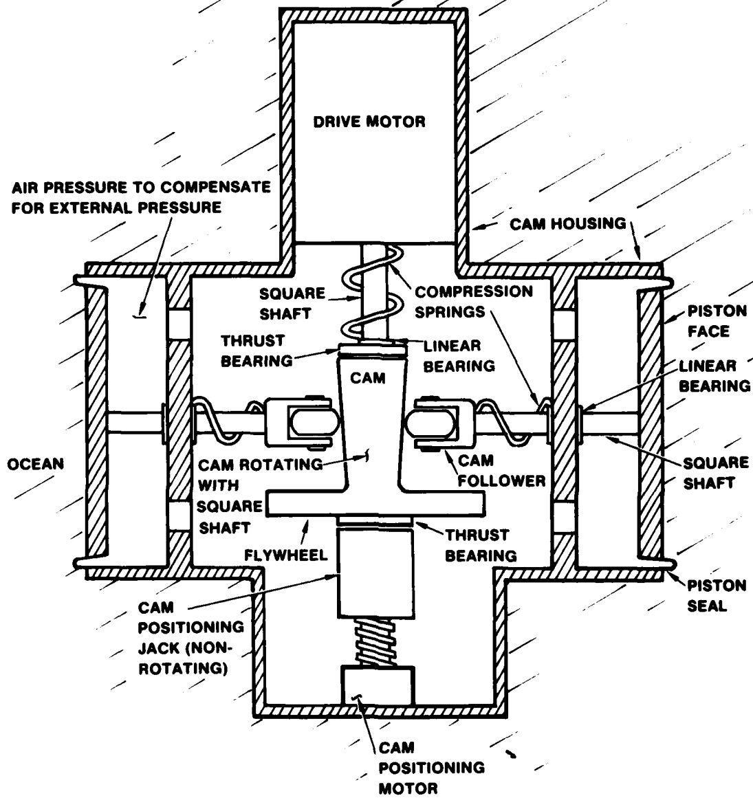
Figure 2. Second conceptual design for NRAP.
