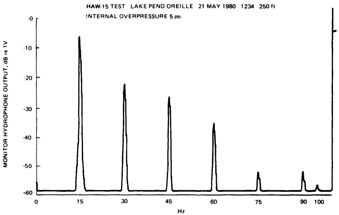
Figure A8. In-water test at 250-foot depth.
