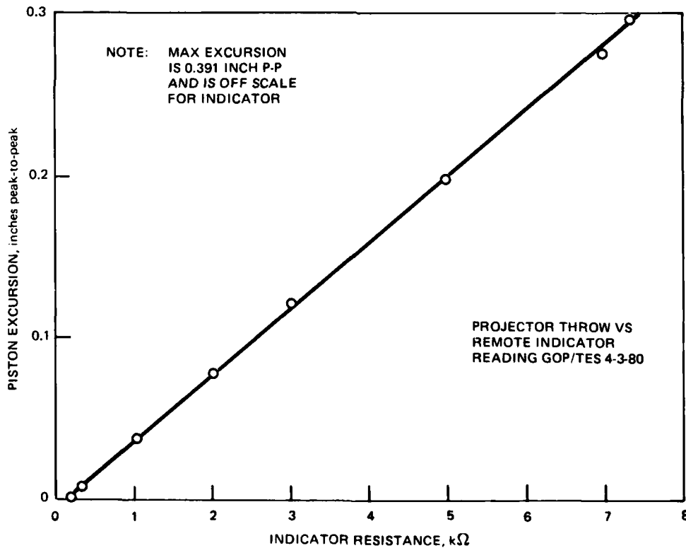
Figure 6. Piston throw vs linear transducer resistance.
