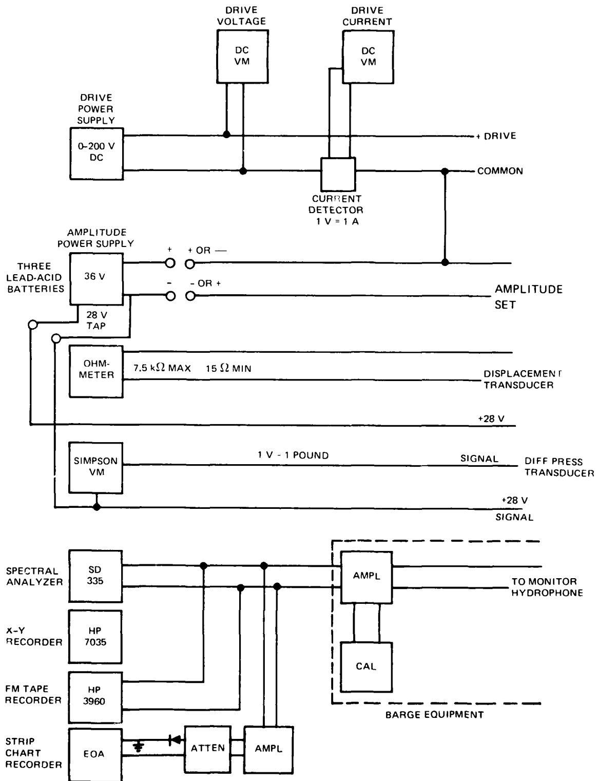
Figure A3. Test setup.
