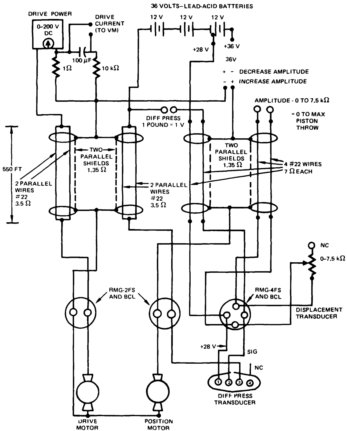
Figure A1. Electrical connections.
