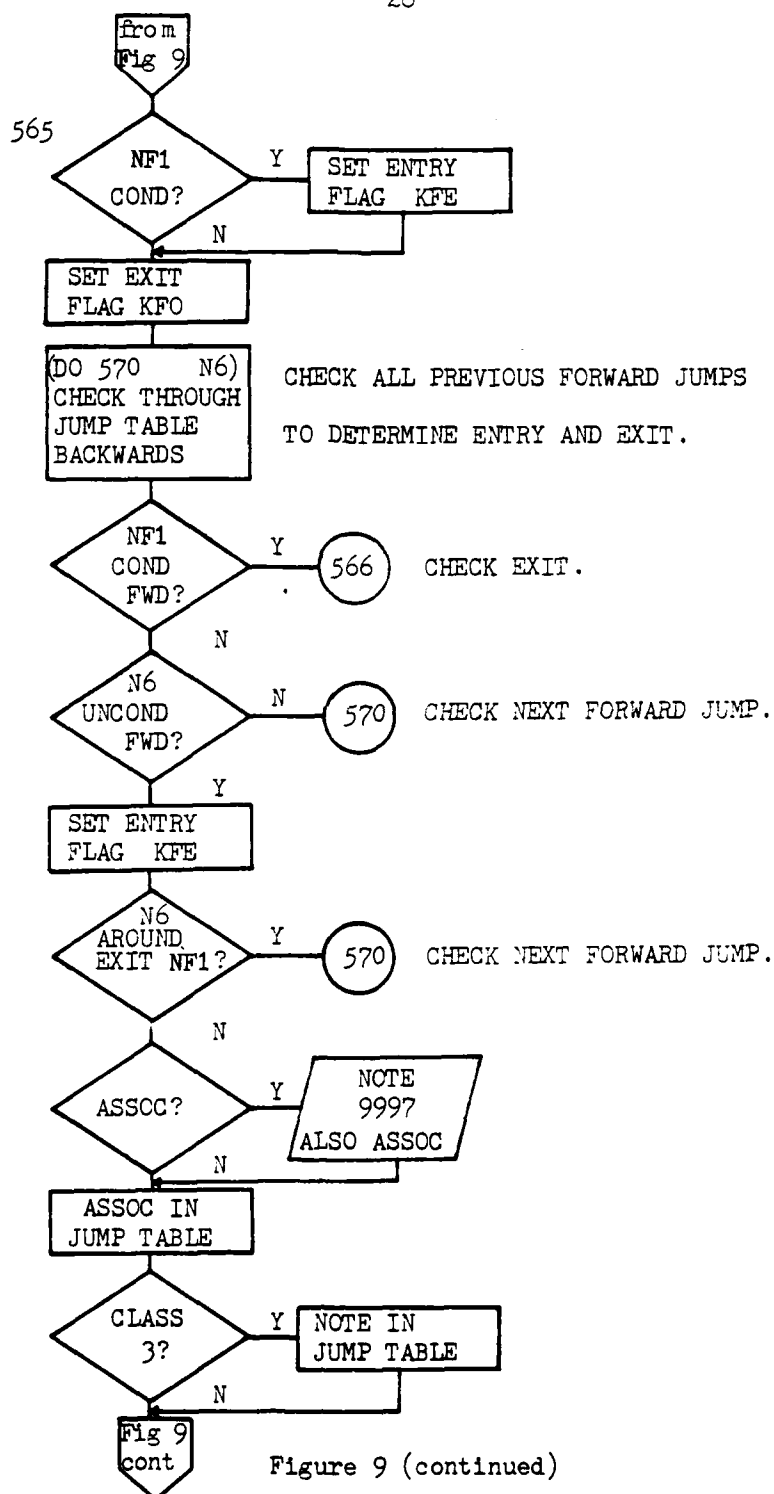
Flowchart for Checking Loop Constructs
