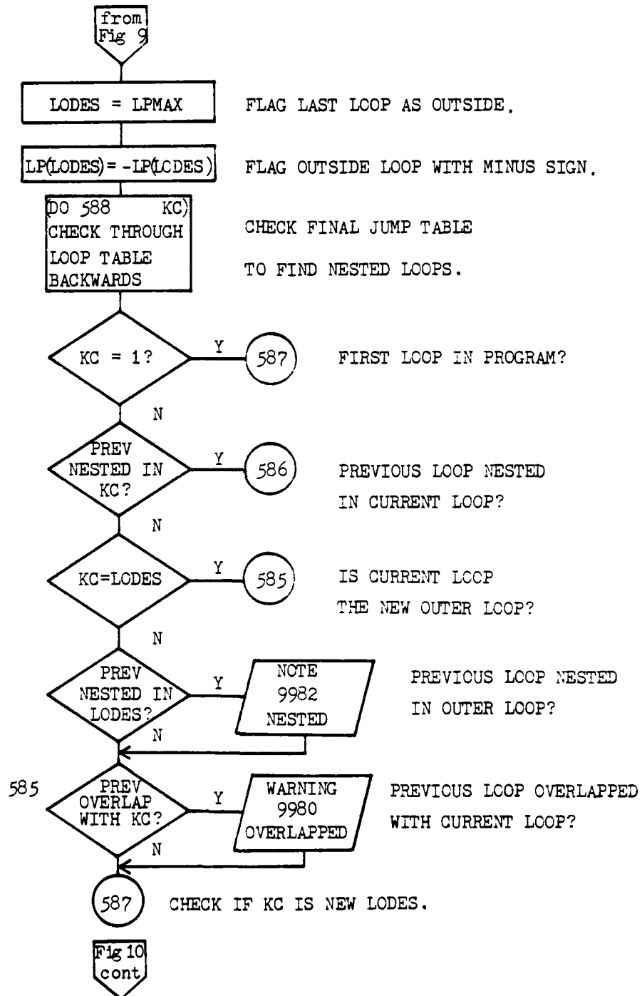
Figure 11 Flowchart for Nest Check
