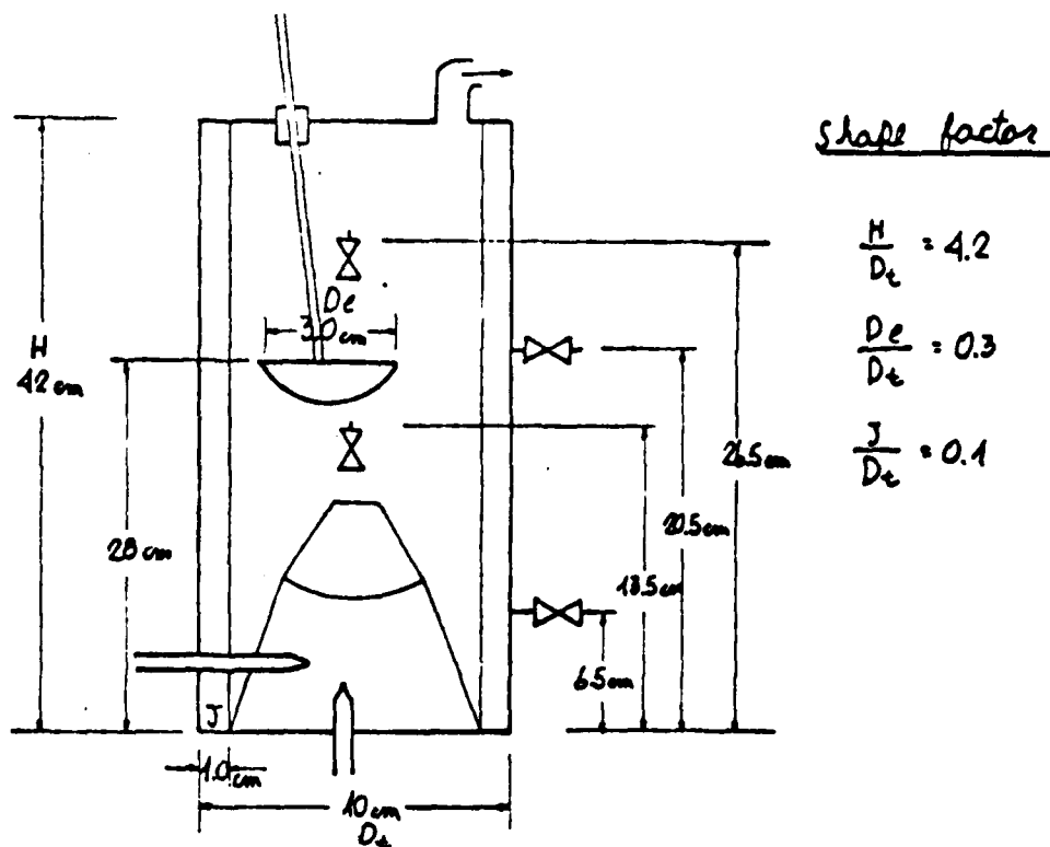
Fig. 10: The glass reactor
