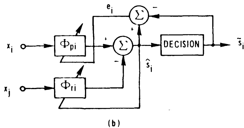
FIGURE 2.13. Dual-Filter Extractors for Dual-Channel Data Communications ( i = 1, 2 ; j = 1, 2 ; i \neq j )
