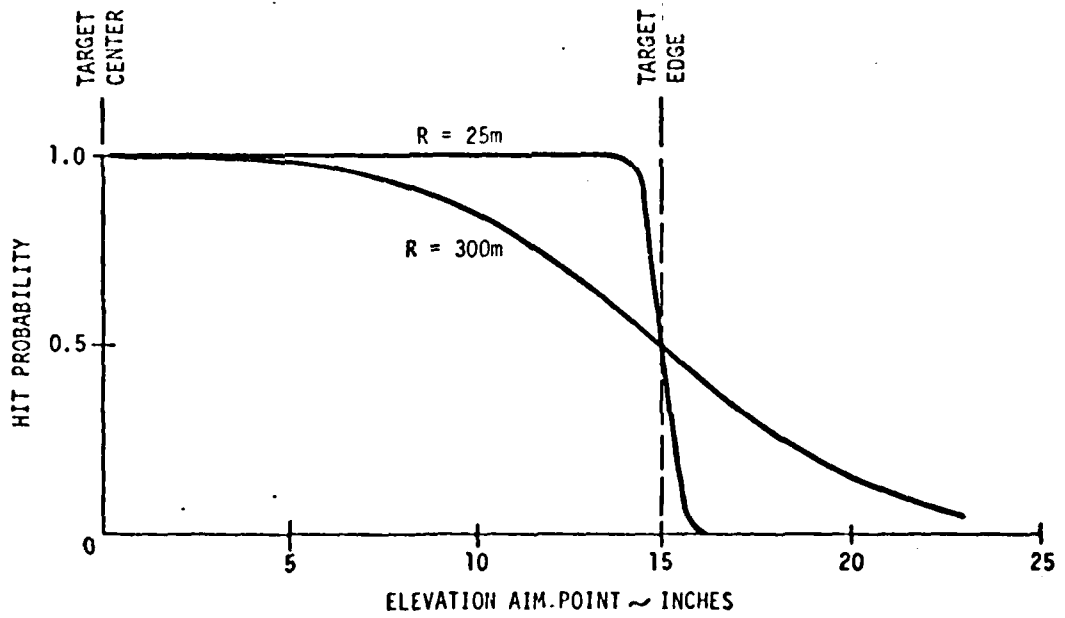
Figure 11. E-Target Hit Probability for the 0.4 m \sigma , 1 \sigma , Weapon Dispersion
