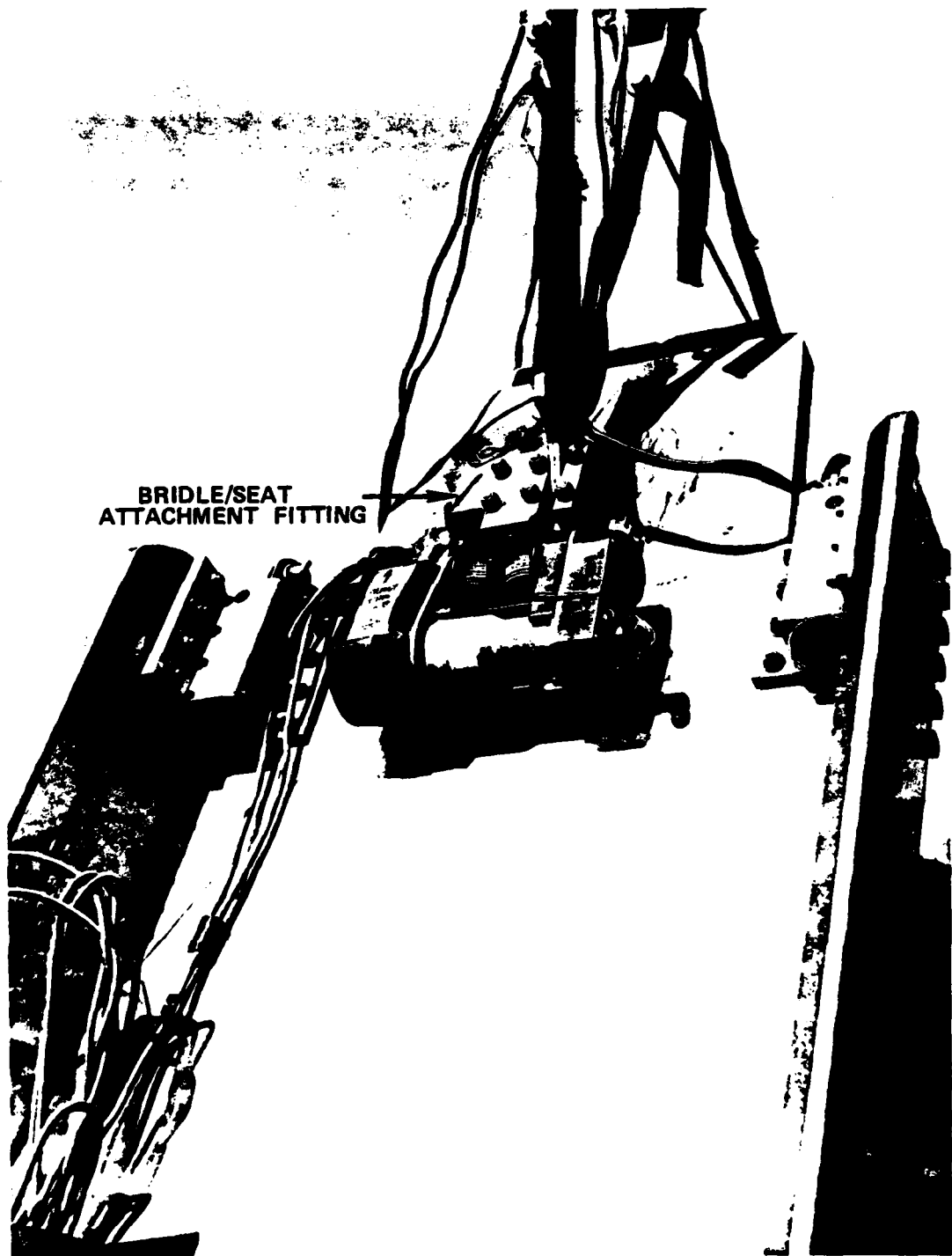
Figure D-3- Bridle/Seat Attachment Fitting Location for Pull Force Test
