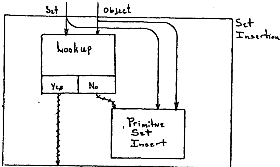
Figure 11: Plan for Set Insertion.
