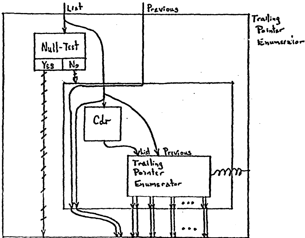
Figure 9: Plan diagram for 'Trailing Pointer Enumeration.
