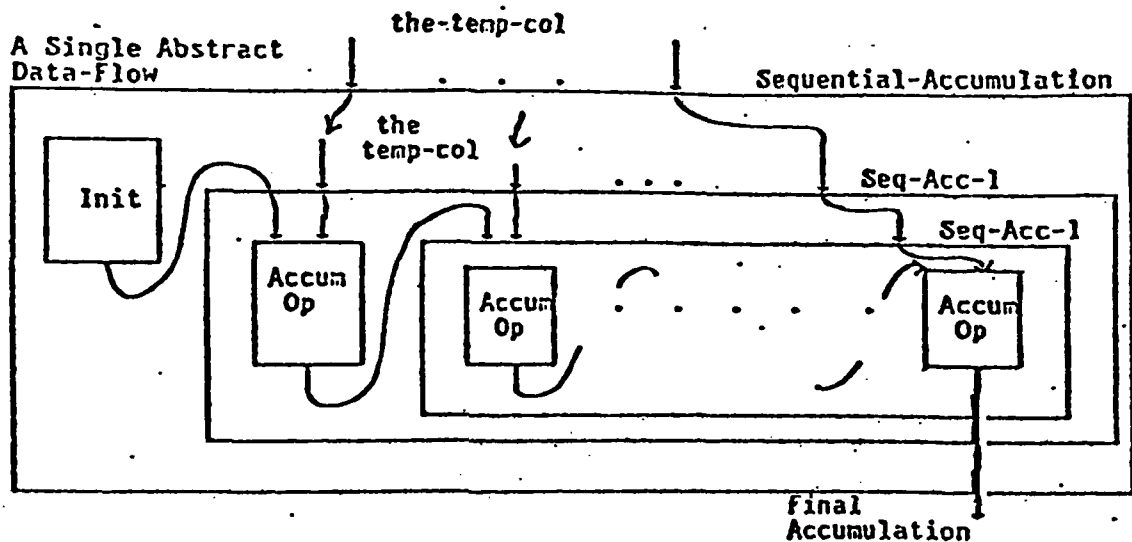
Figure 4: Sequential Accumulation with a Temporal Collection input.
