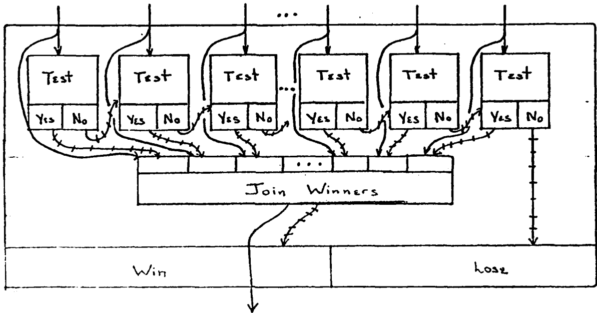
Figure 8: Plan diagram for Linear Search.
