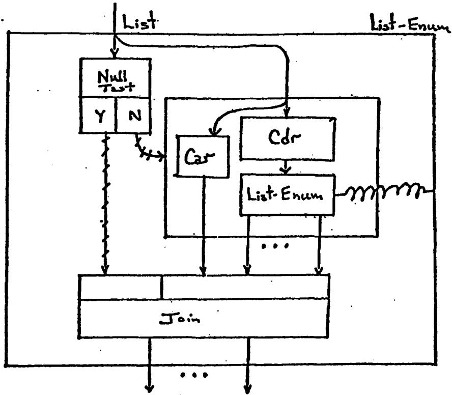
Figure 2: The plan diagram for List Enumeration.
