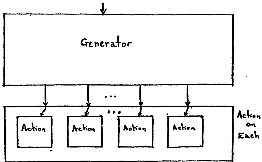
Figure 10: Plan diagram for Enumerate and Side-Effect Each.
