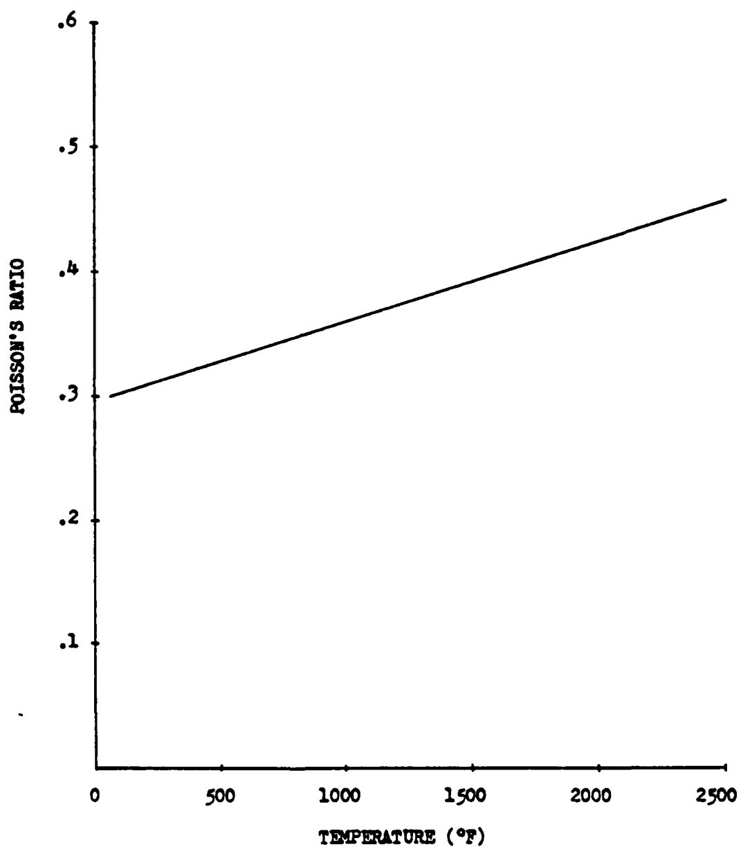
Figure 6- ESTIMATED EFFECT OF TEMPERATURE ON POISSON'S RATION FOR HY-130
