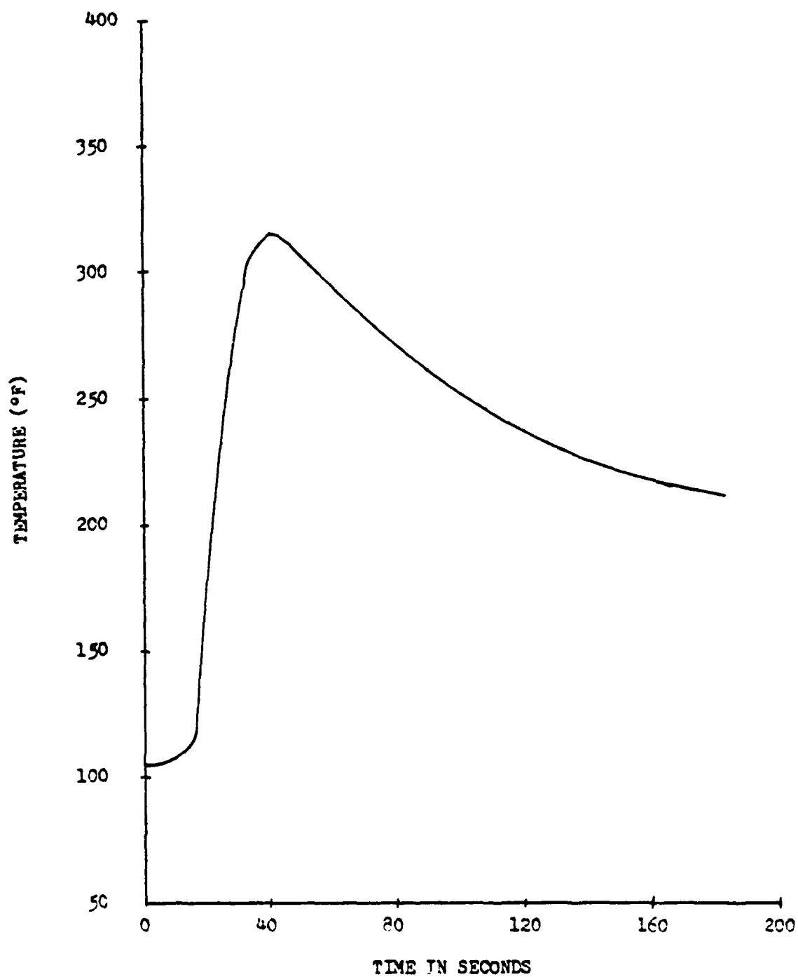
Figure 20- HY 130 SPECIMEN II, TEMPERATURE VERSUS TIME .50" from WELD LINE, PASS #2
