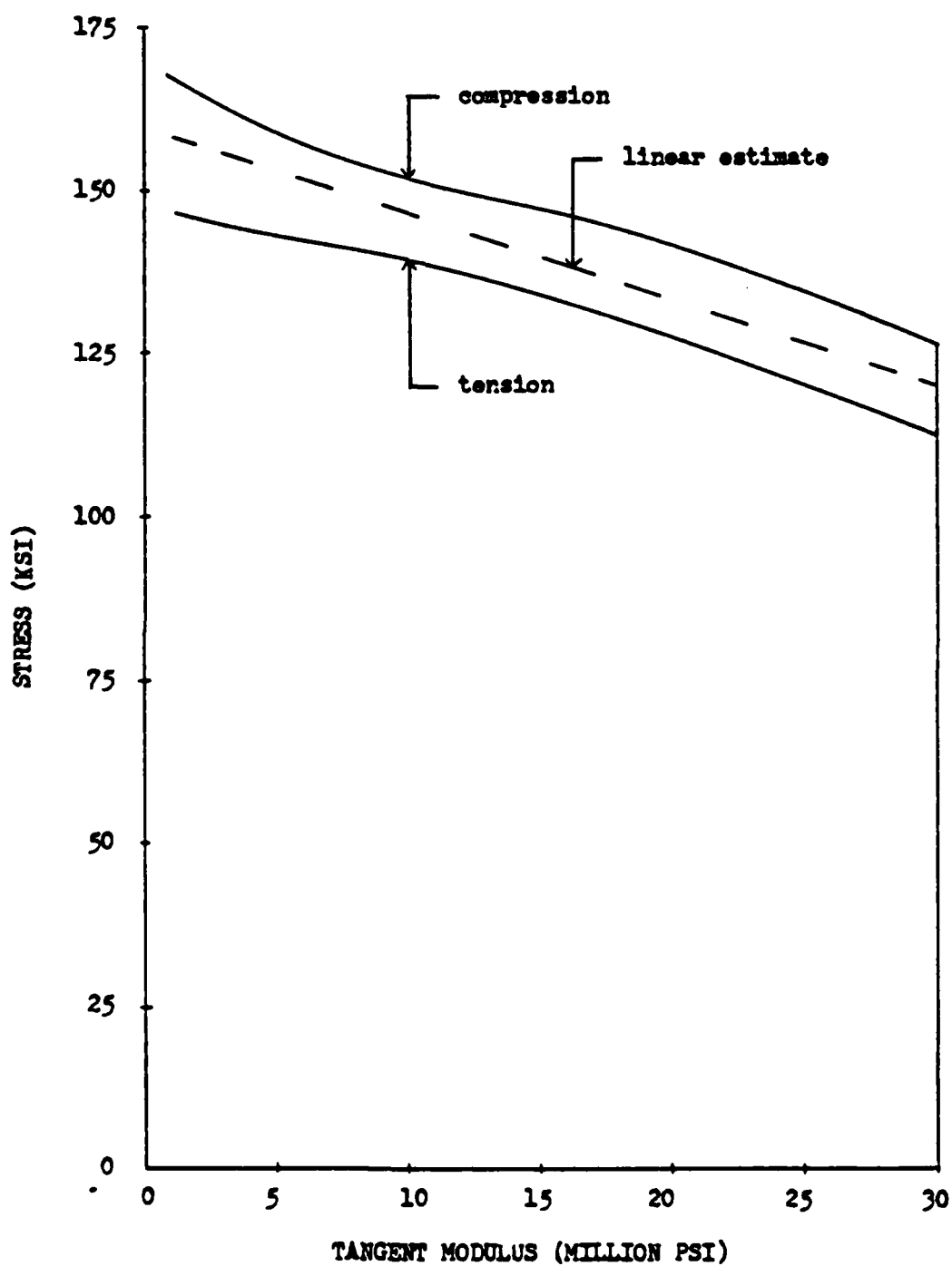
Figure 4- TANGENT MODULUS FOR HY-130
