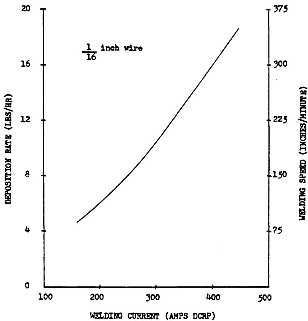
Figure 38- GMA DEPOSITION RATES
