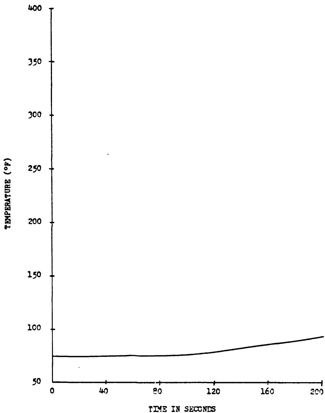
Figure 19- HY 130 SPECIMEN II, TEMPERATURE VERSUS TIME
