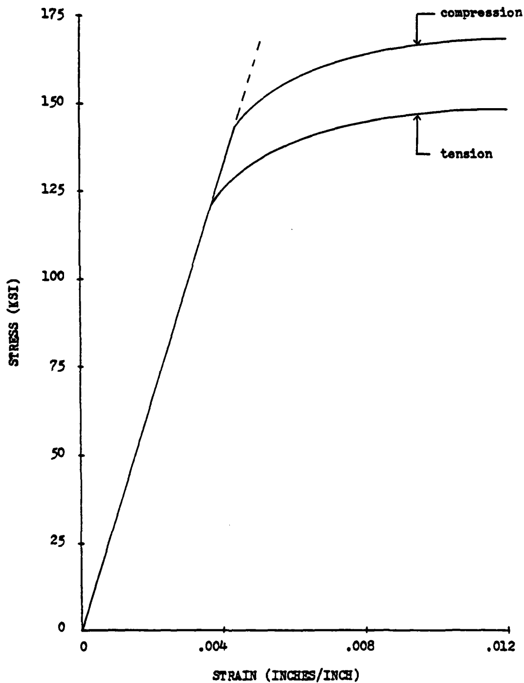
Figure 1- TYPICAL STRESS STRAIN DIAGRAM FOR HY-130 AT ROOM TEMPERATURE
