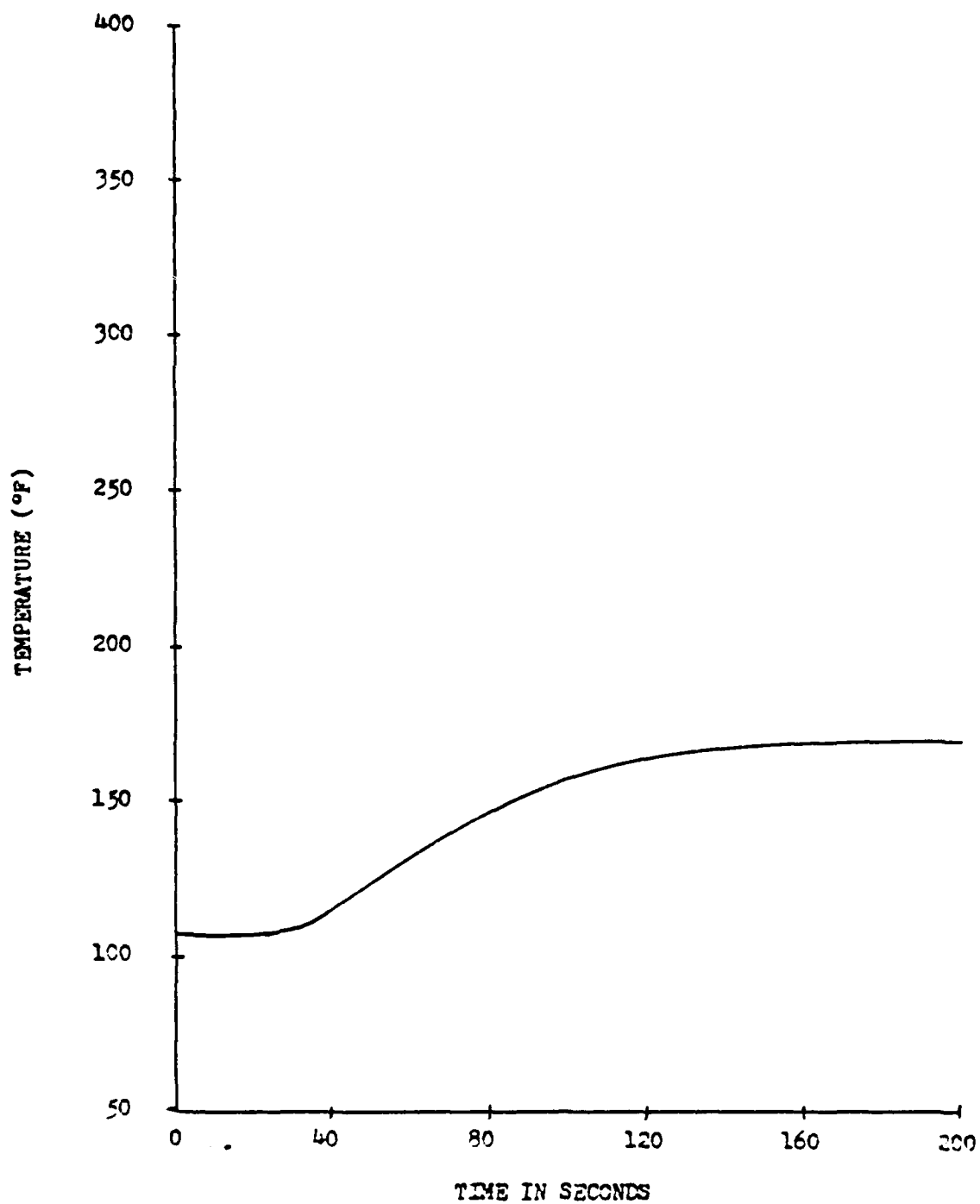
Figure 22- HY 130 SPECIMEN II, TEMPERATURE VERSUS TIME 2.25" from WELD LINE, PASS #2
