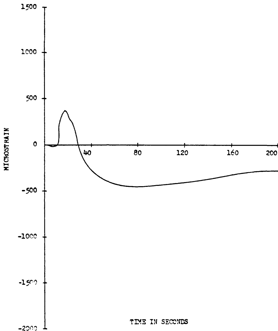
Figure 25- HY 100 SPECIMEN II, LONGITUDINAL STRAIN VERSUS TIME 1.25" from WELD LINE, PASS #1
