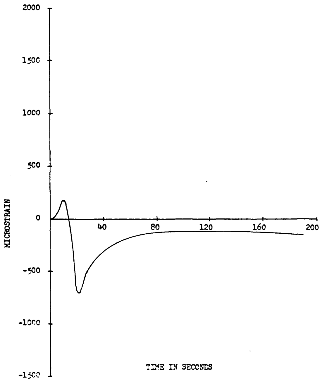
Figure 34- HY 130 SPECIMEN II, TRANSVERSE STRAIN VERSUS Time 1.25" from WELD LINE, PASS #2
