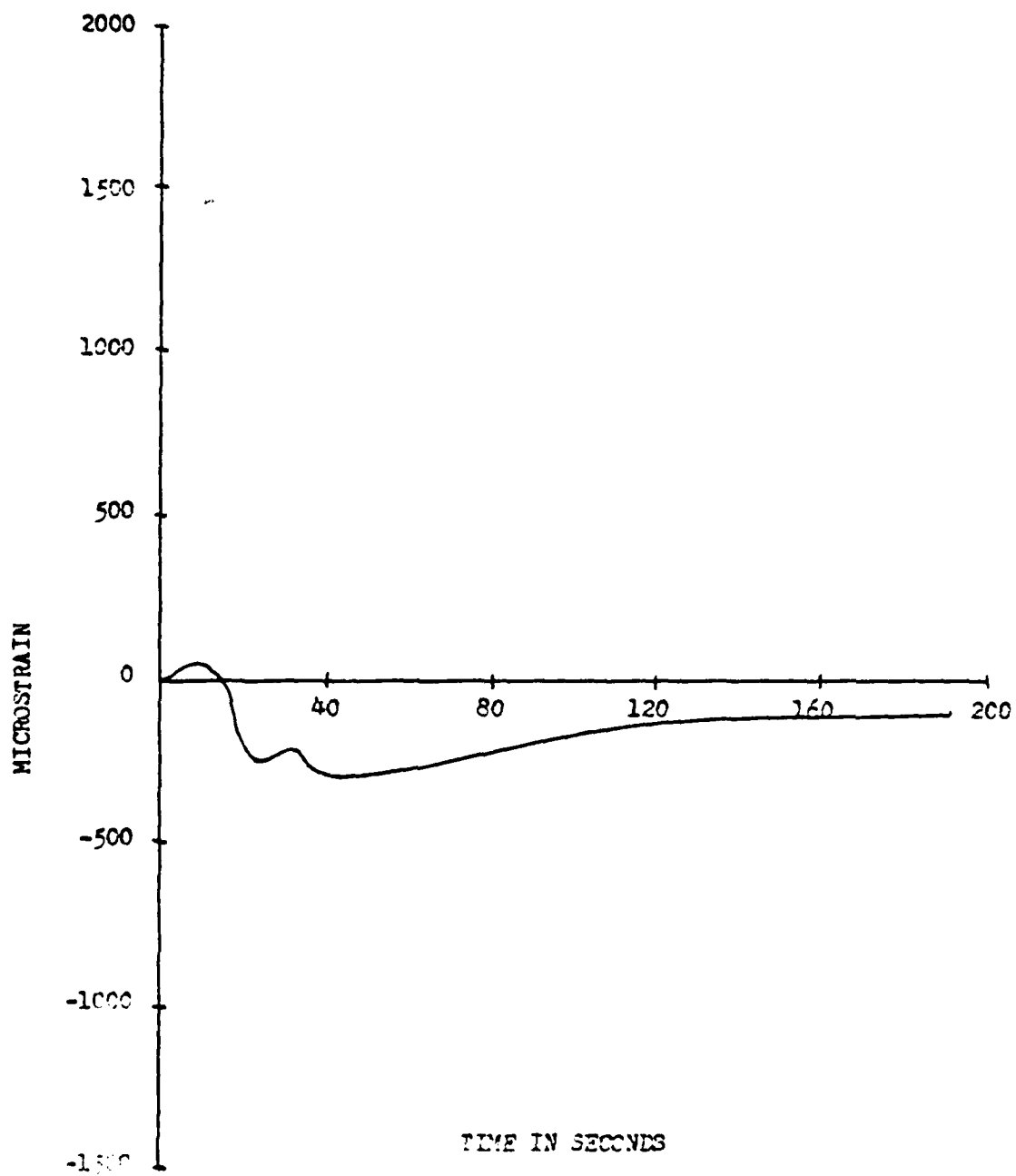
FIGURE 35- SPECIMEN II, TRANSVERSE STRAIN VERSUS TIME 0.15" FROM WELD LINE, PASS #2
