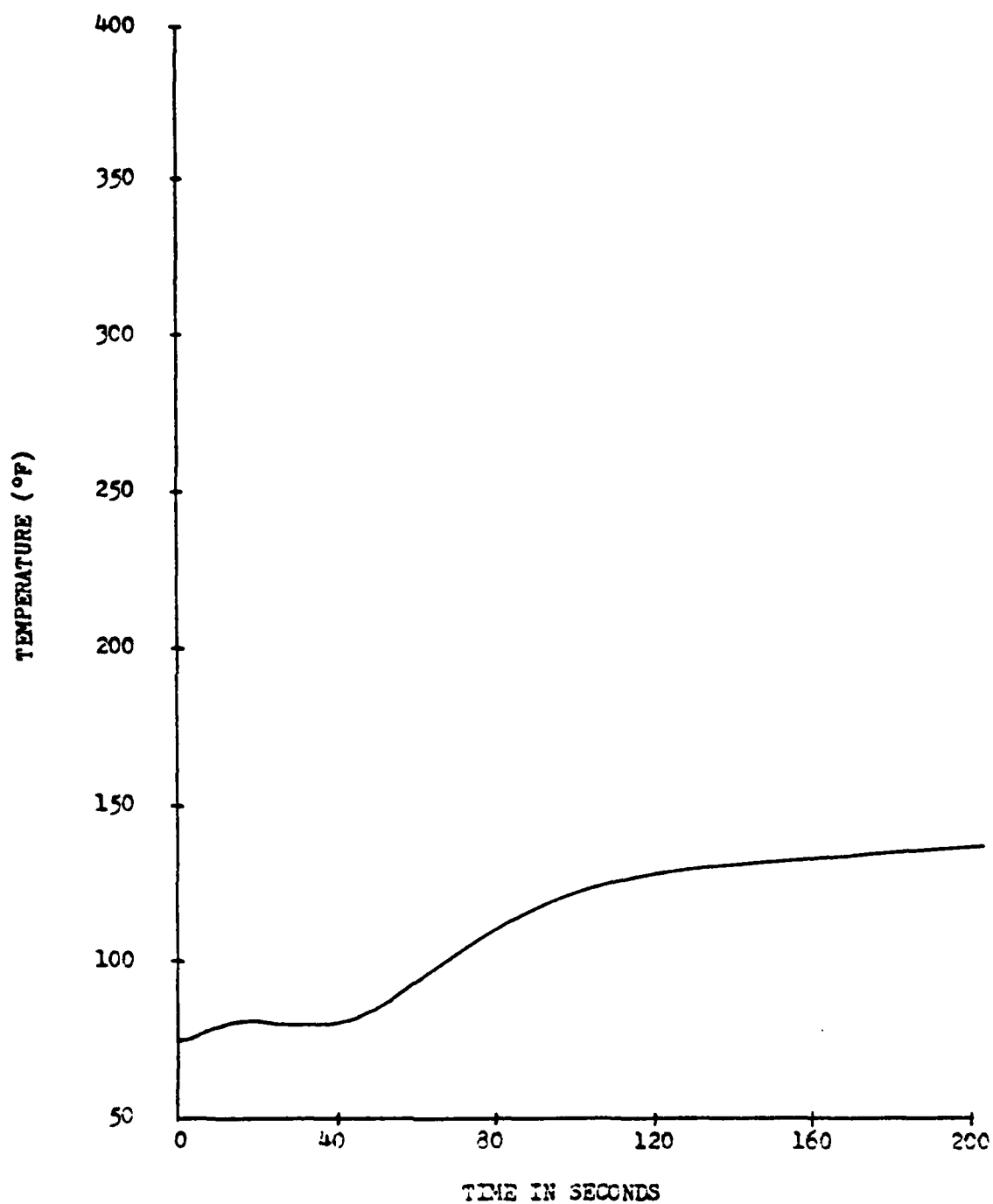
Figure 18- HY 130 SPECIMEN II, TEMPERATURE VERSUS TIME 2.25" from WELD LINE, PASS #1
