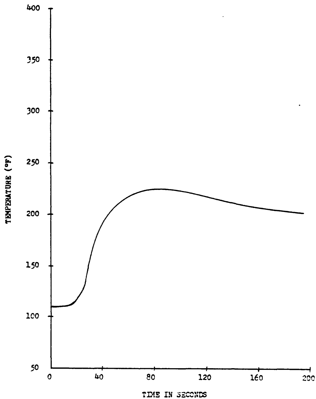
Figure 21- HY 130 SPECIMEN II, TEMPERATURE VERSUS TIME 1.25" from WELD LINE, PASS #2
