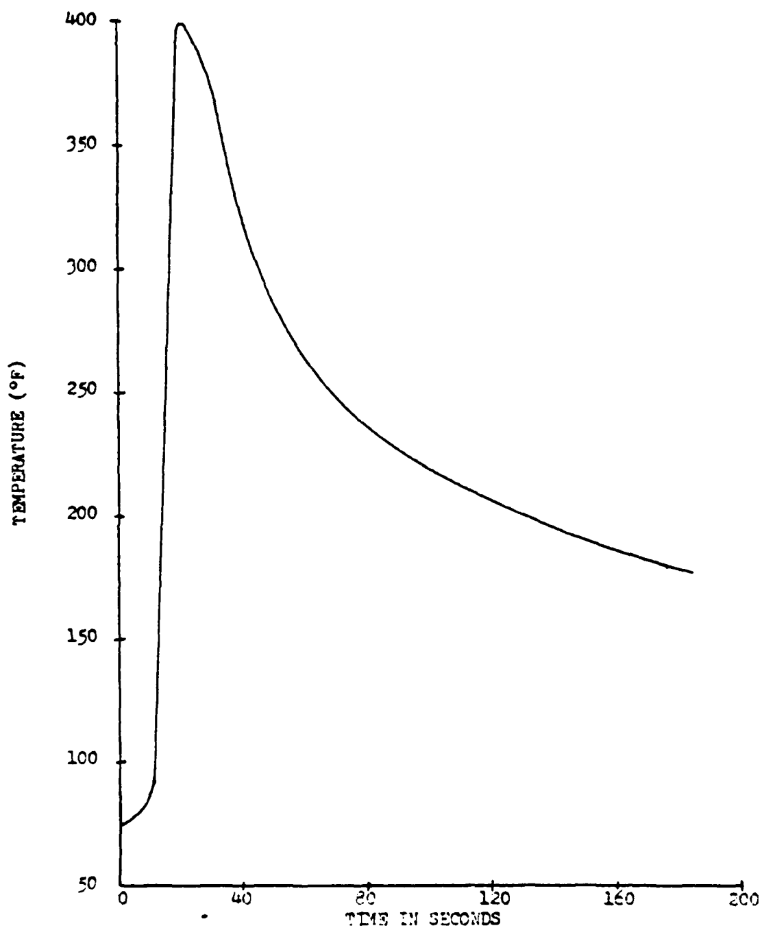
Figure 16-HY 130 SPECIMEN II, TEMPERATURE VERSUS TIME .50" from WELD LINE, PASS #1
