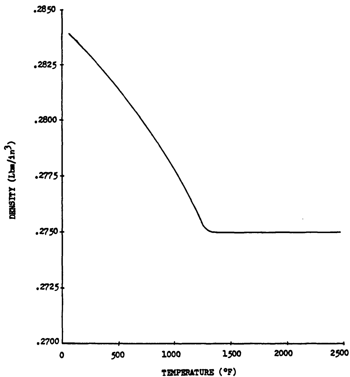
Figure 8- ESTIMATED EFFECT OF TEMPERATURE ON DENSITY FOR HY-130
