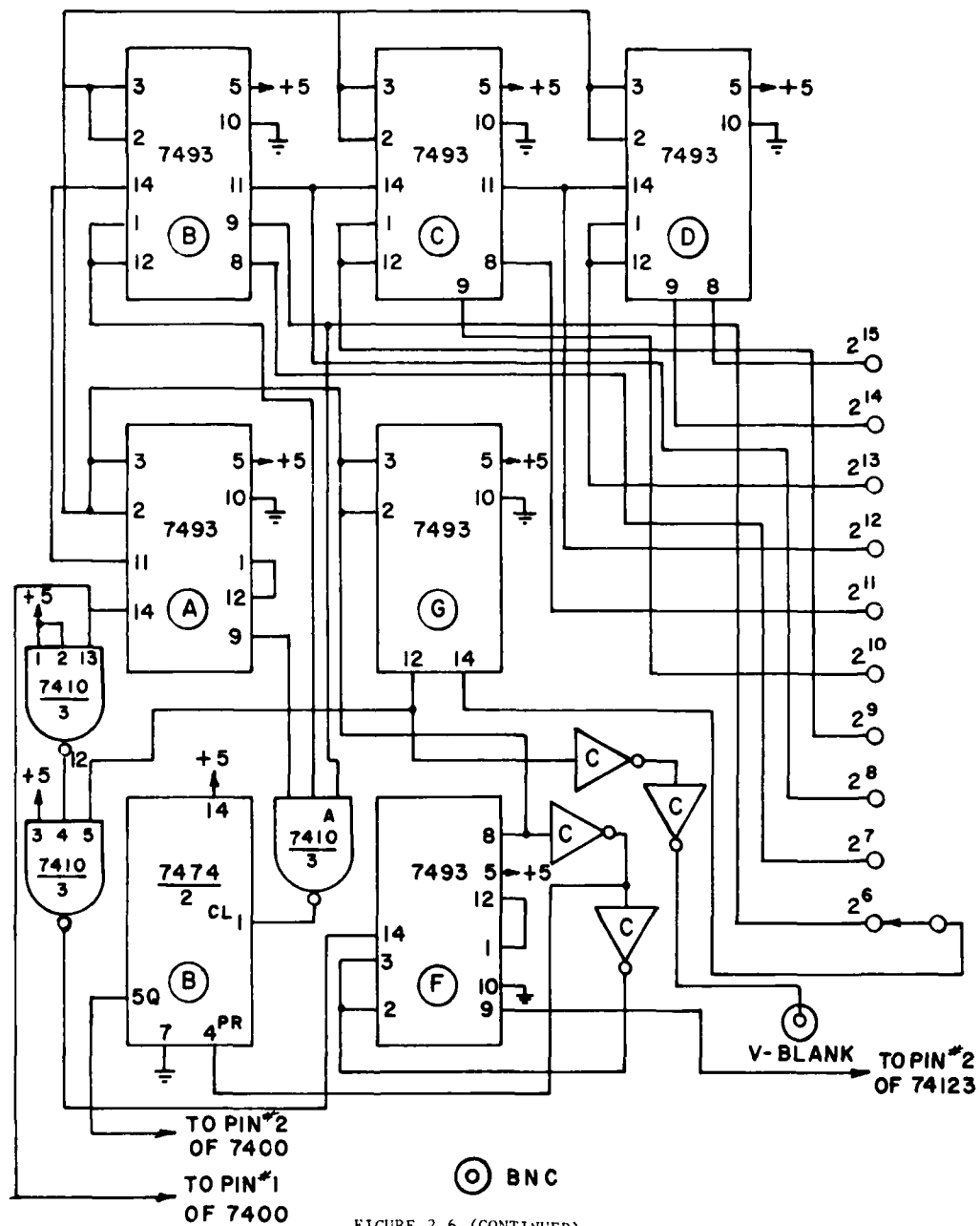
FIGURE 2.6 (CONTINUED) MODULE 2AB DIAGRAM
