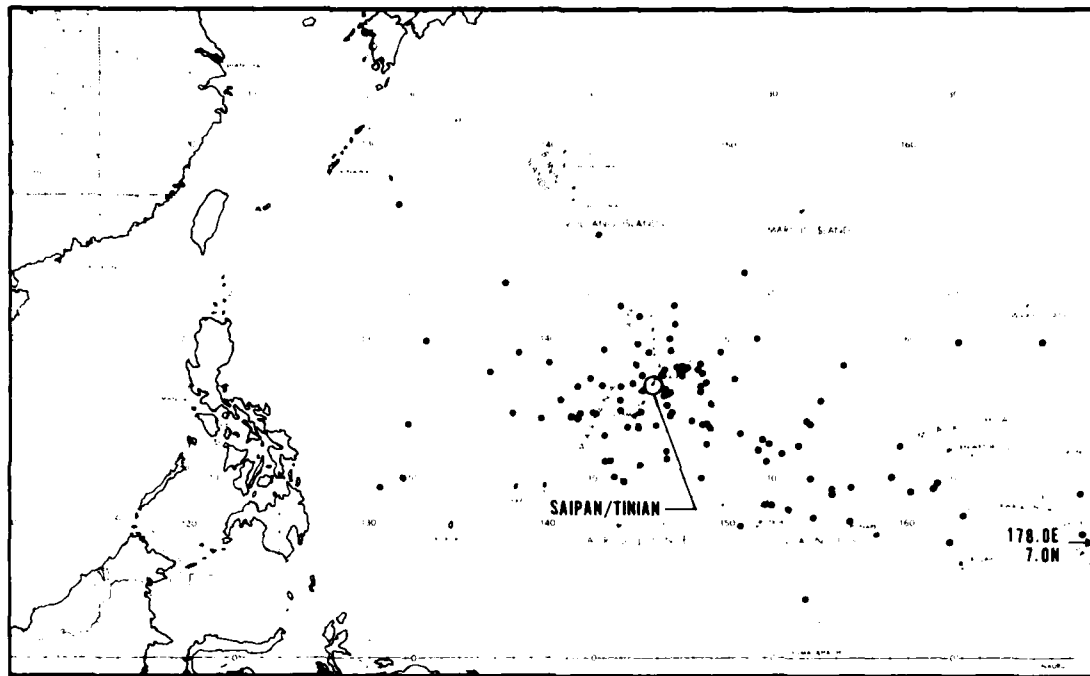
Figure XIV-7. Initial point of attainment of tropical storm intensity (>34 kt) for 126 tropical cyclones passing within 180 n mi of Saipan/Tinian (1947-1977). Since 11 tropical depressions did not achieve the above criteria, only 115 positions are plotted.
