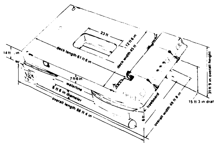
Figure 5. KAIMALINO sketch with dimensions.
