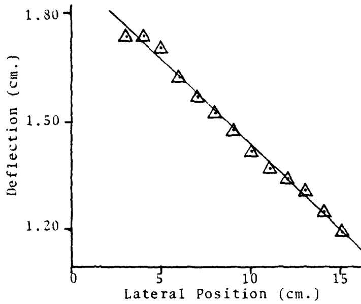
Fig. 28. Deflection Mean (Column) vs Lateral Monitor Position
