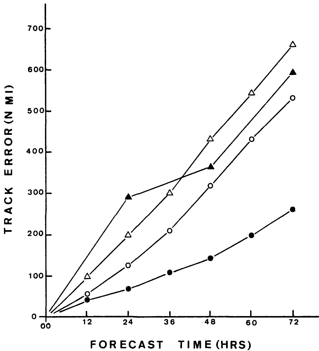
Figure 5. Means of the error vector lengths calculated from the 500 mb independent sample for HATRACK forecasts ( \Delta ), MOHATT forecasts ( \blacktriangle ), STATRAK forecasts (O), and from the 500 mb dependent sample for STATRAK ( \bullet ).
