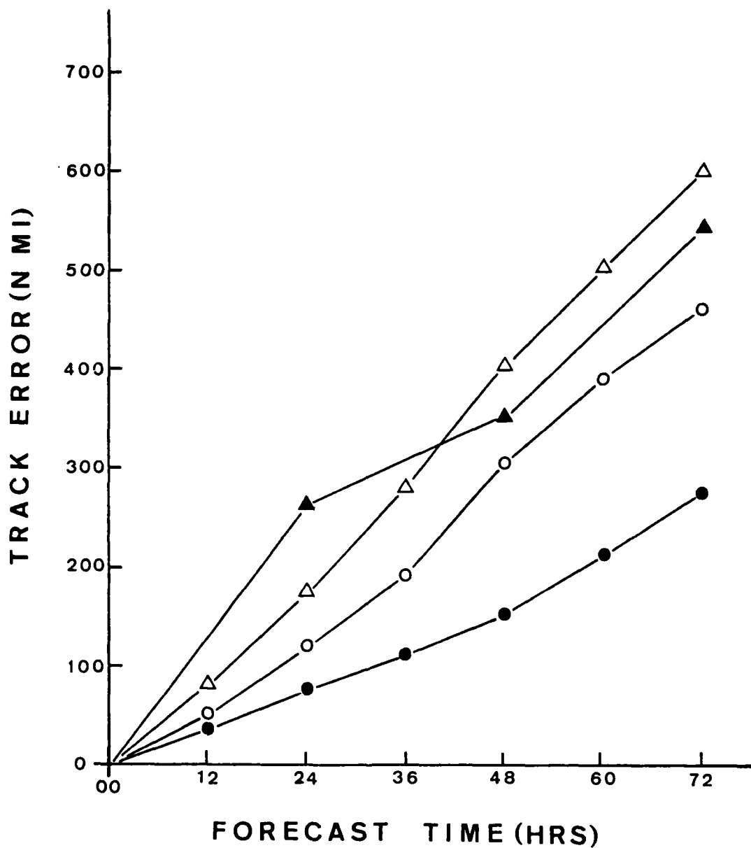
Figure 8. Means of the error vector lengths calculated from the 700 mb independent sample for HATRACK forecasts ( \Delta ), MOHATT forecasts ( \blacktriangle ), STATRAK forecasts (O), and from the 700 mb dependent sample for STATRAK ( \bullet ).
