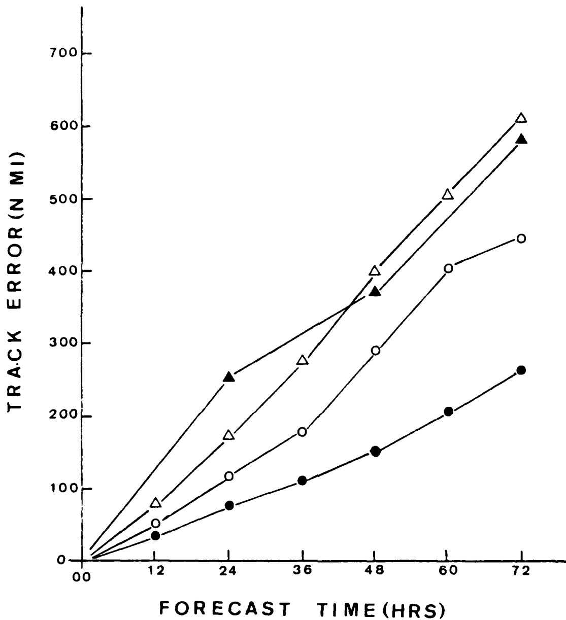
Figure 11. Means of the error vector lengths calculated from the 850 mb independent sample for HATRACK forecasts ( \Delta ), MOHATT forecasts ( \blacktriangle ), STATRAK forecasts ( \circ ), and from the 850 mb dependent sample for STATRAK ( \bullet ).
